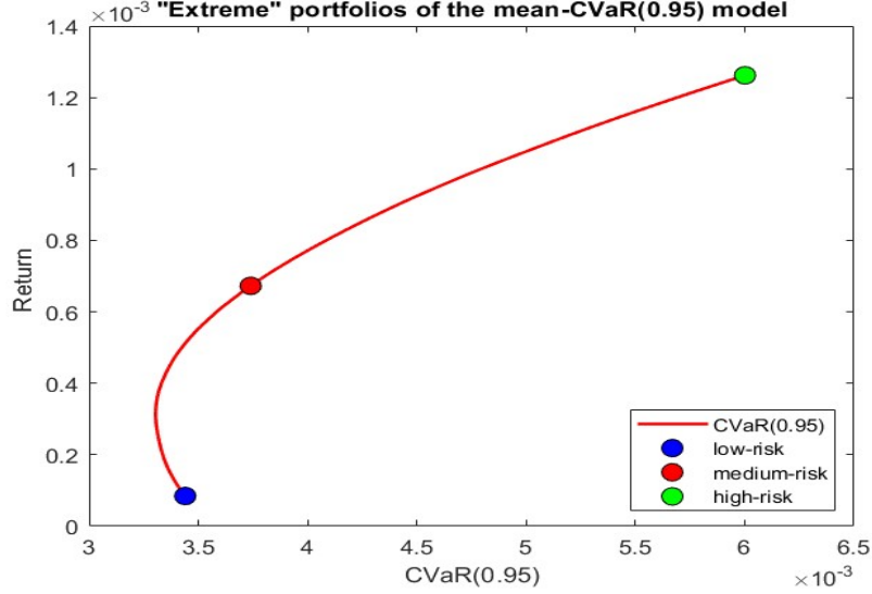
Figure 5.8: Mean-CVaR(0.95) “extreme” portfolios.
