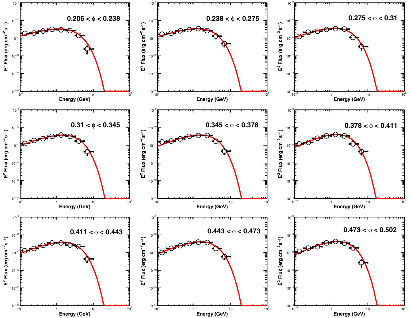
Figure 10. Phase-resolved SEDs of the Geminga pulsar in the phase range \phi = 0.206 – 0.502 . (A color version of this figure is available in the online journal.)
