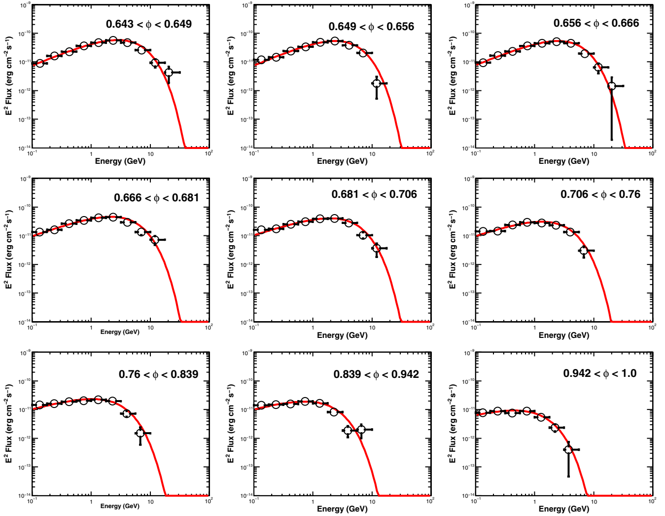
Figure 12. Phase-resolved SEDs of the Geminga pulsar in the phase range \phi = 0.643 – 1.0 .
