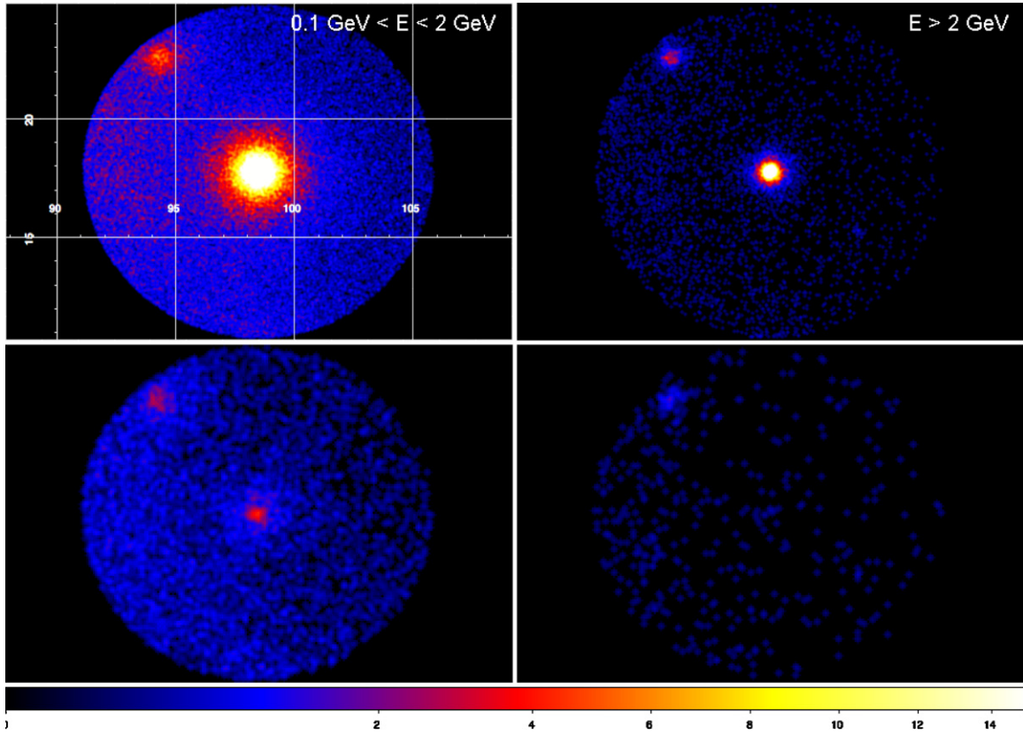
Figure 8. Maps representing the phase interval ( \phi = 0.0\text{--}0.9 , top row) compared to the second interpeak ( \phi = 0.9\text{--}1.0 , bottom row), in the two energy bands 0.1\text{--}2\text{ GeV} and >2\text{ GeV} . Each map represents the photons within 7^\circ from Geminga, binned in pixels of 0.045 (top row) and 0.09 (bottom row), smoothed with a Gaussian filter with a radius of 2 pixels. In the upper left panel, we reported the right ascension in the horizontal axis and the declination in the vertical axis. Bottom row shows that the off-peak point source image is visible at low energies but vanishes at E > 2\text{ GeV} due to the spectral cutoff.
