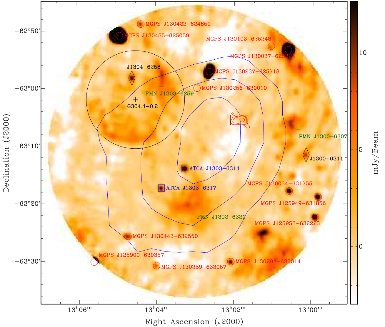
Fig. 2. Radio map of the HESS J1303–631 region at 1.384 GHz. Red contours represent the X-ray PWN as detected with XMM-Newton and blue contours represent HESS J1303–631 as detected by H.E.S.S. (Abramowski et al. 2012). The black circle indicates the SNR candidate G304.4–0.2 and the black cross indicates its centre. MGPS-2 catalogue sources (Murphy et al. 2007) are shown as red circles; PMN survey sources (Condon et al. 1993), excluding those which are coincident with MGPS-2 sources, are shown as green crosses and two ATCA sources (Schinzel et al. 2015) are shown as blue squares. The two new point-like radio sources reported in this paper are indicated with black diamonds. The synthesised beam is determined by an ellipse with the major and minor axes of 51.3'' and 43.8'', respectively, and the positional angle of 20.9°.
