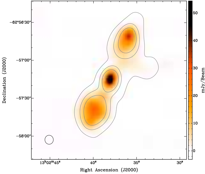
Fig. 3. Radio map of MGPS J130237–625718 at 2.368 GHz overlaid with contours indicating the significance of the emission at 1.384 GHz at the level of 10, 40, and 80 times the rms noise. The synthesised beam is shown with a black ellipse in the bottom left corner.
