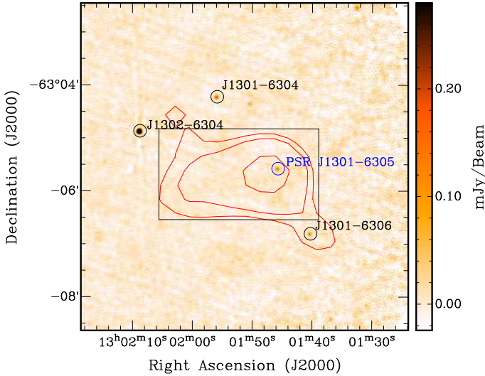
Fig. 1. Radio map of the HESS J1303–631 region at 5.5 GHz overlaid with contours of the X-ray PWN (red) as detected with XMM-Newton (Abramowski et al. 2012). X-ray contours show the peak of the emission close to the pulsar with a trail expanding in the eastern direction. The blue circle indicates the position of the pulsar PSR J1301–6305. The black box determines the region used for the flux density upper limit calculation. New point-like sources are indicated with index numbers. The synthesised beam is determined by an ellipse with the major and minor axes of 3.79'' and 3.65'', respectively, and the positional angle of -7.6^\circ .
