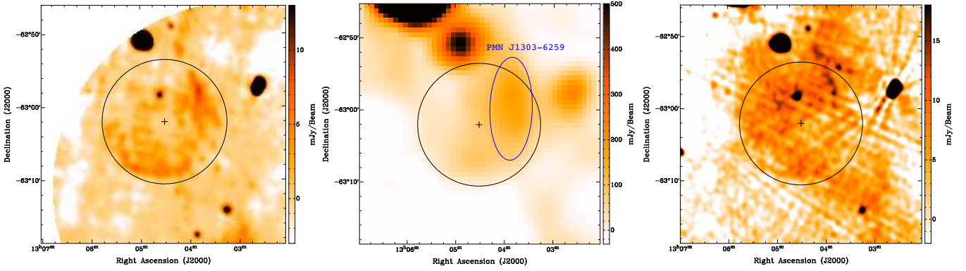
Fig. 4. Left: radio map of the G304.4–0.2 region at 1.384 GHz. Middle: radio map of the G304.4–0.2 region at 4.85 GHz obtained in the PMN survey (Condon et al. 1993). The blue ellipse shows the extension of the PMN survey source PMN J1303–6259 as presented in the catalogue (Wright et al. 1994). The resolution of this map is \sim 5' (Condon et al. 1993). Right: radio map of the G304.4–0.2 region at 843 MHz obtained in the MGPS-2 survey (Murphy et al. 2007). The size of the beam is \sim 45'' \times 50'' . The black circle in all the panels indicates the extension of the shell-like structure and the black cross shows its centre. Middle and right images were obtained using the NASA SkyView online tool ( http://skyview.gsfc.nasa.gov ).
