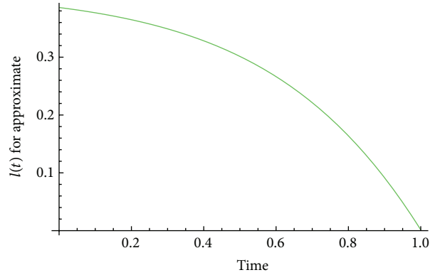
FIGURE 1: Approximated solution.
