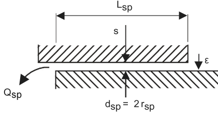
Fig. 1. Geometry of single stage annular seal (Gulich, 2014).
