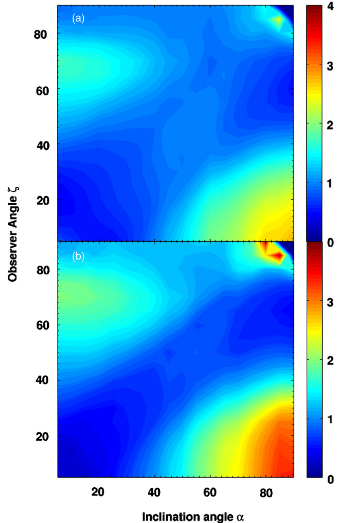
Figure 23. Flux correction factor f_{\Omega}(\alpha, \zeta, P) vs. \alpha and \zeta for a PC2 model, with panels (a) and (b) for P = 2 ms and P = 5 ms, respectively. (A color version of this figure is available in the online journal.)
