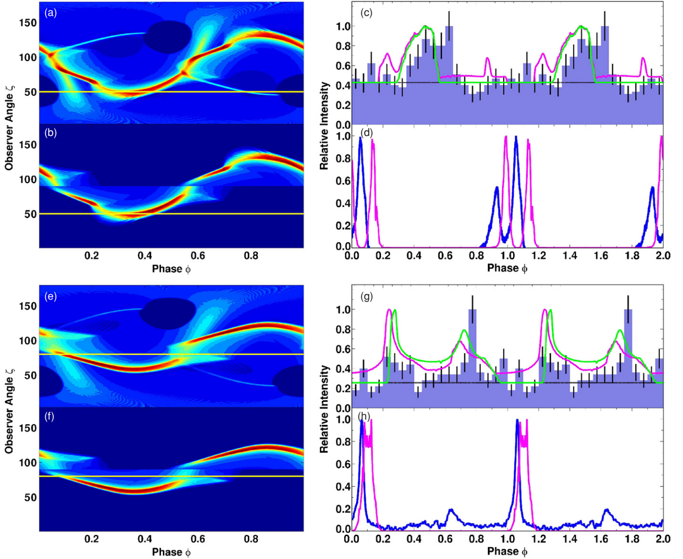
Figure 18. Same as Figure 16, but for PSR J0751+1807 (panels (a)–(d), P = 3 ms) and PSR J16142–230 (panels (e)–(h), P = 3 ms). Panel (a) is for a TPC2 model with (\alpha, \zeta) = (50^\circ, 50^\circ) , (b) for an OG1 model with (\alpha, \zeta) = (50^\circ, 50^\circ) , (e) for a TPC2 model with (\alpha, \zeta) = (40^\circ, 80^\circ) , and (f) for an OG1 model with (\alpha, \zeta) = (40^\circ, 80^\circ) .
