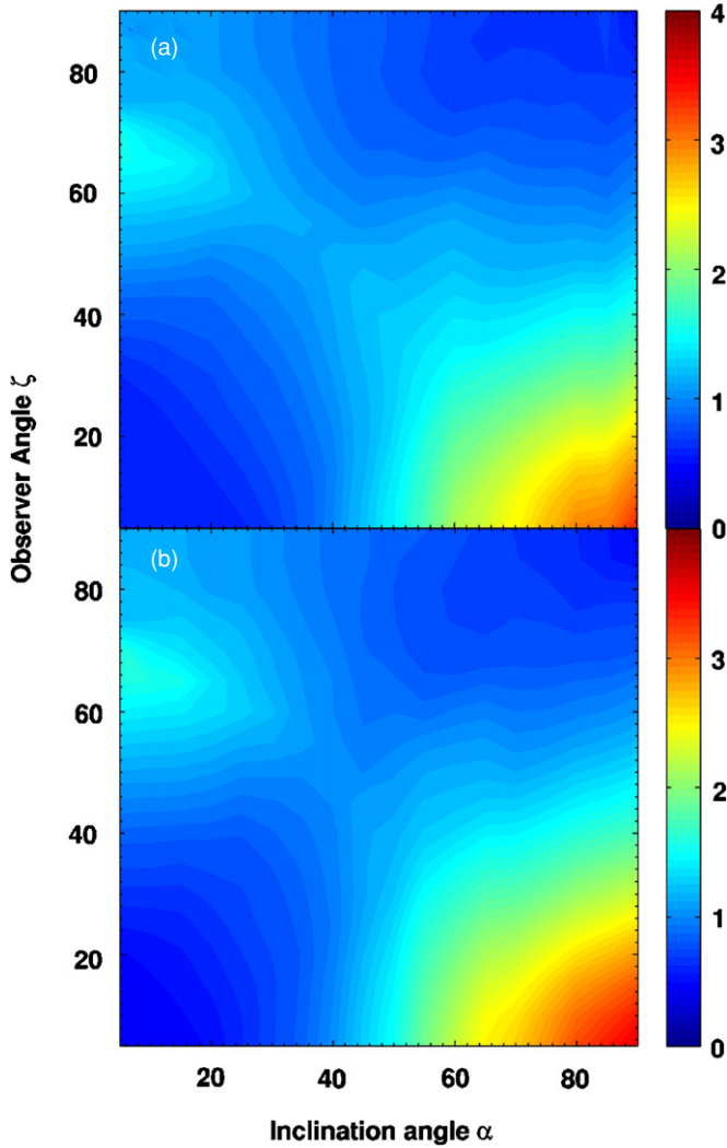
Figure 22. Flux correction factor f_{\Omega}(\alpha, \zeta, P) vs. \alpha and \zeta for a PC1 model, with panels (a) and (b) for P = 2 ms and P = 5 ms, respectively. (A color version of this figure is available in the online journal.)
