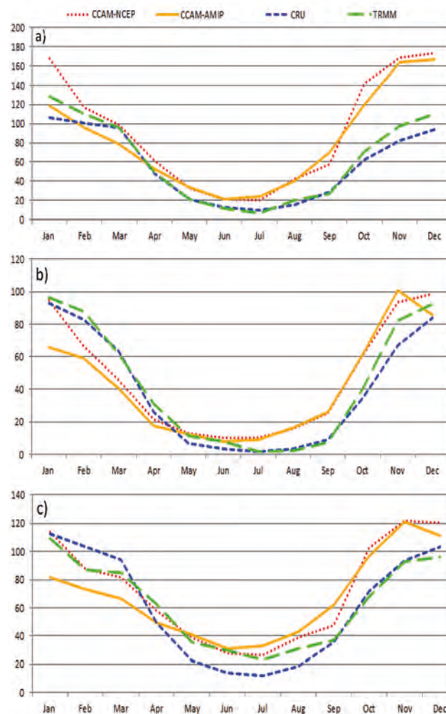
Figure 9 Intra-annual area-averaged rainfall totals (mm) for CCAM-AMIP (1979–2005), CCAM-NCEP (1979–2005), CRU (1979–2005) and TRMM (1998–2012) over the regions of a) LES, b) NESA and c) ESA
