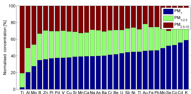
Figure 3. Mean size distributions of individual trace metal species detected. Species are arranged by increasing concentration in the PM_1 size fraction.
