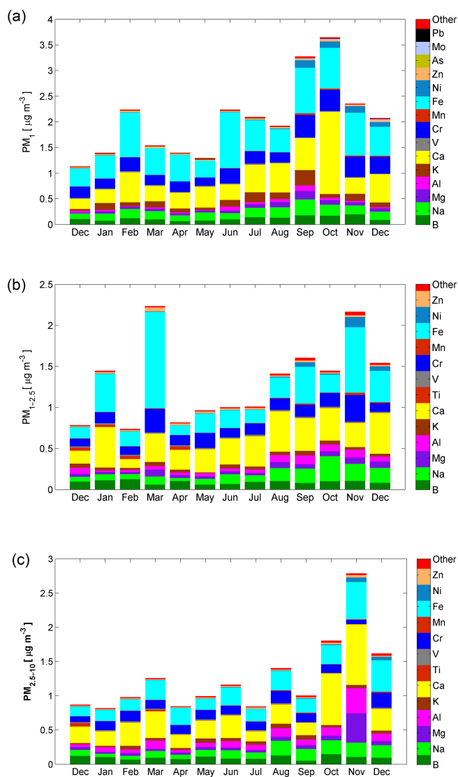
Figure 4. The monthly median trace metal concentrations in the \text{PM}_1 (a), \text{PM}_{1-2.5} (b) and \text{PM}_{2.5-10} (c) size fractions.
