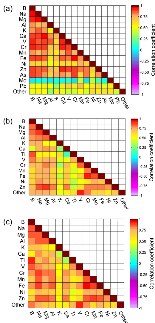
Figure 5. Spearman correlations of trace metal species in the \text{PM}_1 (a), \text{PM}_{1-2.5} (b) and \text{PM}_{2.5-10} (c) size fractions.
