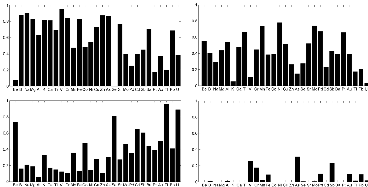
Figure 6. PCFA of the trace metal concentration in the PM_{10} size fraction. Four dominant factors are identified.
