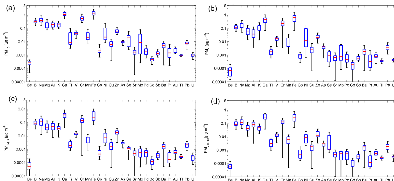
Figure 2. Box-and-whisker plots of trace metal concentrations in the (a) PM_{10} (sum of trace metal concentrations in the three size fractions), (b) PM_1 , (c) PM_{1-2.5} and (d) PM_{2.5-10} size fractions. The red line indicates the median concentrations, the blue rectangle of the box plot represents the 25th and 75th percentiles, and the whiskers indicate \pm 2.7 times the standard deviation.
