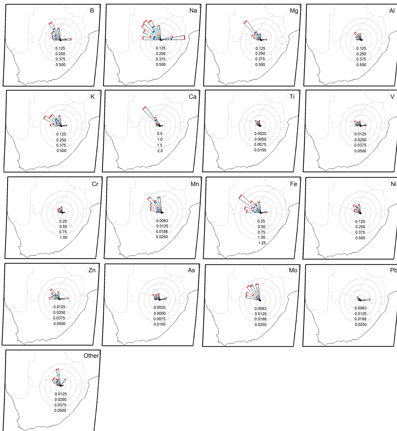
Figure 7. Pollution roses of trace metal species that were 25 % or more of the time detected with the analytical technique.
