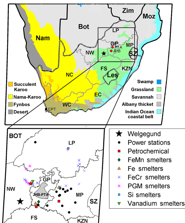
Figure 1. A bio-geographical map indicating Welgegund (black star), as well as the major point sources and the Johannesburg–Pretoria (JHB-PTA) conurbation. Neighbouring countries to South Africa (Nam: Namibia; Bot: Botswana; Zim: Zimbabwe; Mos: Mozambique; SZ: Swaziland; Les: Lesotho) as well as South African provinces (LP: Limpopo; NW: North West; FS: Free State; KZN: Kwa-Zulu Natal; MP: Mpumalanga; NC: Northern Cape; EC: Eastern Cape; WC: Western Cape) are also indicated.
