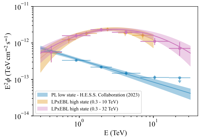
Fig. 2. Detected spectral energy distribution of M 87 data with H.E.S.S. The best-fit LPxEBL finke2022 spectral models are shown in yellow for the reduced energy range (0.3–10 TeV) and in purple for the full energy range (0.3–32 TeV). The best-fit PL spectrum for the low-state data (based on H.E.S.S. Collaboration 2023) is shown for comparison in blue. The color bands show the 1\sigma uncertainty contours. The upper limit (UL) in the last bin of the low-state spectrum is defined at a 95% confidence level (c.l.).
