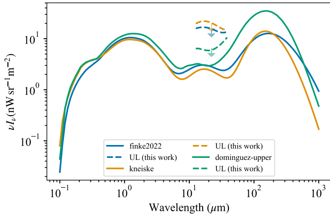
Fig. A.2. EBL photon distribution based on the three models employed in this study - kneiske , finke2022 , and dominguez-upper models - is depicted in orange, blue, and green, respectively. The 95% confidence level upper limits (ULs) derived from fitting the high state, as defined in the main text, to LPxEBL models are represented by dashed lines.
