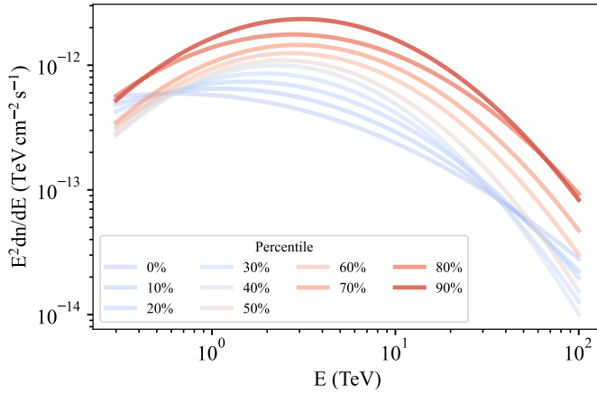
Fig. B.2. Best spectral fits for the LPxEBL models are illustrated for the various datasets, revealing the emergence of a curved spectrum in the high state.
