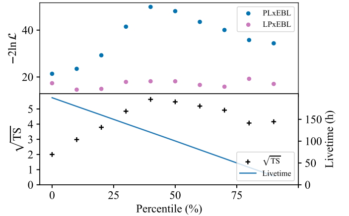
Fig. B.1. TS distribution for the PLxEBL (blue) and LPxEBL (purple) models, incorporating the finke2022 EBL model, is analyzed in relation to datasets defined by the flux distribution above 1 TeV. Each dataset encompasses observations with flux surpassing a specified percentile. The lower panel presents the distribution of \sqrt{TS} denoted by black crosses, while the solid line illustrates the dataset's livetime distribution.
