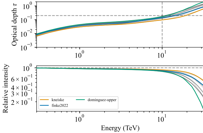
Fig. A.1. Optical depth (top) and the relative intensity of the gamma-ray flux after absorption (bottom) at z=0.0042 of the three EBL models employed in this study are presented based on the information provided in the table from Meyer (2022). The two dashed lines in the upper panel indicate the energy and attenuation levels at which we deem the influence of the EBL spectrum on the overall spectrum as non-negligible. Additionally, for comparison, the remaining available EBL models are depicted in faded black. In the bottom panel, a reference dashed line is provided to guide the eyes in the case of no absorption.
