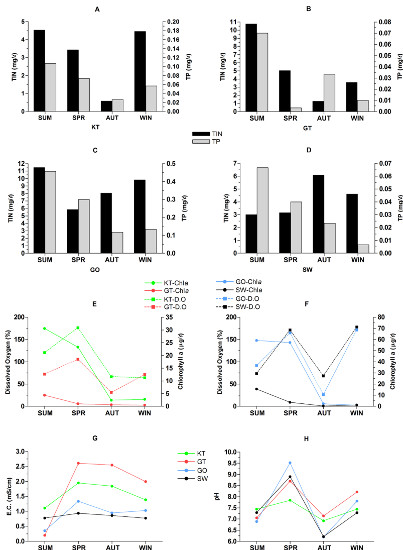
Figure 2 Seasonal fluctuations in TIN (total inorganic nitrogen), TP (total inorganic phosphorus), chlorophyll a, dissolved oxygen, electrical conductivity (EC) and pH for the four reed pans.
