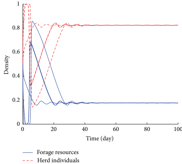
FIGURE 4: Chronological evolution of the herd's animals and forage resources of System (1) when r = 500 kgDM/ha, e = 0.05 /day, a = 0.013 /ha, K = 10-40 kgDM/ha, q = 0.4 /day, and \gamma = 0.07 /day. Stability of the coexisting equilibrium E_2 = (R^*, H^*) .
