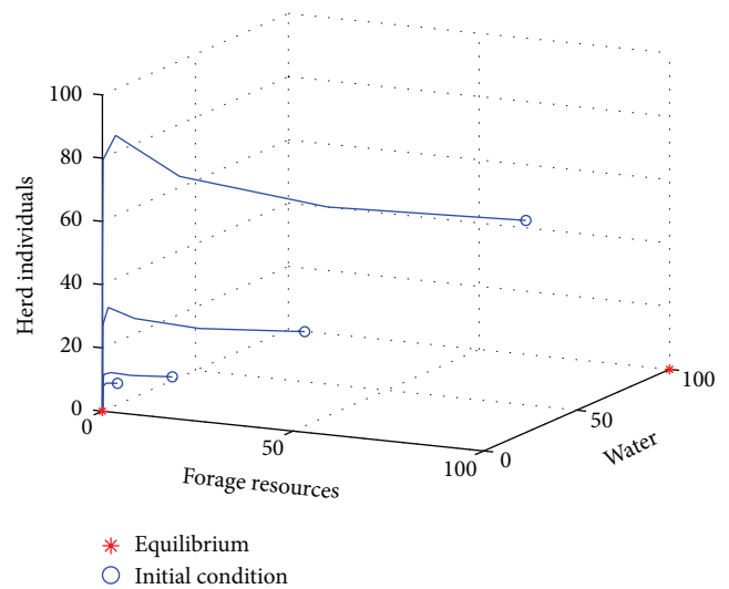
FIGURE 9: Phase portrait corresponding to the disappearing of forage resources and water resources and removal of the pastoralists with their herds for System (2). We can observe here the global asymptotic stability of E_{10} = (0, 0, 0) when r_1 = -0.4 < 0 and r_2 = -60 < 0 . The rest of parameters are in Tables 1 and 2.
