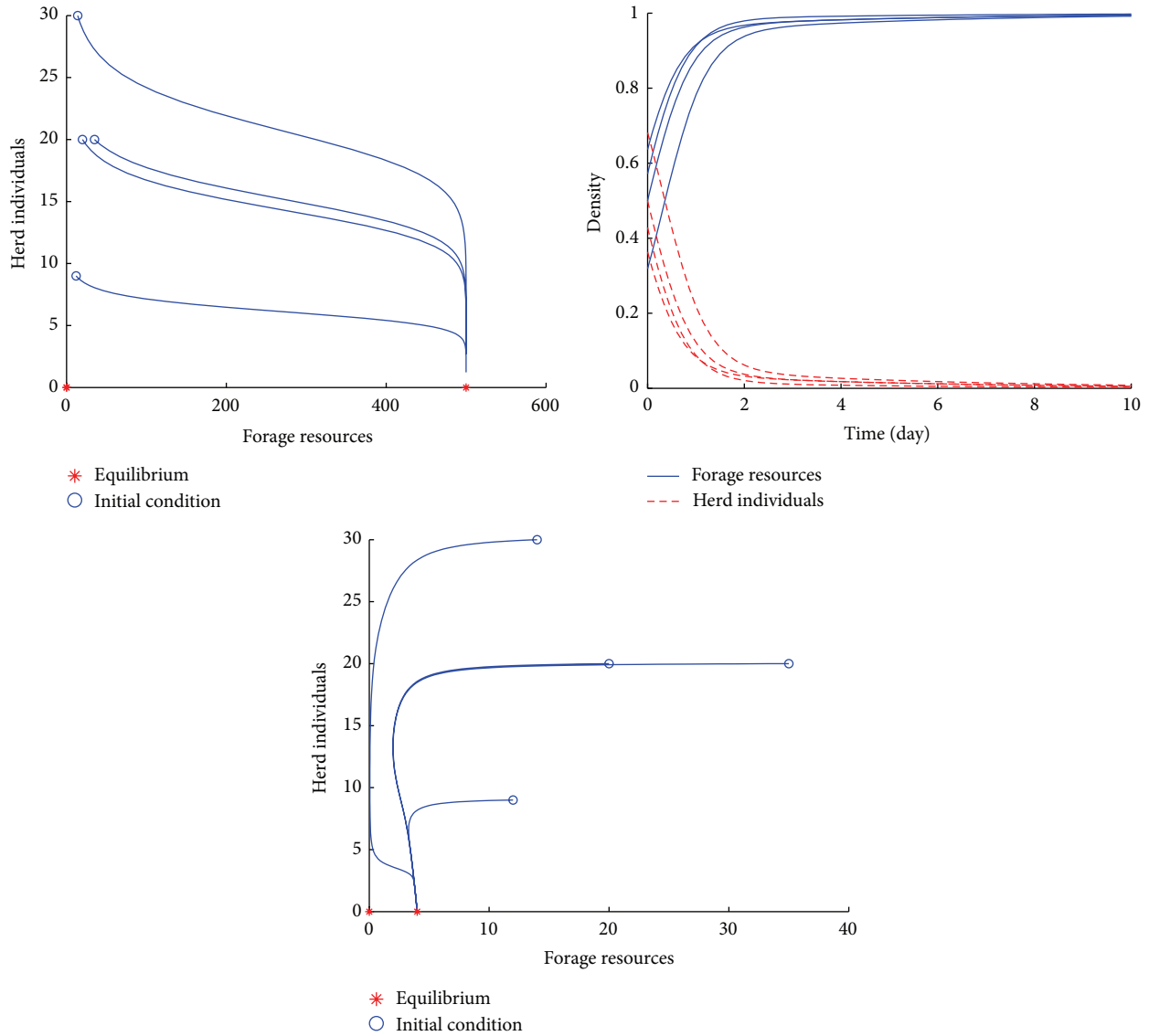
FIGURE 3: Chronological evolution and phase portrait of the herd individuals and forage resources of System (1) when r_{01} = 200 kgDM/ha, r_{02} = 55 kgDM/ha, r_1 = 80 kgDM/ha, K = 30-600 kgDM/ha, e = 0.05 /day, a = 0.013 /ha, q = 0.4 /day, and \gamma = 0.07 /day. Global stability of equilibrium E_1 = (K, 0) for System (1). This illustrates the case when pastoralists decide to migrate for reasons different from unavailability of forage resources.
