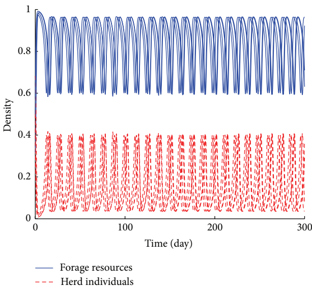
FIGURE 7: Chronological evolution of the herd’s animals and forage resources of System (1) when r = 650 kgDM/ha, e = 0.05 /day, a = 0.013 /ha, K = 800 kgDM/ha, q = 0.4 /day, and \gamma = 1.0 /day. This illustrates the global stability of the unique coexisting equilibrium E_2 = (R^*, H^*) . This means that the herd’s animals and forage resources have periodic curves since there is a stable limit cycle. The two populations can exist together.
