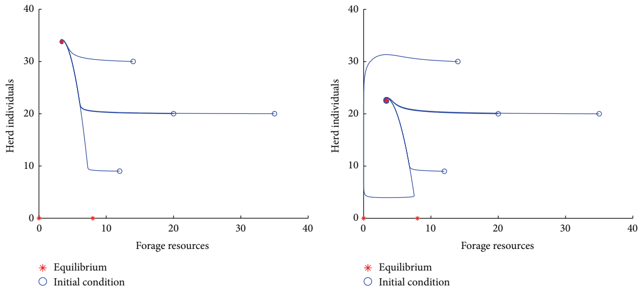
FIGURE 5: Phase portrait of the herd's animals and forage resources of System (1) when r = 500 kgDM/ha, e = 0.05 /day, a = 0.013 /ha, K = 8-30 kgDM/ha, q = 0.4 /day, and \gamma = 0.07 /day. Illustration of the stability of the unique coexisting equilibrium E_2 = (R^*, H^*) for four initial conditions.
