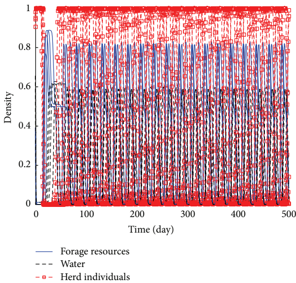
FIGURE 11: Illustration of periodicity of the trajectories at equilibrium E_2 = (R^*, W^*, H^*) for System (2). Alternative peaks are observed between the trajectories of the flock, feed resources, and water resources when r_1 = 800 kgDM/ha, r_2 = 700 kgDM/ha, p = 600 mm, K_1 = 1000 kgDM/ha, and K_2 = 900 kgDM/ha. The rest of parameters are in Tables 1 and 2.
