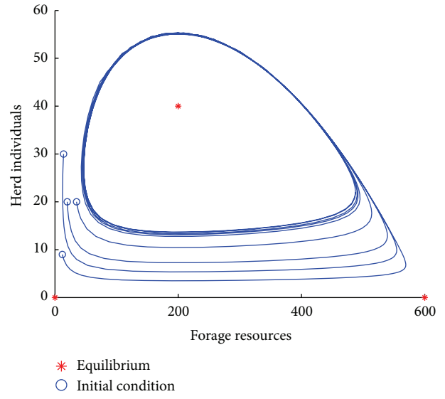
FIGURE 8: Phase portrait for illustration of a stable limit cycle around coexisting equilibrium of System (1) for E_2 = (R^*, H^*) for r = 700 kgDM/ha, e = 0.05 /day, a = 0.013 /ha, K = 960 kgDM/ha, q = 0.4 /day, and \gamma = 1.0 /day. This means that there is a supercritical Hopf bifurcation.
