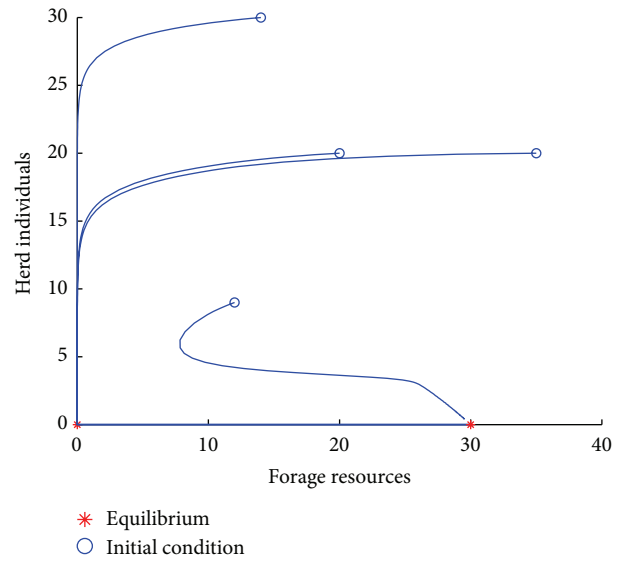
FIGURE 2: Phase portrait of System (1). Illustration of the local asymptotic stability of equilibrium E_0 = (0, 0) and equilibrium E_1 = (K, 0) . These situations happen during transhumance; the pastoralists leave the area because of scarcity of forage resources or some local conditions. The rest of parameters in this case are given in Table 1, with r_{01} = 200 kgDM/ha, r_{02} = 55 kgDM/ha, r_1 = 80 kgDM/ha, and K = 30 kgDM/ha such that r > 0 .
