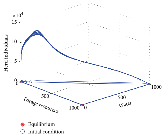
FIGURE 10: Phase portrait of System (2) showing the coexistence of E_{10}, E_{11}, E_{12} . Equilibria E_{11} and E_{12} correspond to the removal of the pastoralists with their herd and persistence of forage or water resources. We can observe here the local asymptotic stability of E_{11} = (K_1, 0, 0) , E_{12} = (0, K_2, 0) , and E_{10} = (0, 0, 0) when r_1 = 400 kgDM/ha and p = 3000 mm. The rest of parameters are in Tables 1 and 2.
