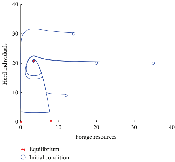
FIGURE 6: Phase portrait of the herd’s animals and forage resources of System (1) when r = 500 kgDM/ha, e = 0.05 /day, a = 0.013 /ha, K = 8\text{--}30 kgDM/ha, q = 0.4 /day, and \gamma = 0.07 /day. Illustration of the stability of the unique coexisting equilibrium E_2 = (R^*, H^*) for four initial conditions.
