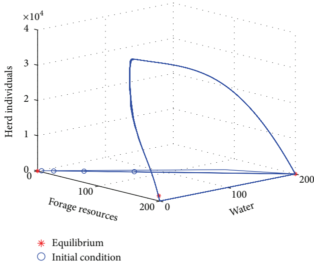
FIGURE 10: Phase portrait of System (2) showing the coexistence of E_{10}, E_{11}, E_{12} . Equilibria E_{11} and E_{12} correspond to the removal of the pastoralists with their herd and persistence of forage or water resources. We can observe here the local asymptotic stability of E_{11} = (K_1, 0, 0) , E_{12} = (0, K_2, 0) , and E_{10} = (0, 0, 0) when r_1 = 400 kgDM/ha and p = 3000 mm. The rest of parameters are in Tables 1 and 2.
