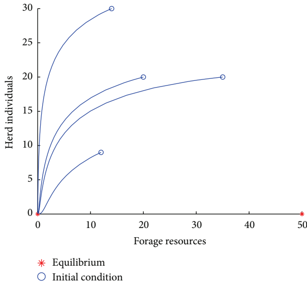
FIGURE 1: Phase portrait of the herd's animals and forage resources when r < 0 . This illustrates the global stability of equilibrium E_0 = (0, 0) for System (1). This is a new situation, which happens during migration of pastoralists with their herds, calling transhumance; the pastoralists leave the area because of scarcity of forage resources. The parameters in this case are given in Table 1.
