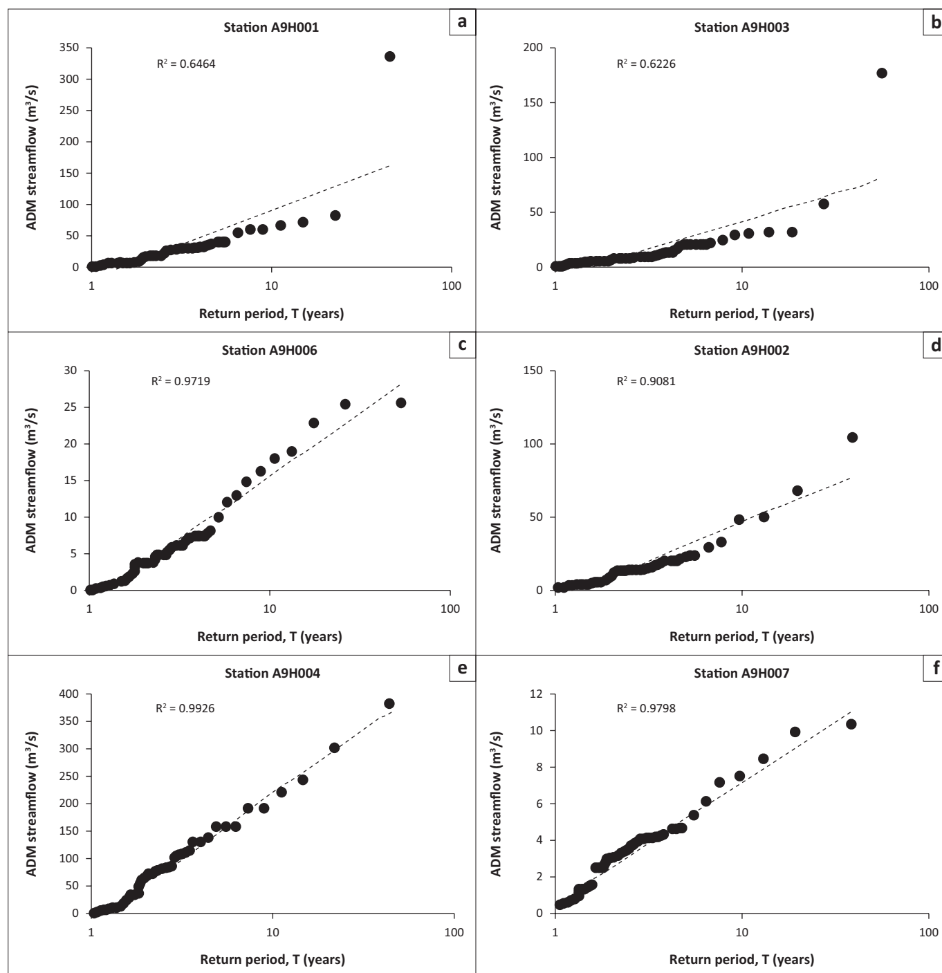
FIGURE 4: Annual daily maximum streamflow versus T_r plot for selected stations in the study area.
