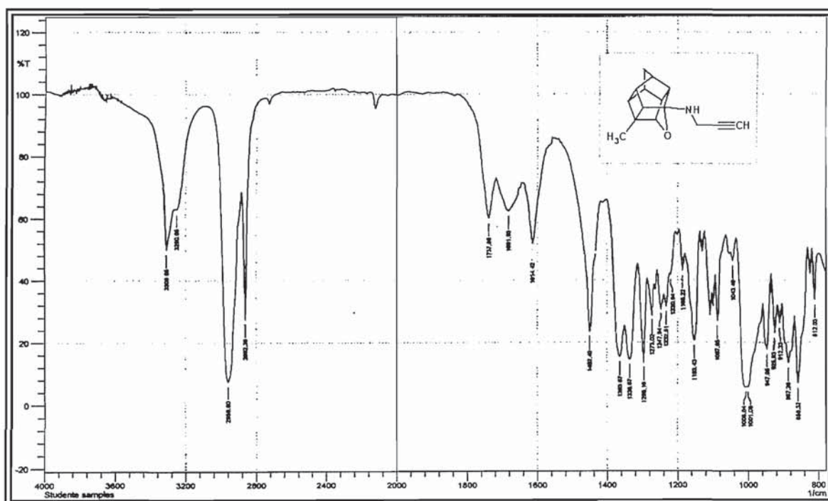
Spectrum 4
