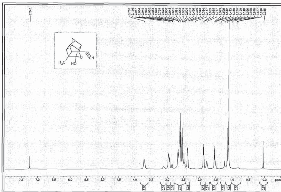
Spectrum 17
