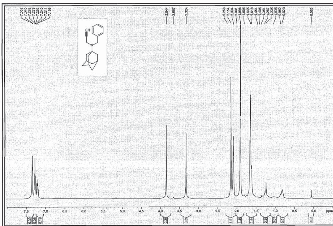
Spectrum 24
