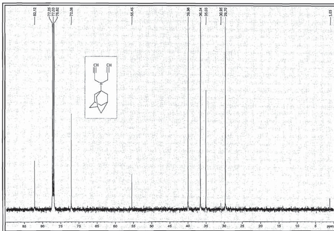
Spectrum 31
