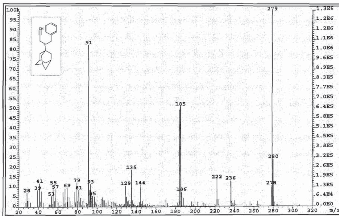
Spectrum 16
