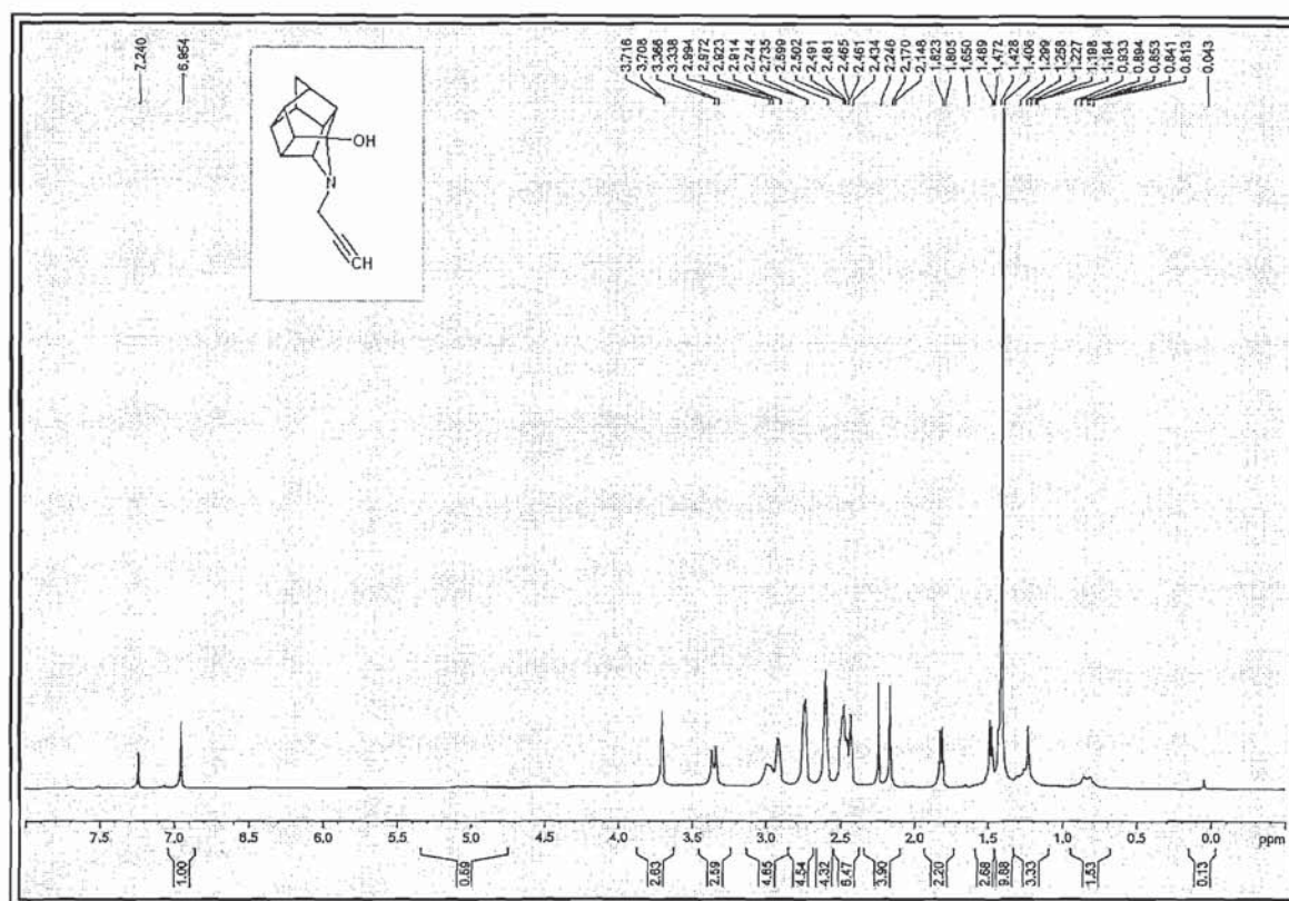
Spectrum 21
