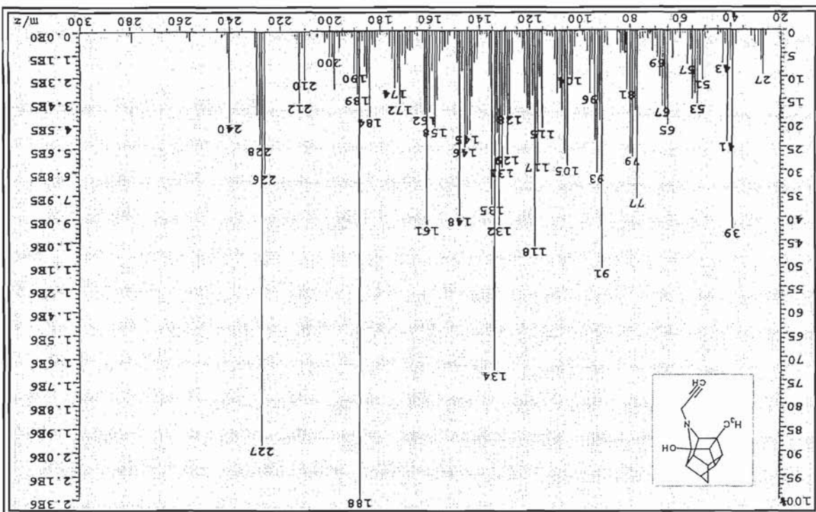
Spectrum 14
