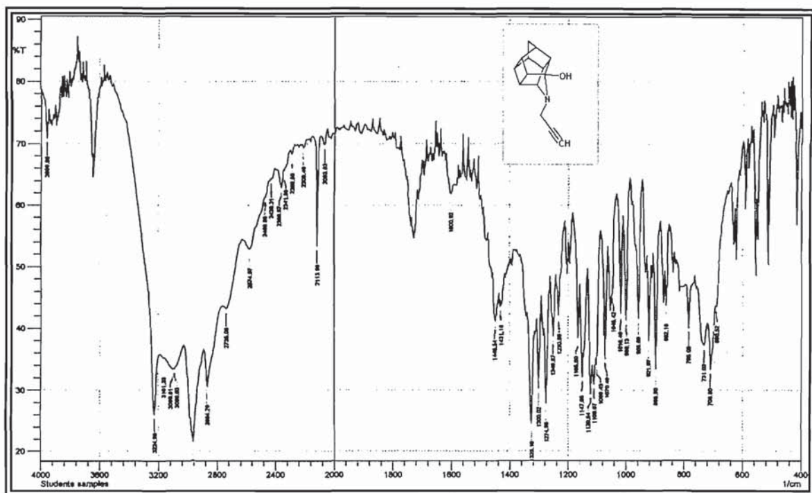
Spectrum 5
