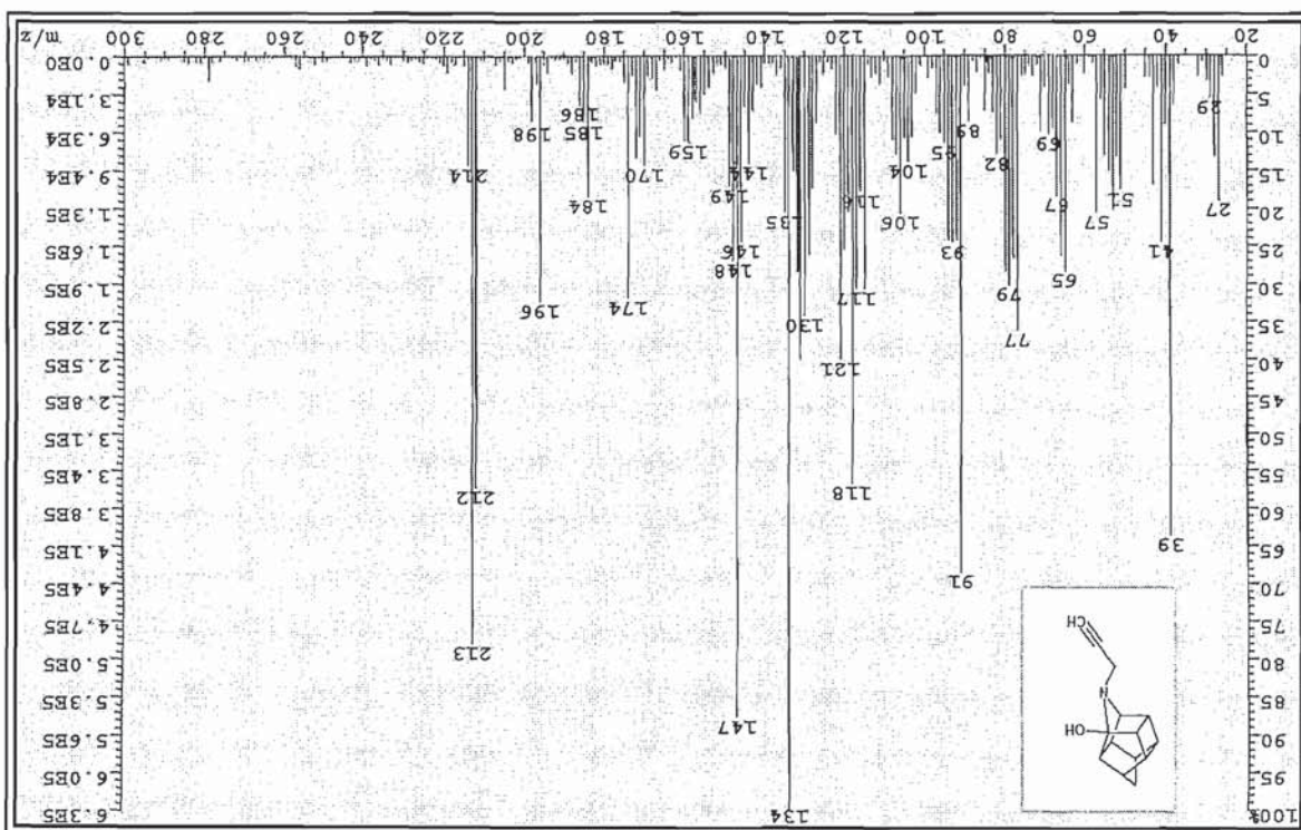
Spectrum 13
