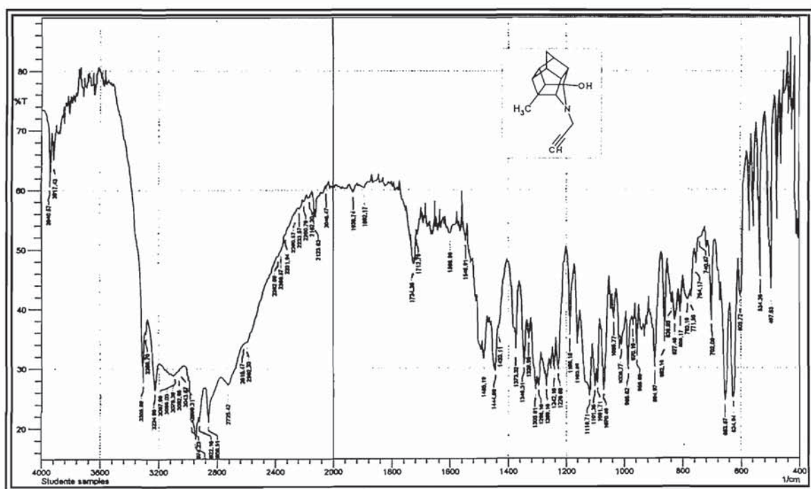
Spectrum 6
