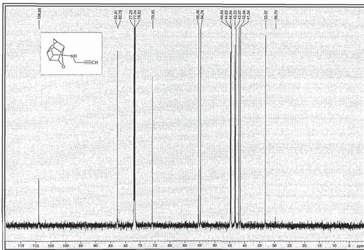
Spectrum 27
