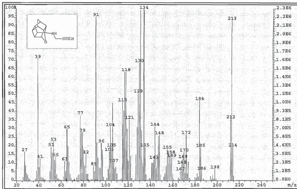
Spectrum 11
