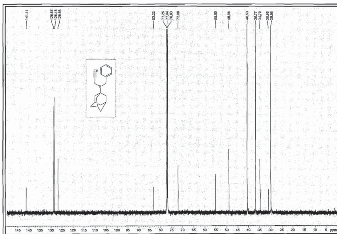
Spectrum 32
