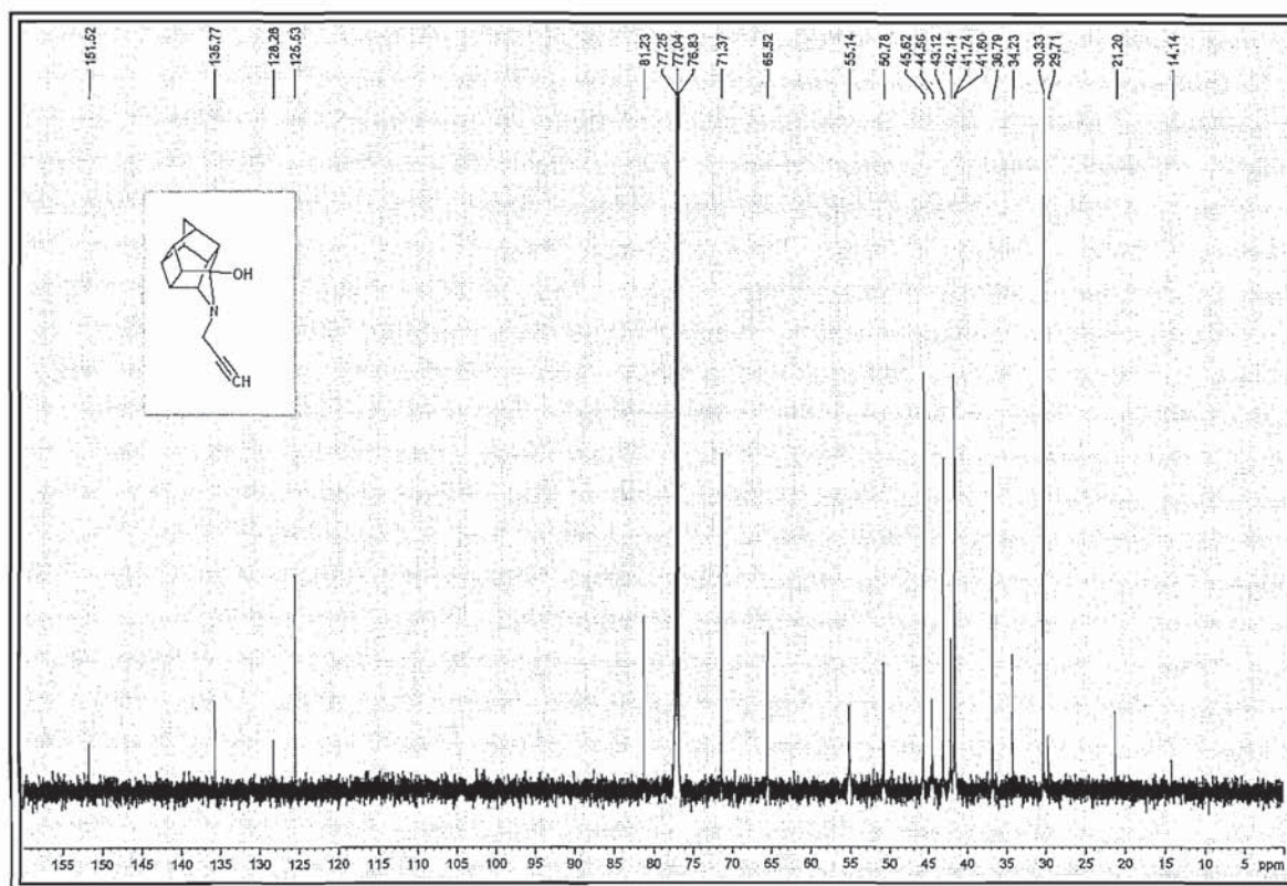
Spectrum 29
