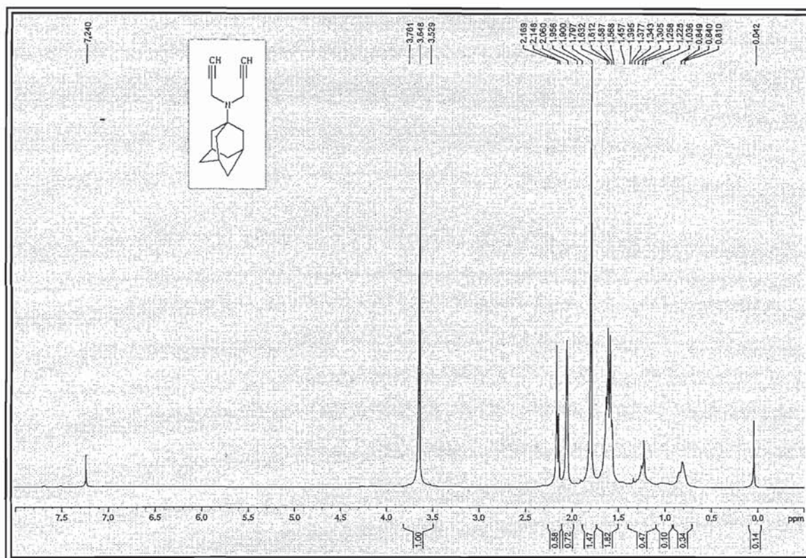
Spectrum 23
