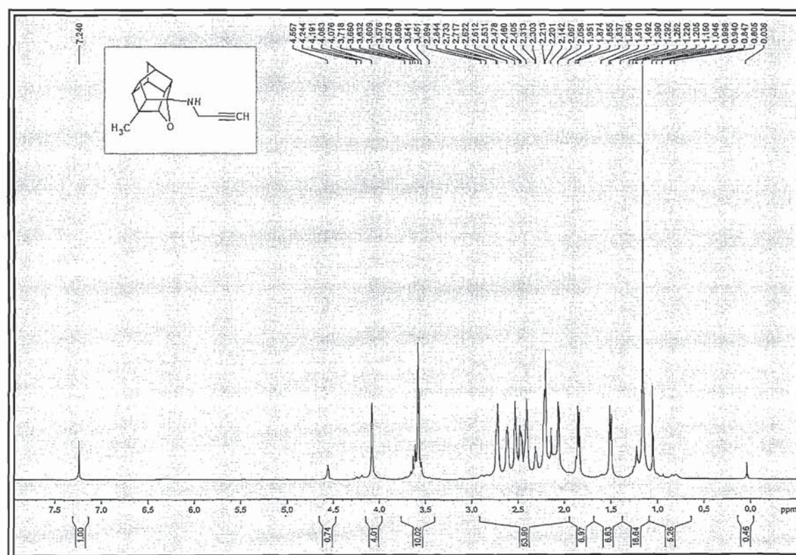
Spectrum 20
