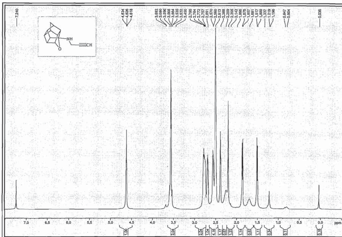
Spectrum 19
