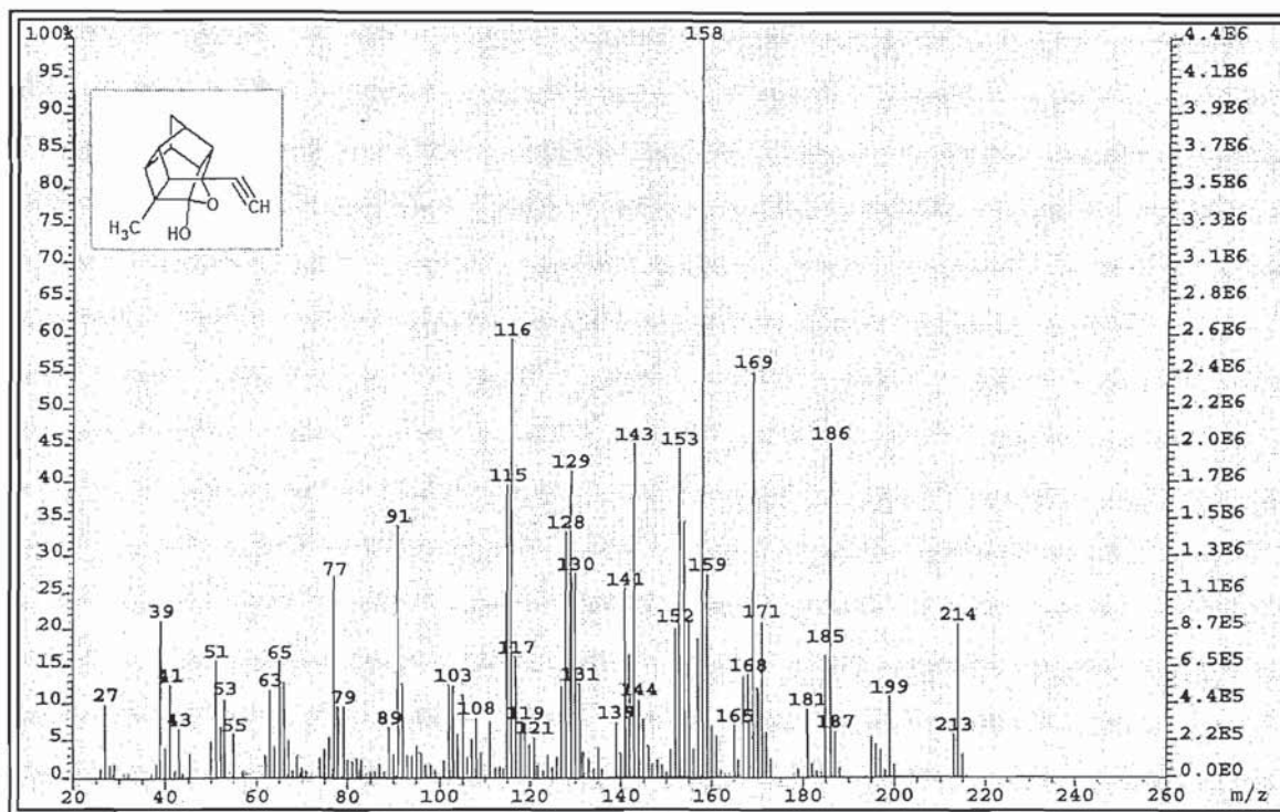
Spectrum 9
