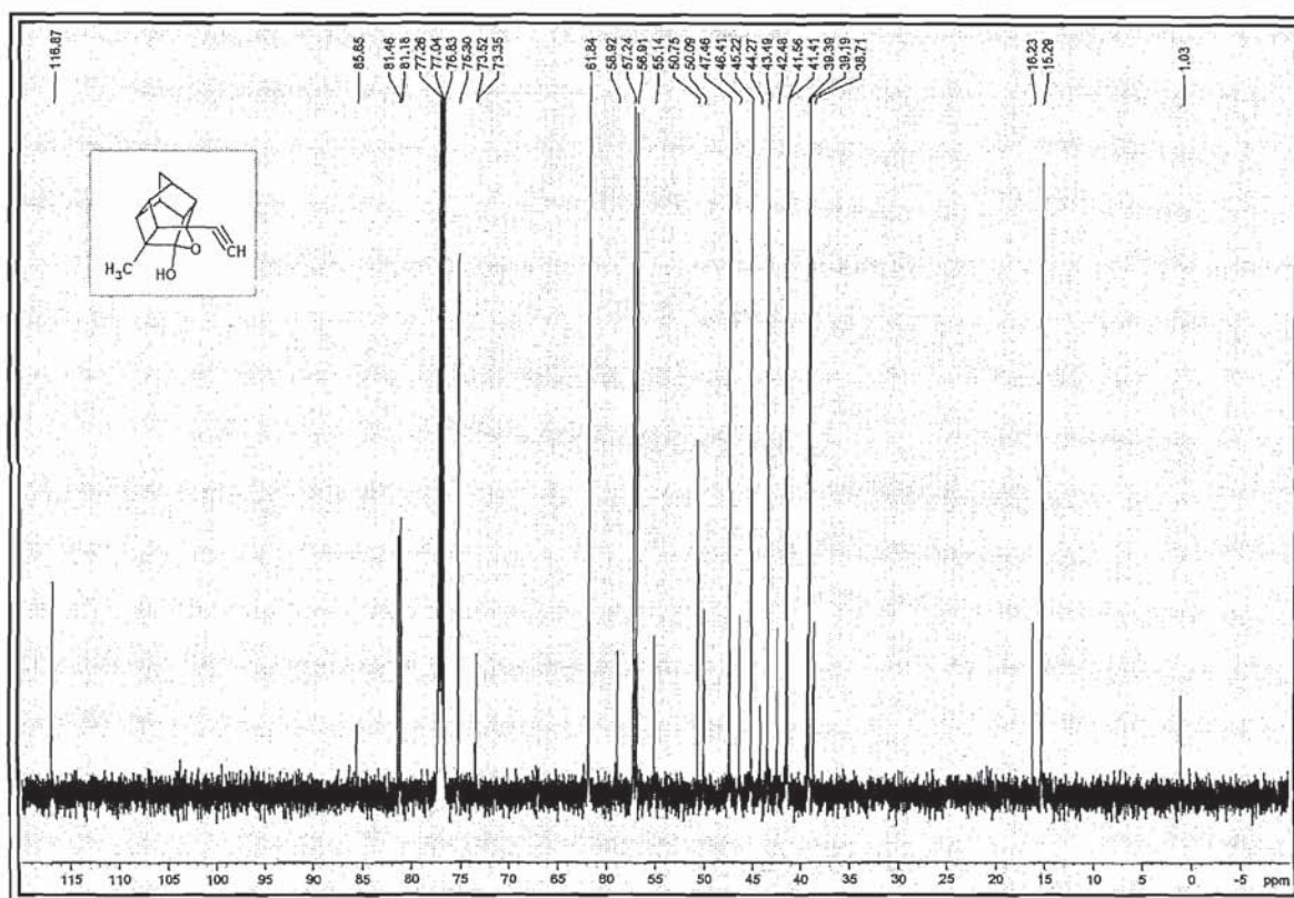
Spectrum 25
