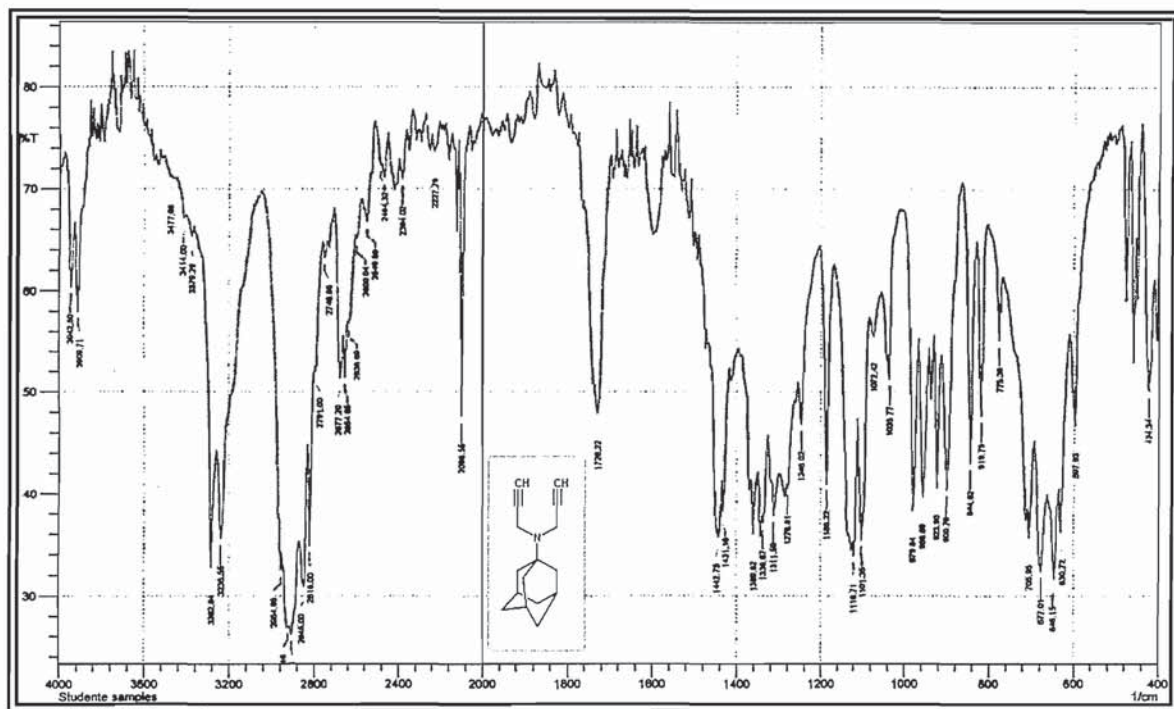
Spectrum 7
