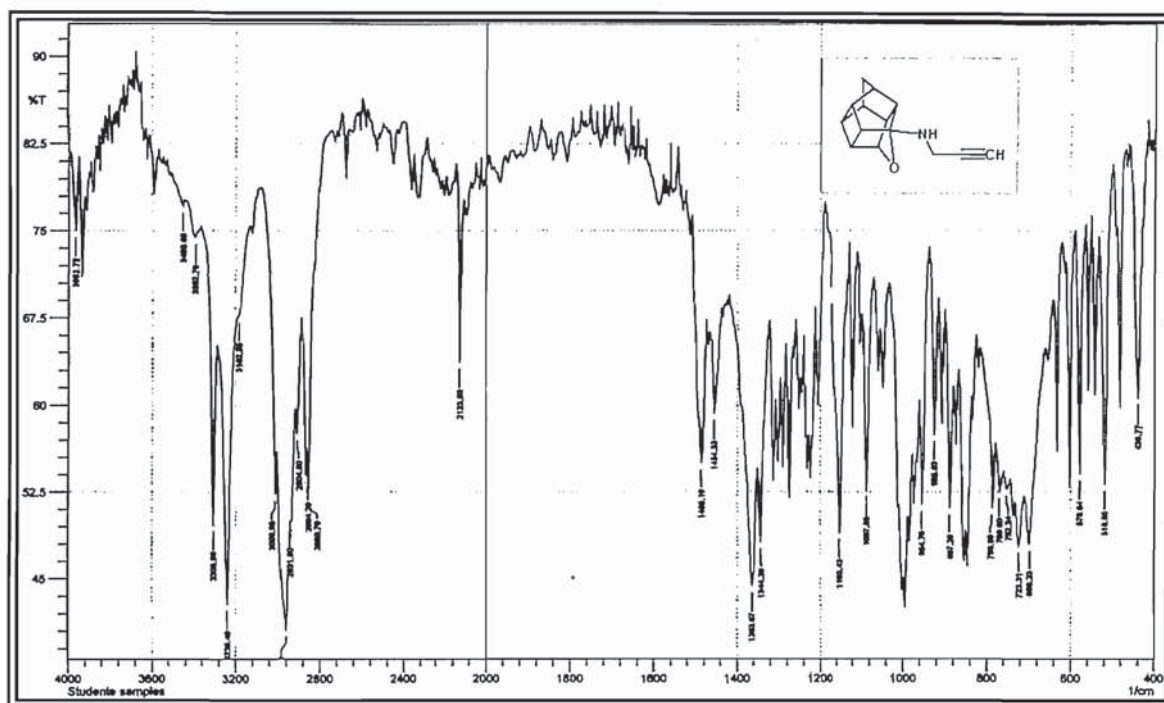
Spectrum 3
