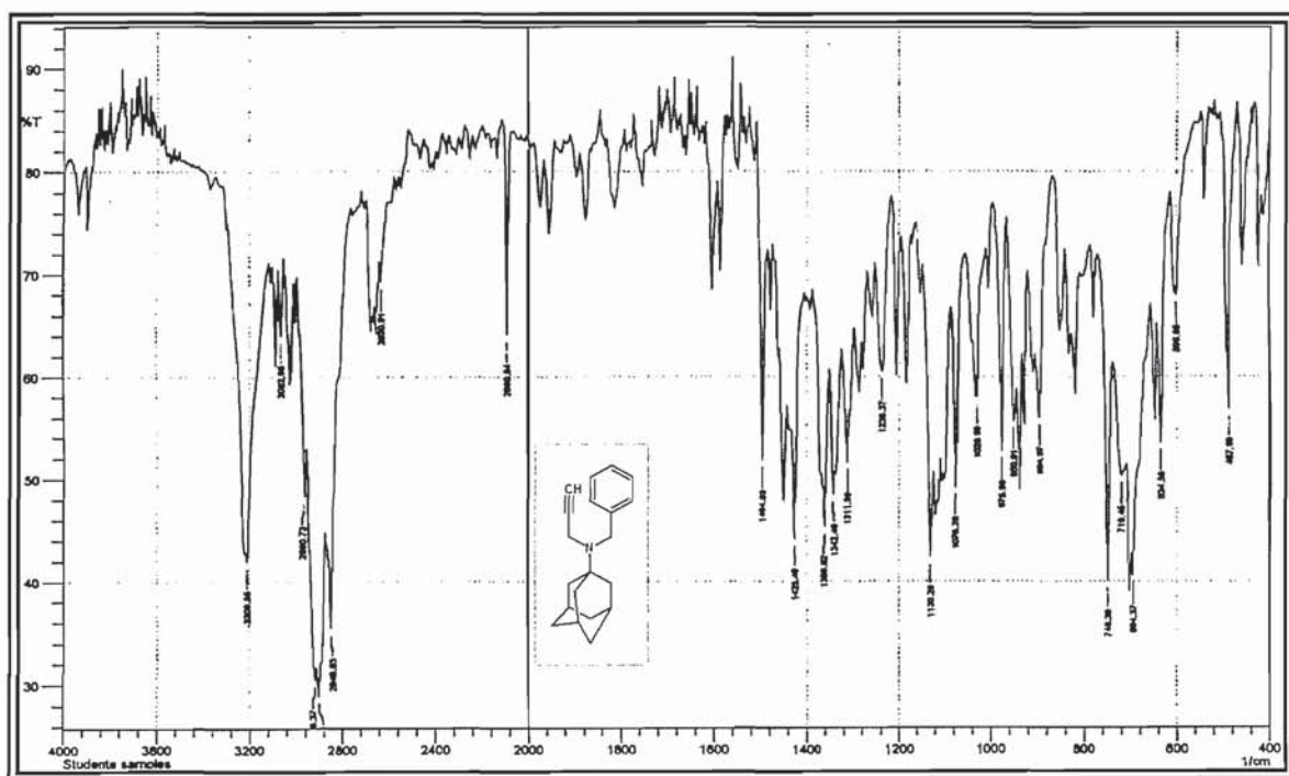
Spectrum 8
