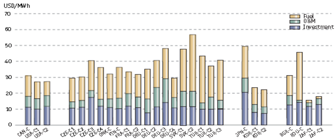
Figure 4.18 Levelized costs of coal generated electricity at 5% discount rate
