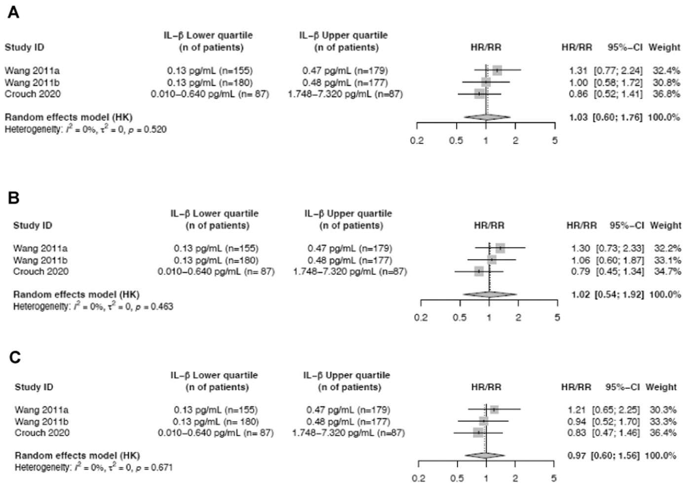
Fig. 3. Forest plots of pooled HR/RR of hypertension for the highest versus lowest quartile of IL-1β. Hazard ratio (HR)/Risk ratio (RR) and 95% confidence interval (CI) from the eligible studies of the association between IL-1β circulating levels and incident hypertension estimates in a random effects model with crude RR/HR pooled in (A), adjusted RR/HR pooled in (B) without BMI and adjusted RR/HR pooled in (C) including BMI.
