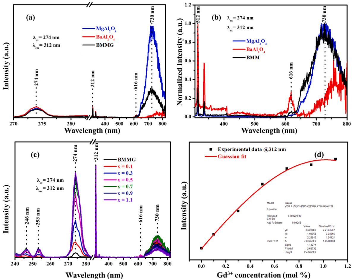
Fig. 8. (a) Emission spectrum of undoped samples ( MgAl_2O_4 , BaAl_2O_4 , and BMM), (b) normalized spectra of the Fig (a), (c) excitation and emission spectrum of the BMM:x% Gd^{3+} ( 0 \leq x \leq 1.1 ) and (d) emission intensity at 312 nm as a function of Gd^{3+} concentration.
