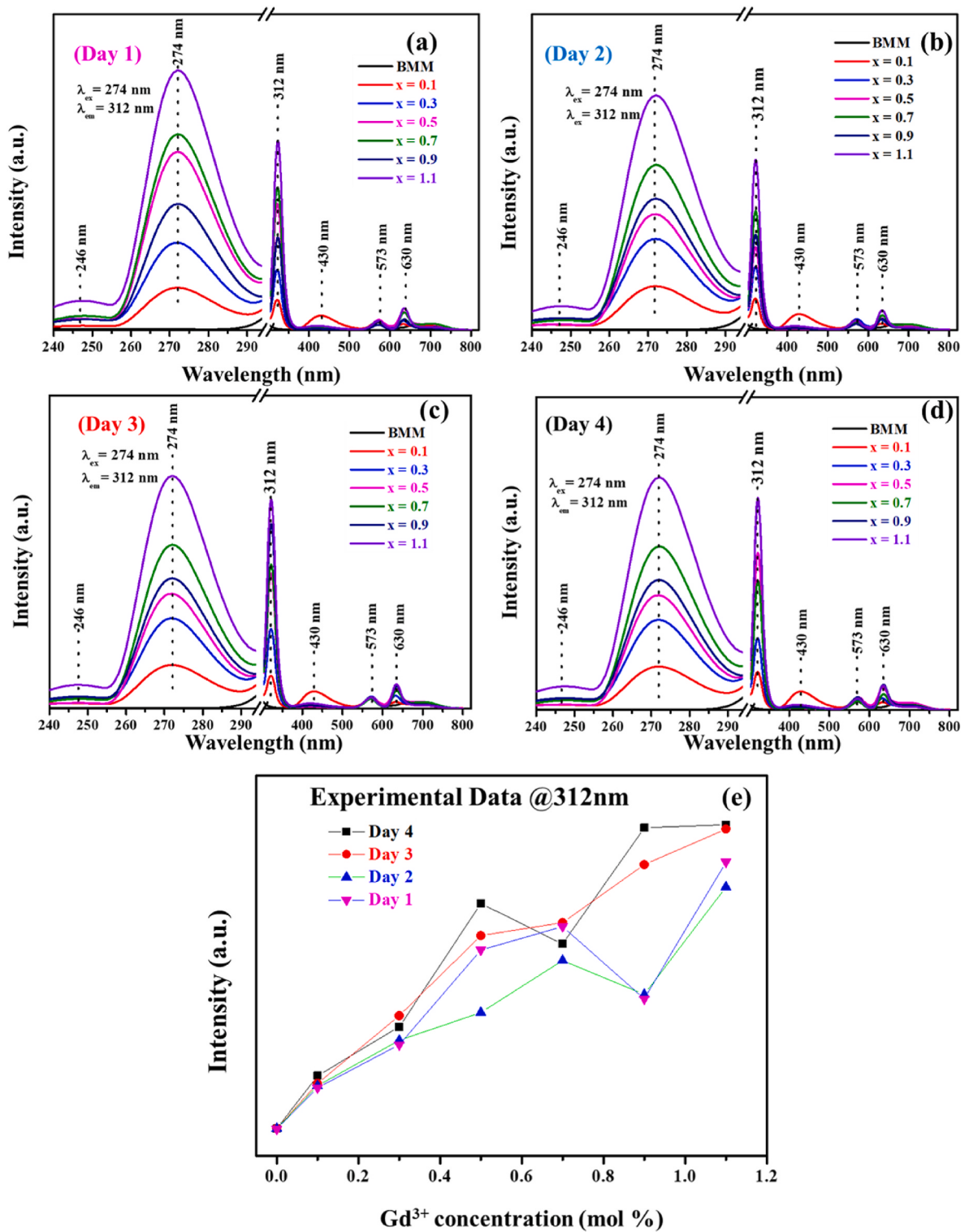
Fig. 9. The PL intensity of the BMM:x% Gd³⁺ (0 ≤ x ≤ 1.1) samples as a function of time over (a) 1 day, (b) 2, (c) 3, (d) 4 days, and emission intensity at 312 nm as a function of Gd³⁺ concentration for different days.
