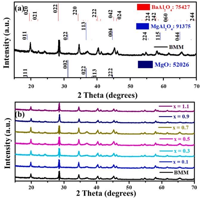
Fig. 2. The X-ray patterns of the (a) BMM and (b) BMM:x% \text{Gd}^{3+} ( 0 \leq x \leq 1.1 ) series.
