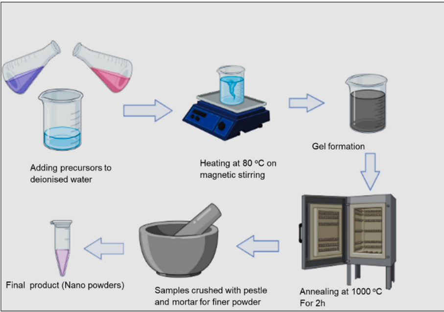
Fig. 1. Schematic diagram of the synthesis of BMM:x% \text{Gd}^{3+} ( 0 \leq x \leq 1.1 ) via sol-gel method.
