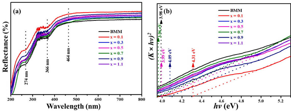
Fig. 7. (a) The diffuse reflectance spectra of BMM:x% Gd^{3+} ( 0 \leq x \leq 1.1 ) (b) Tauc of BMM: x% Gd^{3+} ( 0 \leq x \leq 1.1 ).
