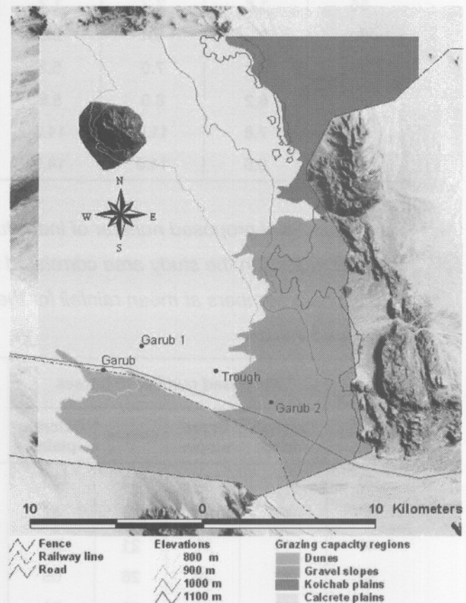
Fig. 3.10: Location and size of four regions used for determining animal numbers in study area.
