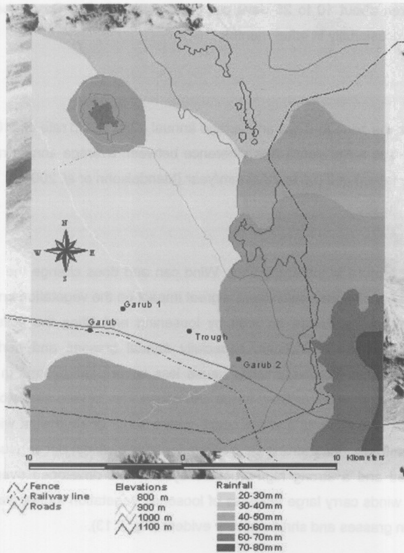
Fig. 2.12: Mean annual rainfall across the study area measured 2003 to 2005.
