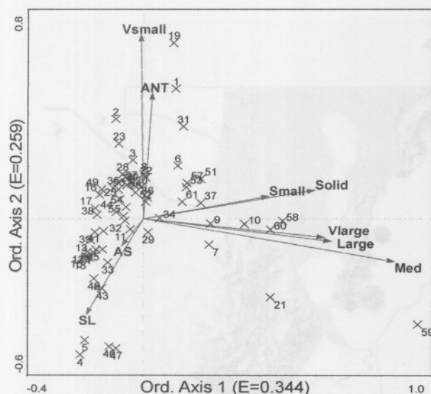
Fig. 3.3: CCA ordinations of relevés correlated to environmental variables (ANT-ant nests, AS-aspect, SL-slope, Rockiness: Vsmall-1 to 10mm; Small-11 to 30mm; Med-31 to 70mm; Large-71 to 150mm; Vlarge->150mm stones; Solid – solid rock).
