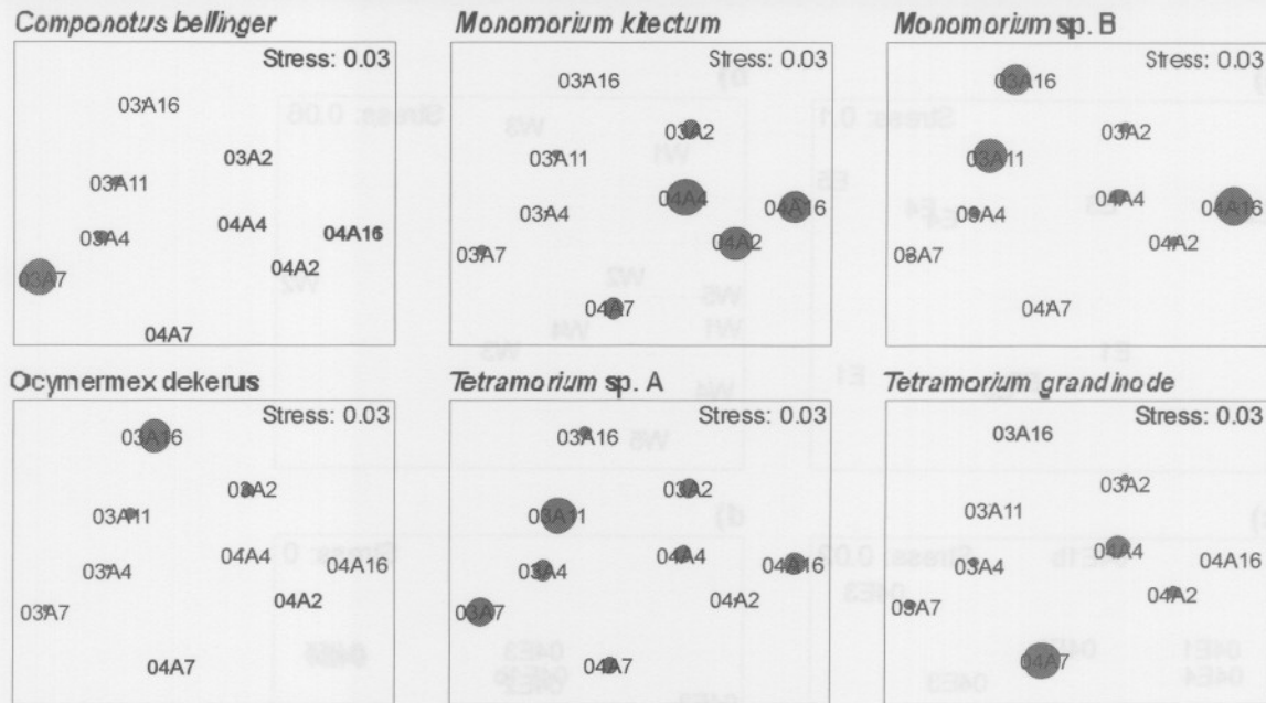
Fig. 6.8: Multidimensional scaling ordination of 2003 and 2004 East transects (presence/absence) with the abundances of some ant species indicated on each plot (the first two numbers indicate the year and the last number the distance from the trough, e.g. 03A2 = 2003 at 2 km, 04A2 = 2004 at 2 km).
