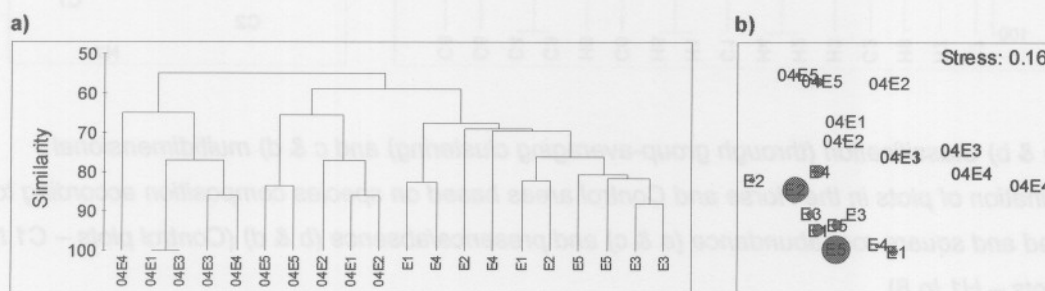
Fig. 6.18: a) Classification of plots with group-averaging clustering and b) multidimensional scaling ordination (presence/absence) of 2003 and 2004 East transect plots. The abundance of Rhammatodes sp. A is indicated as bubble values on each plot in the ordination (2003 plots – E1 to 5; 2004 plots – 04E1 to 5).
