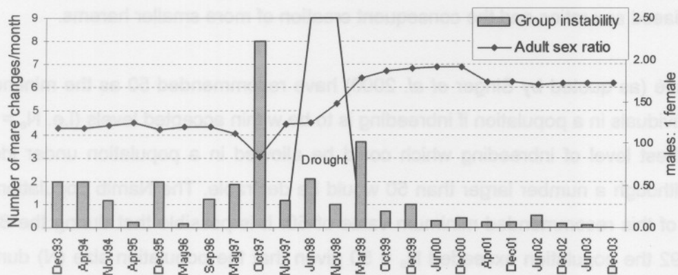
Fig. 5.18: Group instability plotted with adult sex ratio (males :1 female).
