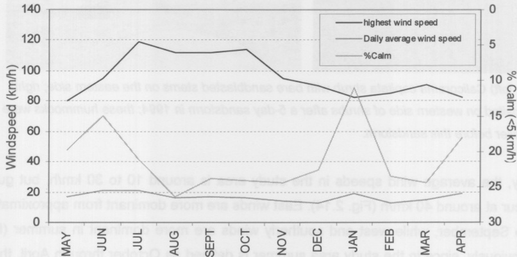
Fig. 2.15: The % calm and maximum wind speeds for each month recorded at Garub during 2003 to 2005.
