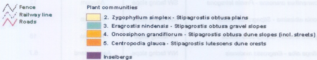
Fig 3.4: Plant communities of the Garub area. Note that the dune streets and dune slopes are not separated on the map.
