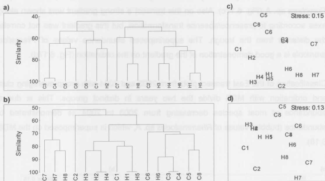
Fig. 6.19: a & b) Classification (through group-averaging clustering) and c & d) multidimensional scaling ordination of plots in the Horse and Control areas based on species composition according to standardized and square root abundance (a & c) and presence/absence (b & d) (Control plots – C1 to 8; Horse plots – H1 to 8).
