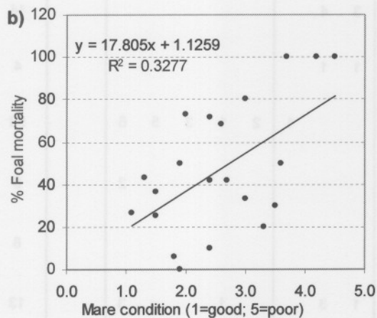
Fig. 5.9: a) Foal mortality (%) over time, b) the relationship between foal mortality (%) and the condition of mares (related to rainfall), and c) the relationship between foal mortality (%) and group instability (measured as the number of mare changes per month).
