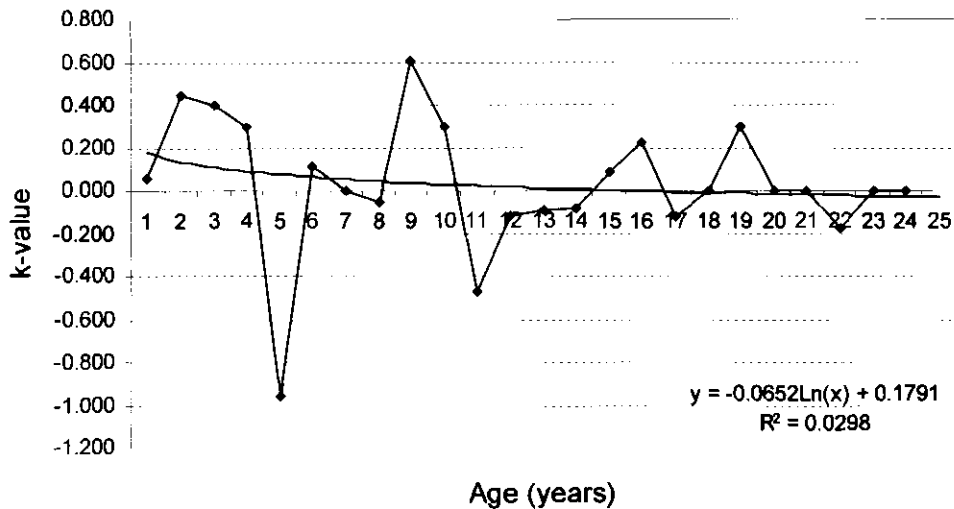
Fig. 5.4: k-values against age groups for the 2003 Namib horse population (Logarithmic trend line indicated).
