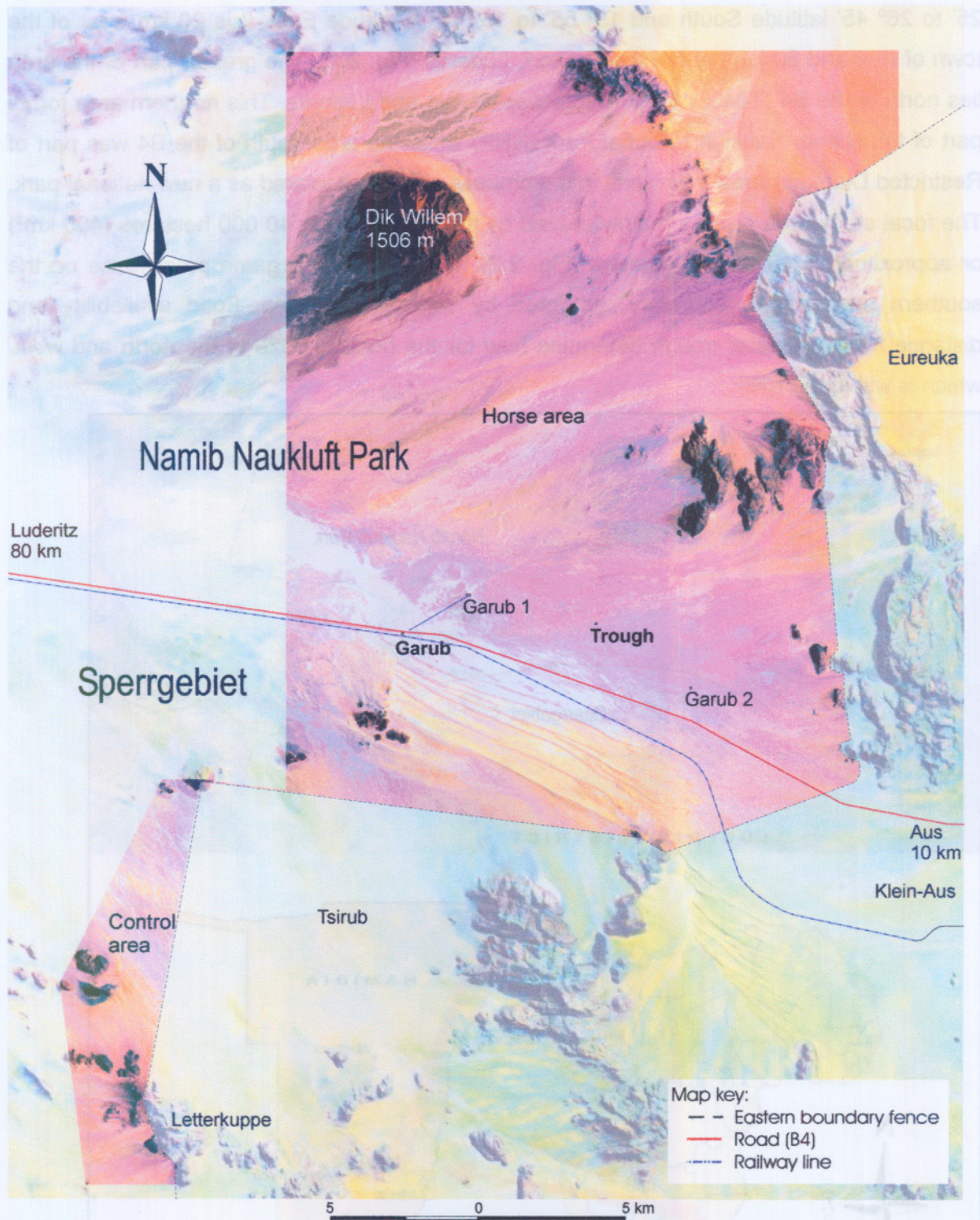
Fig. 2.2: Satellite image of study area (processing by Ingrid Stengel, Landsat5 Thematic Mapper Satellite Image: path/row 178/079, spectral bands RGB = 542)
