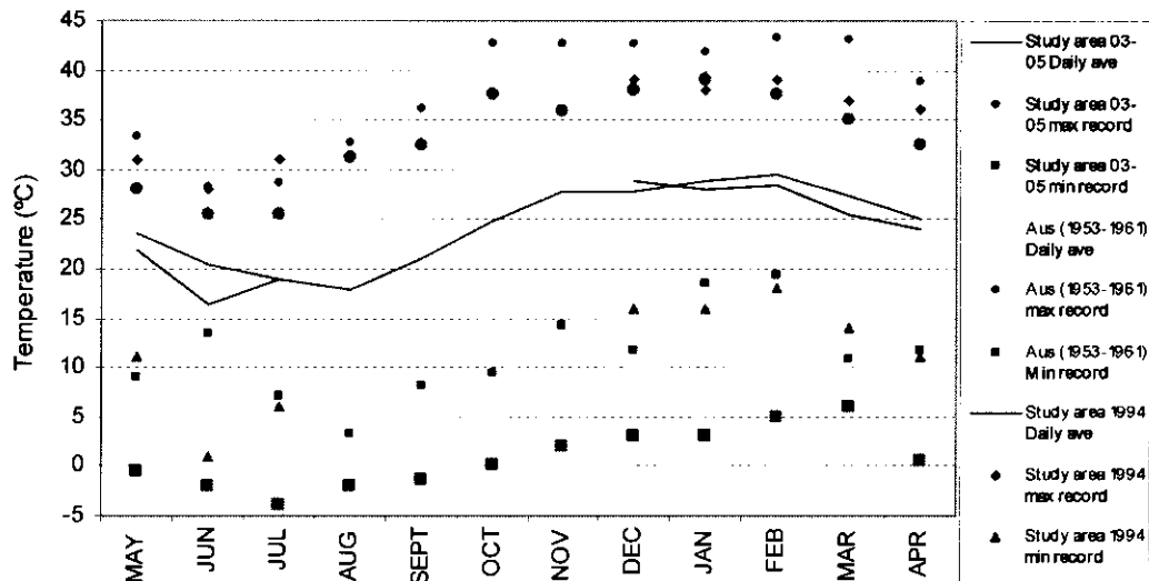
Fig. 2.7: Daily average, average maximum and minimum temperatures for each month as recorded at Garub during 1994 and 2003 to 2005 and at Aus during 1953 to 1961.
