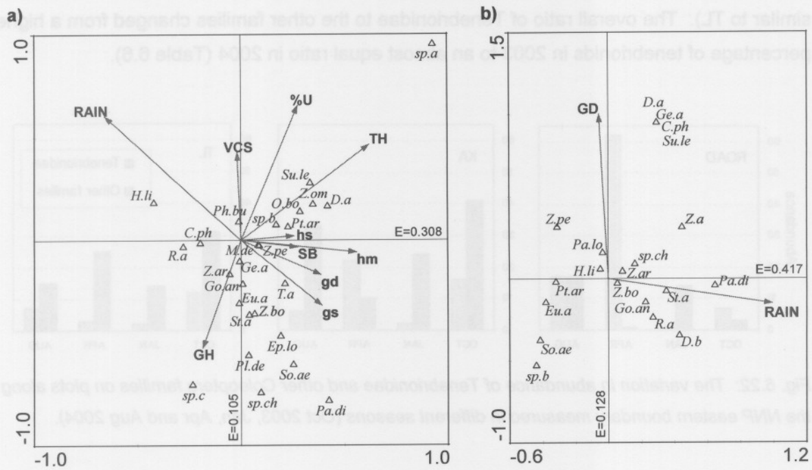
Fig. 6.21: CCA of Tenebrionidae species composition and environmental variables on a) the 2003 East and West transects and b) 2004 Horse and Control areas (GH – grass height, gs – gemsbok spoor, gd – gemsbok dung, hs – horse spoor, hm – horse manure, VCS – veld condition score, TH – termite soil heaps, %U - % utilized vegetation, RAIN – rainfall, SB – standing biomass and GD – grass density; C.ph - Cauricara phalangium , H.li - Histrionotus lightfooti , Pt.ar - Pterostichula cf. arenicola , Pa.lo - Pachynotelus longipilis , Eu.a - Eurychora sp. A , So.ae - Somaticus aeneus , St.a - Stipsostoma sp. A , R.a - Rhammatodes sp. A , Pa.di - Pachynotelus dimorphus and Su.le - Sulcipectus levis ).
