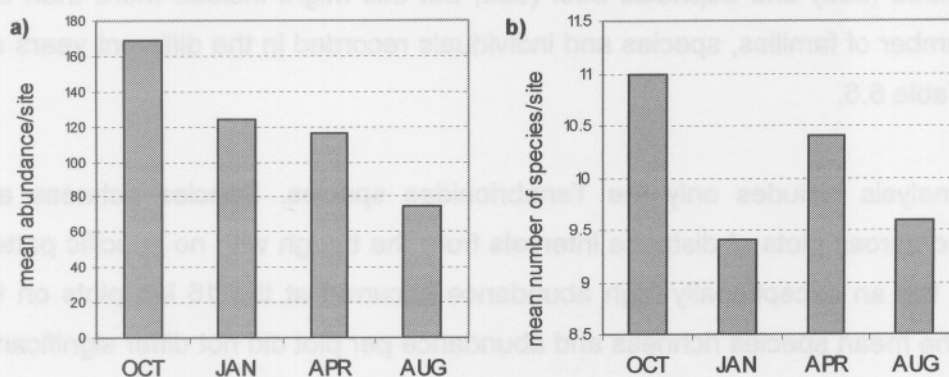
Fig. 6.15: a) The mean abundance and b) mean number of species per plot (5 plots) along the NNP eastern boundary measured on 4 occasions; Oct 2003, Jan 2004, Apr 2004 and Aug 2004.
