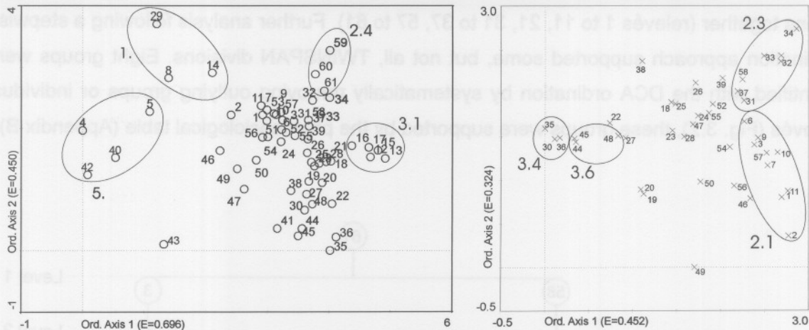
Fig. 3.2: DCA ordination of relevés; left) all relevés and right) 19 relevés removed. Groups representing communities and sub communities are encircled (community numbers in bold).
