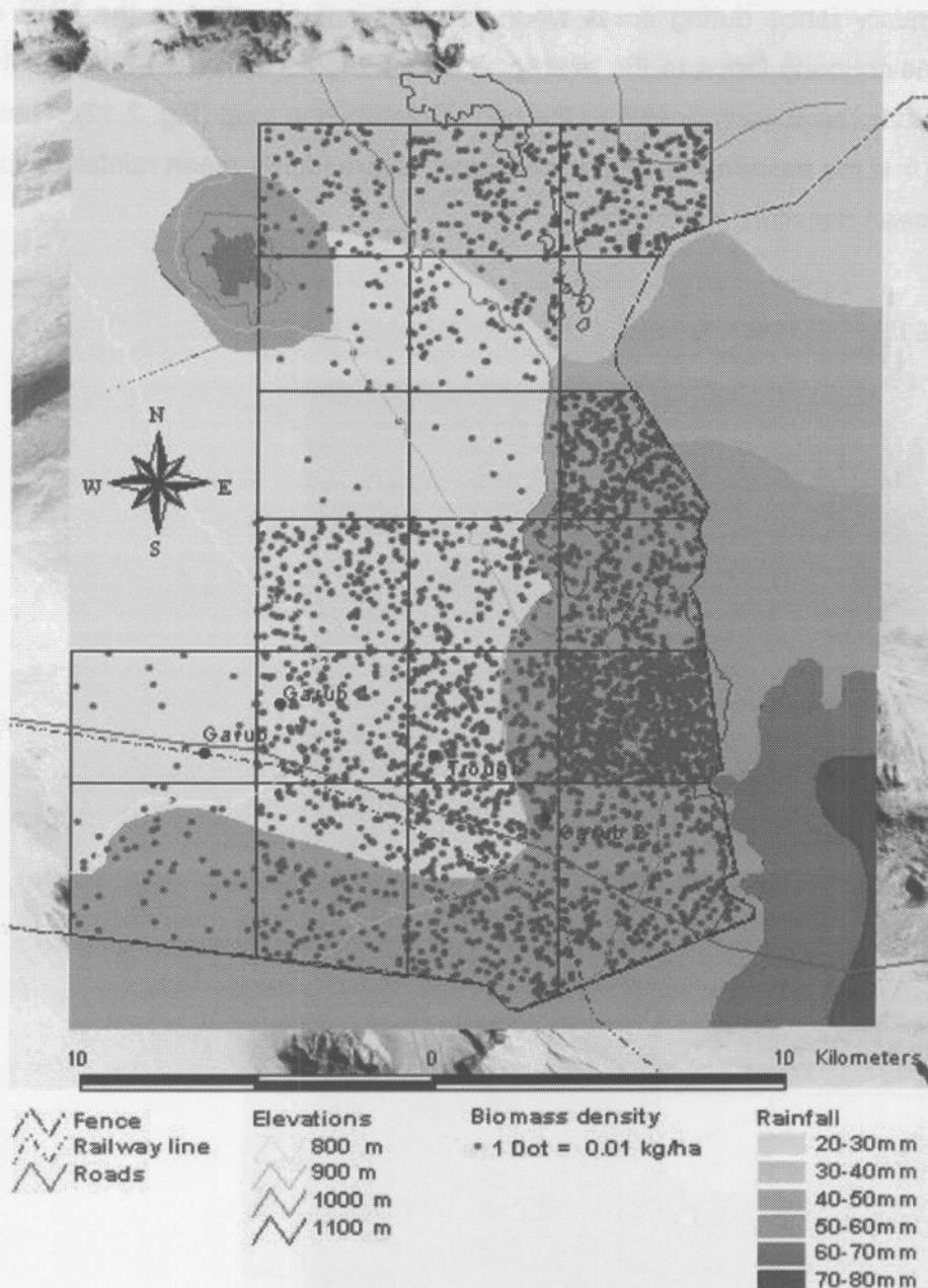
Fig. 4.3: The mean density (kg/ha) of all large herbivores in different zones of the study area (June 2003 to December 2004 ground surveys) superimposed on the rainfall distribution map to give an indication of how rainfall influence herbivore distributions.
