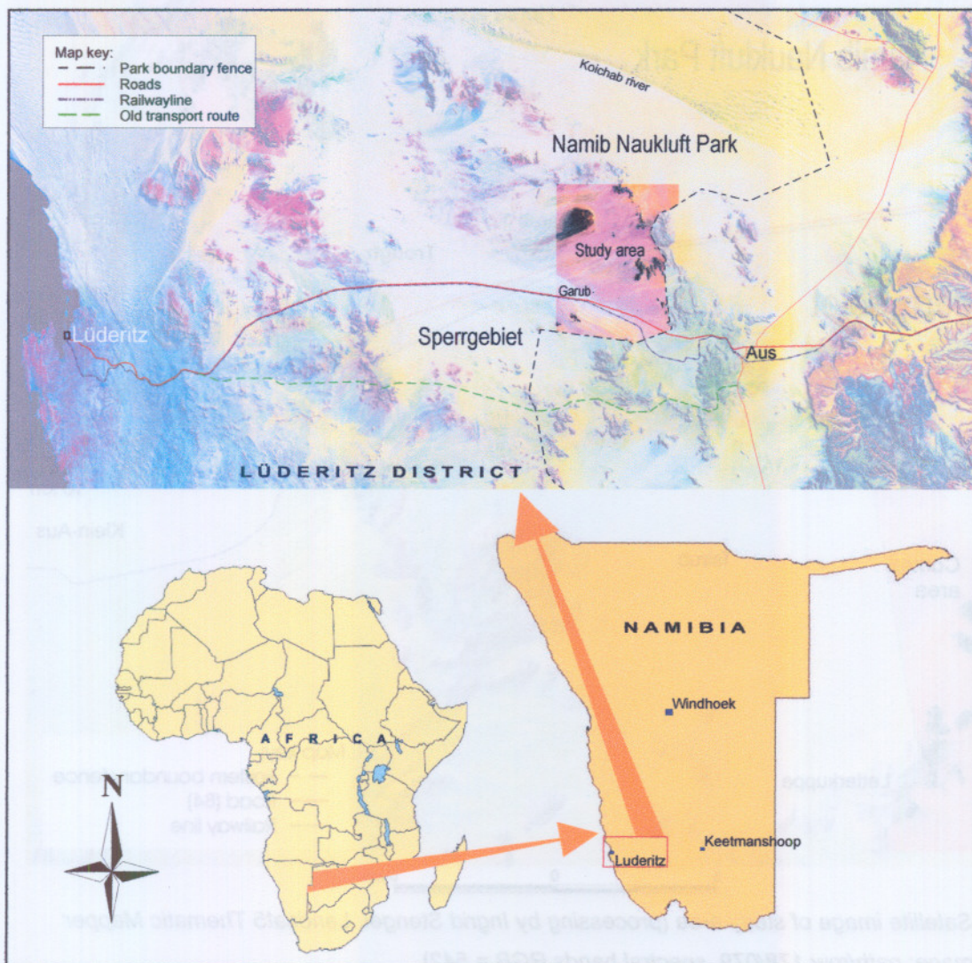
Fig. 2.1: Location of the study area.
