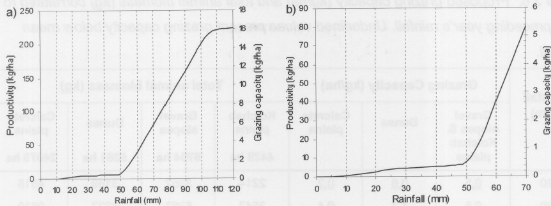
Fig 3.9: Final production curve correlating standing biomass, rainfall and grazing capacity for the Zygophyllum simplex - Stipagrostis obtusa plains community (calcrete plains). a) 0 to 120 mm rainfall range; b) enlarged 0 to 70 mm rainfall range.
