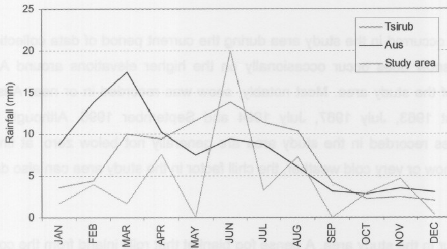
Fig. 2.11: The monthly average rainfall on the farm Tsirub (south of study area), Aus (east of the study area) and in the study area.
