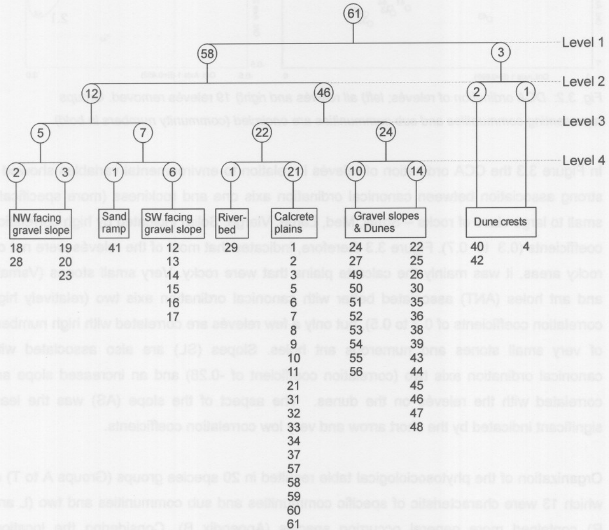
Fig. 3.1: Dendrogram showing relevé divisions according to TWINSpan; encircled values represent the number of relevés in groups.
