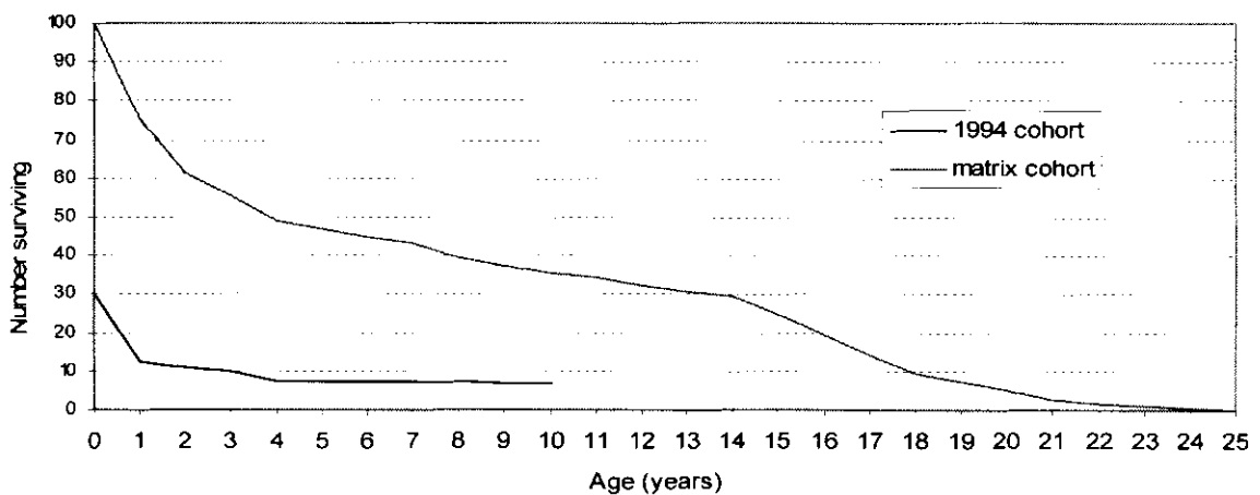
Fig. 5.5: Two survivorship curves, one for the 1994 cohort of Namib foals and the other an imaginary cohort (matrix cohort) of 100 foals surviving according to the mean survival rates determined in Table 5.5 & 5.6.
