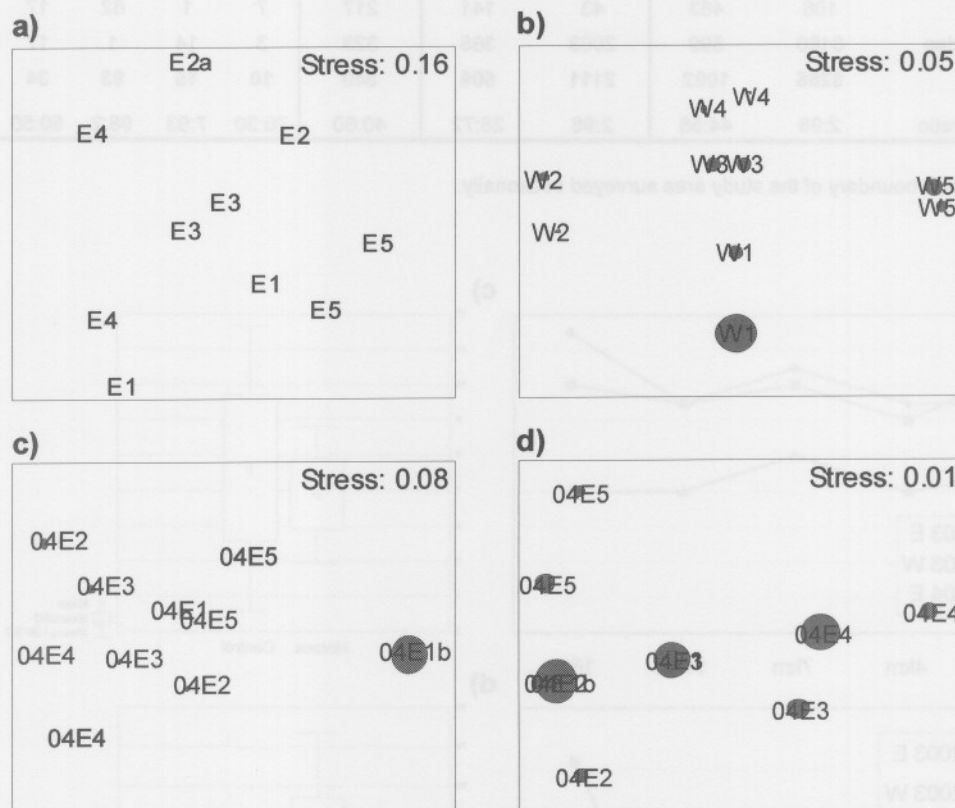
Fig. 6.17: Multidimensional scaling ordination: a) East 2003 transect, standardized and square root transformed; b) West 2003 transect, square root transformed with Pterosticula cf. arenicola abundance bubble values; c) East 2004 transect, no transformation with Stipsosoma sp. A. abundance bubble values; and d) East 2004 transect, presence/absence with Pterosticula cf. arenicola abundance bubble values. The distance intervals are 1=2 km, 2=4 km, 3=7 km, 4=11 km and 5=16 km.
