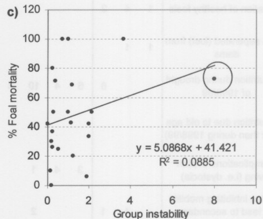
Fig. 5.9: a) Foal mortality (%) over time, b) the relationship between foal mortality (%) and the condition of mares (related to rainfall), and c) the relationship between foal mortality (%) and group instability (measured as the number of mare changes per month).
