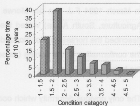
Fig. 5.19: The percentage time (over 120 months from Jan 1993 – Dec 2003) that the Namib horses were recorded in different condition categories (each month was placed in a category according to the mean condition of horses during that month).
