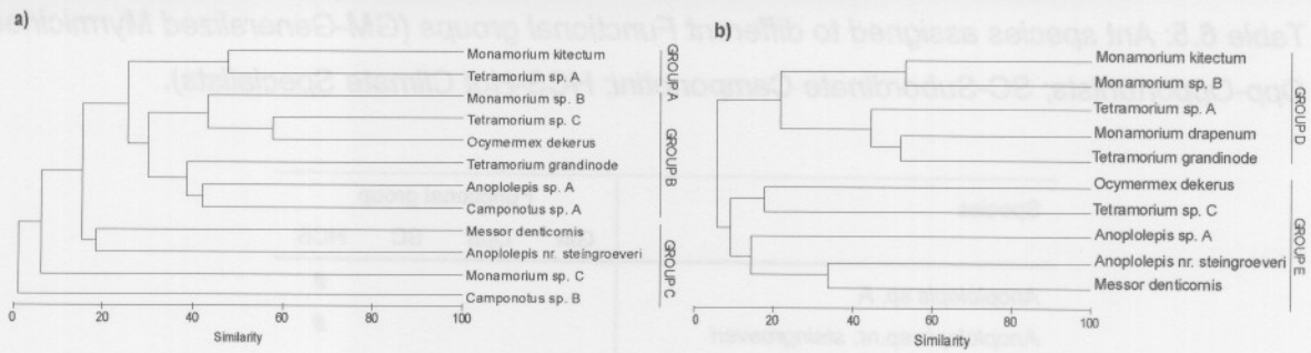
Fig. 6.12: Classification (through group averaging clustering) of ant species on a) 2003 East and West transects and b) the Horse and Control area.
