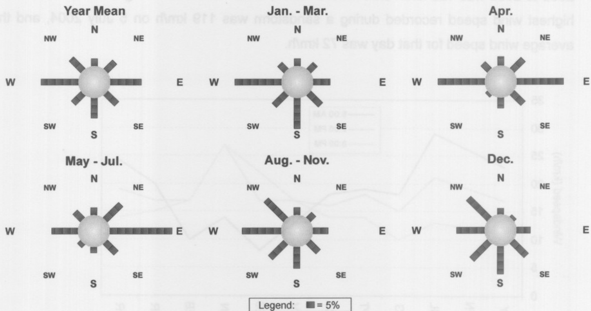
Fig. 2.16: Wind direction recorded at Garub during 2003 to 2005.
