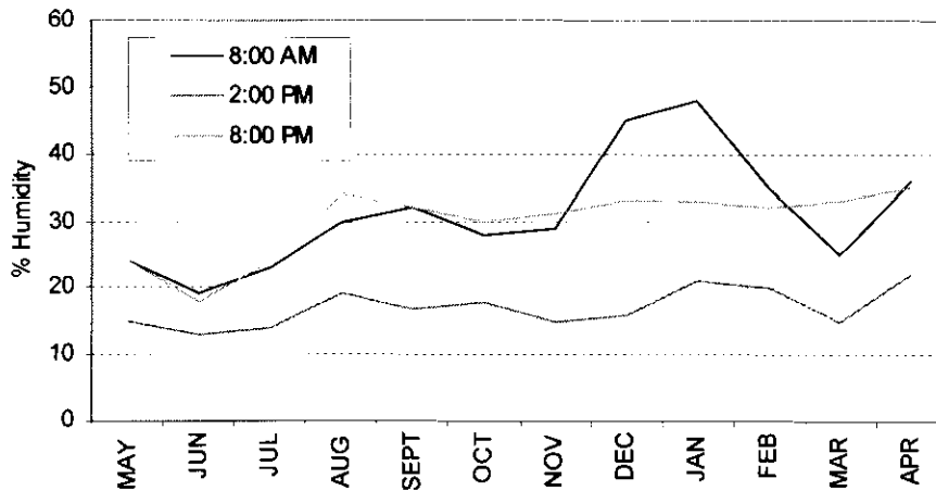
Fig. 2.8: The daily average humidity for each month at 8:00 a.m., 2:00 p.m. and 8:00 p.m.
