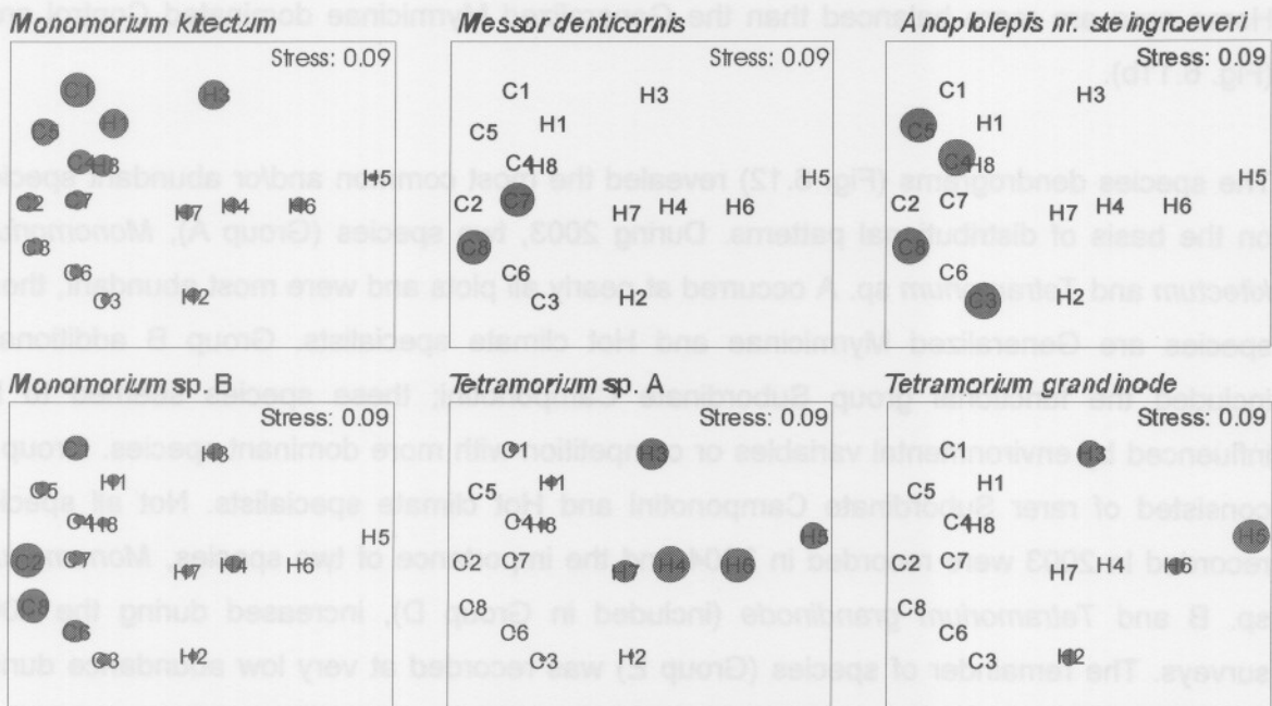
Fig. 6.10: Ant species presence and abundance between horse (H) and control (C) plots as superimposed on a MDS ordination according to species composition (no transformation).
