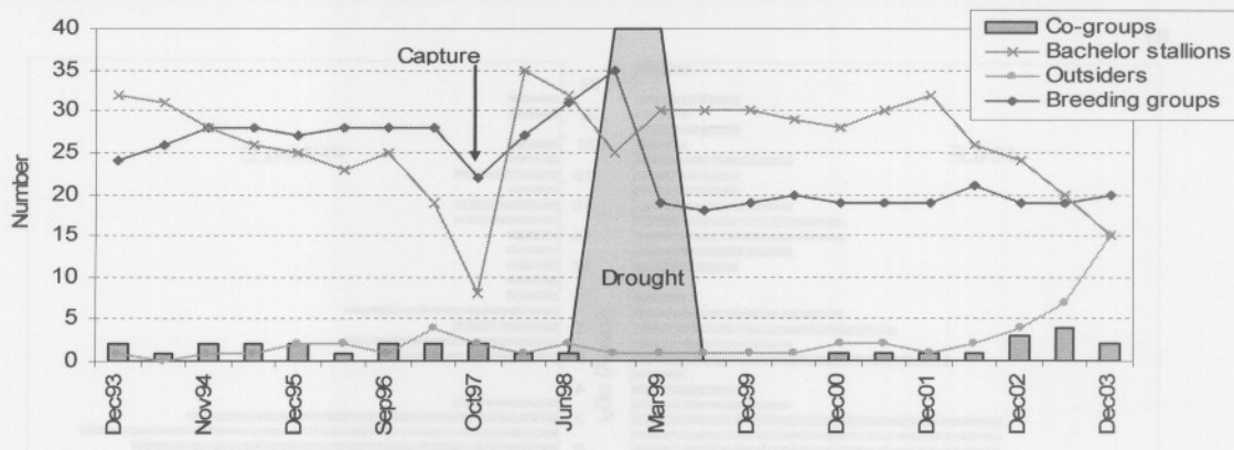
Fig. 5.16: The number of breeding groups, bachelor stallions, co-operating stallion groups (co-groups) and outsiders during 1993 to 2003 in the Namib feral horse population.
