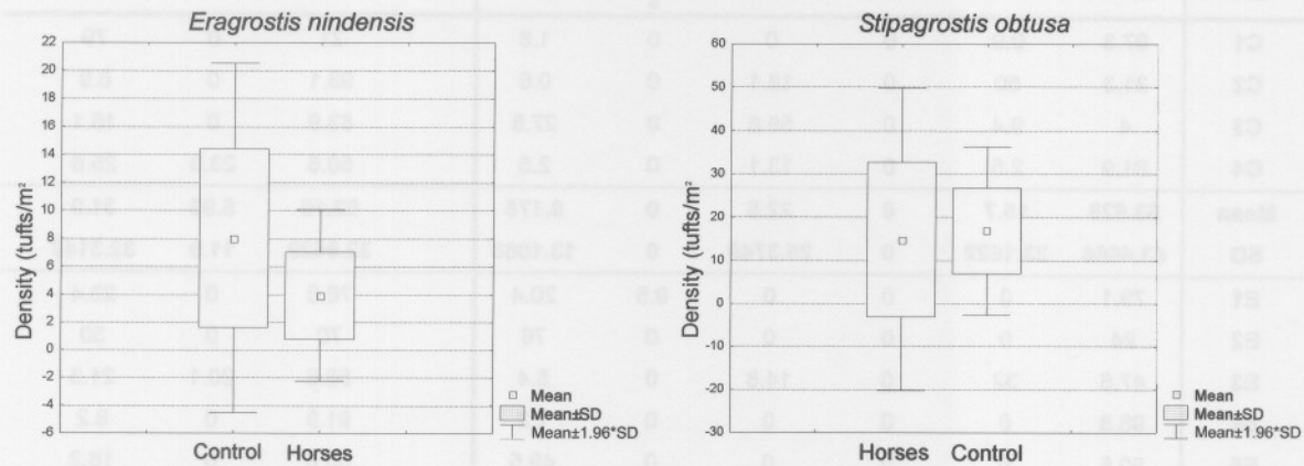
Fig. 6.5: Variation in density (tufts/m 2 ) of Stipagrostis obtusa and Eragrostis nindensis in the Horse and Control areas.
