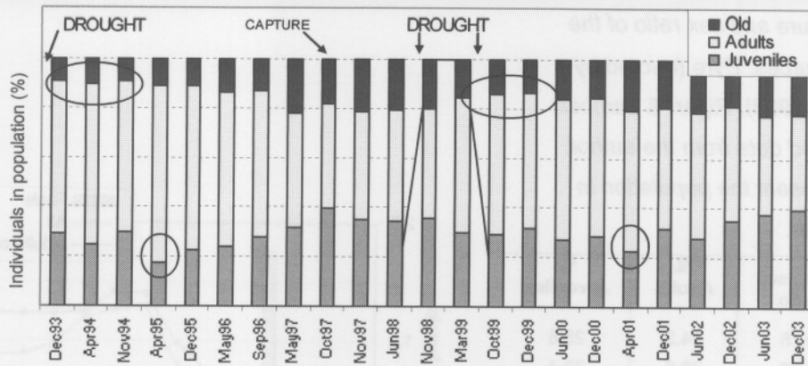
Fig. 5.14: The % juveniles (0 to 4 years), adults (5 to 15 years) and old horses (>15 years) during 1993 to 2003 (the Oct97 "capture" ratio excludes 35 horses temporarily removed; these horses are included again in Nov97).
