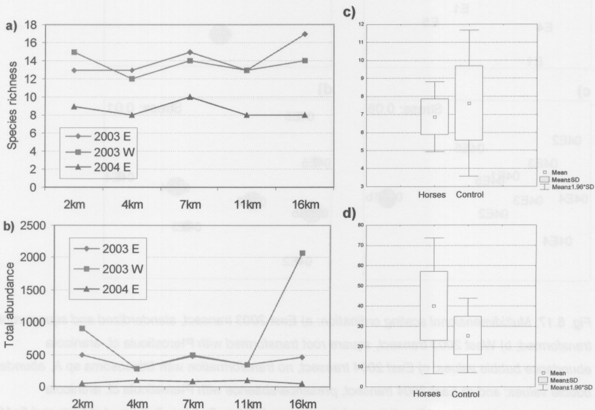
Fig. 6.16: a) Tenebrionidae species richness and b) abundance at increasing distances from the trough on three transects; and c) the mean species richness and d) abundance per plot compared between the Horse and Control areas.
