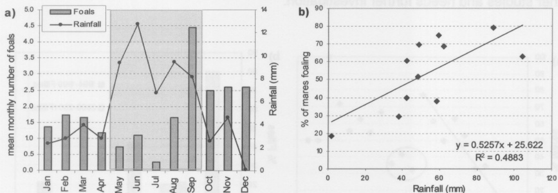
Fig. 5.10: a) The mean monthly number of foals born (1993 to 2004) with the mean rainfall (mm) over the same period (the shaded area indicates winter months), and b) the correlation between annual foaling rate (measured as the percentage of breeding mares that foaled) and the rainfall of the preceding year.
