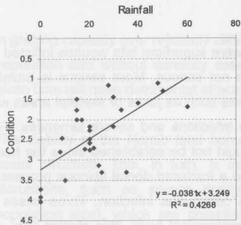
Fig. 5.20: The relationship between rainfall and condition of horses.
