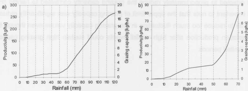
Fig 3.8: Final production curve correlating standing biomass, rainfall and grazing capacity for the Oncosiphon grandiflorum - Stipagrostis obtusa dune slopes community. a) 0 to 120 mm rainfall range; b) enlarged 0 to 70 mm rainfall range.
