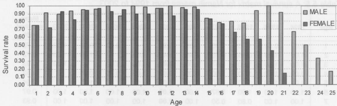
Fig. 5.6: The mean annual age specific survival rates for male and female horses from 1993 to 2003 as per survival matrix values.
