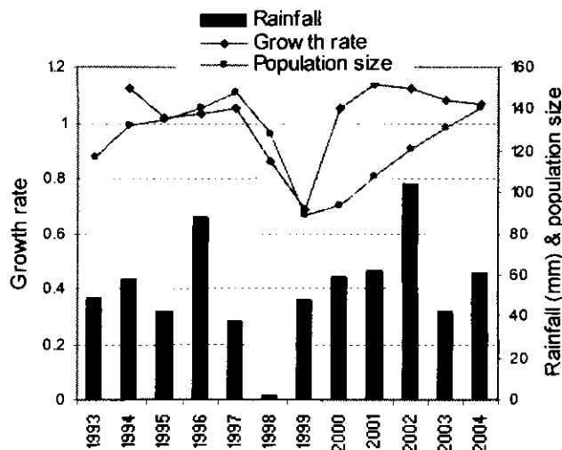
Fig. 5.3: Population size and growth rate of horses compared to rainfall during 1993 to 2004.
