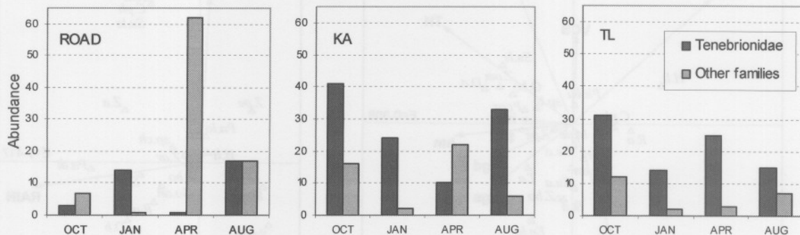
Fig. 6.22: The variation in abundance of Tenebrionidae and other Coleoptera families on plots along the NNP eastern boundary measured in different seasons (Oct 2003, Jan, Apr and Aug 2004).
