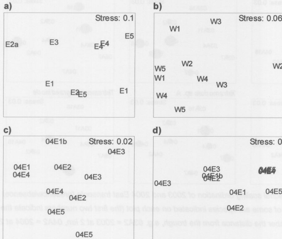
Fig. 6.7: Multidimensional scaling ordination: a) East 2003 transect (presence/absence); b) West 2003 transect (presence/absence); c) East 2004 transect (standardized abundance); and d) East 2004 transect (presence/absence). The distance intervals are 1=2 km, 2=4 km, 3=7 km, 4=11 km and 5=16 km.
