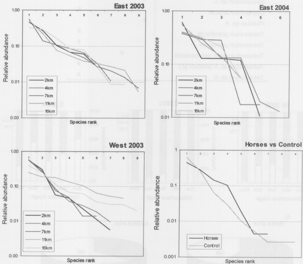
Fig. 6.13: Rank-abundance plots for ant species at distance intervals from the trough on three transects (total ant abundance in two plots at each distance interval) and the Horse vs. Control area (mean ant abundance/plot).
