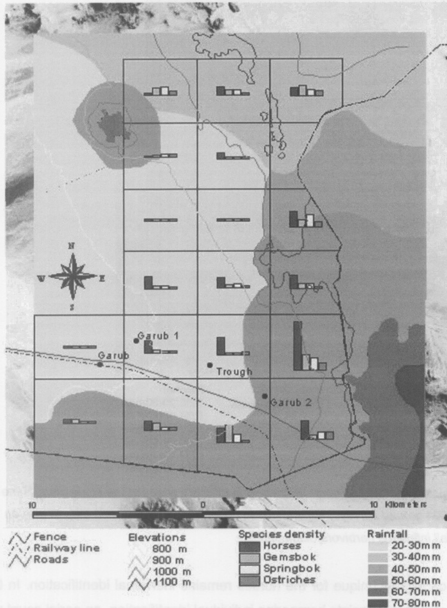
Fig. 4.2: The mean densities (individuals/km 2 ) of large herbivore species in different zones of the study area (June 2003 to December 2004 ground surveys) superimposed on the rainfall distribution map to give an indication of how rainfall influence herbivore distributions.
