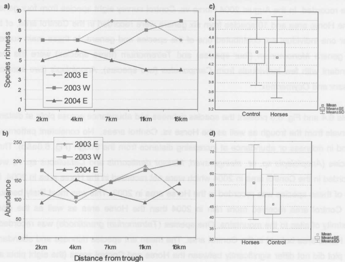
Fig. 6.6: a) The total ant species richness and b) abundance at increasing distance from the trough; and c) the mean species richness and d) mean abundance per plot compared between the Horse and Control areas.
