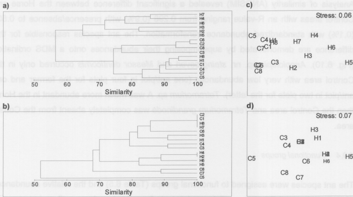
Fig. 6.9: a & b) Classification (through group-averaging clustering) and c & d) multidimensional scaling ordination of the Horse (H1 to H8) and Control (C1 to C8) areas based on species composition (standardized abundance (a & c) and presence/absence (b & d)).
