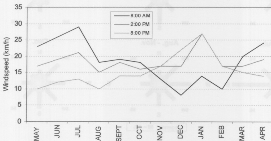
Fig. 2.14: The daily average wind speeds for each month at 8 am, 2 pm and 8 pm recorded at Garub during 2003 to 05.
