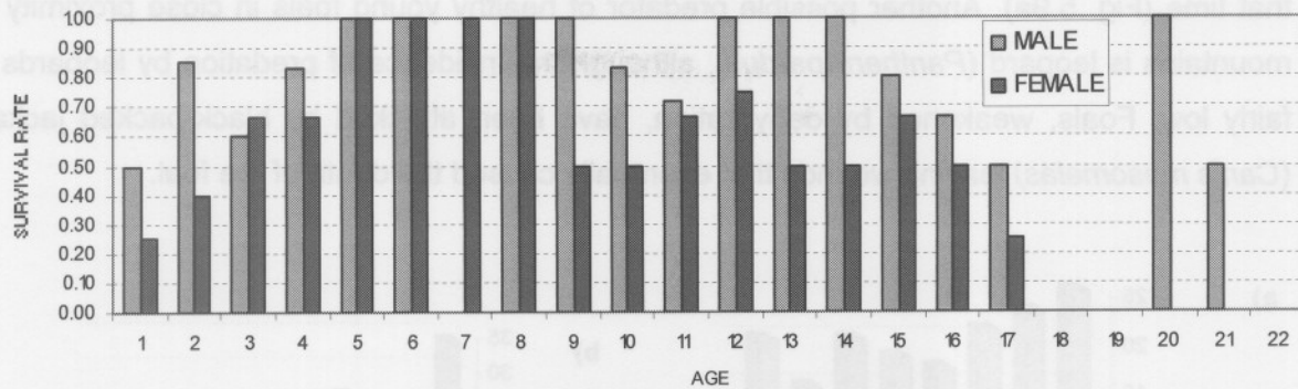
Fig. 5.7: The age specific survival rates for male and female horses during the 1998/99 drought.
