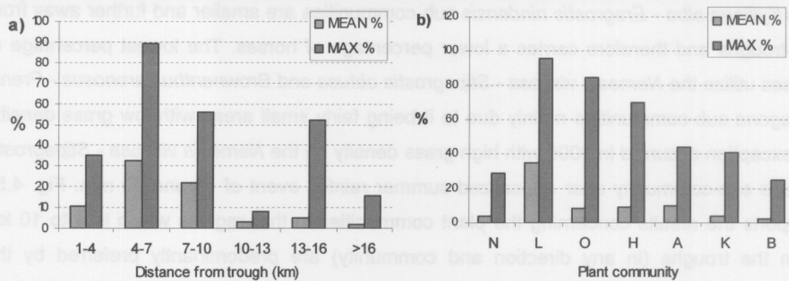
Fig. 4.5: The mean and maximum percentage of the horse population a) at different distance intervals from the trough and b) utilizing the different plant communities (June 2003 to December 2004 ground surveys), (N - Nemesia viscosa - Stipagrostis obtusa ; L - Leysera tenella - Stipagrostis obtusa ; O - Oncosiphon grandiflorum - Stipagrostis obtusa dune slopes ; H - Helichrysum herniarioides - Stipagrostis obtusa ; A - Avonia albissima - Stipagrostis obtusa ; K - Kyllinga alba - Eragrostis nindensis ; B - Brownanthus arenosus - Prenia tetragona ).
