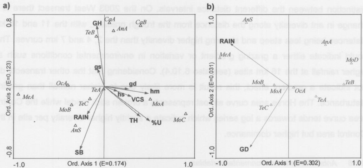
Fig. 6.14: Ordination with Canonical Correspondence Analyses (CCA) of ant species and environmental variables on a) 2003 East and West transects and b) 2004 Horse and Control areas.
