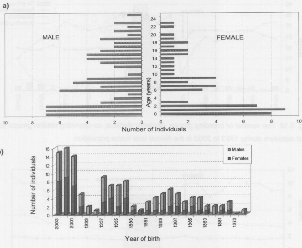
Fig. 5.15: Number of horses in each age class for the 2003 Namib population (ages observed for 0 to 12 years and estimated for horses older than 12 years), a) indicating age in years and b) indicating year of birth.
