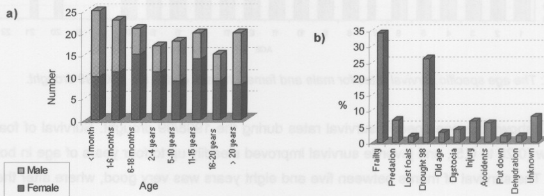
Fig. 5.8: a) Age and sex specific number of horses that died during Dec 1993 to Dec 2004, and b) the percentage of horses during this period that died due to various mortality factors.
