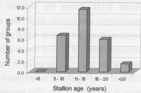
Fig. 5.12: The number of groups with stallions in different age classes.
