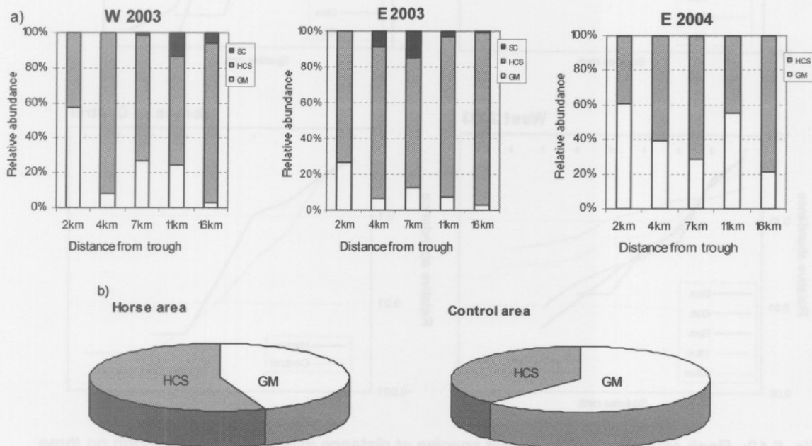
Fig. 6.11: Relative abundance of different ant Functional groups a) at various distances from the trough for the East and West transects as well as b) the Horse and Control area (GM-Generalized Myrmicinae; SC-Subordinate Camponotini; HCS- Hot Climate Specialists).
