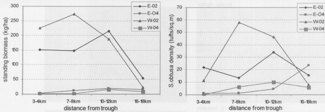
Fig. 6.4: a) The mean standing biomass of all grasses and b) density of Stipagrostis obtusa at various distances from the trough measured on the eastern slopes (E) and western plains (W) during September 2002 (E-02 and W-02) and September 2004 (E-04 and W-04).
