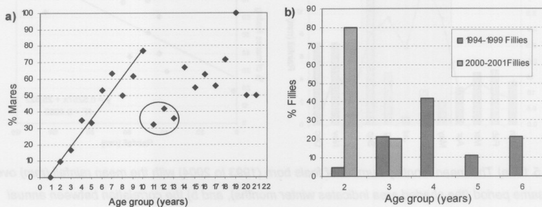
Fig. 5.11: a) The mean percentage of mares in each age group producing foals and b) the percentage of fillies in different age groups producing their first foals.
