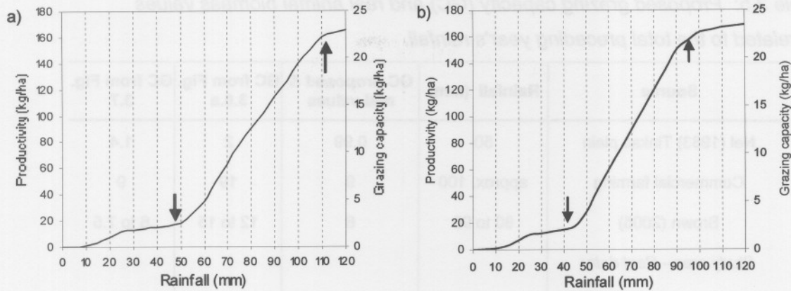
Fig 3.6: Production curves correlating standing biomass, rainfall and grazing capacity (from Table 3.3) of the Leysera tenella - Stipagrostis obtusa sub-community using a) total rainfall of the preceding year; and b) the preceding 2 years running mean rainfall.
