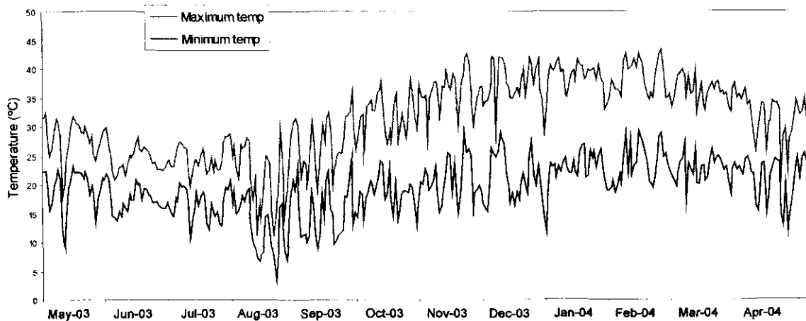
Fig. 2.5: The daily maximum and minimum temperatures from 1 May 2003 to 30 April 2004.
