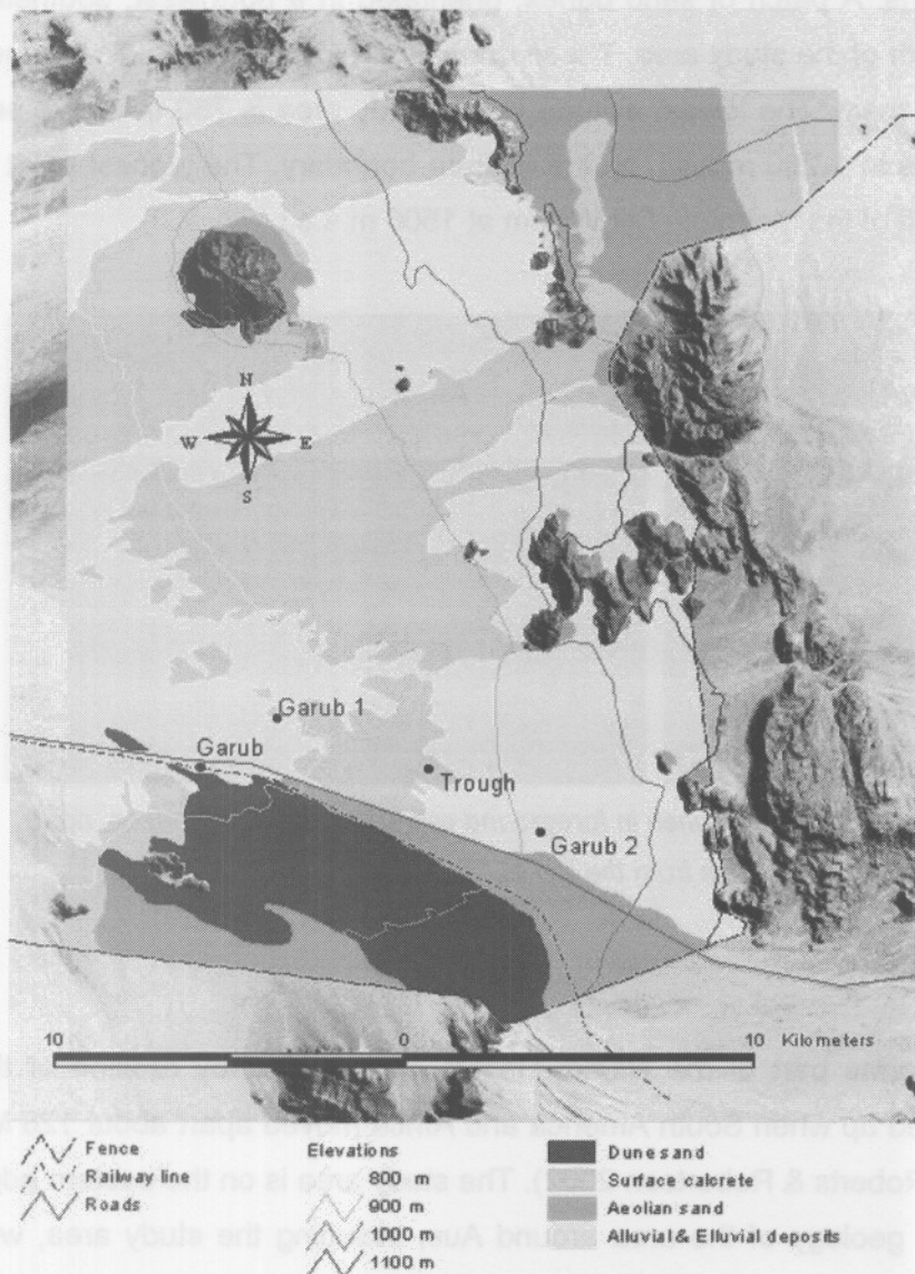
Fig. 2.4: Surface geology of the plains in the study area, adapted from the geological map by Jackson (1975). For detailed geology of the inselbergs and rock formations see Jackson (1975) and the Geological map of Namibia, sheet 2616 – Bethanien, 1999, Geological Survey of Namibia.
