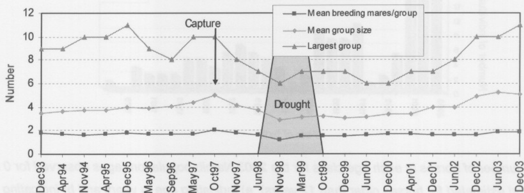
Fig. 5.17: The mean number of breeding mares per group, mean group size and number of horses in the largest group.
