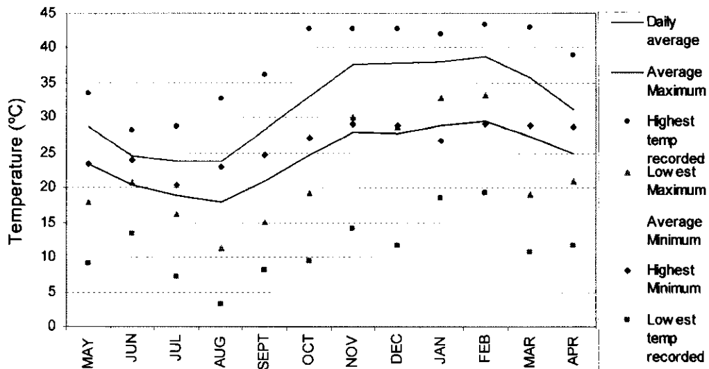
Fig. 2.6: Daily average, average maximum and average minimum temperatures with ranges for each month as recorded at Garub during 2003 to 2005.
