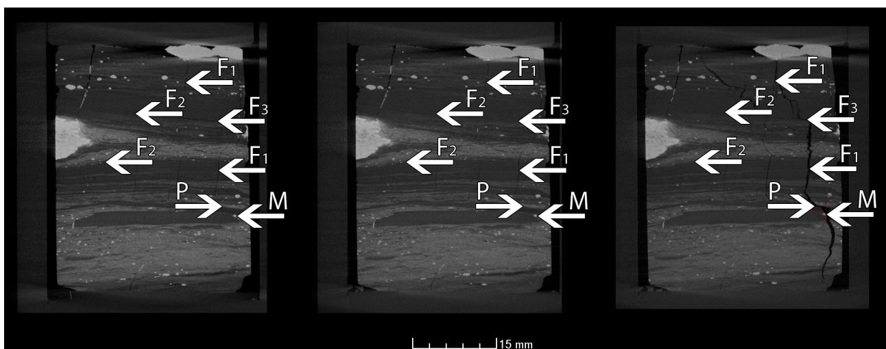
F indicates cleats or cracks that existed in the pre-loaded particles that enlarged during compression; M indicates mineral inclusions that may have had an influence on either crack initiation or crack propagation; P indicates either maceral-maceral boundaries or maceral-mineral boundaries that may have had an influence on crack initiation.
