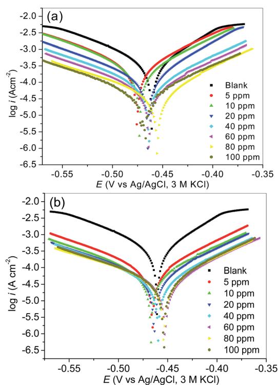
Fig. 2 Tafel plots for mild steel in 1 M HCl without and with various concentrations of (a) MS-2-PQPP, and (b) MS-2-PQPMS, as representative Tafel plots for the studied compounds.
