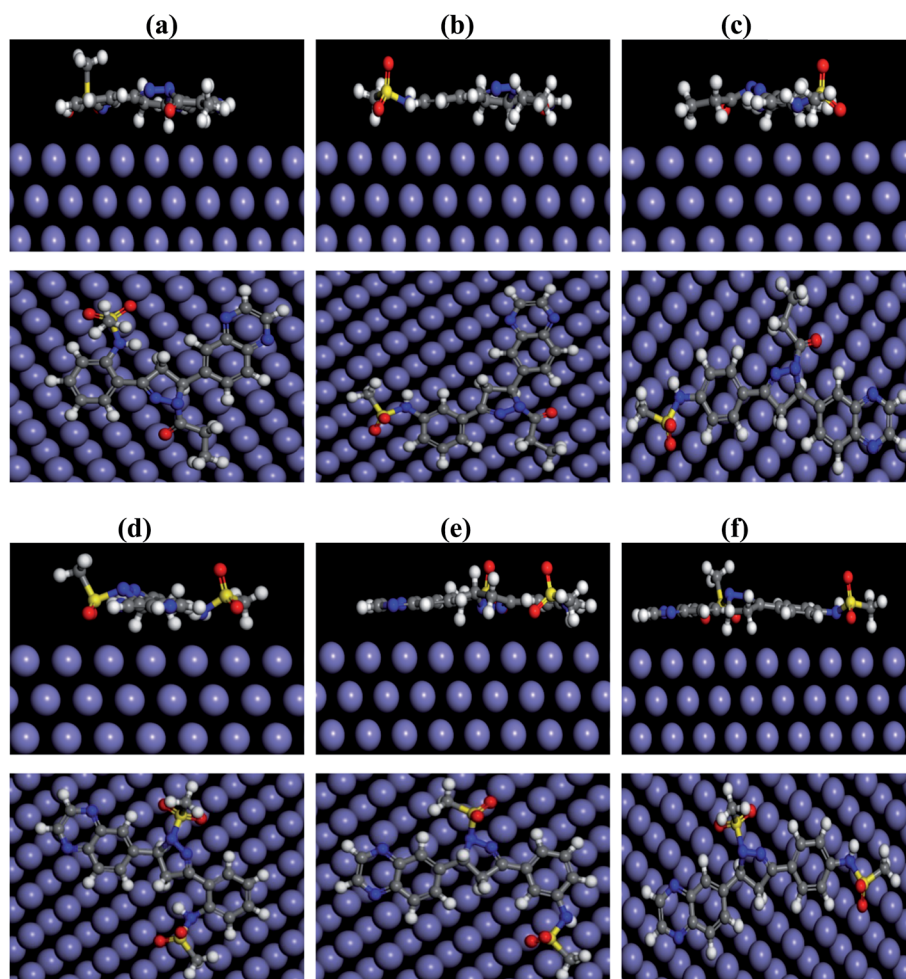
Fig. 11 Side (above) and top (below) views of the low adsorption energy configurations of (a) MS-2-PQPP, (b) MS-3-PQPP, (c) MS-4-PQPP, (d) MS-2-PQPMS, (e) MS-3-PQPMS and (f) MS-4-PQPMS interactions with Fe(110) using molecular dynamics simulations.
