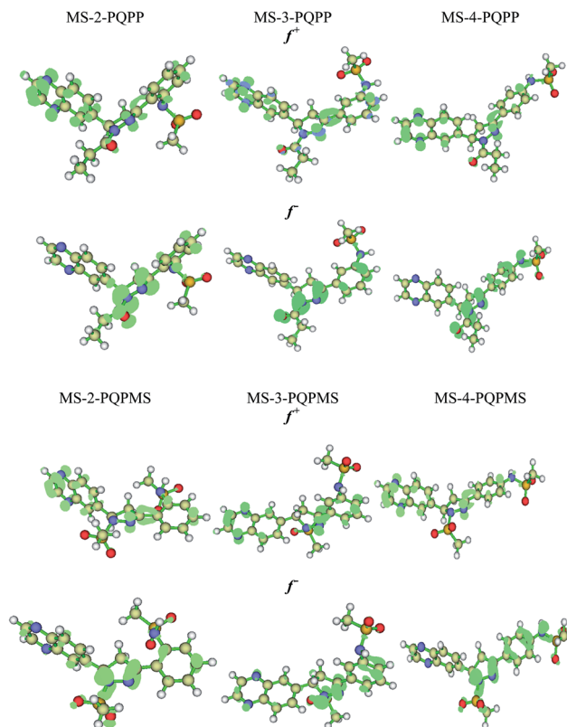
Fig. 9 Fukui functions for the inhibitor molecules (isosurface = 0.003).
