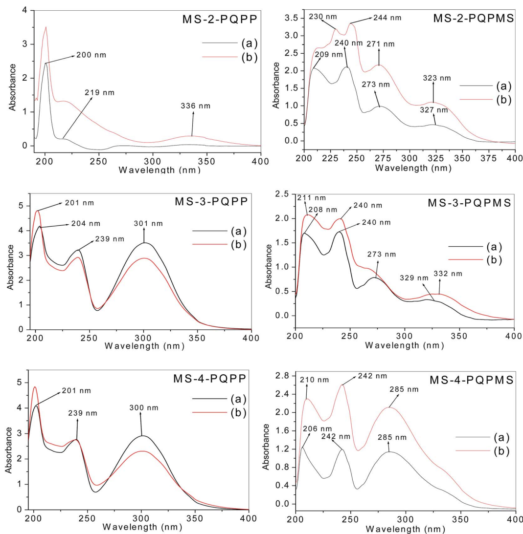
Fig. 5 UV-vis spectra of acidic solutions of studied inhibitors (a) before, and (b) after mild steel immersion.
