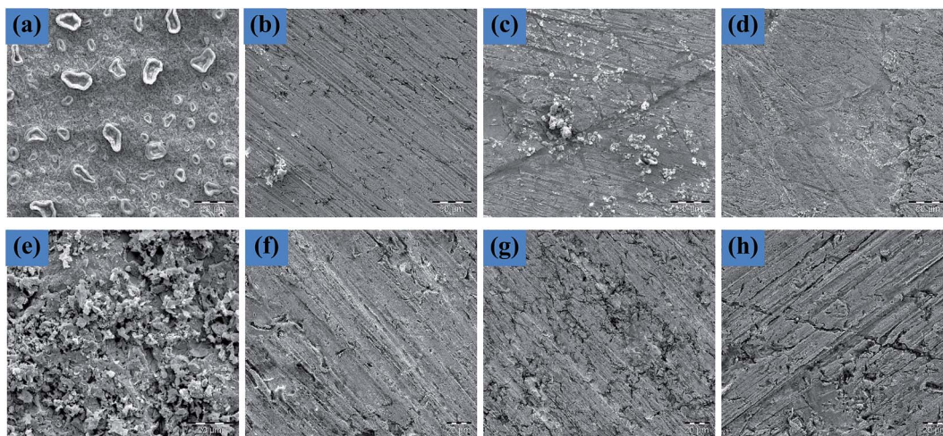
Fig. 6 SEM images of mild steel in 1 M HCl (a & e) without inhibitors, and with 100 ppm of (b) MS-2-PQPP, (c) MS-3-PQPP, (d) MS-4-PQPP, (f) MS-2-PQPMS, (g) MS-3-PQPMS and (h) MS-4-PQPMS (image size: 50 \mu\text{m} (a–d); 20 \mu\text{m} (e–h)).
