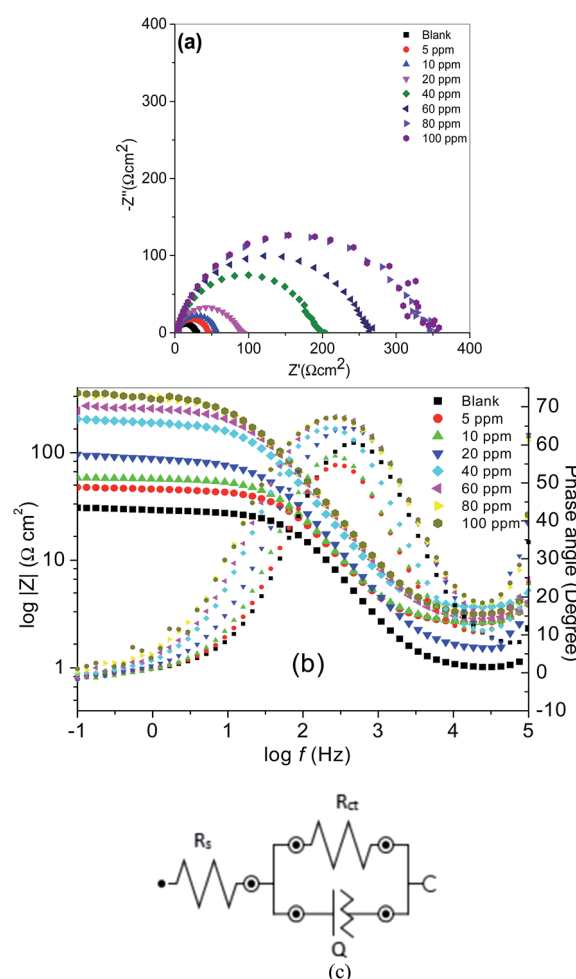
Fig. 3 Nyquist (a) and Bode (b) plots for mild steel in 1 M HCl without and with various concentrations of MS-2-PQPP as representative impedance spectra of the studied compounds; (c) equivalent circuit for the EIS spectra.
