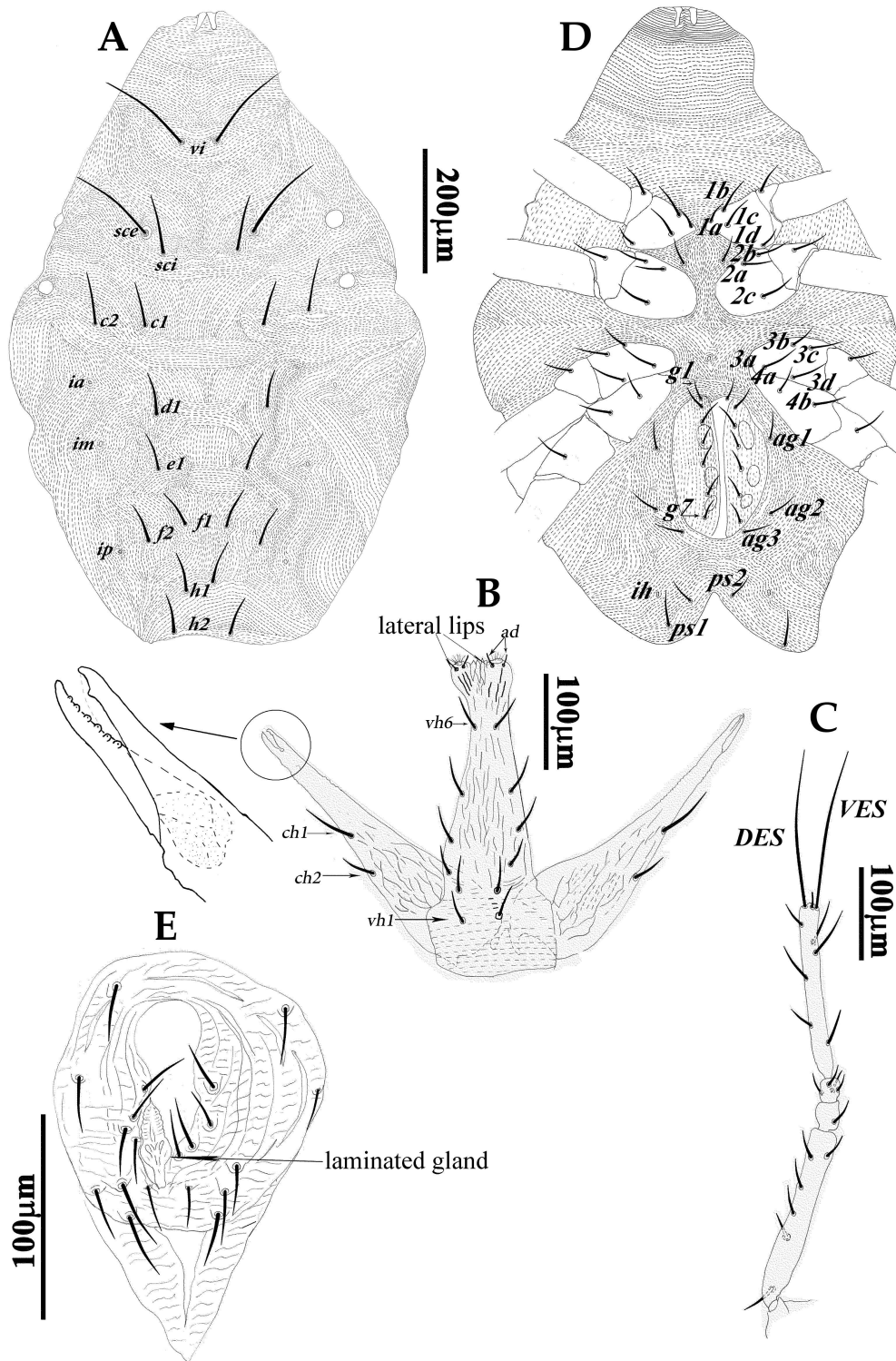
FIGURE 3: Odontoscirus denheyri Eghbalian, Khanjani & Ueckermann n. sp. (Female): A – Dorsum of idiosoma; B – Gnathosoma; C – Palp; D – Venter of idiosoma; E – Ovipositor.
