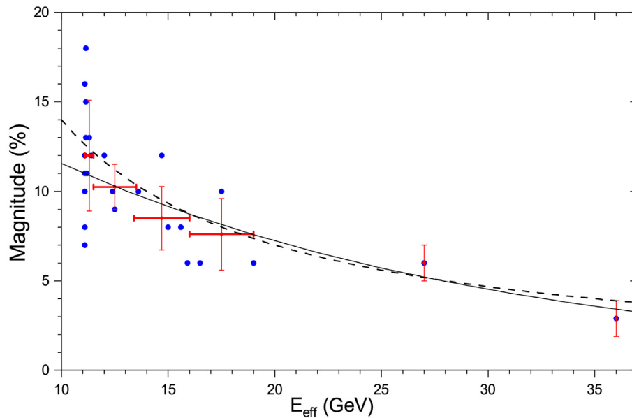
Fig. 9. Maximum magnitude (in %) of the Forbush decrease as a function of the effective energy E_{\text{eff}} (as defined in Asvestari et al., 2017) of the NMs studied here. Blue dots depict values for individual NMs, and red crosses show averaged values over 2-GV bins. The solid and dashed lines depict the best-fit exponential ( M = (18.5 \pm 3.5) \cdot \exp((-0.047 \pm 0.010) \cdot E_{\text{eff}}) ) and power-law ( M = (140 \pm 60) \cdot E_{\text{eff}}^{-1.0 \pm 0.1} ) functions, respectively.
