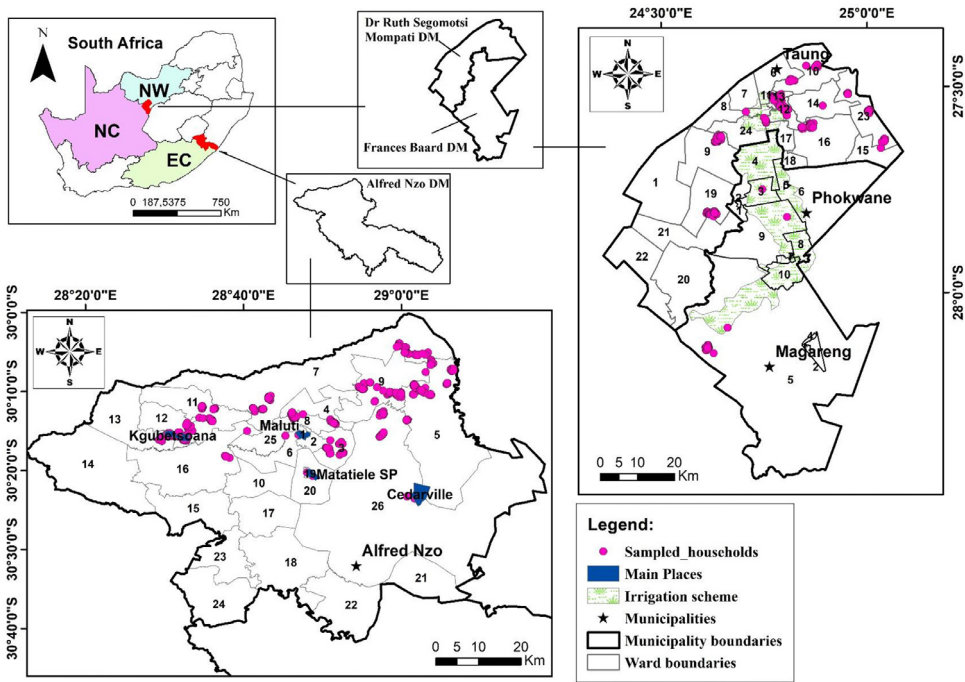
Fig. 23. Study area.
