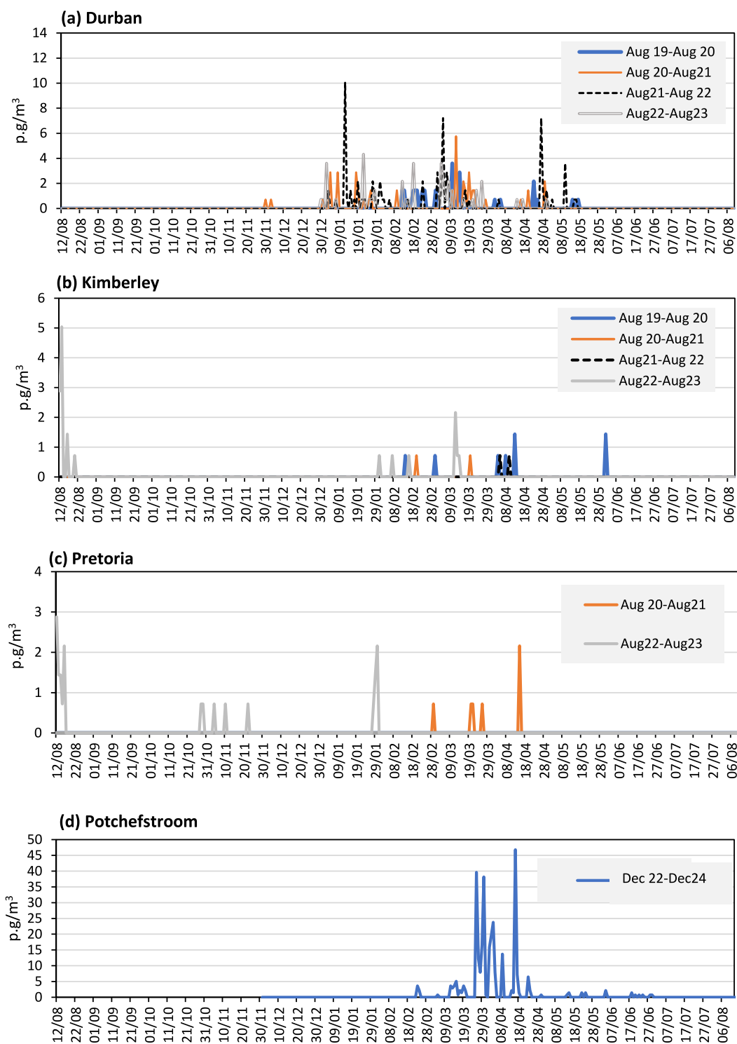
Fig. 3 Fluctuations of Ambrosia pollen in the aerobiological sampling stations during the studied period. a. Durban, b. Kimberley, c. Pretoria, d. Potchefstroom
