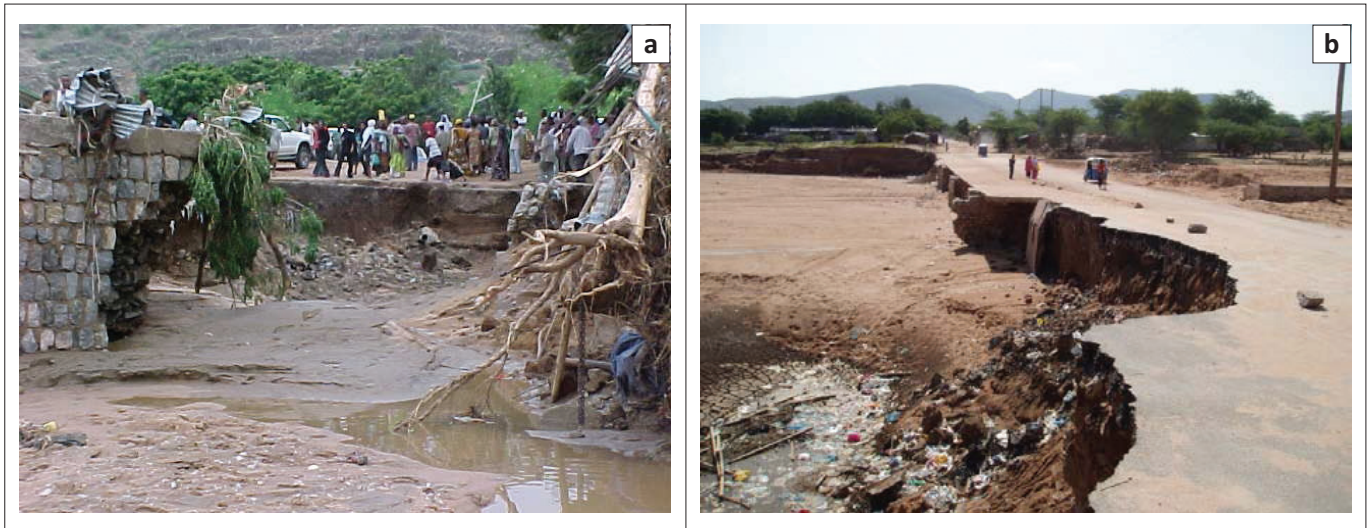
FIGURE 3: (a & b) Damage caused by 2006 floods on Dachatu Bridge and the road.
