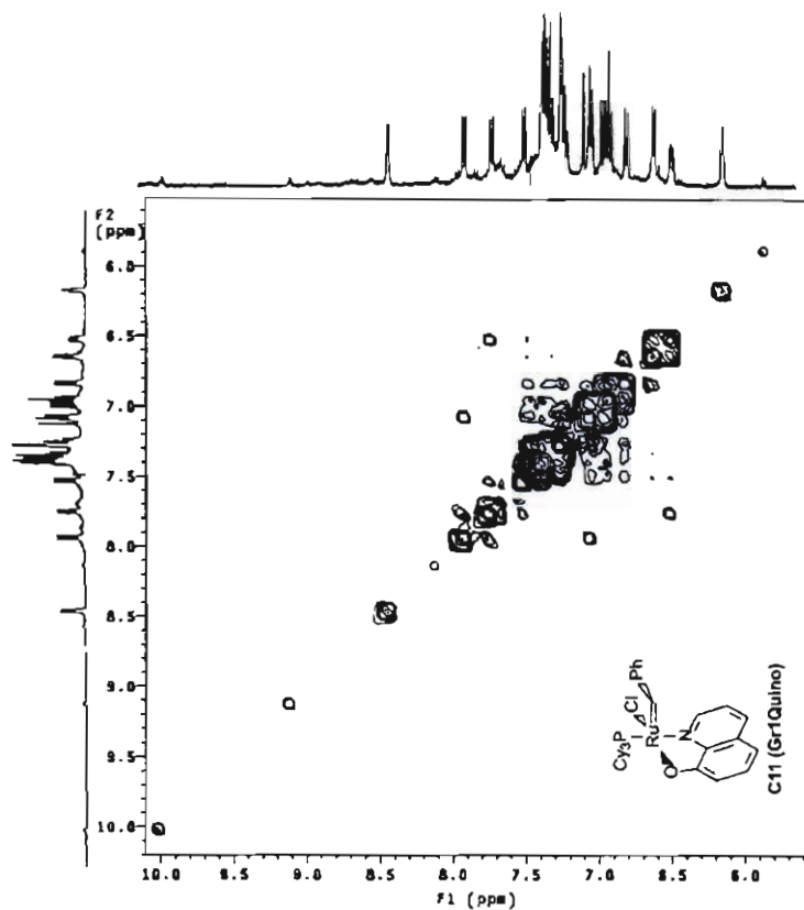
Spectrum C.35 COSY NMR spectrum of benzylidene-chloro(tricyclohexylphosphine)-[8-quinolinolato]ruthenium.
