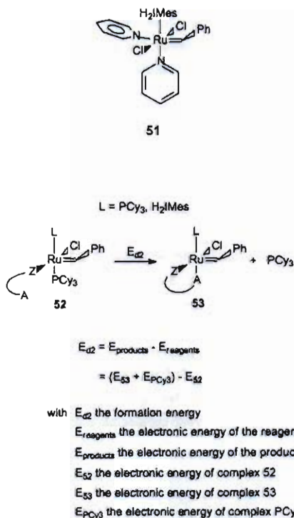
Scheme 4.10 Calculation of the formation energy of the chelating complexes.
