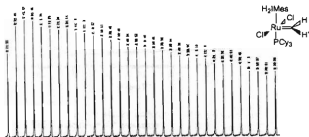
Figure 5.27 ^1\text{H} NMR signals at different time intervals of the carbene \alpha -H's in a 1-octene/Gr2 reaction mixture in \text{CDCl}_3 at 50^\circ\text{C} .
