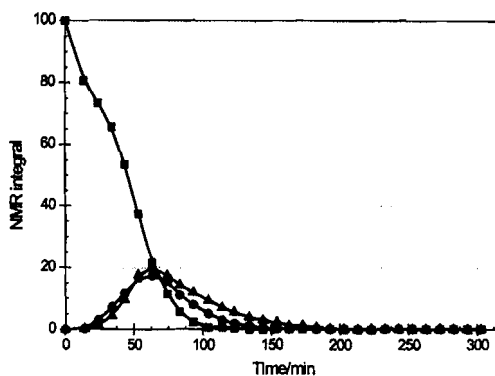
Figure 5.40 The ^1\text{H} NMR peak integration values (normalised) of the carbenes involved in the metathesis reaction of 1-octene in the presence of C7. [■ \delta 17.846 ppm, ● \delta 17.002 ppm, ▲ \delta 16.170 ppm]
