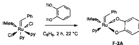
Scheme 4.7 Synthesis of a chelating catecholato derivative of a second generation Grubbs system. 18
