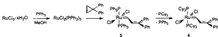
Scheme 2.5 Development of well-defined metathesis active ruthenium alkylidenes. 38,39
