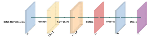
FIGURE 9. DL - Convolutional long-short-term memory neural network parameters (telemetry for predictive maintenance).
