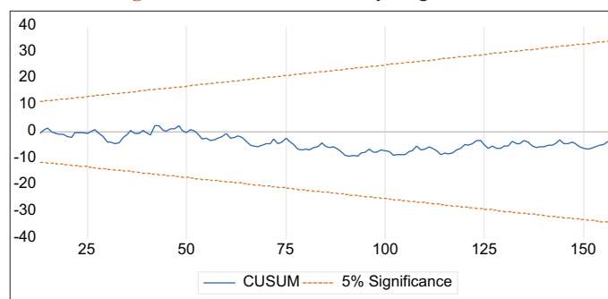
Figure 1: CUSUM for Stability diagnostic test
