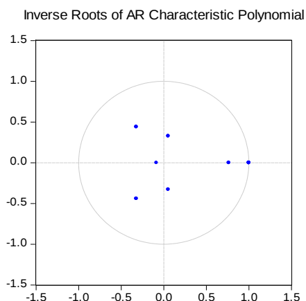
Figure 2: VEC stability condition check (Greece)
