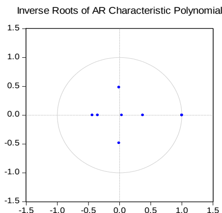
Figure 1: VEC stability condition check (USA)
