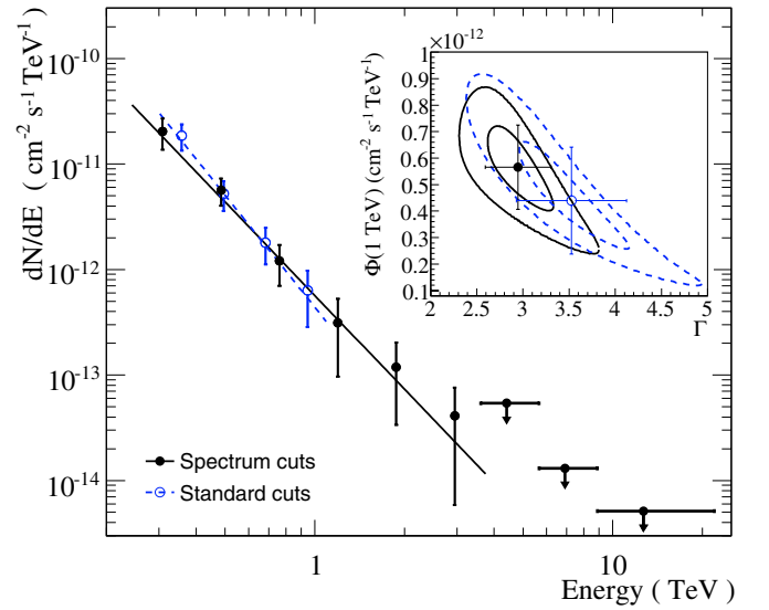
Fig. 2. Differential spectrum of RGB J0152+017. The spectrum obtained using spectrum cuts (black closed circles) is compared with the one obtained by the standard cuts (blue open circles). The black line shows the best fit by a powerlaw function of the former. The three points with the highest photon energy represent upper limits at 99% confidence level, calculated using Feldman & Cousins (1998). All error bars are only statistical. The fit parameters of a powerlaw fit are \Gamma = 2.95 \pm 0.36_{\text{stat}} \pm 0.20_{\text{syst}} and \Phi(1\text{ TeV}) = (5.7 \pm 1.6_{\text{stat}} \pm 1.1_{\text{syst}}) \times 10^{-13} \text{ cm}^{-2} \text{ s}^{-1} \text{ TeV}^{-1} for the spectrum cuts , and \Gamma = 3.53 \pm 0.60_{\text{stat}} \pm 0.2_{\text{syst}} and \Phi(1\text{ TeV}) = (4.4 \pm 2.0) \times 10^{-13} \text{ cm}^{-2} \text{ s}^{-1} \text{ TeV}^{-1} for the standard cuts . The insert shows 1 and 2\sigma confidence levels of the fit parameters.
