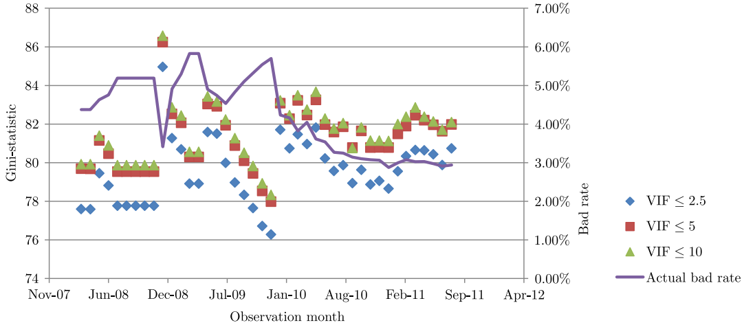
Figure 5: A comparison of the three models' Gini-statistics from month-to-month. [Figure can be viewed in colour in the electronic version, available at http://orion.journals.ac.za .]
