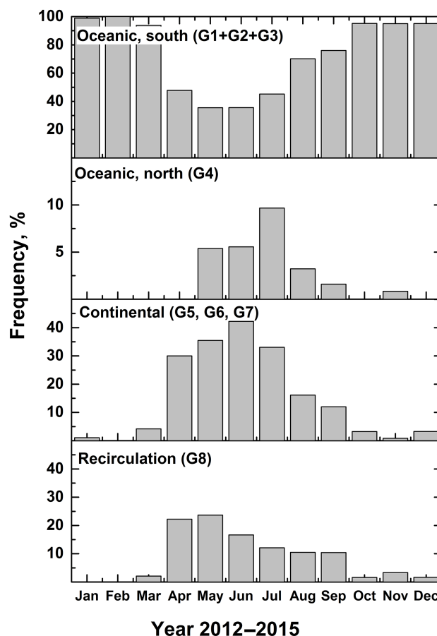
Figure 5. Seasonal variation in the transport pathways of air masses reaching HBAO between 2012 and 2015.
