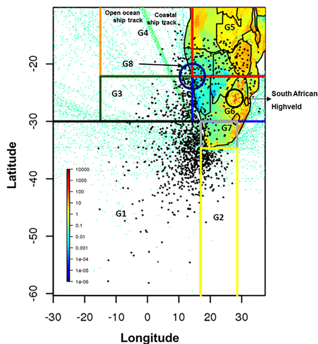
Figure 3. Geographical boundaries of the sectors used to classify the air mass back-trajectories superimposed to the emission grid maps at 0.1^\circ \times 0.1^\circ of BC aerosols from anthropogenic activities for the year 2010 provided by the HTAP_V2 inventory. Emissions are expressed in tonnes.
