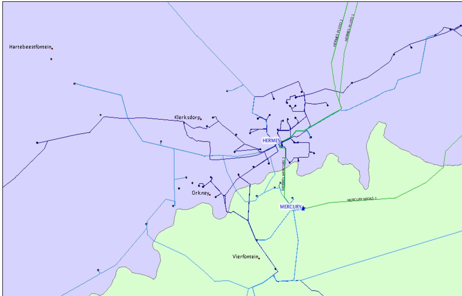
FigureA.9: Distribution - transmission map North West province.
