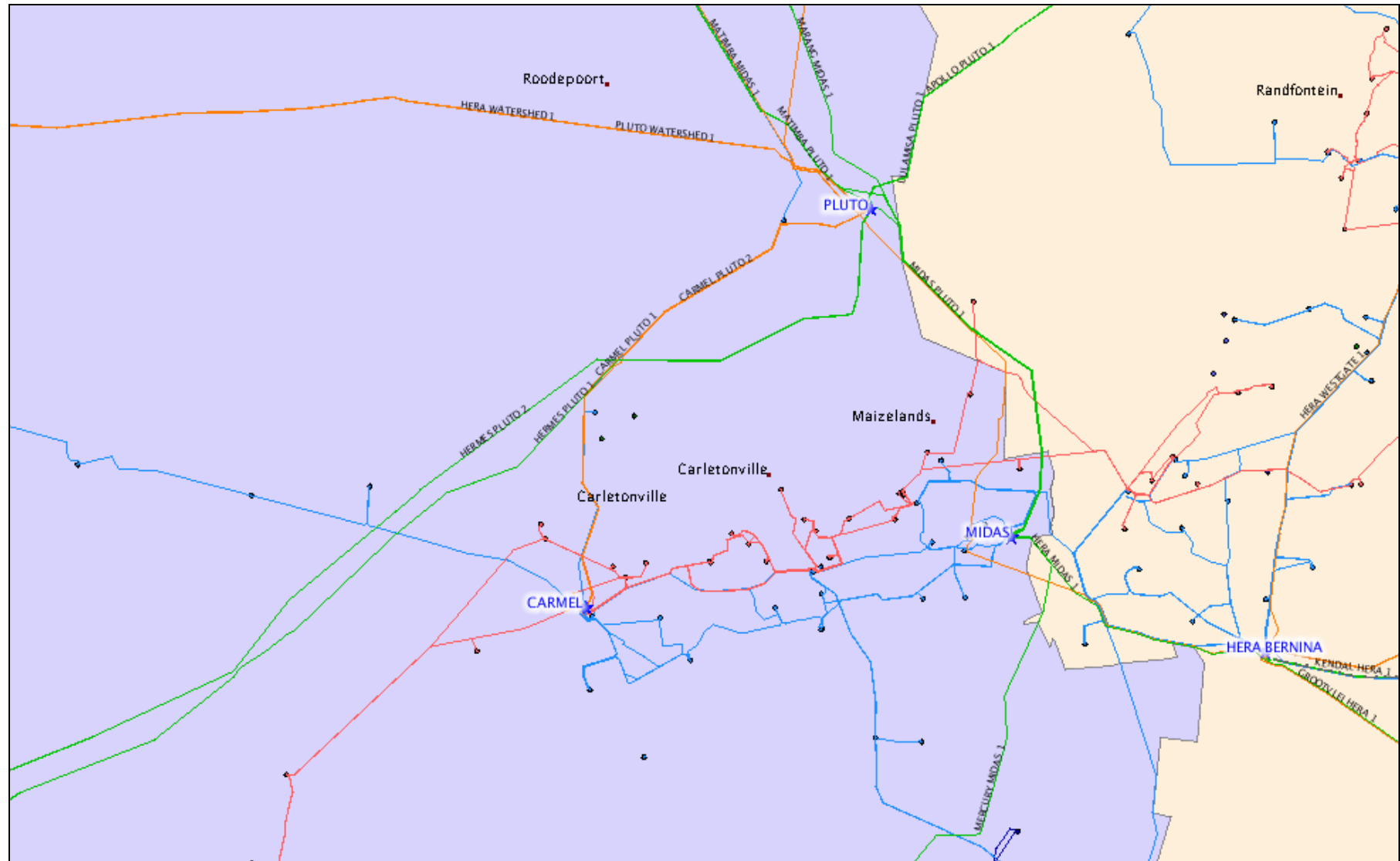
FigureA.10: Distribution - transmission map North West province.
