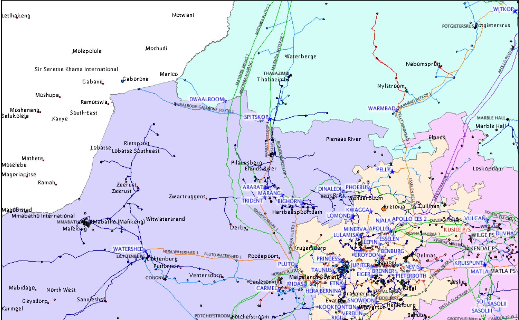
FigureA.1: Distribution - transmission map North West province.
