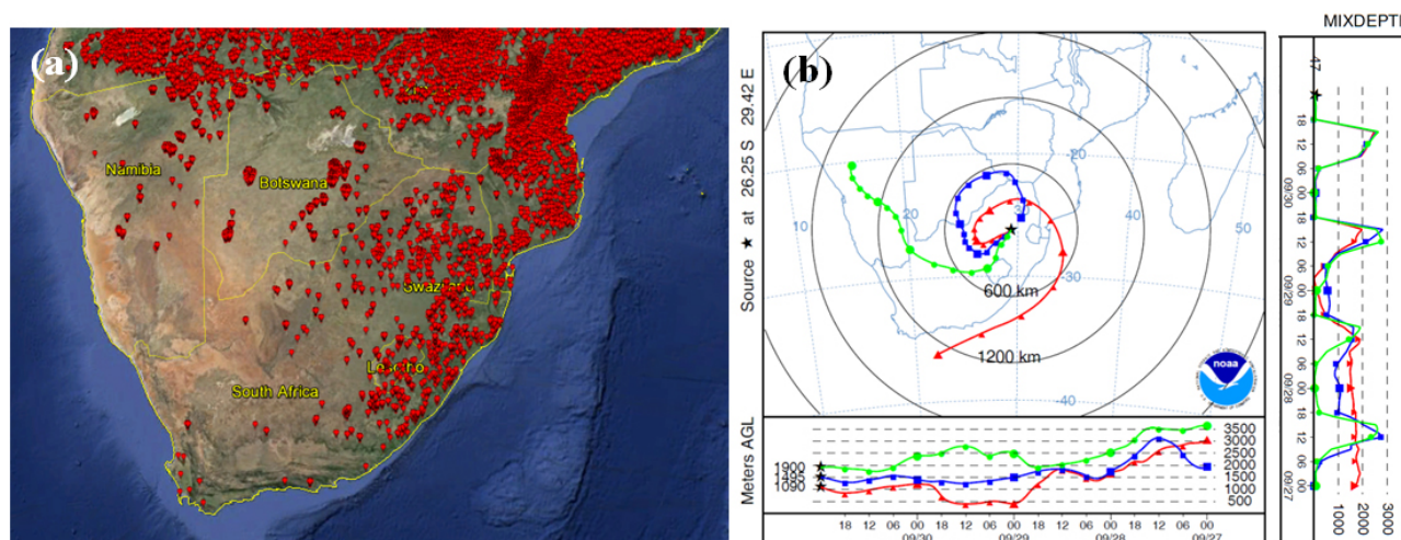
Figure 3. MODIS fire hotspots for the period 28 September 2010–1 October 2010 and for the latitude range between -35 and -15^{\circ} S and the longitude range between 10 and 40^{\circ} E (a). Four-day backward trajectories arriving at Elandsfontein on 1 October 2010 at 00:00 UTC for arrival height of the bottom (1090 m), centre (1495 m) and top (1900 m) of the aerosol layer observed (b).
