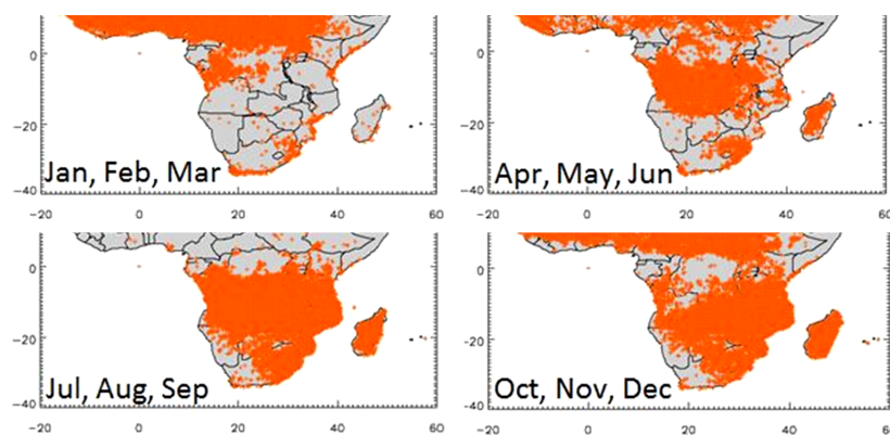
Figure 2. Number of fire hotspots with confidence levels between 80 and 100 % averaged in terms of 3 months for the year 2010 in the latitude range between -40 and 10^{\circ} and longitude range between -20 and 60^{\circ} .
