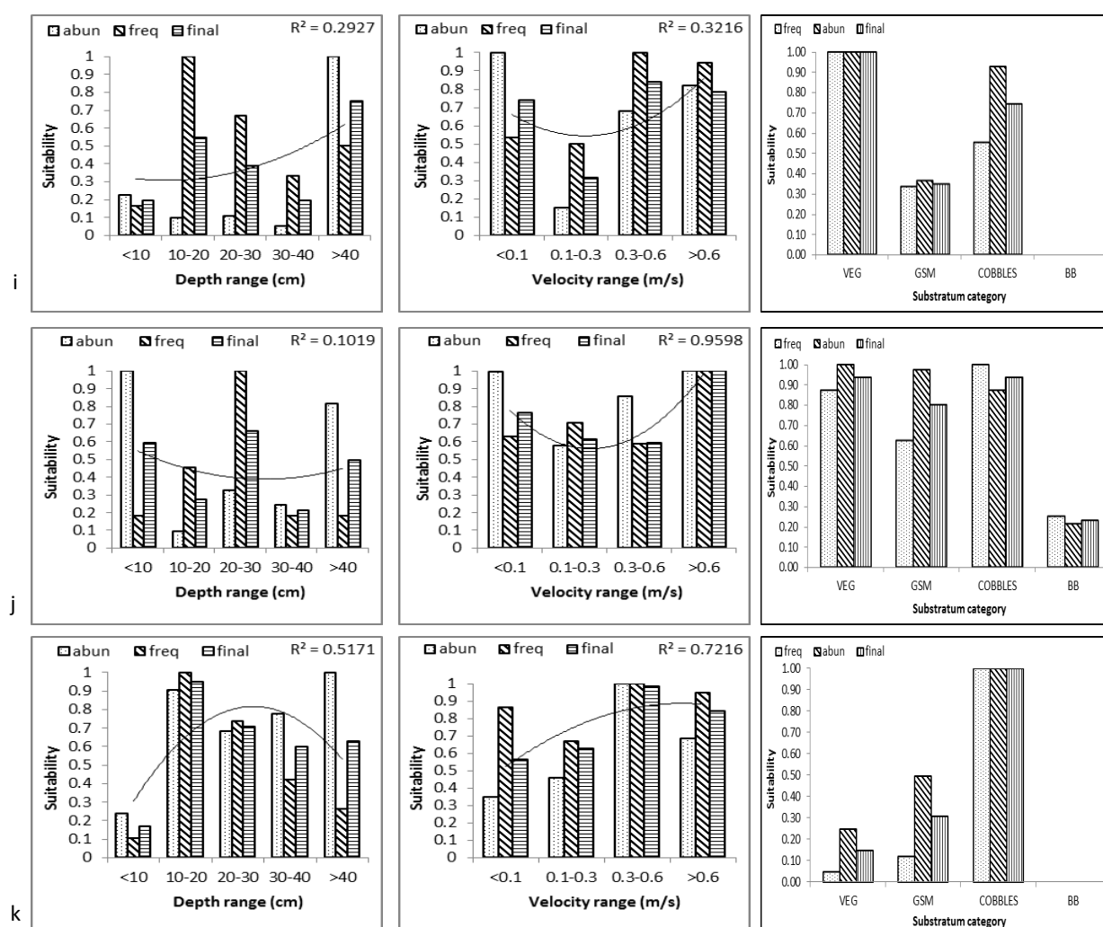
Figure 3.9 (continued): Habitat Suitability Curves based on depth (cm), velocity (m/s) and substratum category for Coleoptera: (a) Dytiscidae, (b-d) Elmidae, (e-g) Gyrinidae, (h) Hydraenidae, (i) Hydrophilidae, (j) Scirtidae, and (k) Psephenidae. A second order polynomial regression was used to fit the data and where significant the R^2 value is provided. Vegetation: VEG; Gravel, Sand & Mud: GSM, Bedrock & Boulders:BB
