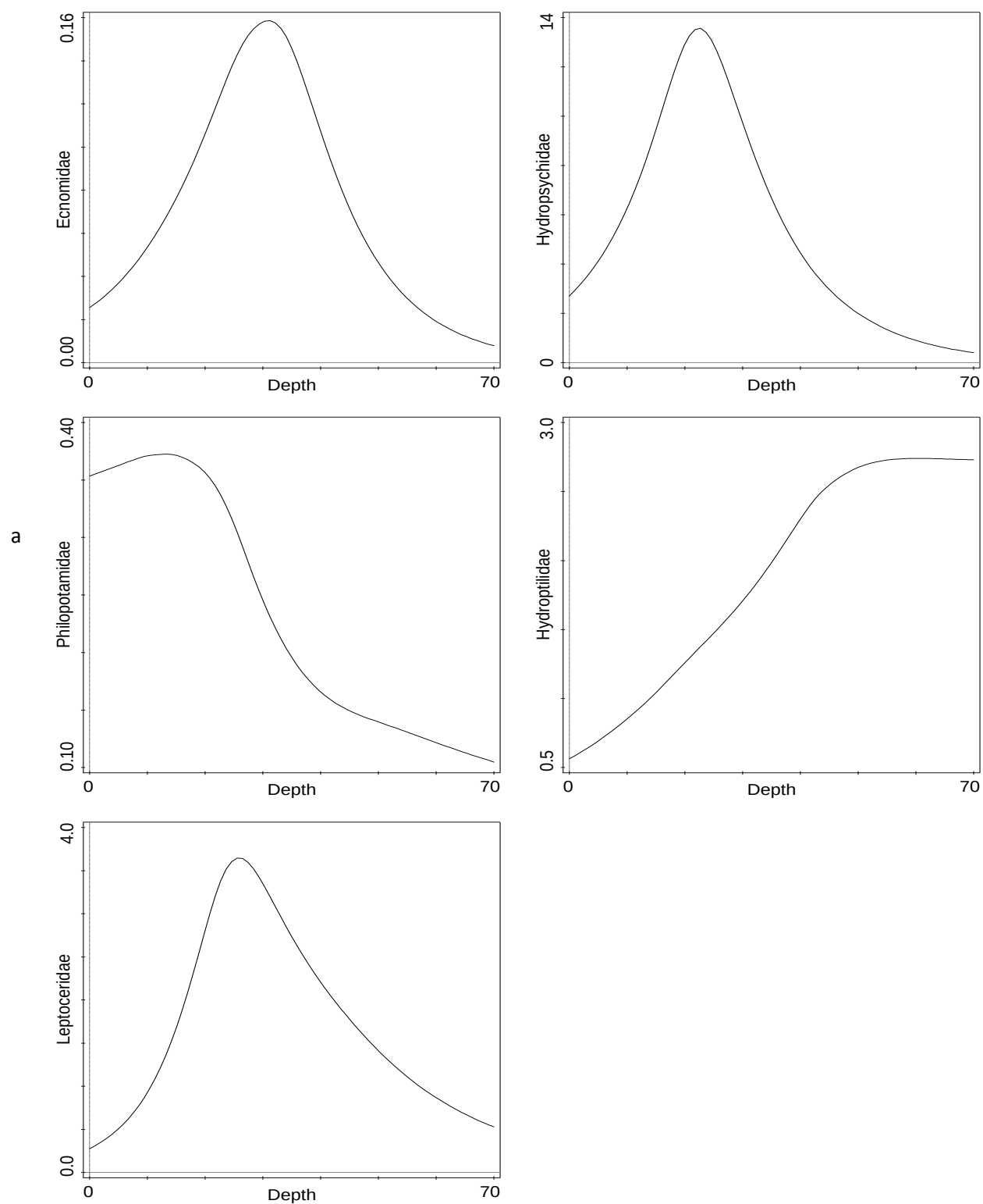
Figure 3.6: Generalised Additive Model graphs indicating the response of Trichoptera to: (a) Depth, (b) Velocity at 60% of the depth (vel@ 60%) and (c) Substratum.
