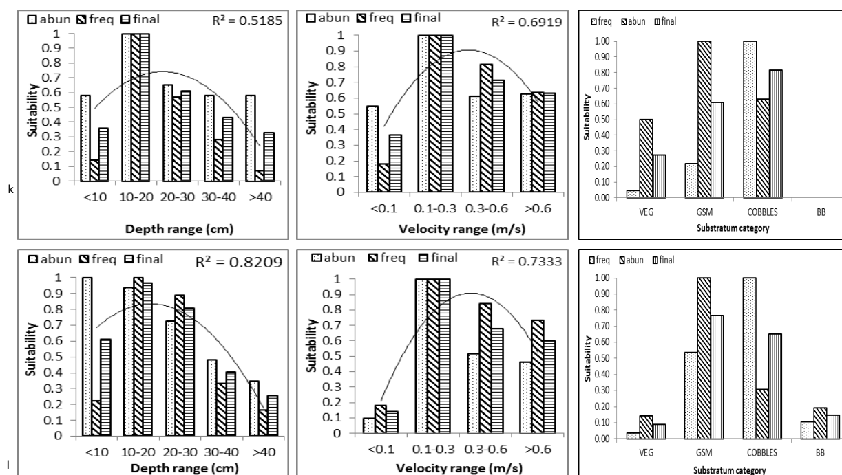
Figure 3.10 (continued): Habitat Suitability Curves based on depth (cm), velocity (m/s) and substratum category for Diptera (a) Athericidae, (b) Blephariceridae, (c) Ceratopogonidae, (d-f) Chironomidae, (g) Empididae, (h-j) Simuliidae, (k) Tabanidae and (l) Tipulidae. A second order polynomial regression was used to fit the data and where significant the R^2 value is provided. Vegetation: VEG; Gravel, Sand & Mud: GSM, Bedrock & Boulders:BB
