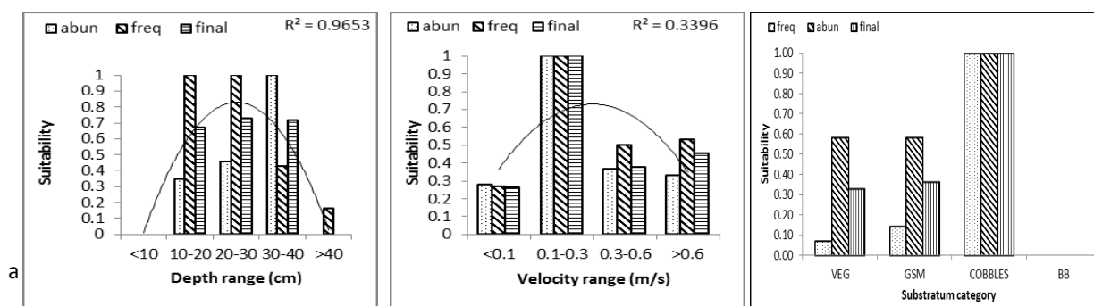
Figure 3.12: Habitat Suitability Curves based on depth (cm), velocity (m/s) and substratum category for Trichoptera: (a) Ecnomidae, (b) Hydropsychidae, (c) Philopotamidae, (d) Hydroptilidae and (e) Leptoceridae. A second order polynomial regression was used to fit the data and where significant the R 2 value is provided. Vegetation: VEG; Gravel, Sand & Mud: GSM, Bedrock & Boulders:BB
