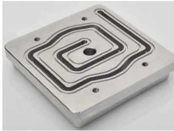
Figure 4: Cooling channels manufactured using conventional machining methods
