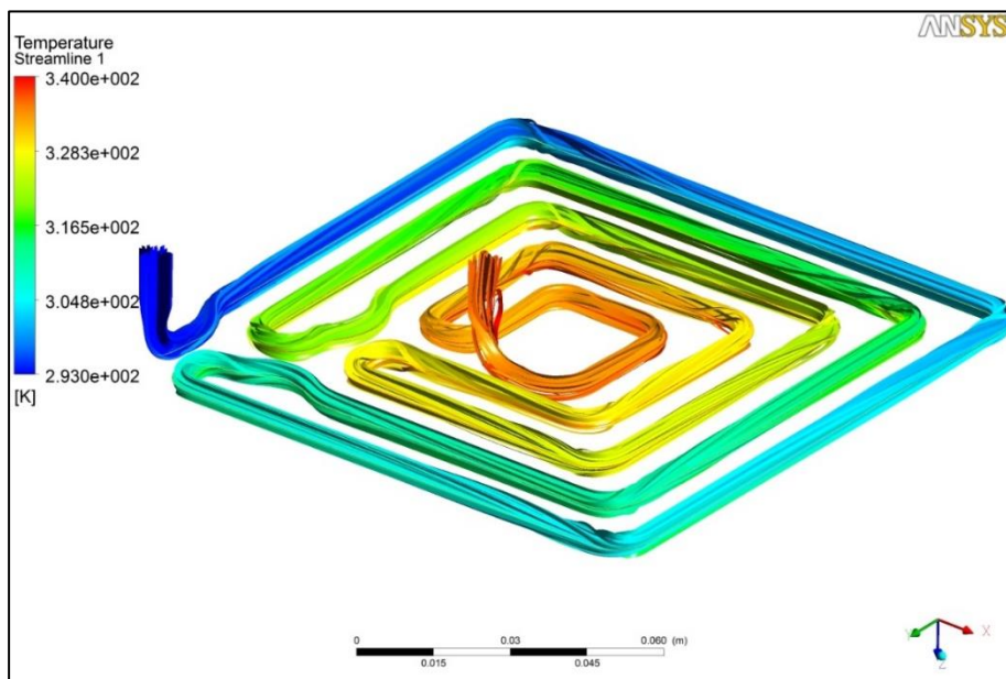
Figure 15: Meander streamline temperature (see online version for colour)
