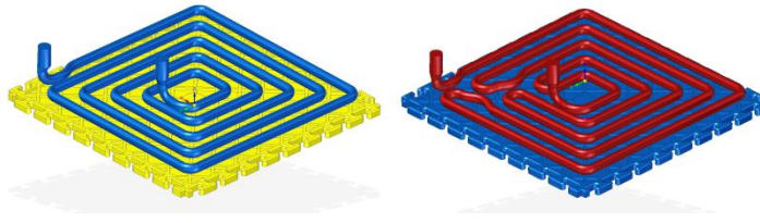
Figure 13: Spiral and meander conformal cooling design
