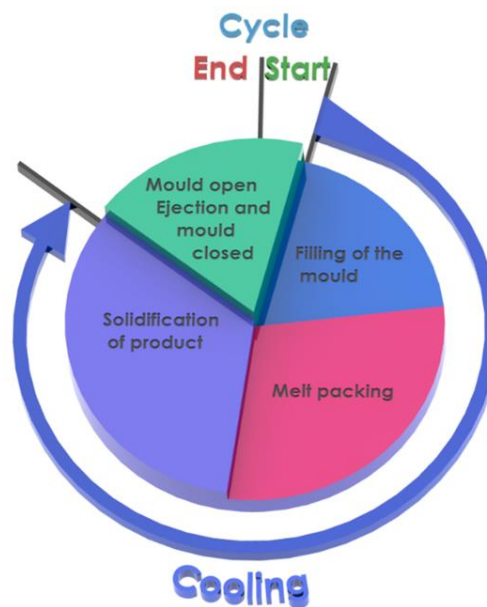
Figure 1: Injection moulding cycle
