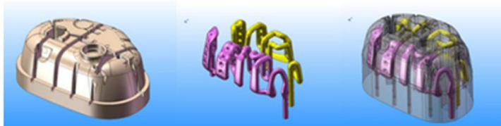
Figure 6: Example of conformal cooling channels designed by Pole Européen de la Plastyrgie (PEP) [2]
