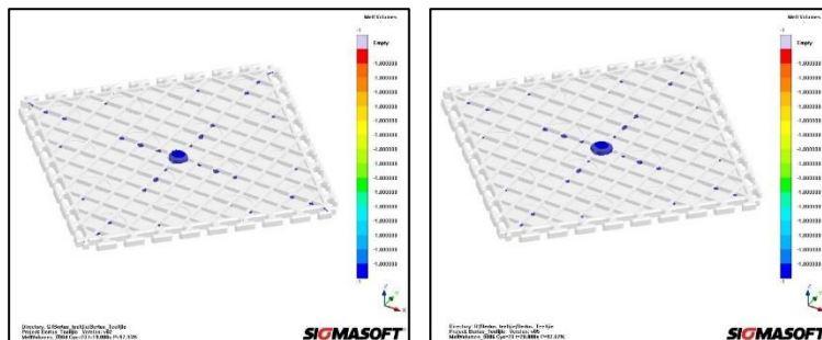
Figure 19: Solidification of product (left side conformal; right side conventional) (see online version for colour)
