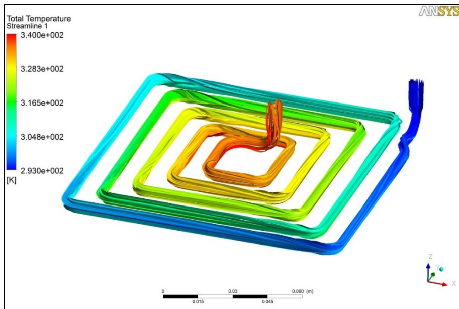
Figure 14: Spiral streamline temperature (see online version for colour)
