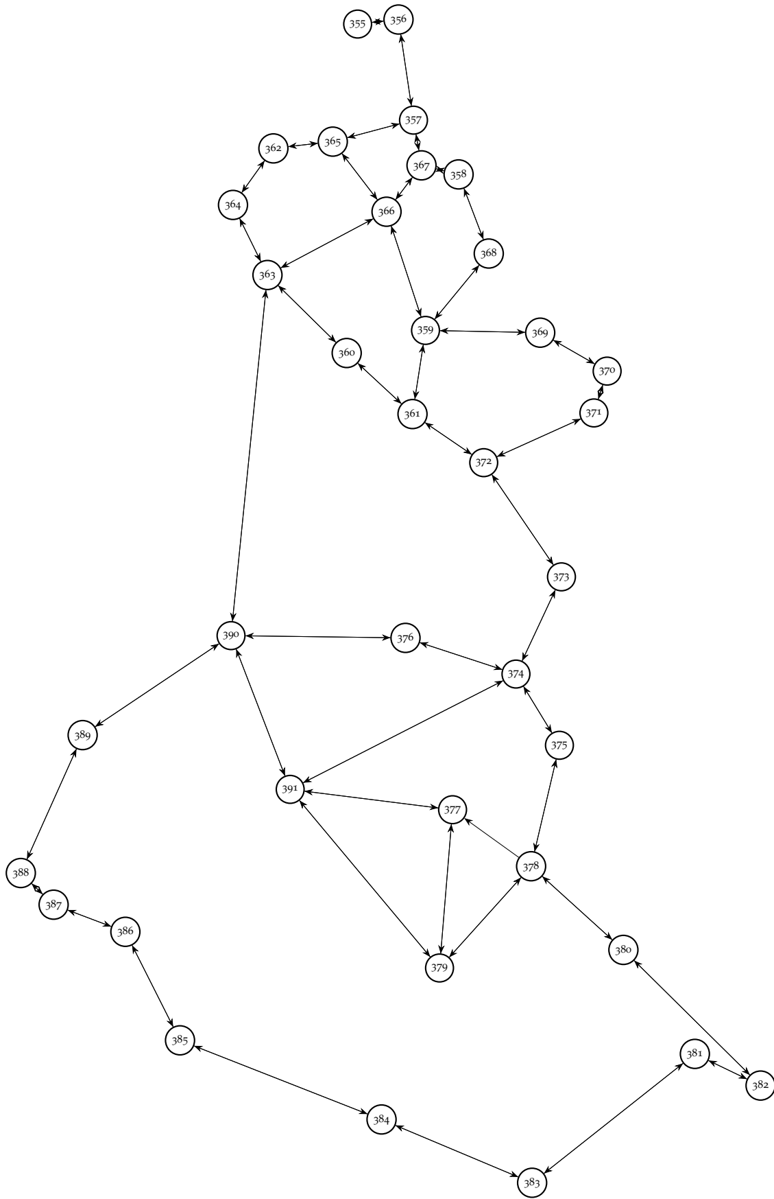
Figure 39: smallo10 visualisation.
