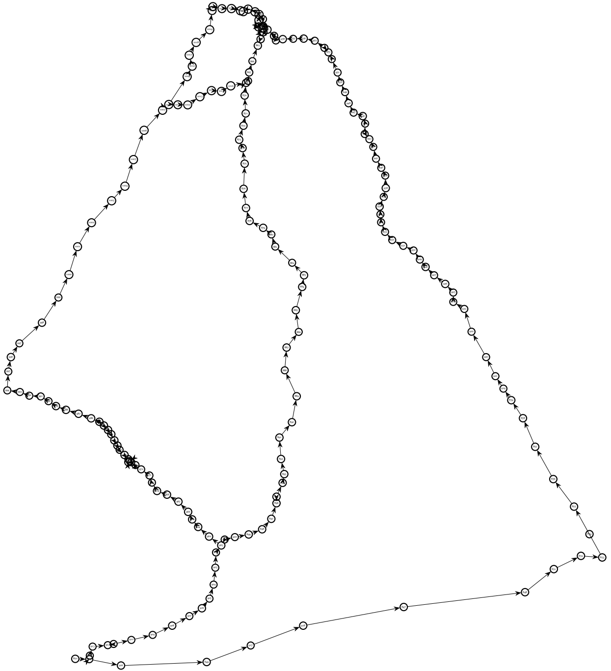
Figure 41: mediumoo2 visualisation.
