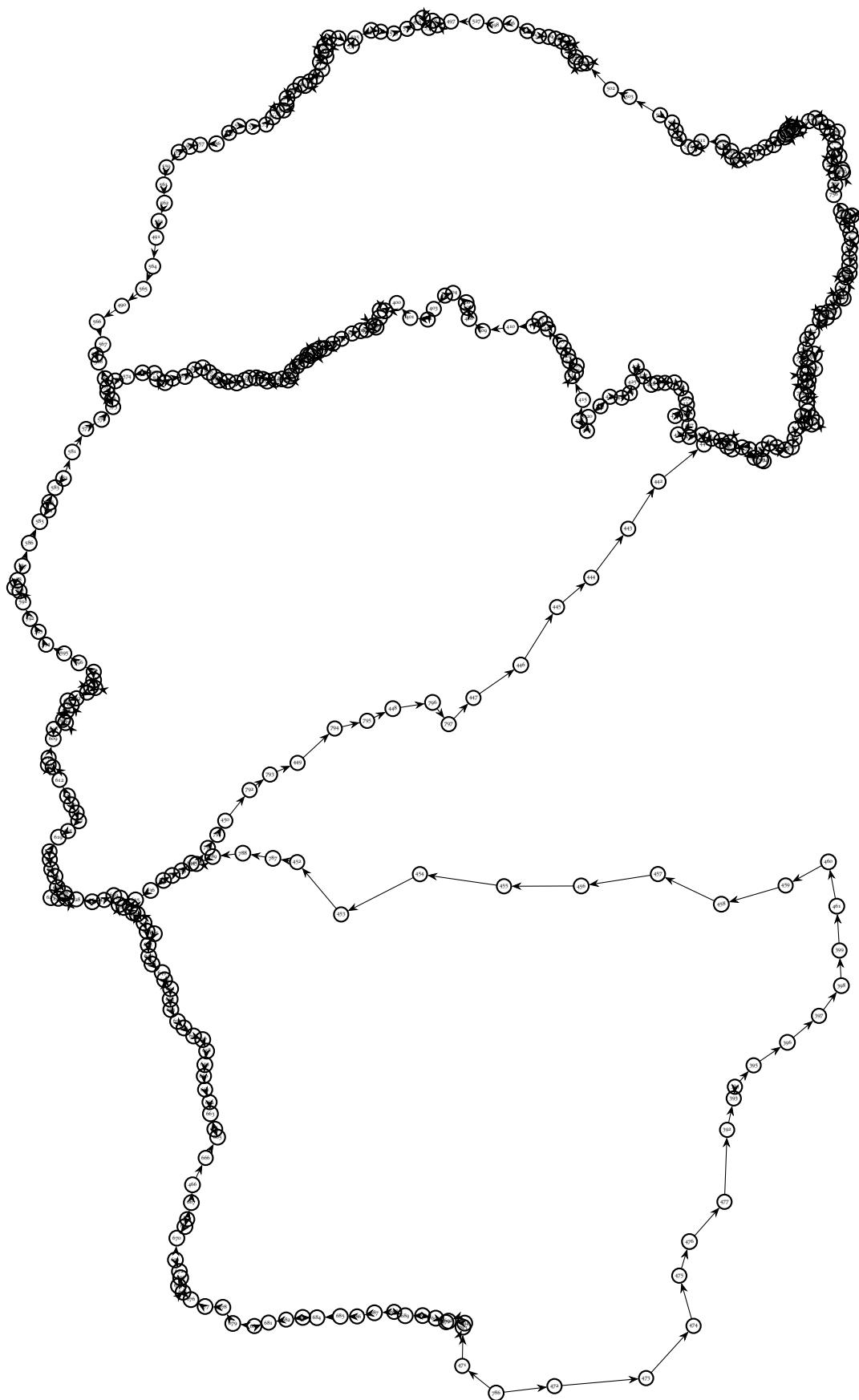
Figure 40: medium001 visualisation.
