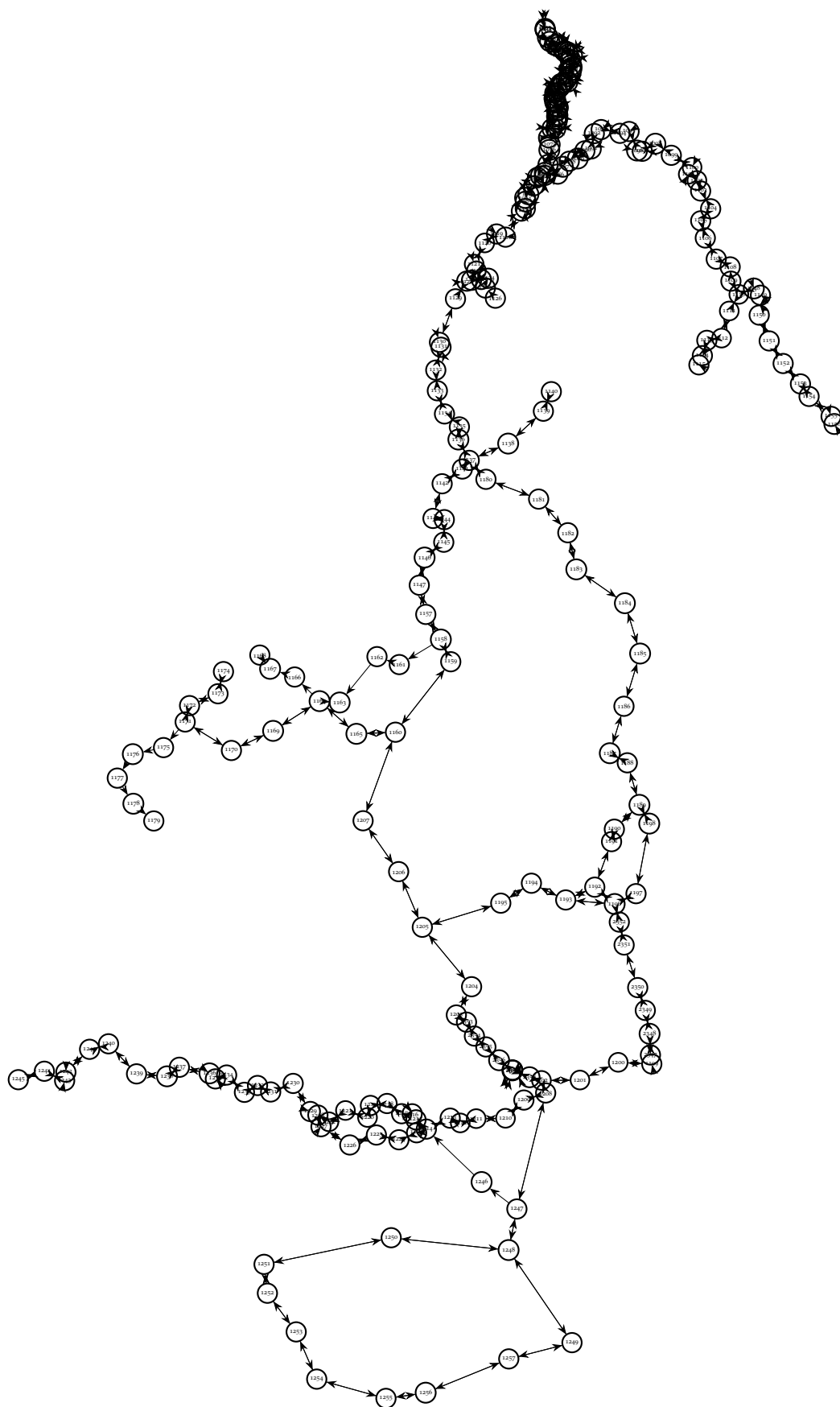
Figure 42: mediumoo3 visualisation.
