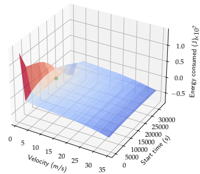
(f) Energy graph for segment 5.
