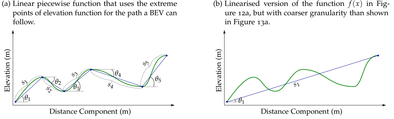
Figure 13: Side-by-side comparison showing the problem of not using enough vertices to linearise a non-linear function (Figure 13b).
