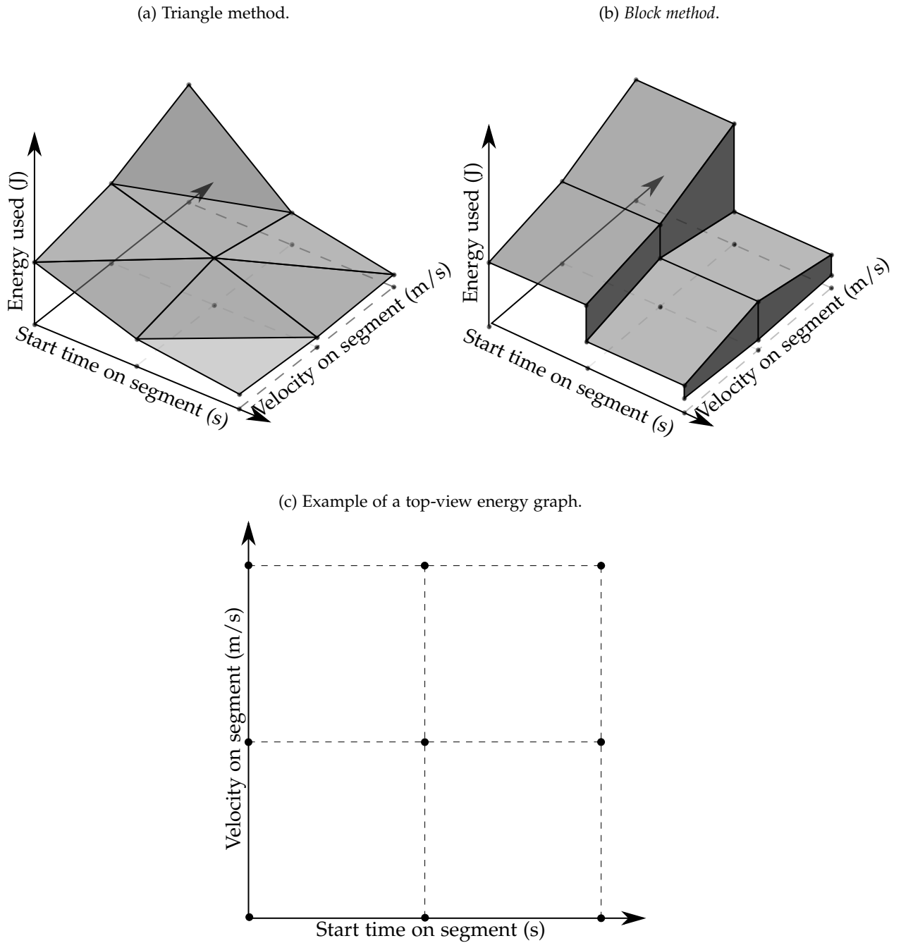
Figure 19: Illustrations to represent energy graphs.
