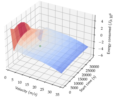
(f) Energy graph for segment 56.
