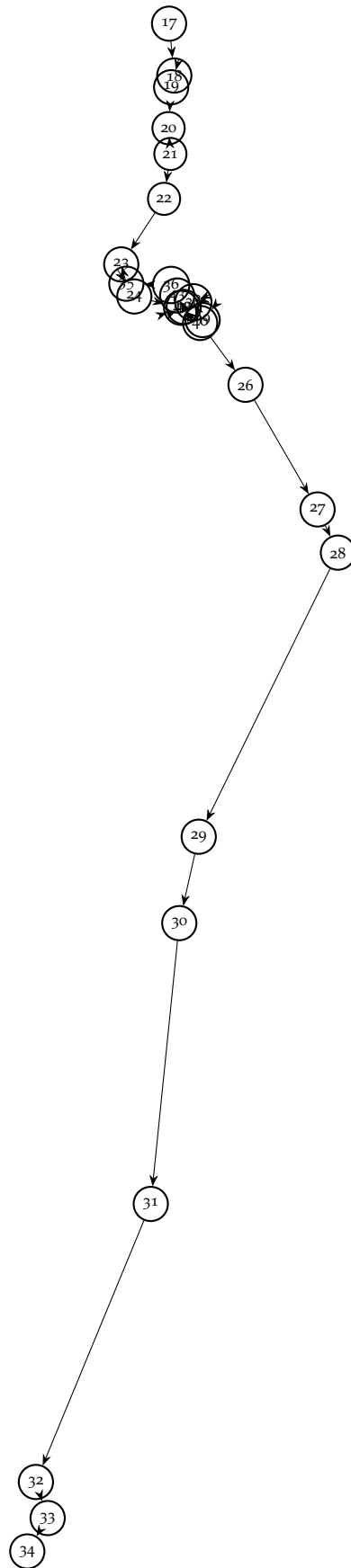
Figure 31: smalloo2 visualisation.
