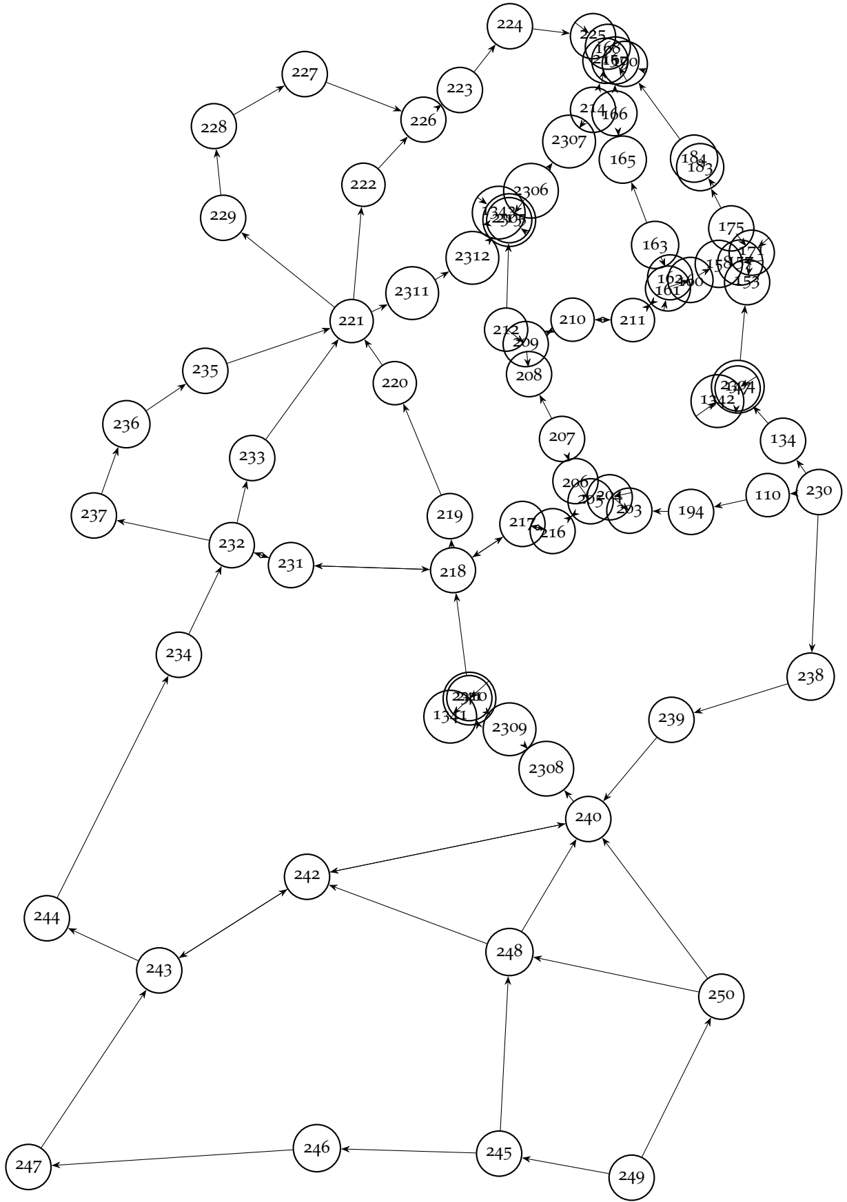
Figure 33: smalloo4 visualisation.
