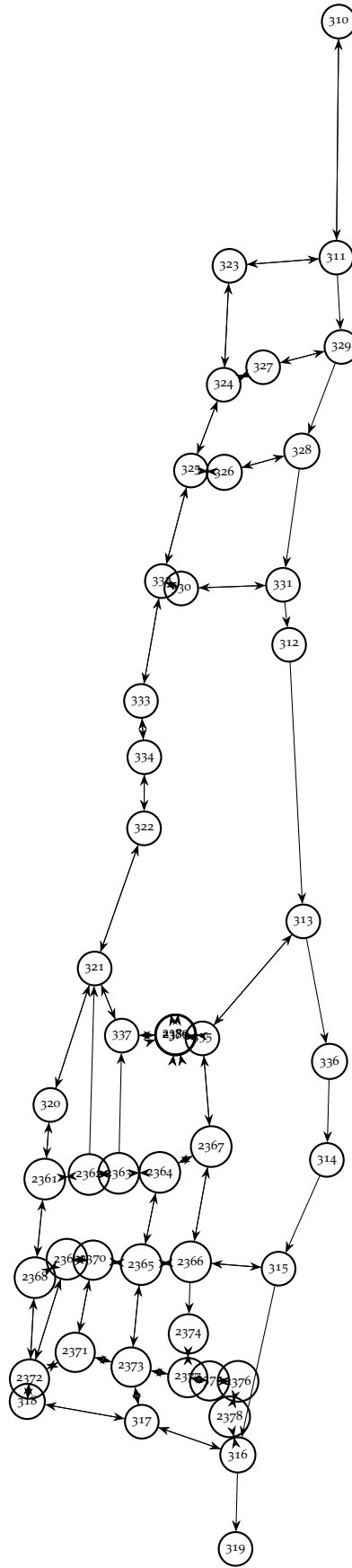
Figure 37: smalloo8 visualisation.
