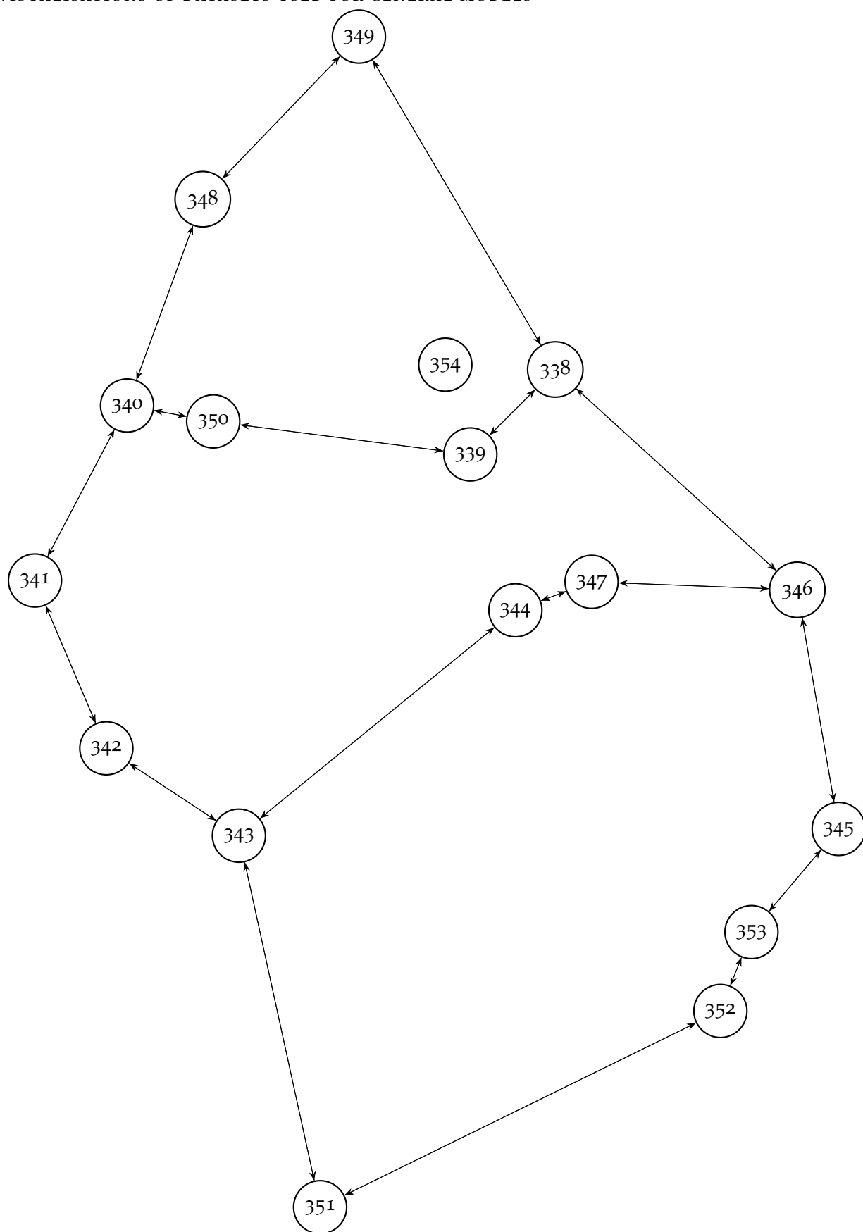
Figure 38: smalloo9 visualisation.
