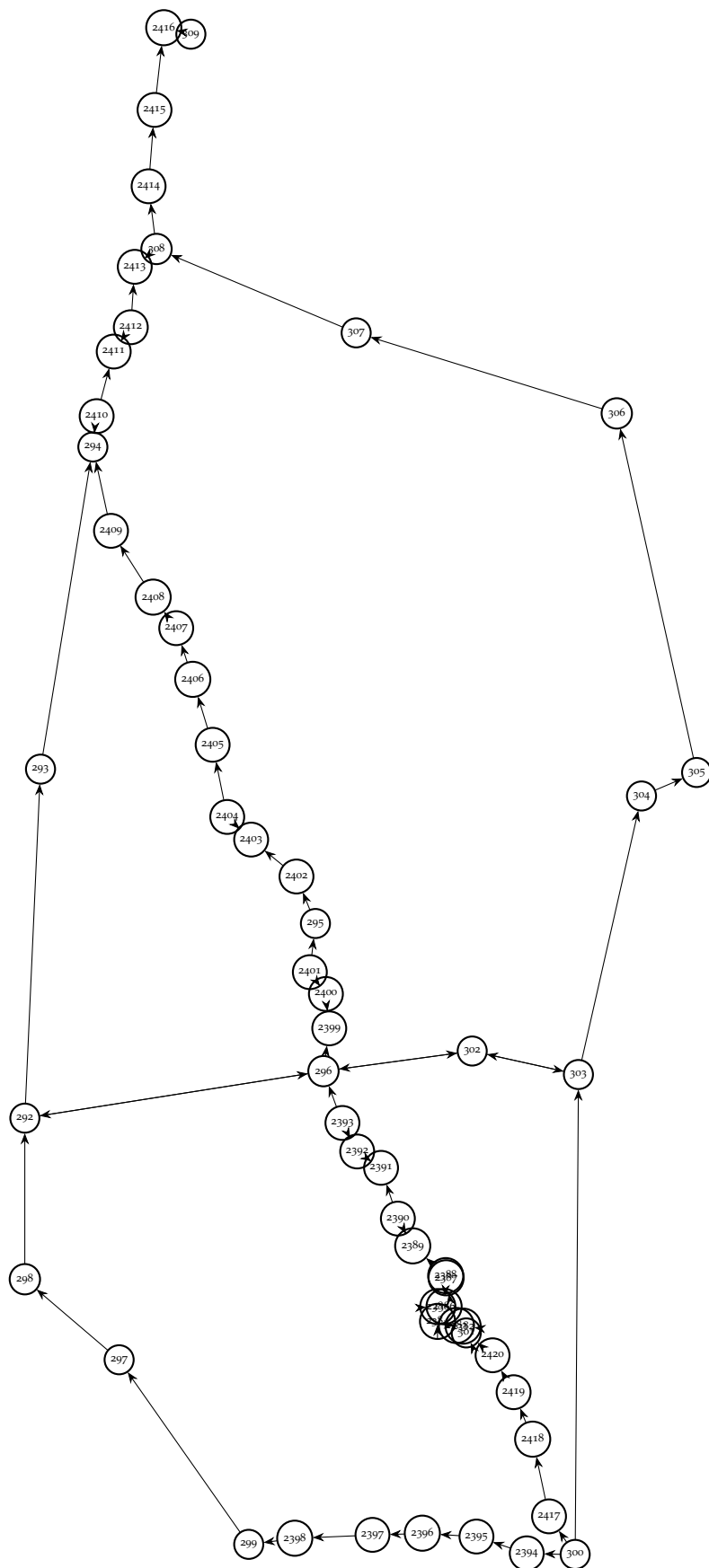
Figure 36: smalloo7 visualisation.
