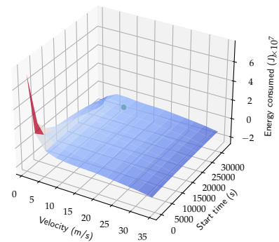
Figure 57: Energy graphs for segment 0 to 5 on day 1.
