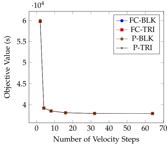
(c) Objective value as granularity of velocity increase.
