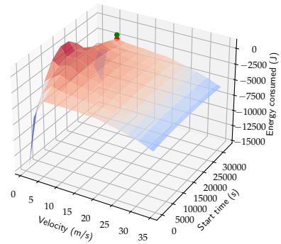
Figure 56: Energy graphs for segment 63 to 68.
