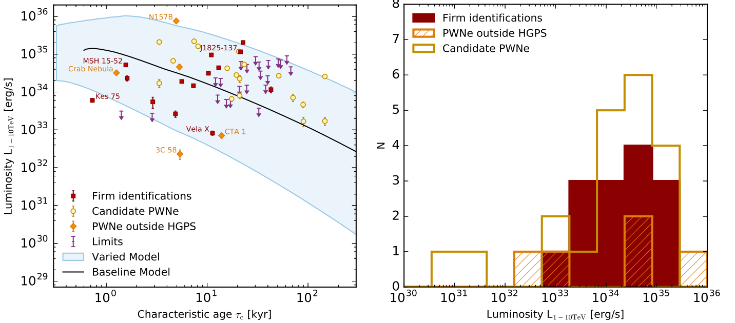
Fig. 8. Left: evolution of TeV luminosity with characteristic age. Right: distribution of 1–10 TeV luminosity for PWNe and PWN candidates treated in this work.
