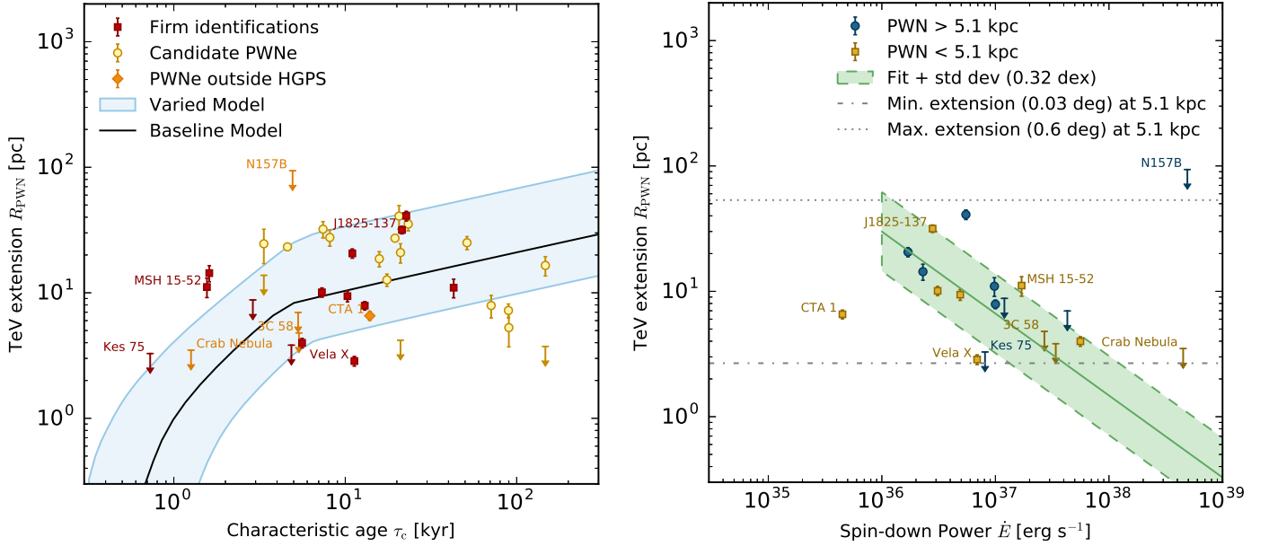
Fig. 5. Left: PWN extension evolution with time, in comparison to the modelling considered in this work. Right: PWN extension evolution with \dot{E} , as fitted in the R_{\text{PWN}}(\dot{E}) column of Table 6 for pulsar wind nebulae with \dot{E} > 10^{36} erg s ^{-1} (see Sect. 5.2.1). The shaded range shows the fit range and standard deviation \sigma_{\text{lg } Y} . 1 dex refers to an order of magnitude and is the unit of the logspace defined \sigma_{\text{lg } Y} . For clarity, this plot excludes PWN candidates and divides the sample into nearby and far pulsar wind nebulae to illustrate the potential selection or reconstruction bias (see text). The dot-dashed and dotted lines indicate the systematic minimum of 0.03^\circ and the maximum measured extension in the HGPS of 0.6^\circ , respectively, which are both projected to the average PWN distance of 5.1 kpc.
