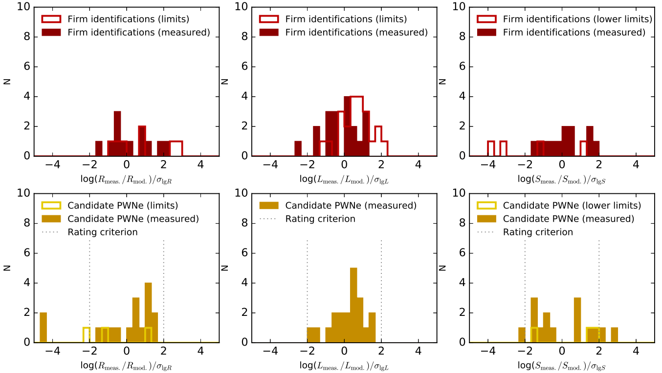
Fig. 11. Common logarithmic residuals of rating criteria 2–4, using the standard deviations \sigma_{\text{lg}Y} explained in Sect. 6. Left: extension with respect to the model shown in Fig. 5 (left). Middle: same for luminosity (Fig. 7, left). Right: same for surface brightness (Fig. 10, left). In all cases, limits are shown separately as outlined histograms.
