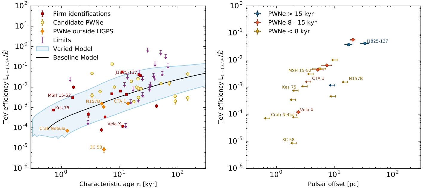
Fig. 9. Left: evolution of TeV efficiency ( L_{1-10\text{TeV}}/\dot{E} ) with pulsar characteristic age. Right: TeV efficiency as a function of pulsar offset, plotted for pulsars of different age groups. High-offset systems tend to be more TeV-efficient than low-offset systems.
