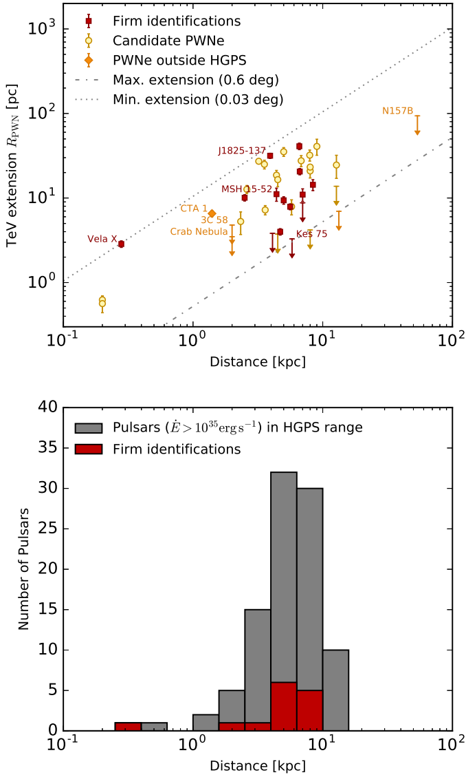
Fig. 4. Top: PWN extension occurrences over distance from Earth, in comparison to the band of extensions that can be expected to be identified in the HGPS analysis chain. Bottom: distribution of known distances of energetic pulsars ( \dot{E} > 10^{35} \text{ erg s}^{-1} ).
