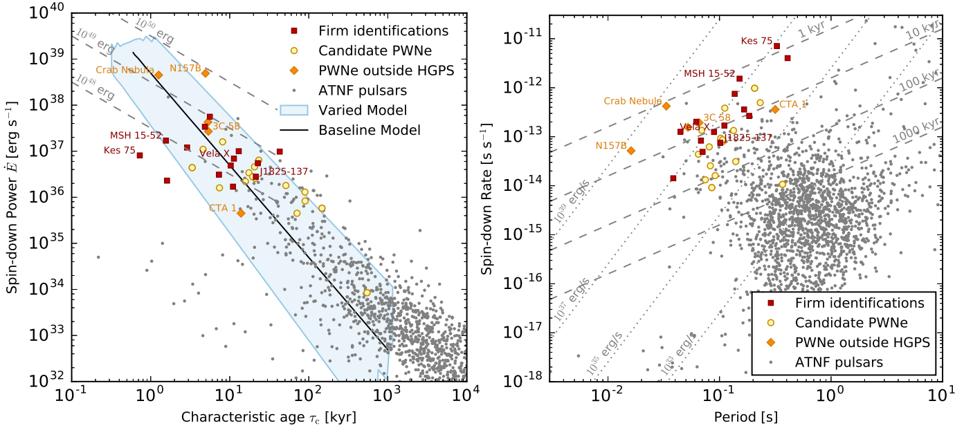
Fig. 2. Left: spin-down power \dot{E} and characteristic age \tau_c of pulsars with a firmly identified PWN, candidate PWN, and without TeV counterpart (grey dots). The black line and shaded band show the injection evolution of the modelling used in this paper. The dashed lines indicate lines of constant total remaining energy \dot{E}\tau_0 ; see Appendix B. Hence a model curve that starts at \dot{E}_0\tau_0 = 10^{49} erg represents a pulsar with total initial rotational energy of 10^{49} erg. Since both \dot{E} and \tau_c depend on P and \dot{P} , the axes in this plot do not represent independent quantities. Right: same data, shown in the commonly used view, using the independently measured P and \dot{P} .
