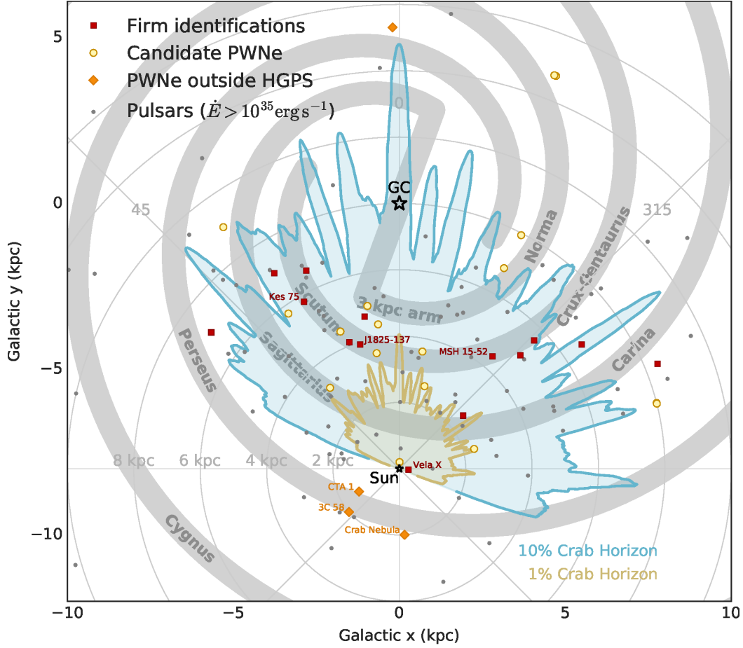
Fig. 3. Schematic of the Milky Way and its spiral arms, along with firmly identified PWNe, candidates, and energetic pulsars ( \dot{E} > 10^{35} \text{ erg s}^{-1} ) without detected TeV wind nebula. The yellow and blue curves outline the sensitivity horizon of the HGPS for point-like sources with an integrated gamma-ray luminosity (1–10 TeV) of 1% and 10% of the Crab luminosity, respectively (see H.E.S.S. Collaboration 2018 , for details).
