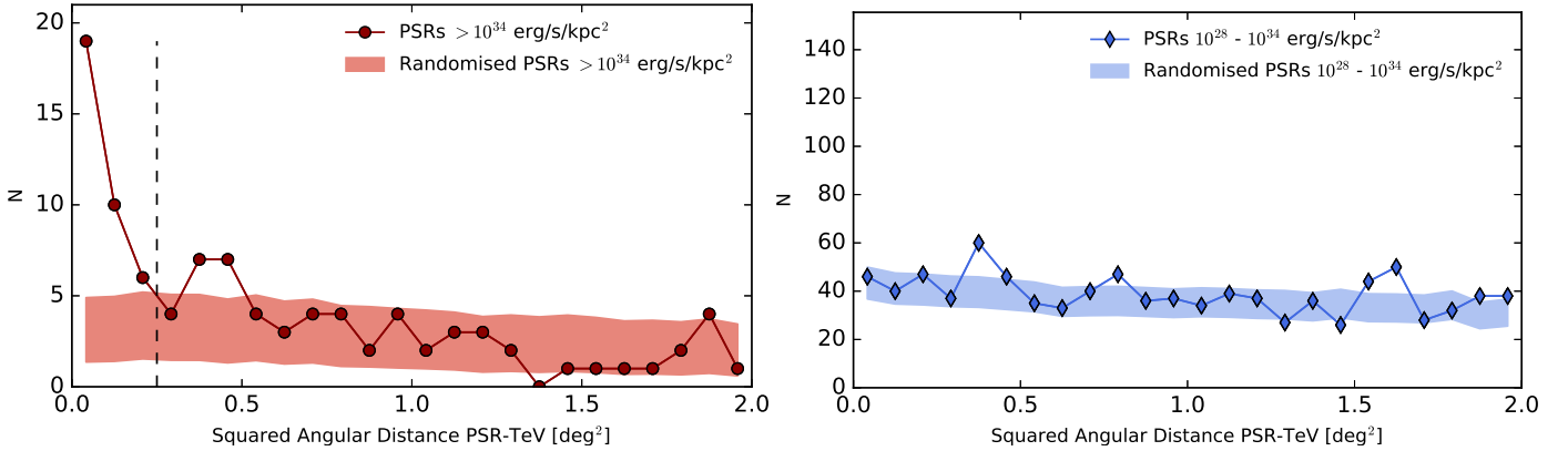
Fig. 1. Histograms of spatial separation between PMPS pulsars and TeV source components from the HGPS list. In the high- \dot{E} pulsar sample (left), a clear correlation is seen as a peak at small squared angular distances, whereas the low- \dot{E} associations, if present, are not significant beyond the expected rate of chance coincidences (right). The angular separation cut of \theta < 0.5^\circ applied in the preselection of PWN candidates (Sect. 3.2) is indicated by a dashed vertical line in the left panel.
