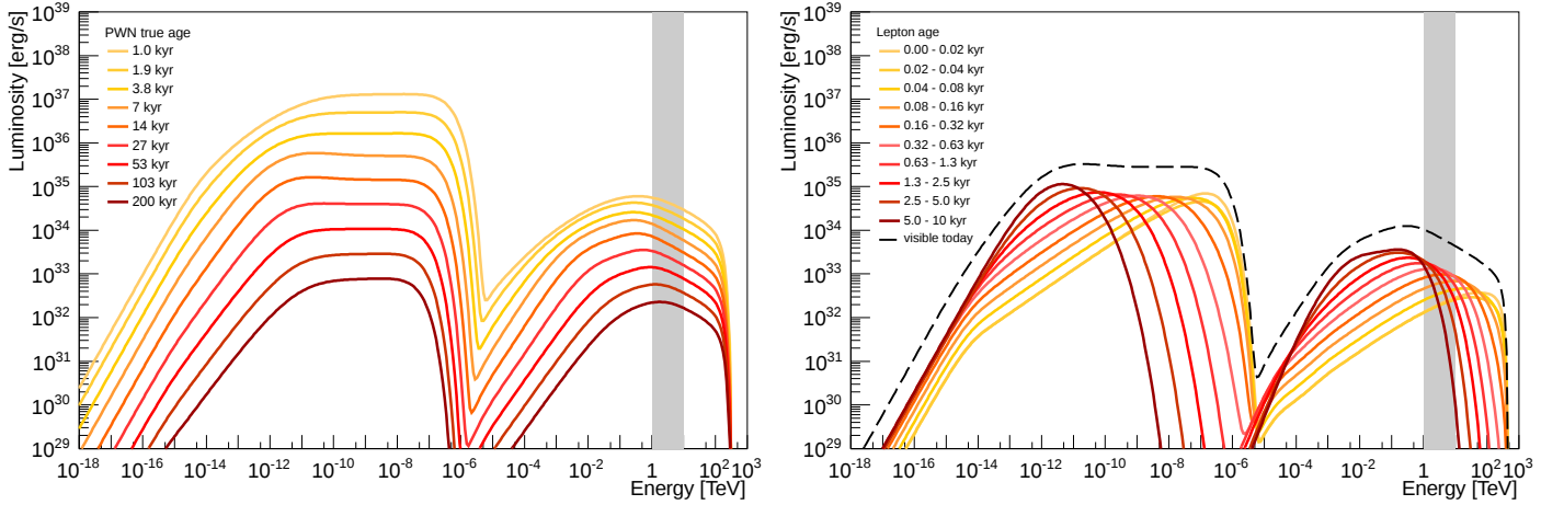
Fig. A.1. Modelled spectral energy distribution (SED) of a generic PWN with parameters according to baseline model given in Table A.1. See Appendix A.7 for caveats of the SEDs. Left: time evolution of the SED, ranging from 1 kyr to 200 kyr. Right: decomposition of the SED of a middle-aged PWN (10 kyr; black dashed curve) into contributions by leptons from various injection epochs (coloured lines). The grey-shaded bands indicate the energy range of 1–10 TeV explored in this paper.
