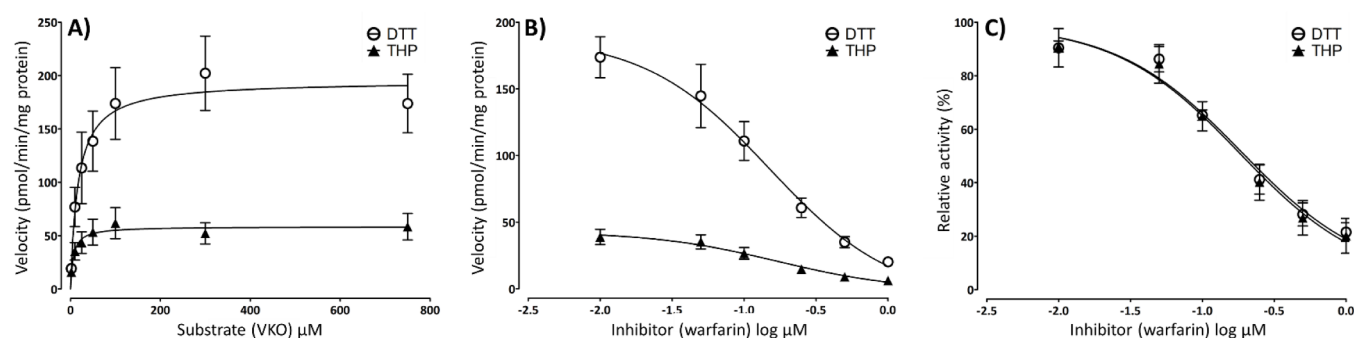
Fig. 1. Michaelis–Menten plots of VKOR activity
