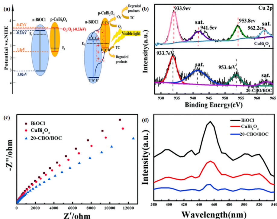
Fig. 6. (a) Proposed charge transfer mechanism for CuBi 2 O 4 /BiOCl (b) XPS spectra of the Cu 2p orbital of CuBi 2 O 4 and CuBi 2 O 4 /BiOCl-the shift in the binding level of the energy confirms the charge transfer from BiOCl to CuBi 2 O 4 (c) EIS spectra of BiOCl, CuBi 2 O 4 and CuBi 2 O 4 /BiOCl and (d) Photoluminescence spectra of BiOCl, CuBi 2 O 4 and CuBi 2 O 4 /BiOCl. Adapted from ref. [140]. Copyright © 2022 RSC.
