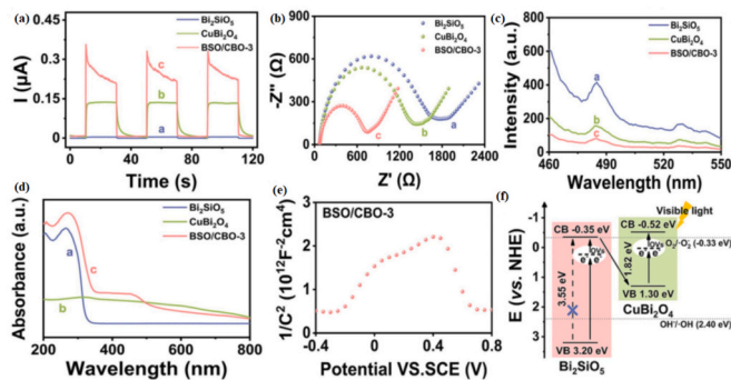
Fig. 7. (a) photocurrent response (b) Nyquist plot, (c) PL spectra (d) UV-vis Drs of Bi 2 SiO 5 , CuBi 2 O 4 and BSO/CBO, (e) Mott-Schottky and (f) charge transfer mechanism of BSO/CBO heterostructure. Adapted from Yu et al. [164]. Copyright © 2023 Elsevier.
