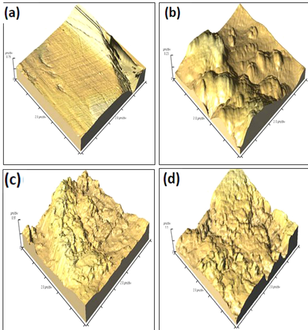
Figure 13. Atomic force micrograph of (a) plain MS surface, (b) MS in 0.5 M \text{H}_2\text{SO}_4 , (c) MS in 0.5 M \text{H}_2\text{SO}_4 + 1600 ppm PNVP-PU (d) MS in 0.5 M \text{H}_2\text{SO}_4 + 1600 ppm PDMAEMA-PU.
