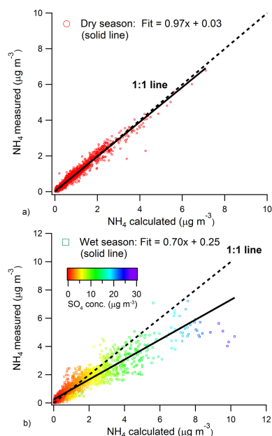
Fig. 5. Measured vs. calculated \text{NH}_4^+ and linear fittings (solid lines) using (a) Eq. (3) (dry season) and (b) Eq. (4) (wet season). Data points (b) are colour-coded according to \text{SO}_4^{2-} concentration.
