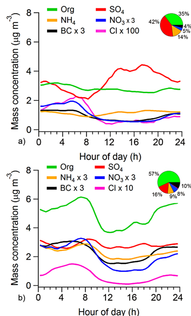
Fig. 4. Diurnal cycle of OA, \text{SO}_4^{2-} , \text{NH}_4^+ , \text{NO}_3^- and BC, in both the wet (a) and the dry (b) seasons. \text{NO}_3^- and BC concentrations were multiplied by 3 and \text{Cl}^- by 10/100 for scaling. Mean compositions are shown in the pie charts (percentages).
