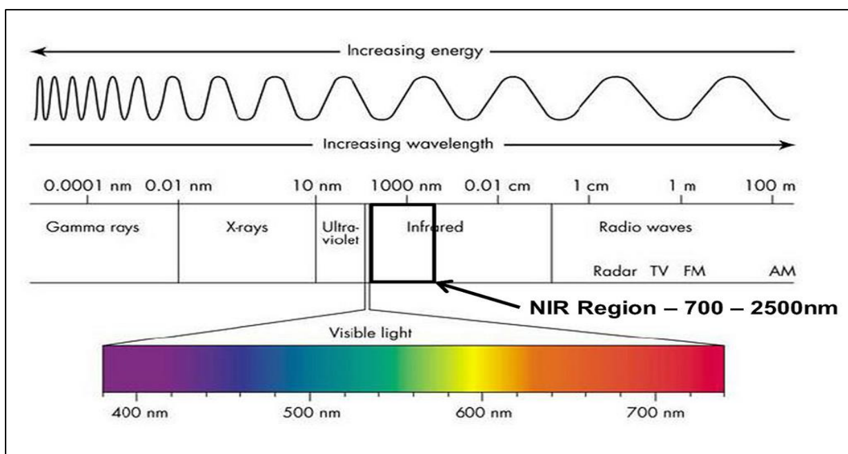
Figure 6: Where the NIR region is on the electromagnetic spectrum (kpm analytics, s.a.)
