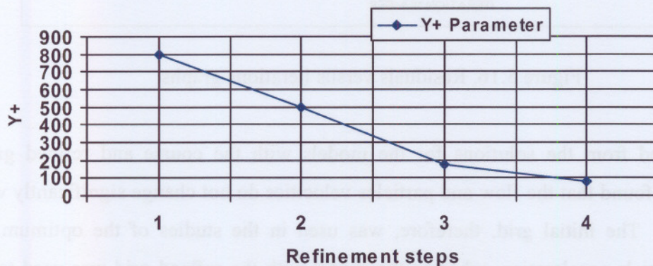
Figure 5.15. y^+ values obtained in the grid-refinement steps
