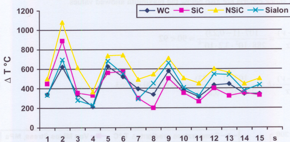
Figure 6.19. Temperature gradients of the nozzle materials in heating up
