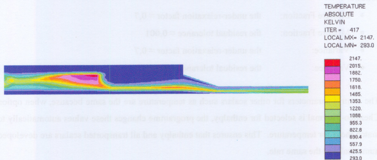
b) Temperature distribution with the RNG k - \varepsilon turbulence model
