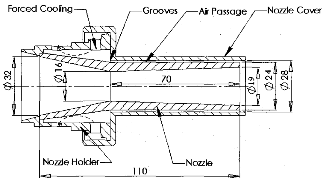
Figure B.2 Schematic section of the WC nozzle arrangement with forced cooling
