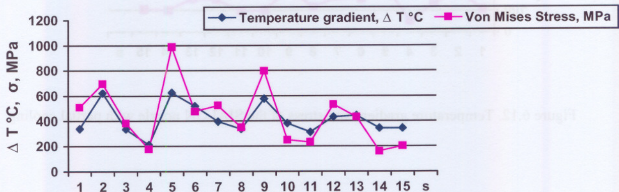
Figure 6.14. Temperature gradient and thermal stress of the WC nozzle in heating up
