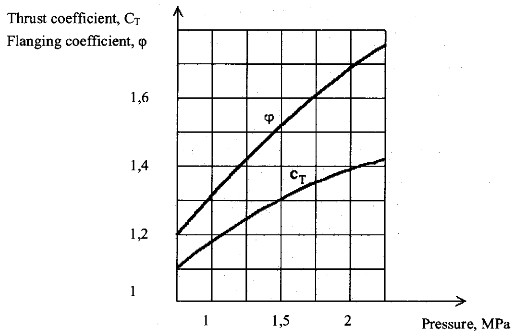
Figure 1.10. Thrust and flanging coefficients versus pressure, Glushko (1973)
