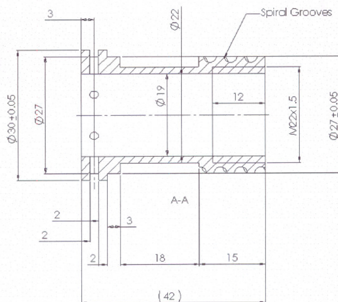
Figure E.5 Sectional view of the injector insert
