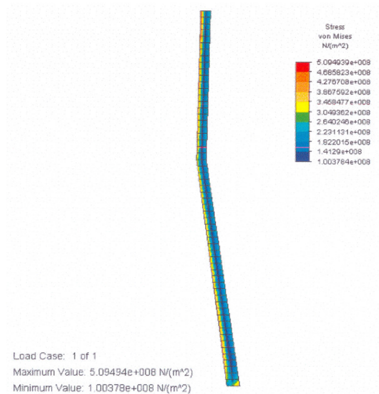
Figure D.76 Thermal stress distribution
