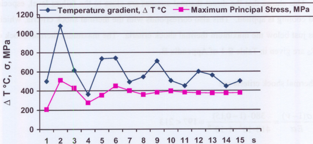
Figure 6.11. Temperature gradient and stress of the NSiC nozzle with forced cooling
