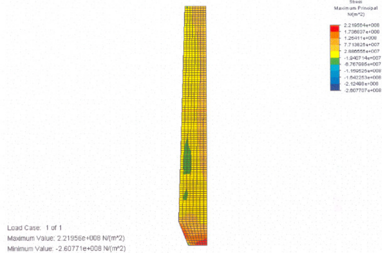
Figure D.33 Thermal stress distribution
