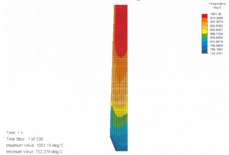
Figure D.38 Temperature distribution
