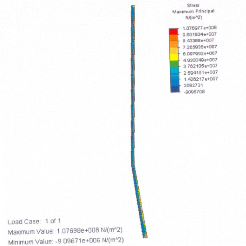
Figure D.51 Thermal stress distribution
