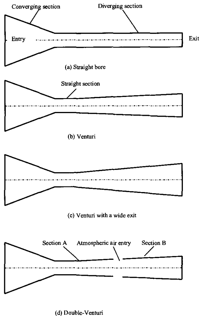
Figure 1.11. Abrasive blasting nozzle designs, (www.airblast.com)
