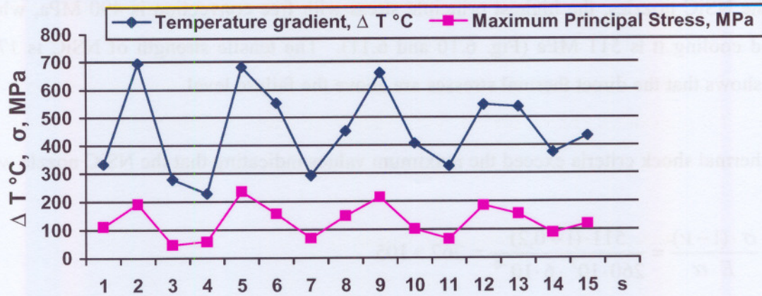
Figure 6.13. Temperature gradient and stress of the SIALON nozzle with forced cooling
