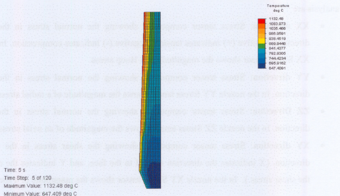
Figure 6.6. Temperature distribution in the SiC nozzle in heating up
