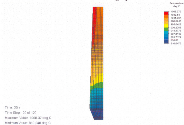
Figure D.7 Temperature distribution
