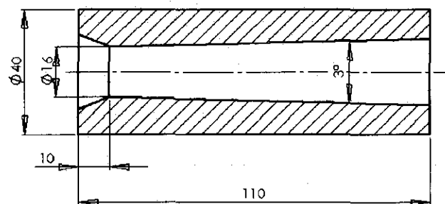
Figure 4.7. Section of the SiC nozzle
