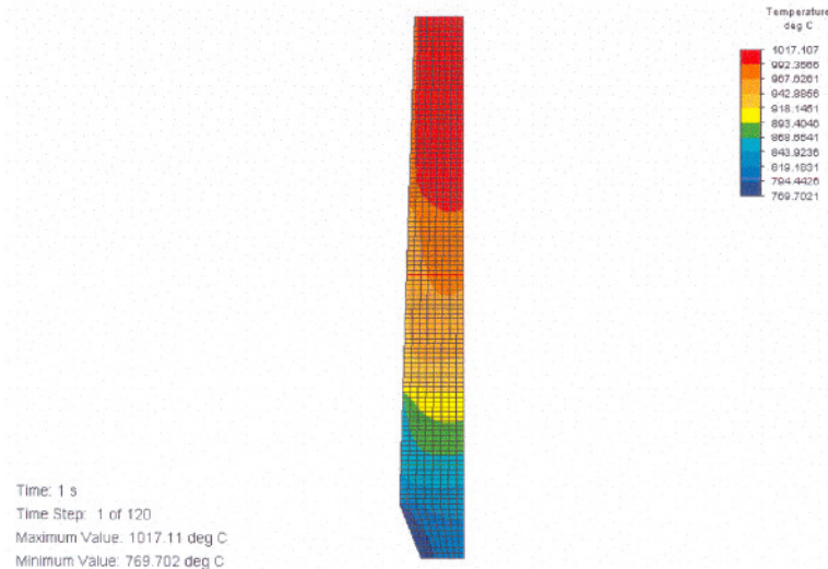
Figure D.13 Temperature distribution
