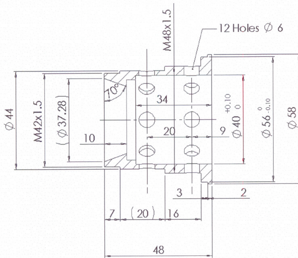
Figure E.6 Sectional view of the nozzle holder
