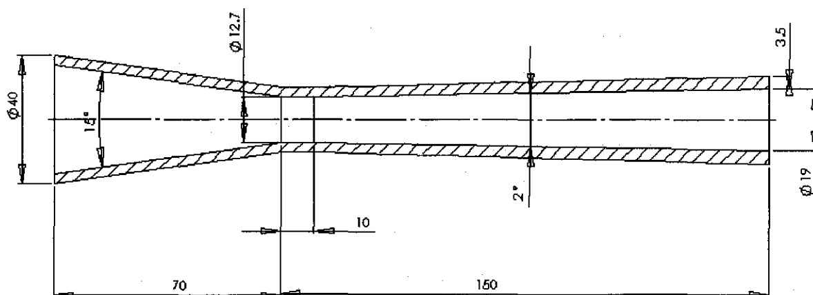
Figure 4.3. Diagram of the conventional abrasive blasting WC nozzle
