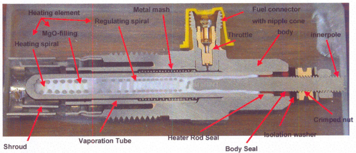
Figure E.11 Schematic section of the flame glow plug
