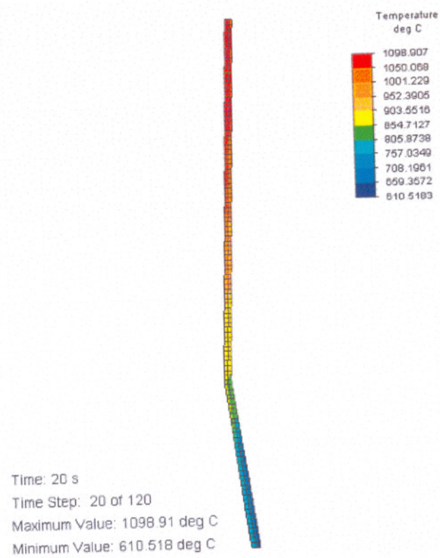
Figure D.55 Temperature distribution
