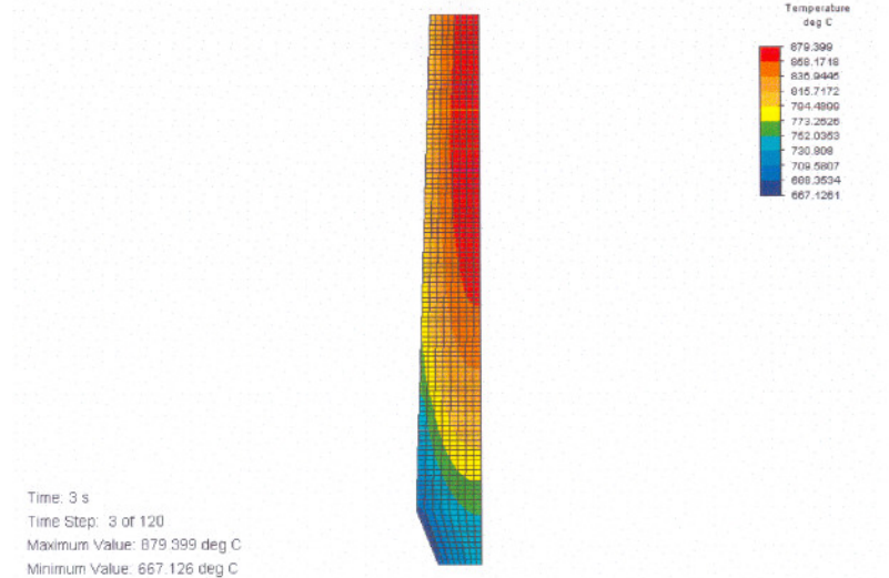
Figure D.19 Temperature distribution
