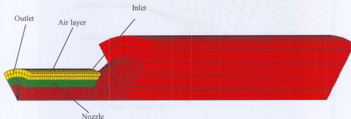
Figure 5.7. Meshed model of the gun with the nozzle and cooling cells
