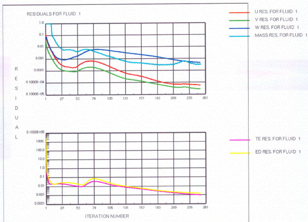
Figure C.24 Residual versus number of iterations for the second grid refinement
