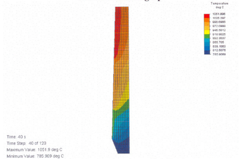
Figure D.34 Temperature distribution
