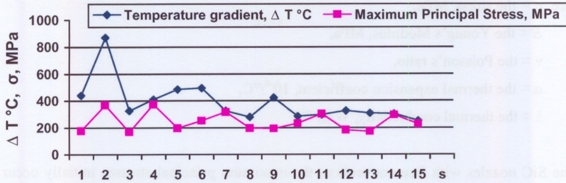
Figure 6.8. Temperature gradient and stress of the SiC nozzle with free convection
