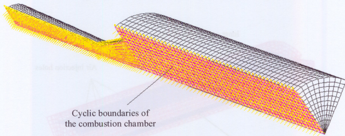
Figure 5.5. Cyclic boundaries of the of the thermo-abrasive gun model
