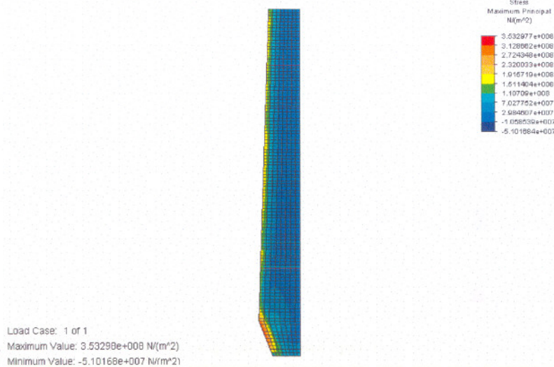
Figure D.45 Thermal stress distribution
