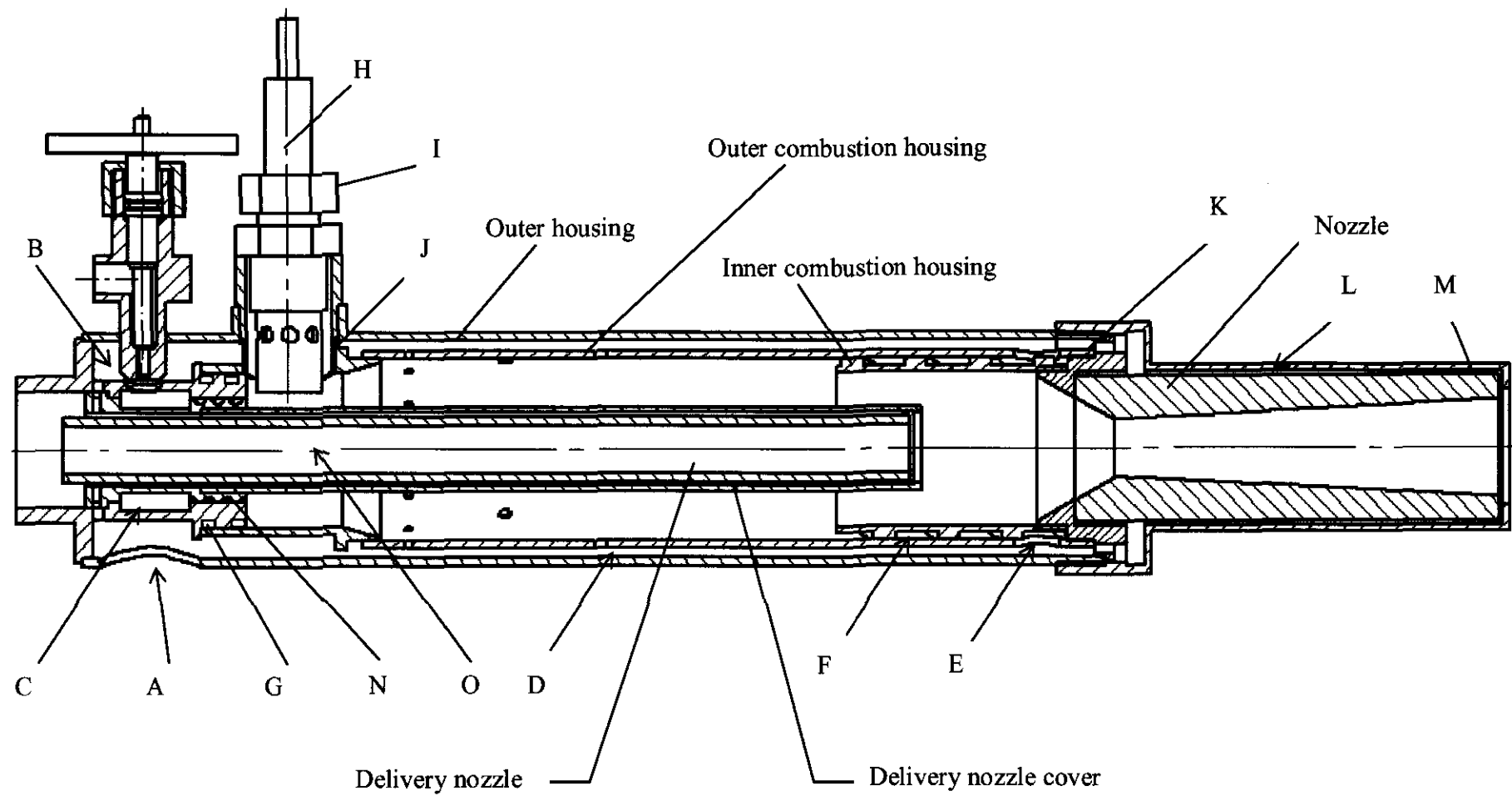
Figure 4.2. Schematic cross section of the advanced design of the thermal-gun
