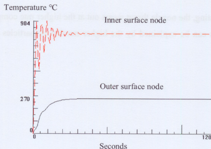
Figure 7.7. FEA temperature graph
