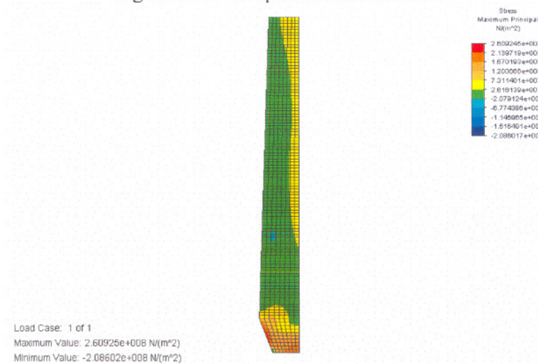
Figure D.37 Thermal stress distribution
