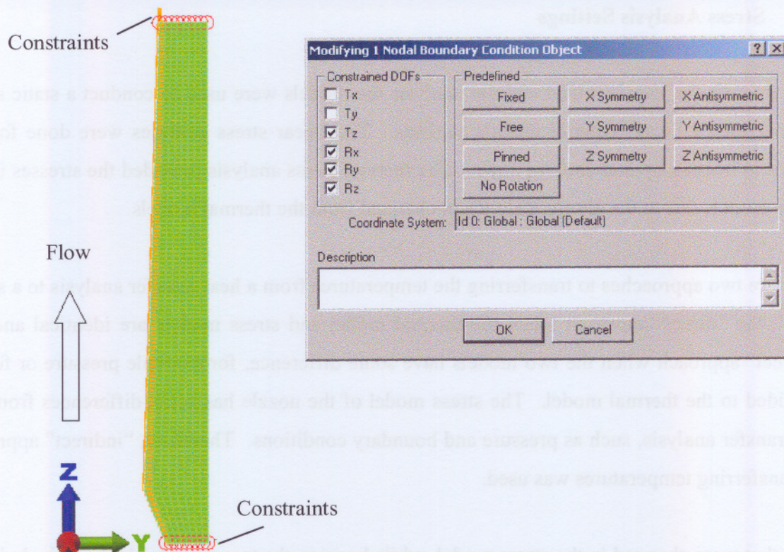
Figure 6.3. Constraints applied to the SiC nozzle
