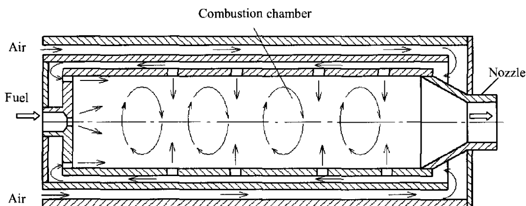
Figure 2. Simplified schematic of a ram jet engine
