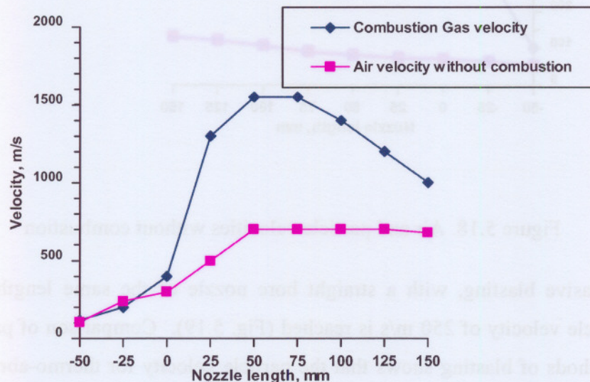
Figure 5.17. Gas and air velocities
