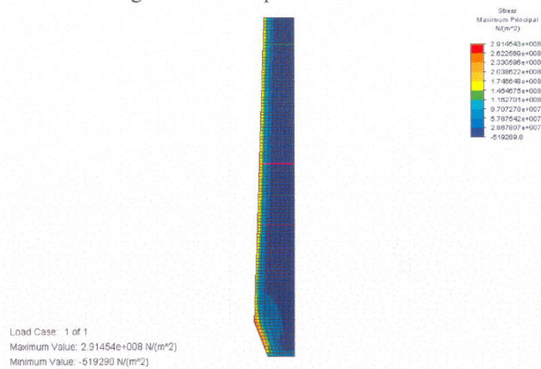
Figure D.49 Thermal stress distribution
