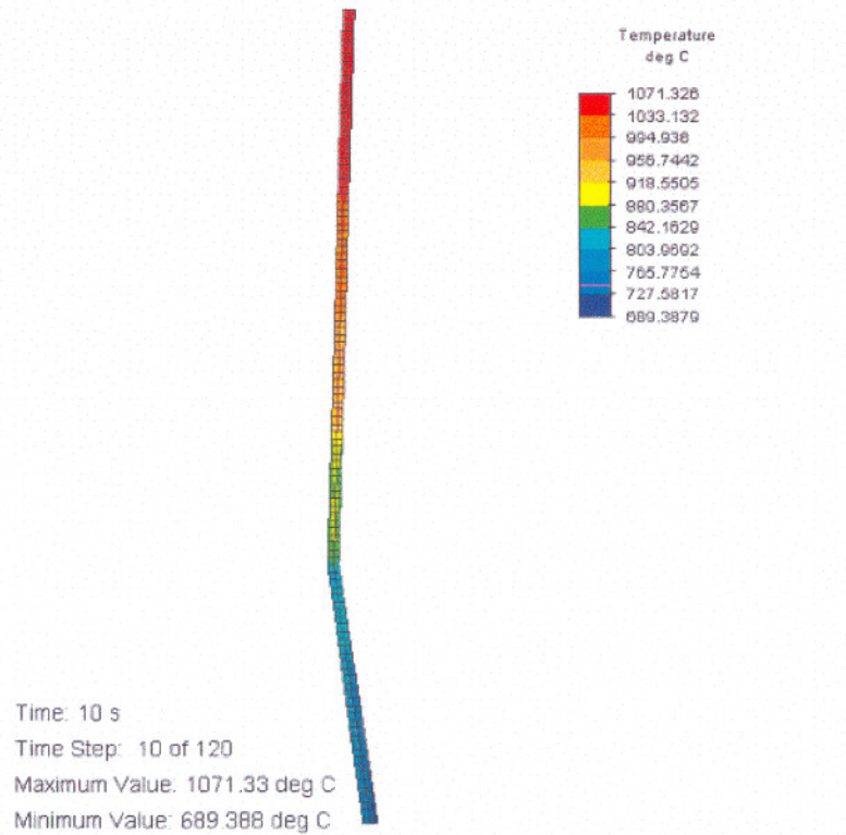
Figure D.79 Temperature distribution
