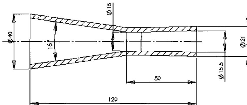
a) 70 mm WC nozzle
