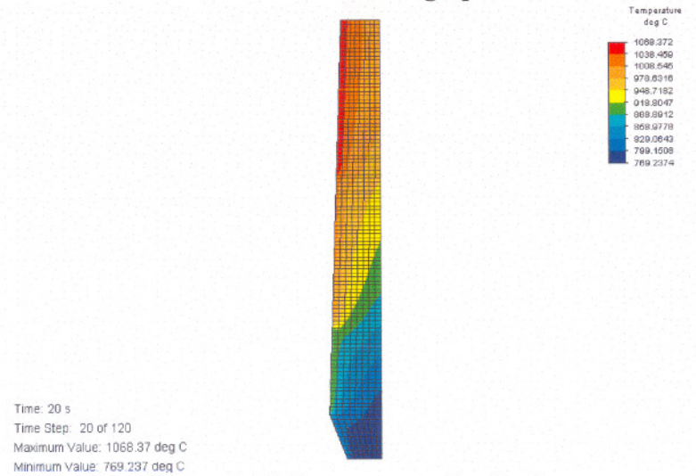
Figure D.32 Temperature distribution
