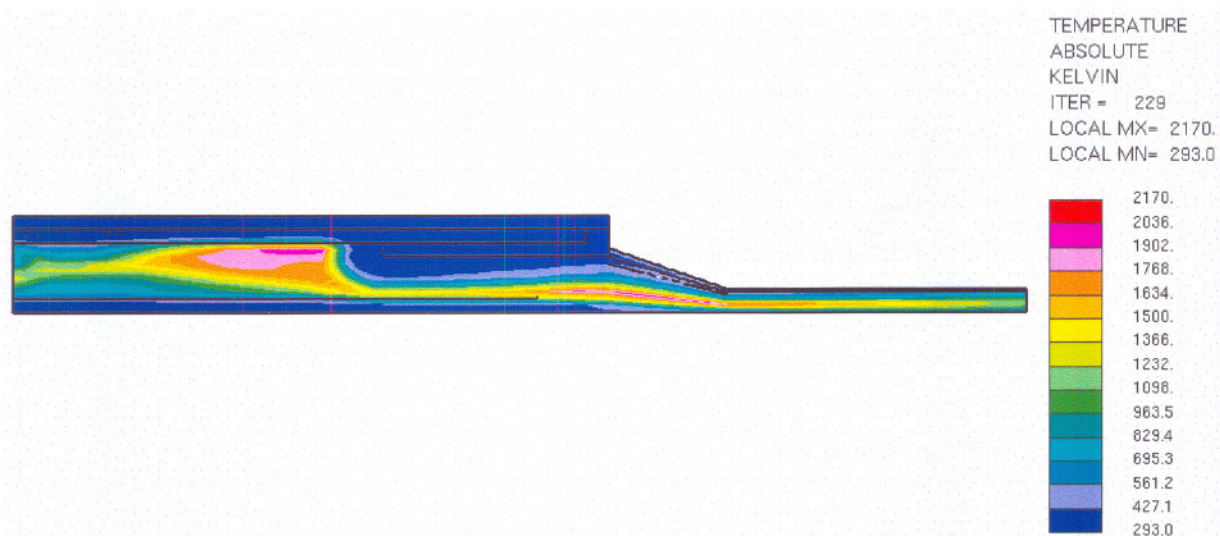
Figure C.26 Temperature distributions with the RNG turbulence model
