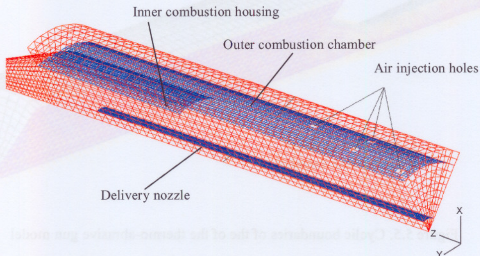
Figure 5.4. Baffle boundaries of the thermo-abrasive gun model
