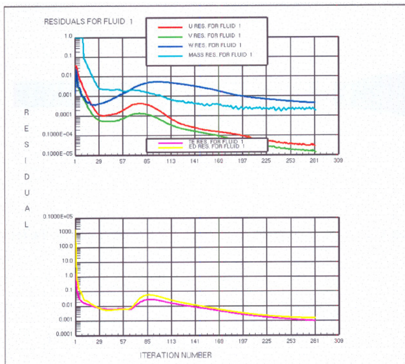
Figure C.24 Residual versus number of iterations for the second grid refinement
