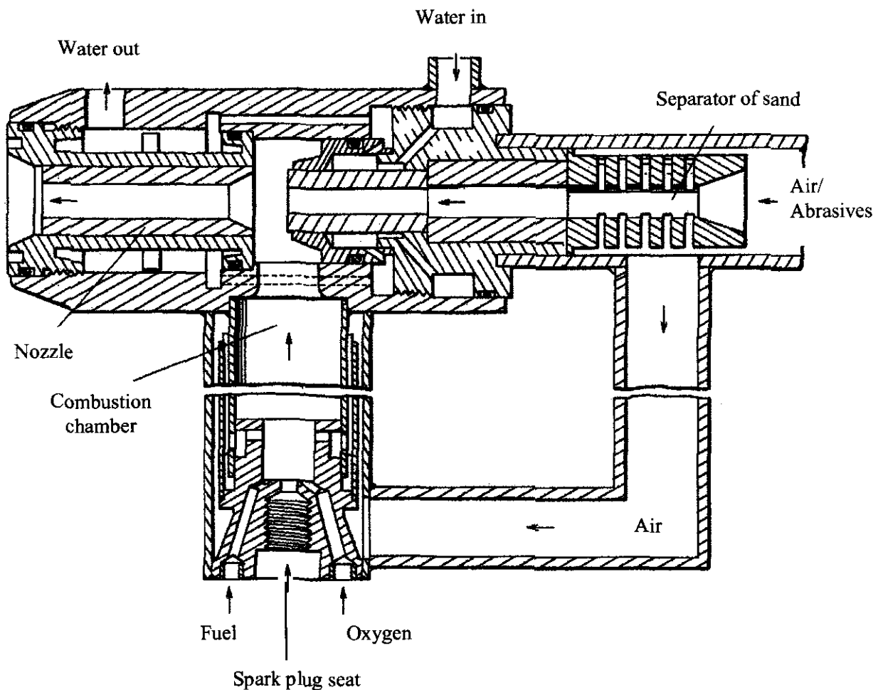
Figure 1.4. Schematic cross section of Browning's HVOF thermal gun, (1983)
