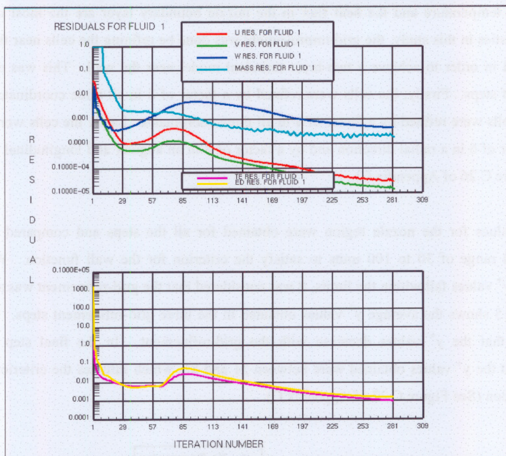
Figure 5.16. Residuals versus iterations graphs
