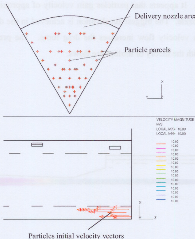
Figure 5.13. Particle parcels spacing inside the thermo-abrasive gun model
