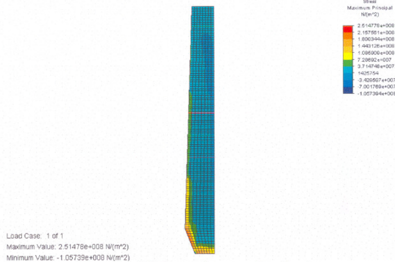
Figure D.18 Thermal stress distribution
