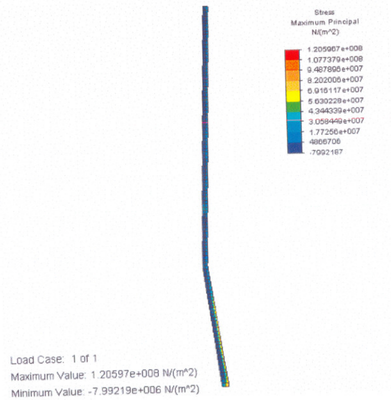
Figure D.58 Thermal stress distribution
