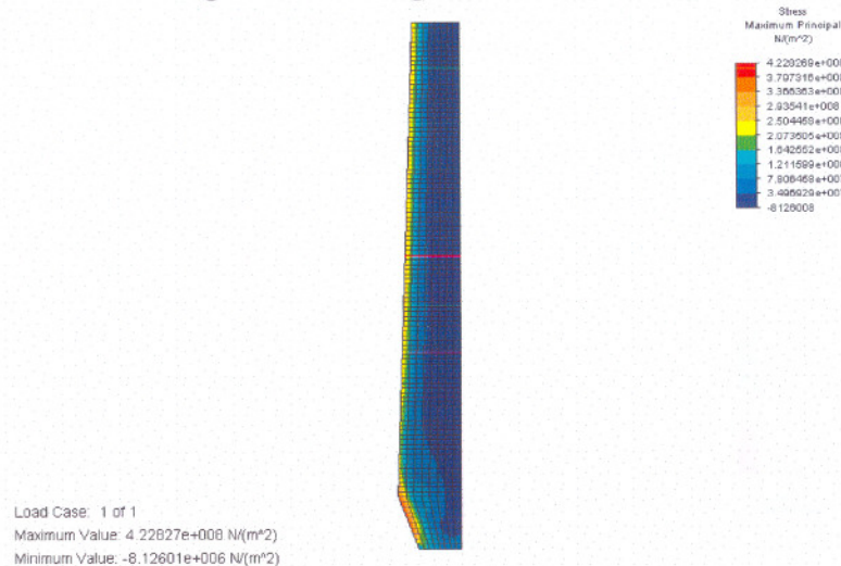
Figure D.43 Thermal stress distribution
