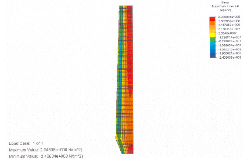
Figure D.27 Thermal stress distribution
