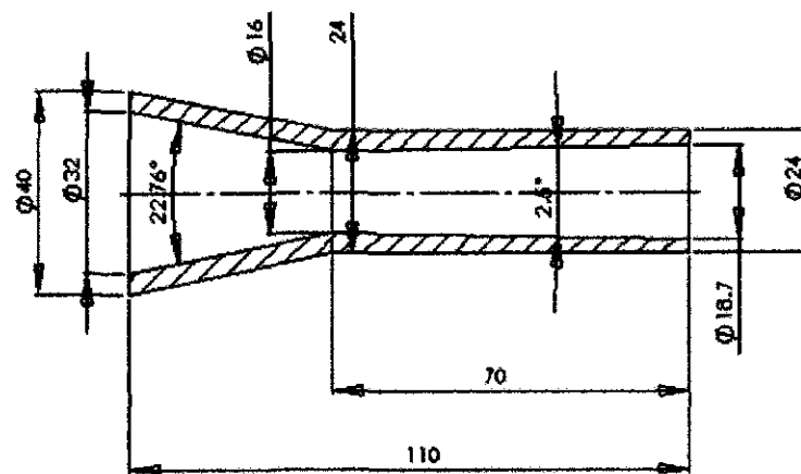
a) 16 mm bore size
