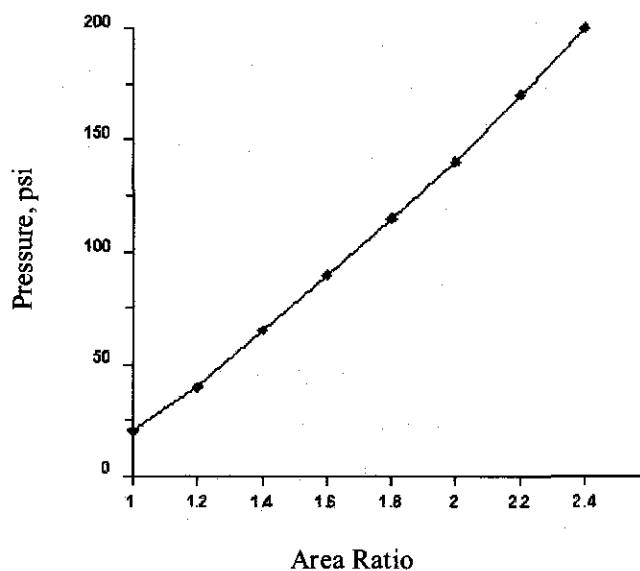
Figure 1.9. Nozzle pressure versus nozzle area ratio, Settles and Garg (1995)
