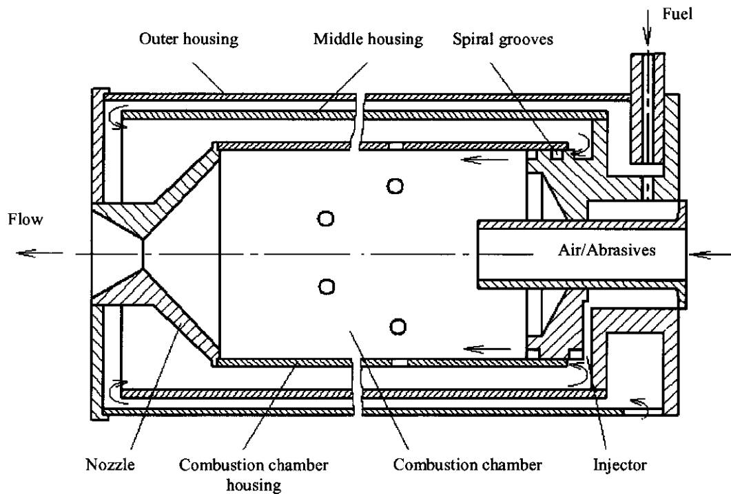
Figure 1.5. Schematic cross section of Galchenko's HVAF thermal gun, (1982)
