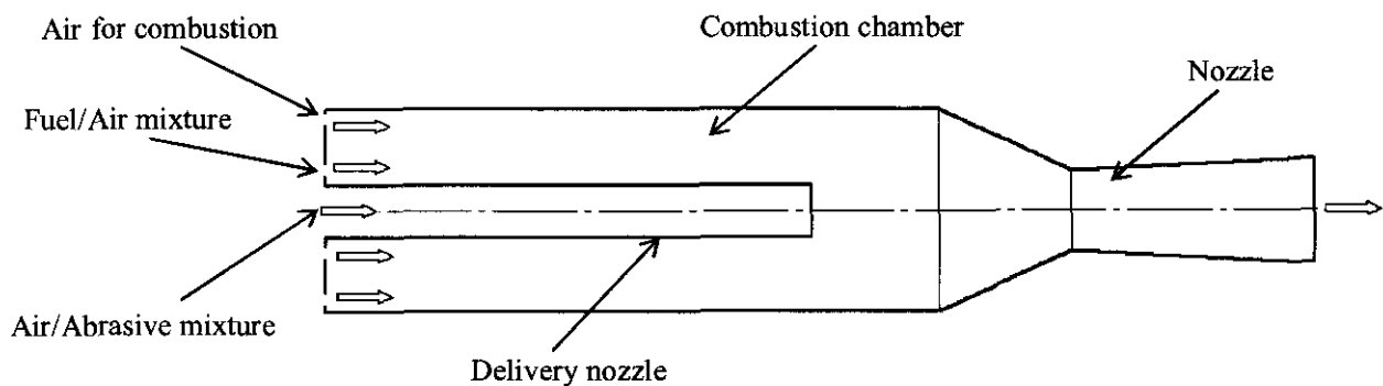
Figure 3.3. Diagram of the HVAF system
