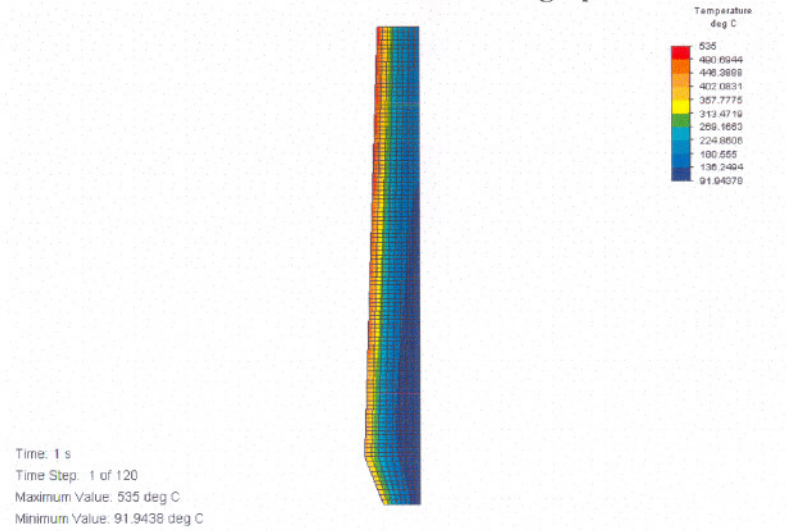
Figure D.1 Temperature distribution
