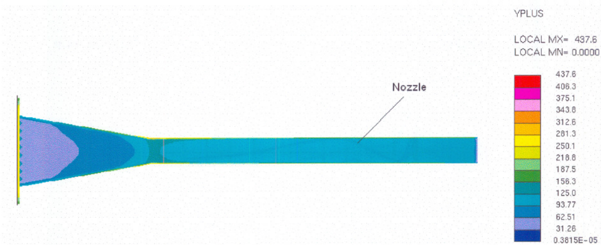
Figure C.27 y^+ parameter for the cells attached to the nozzle of the refined model
