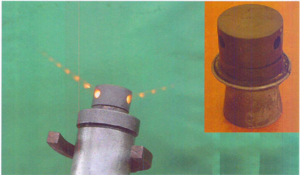
Figure B.9 Angle WC nozzle
