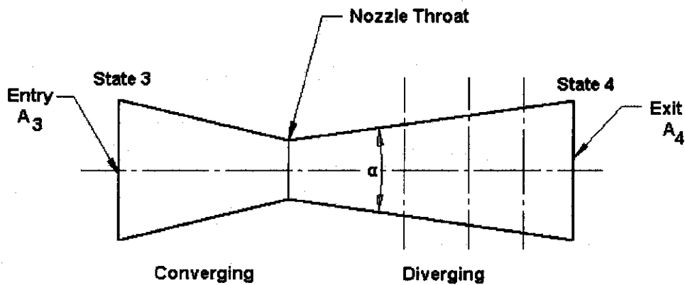
Figure A.1 Diagram of the simplified Laval nozzle
