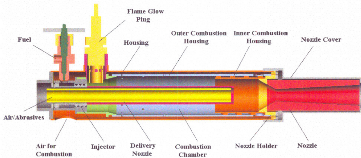
Figure E.3 Schematic section of the new thermo-abrasive gun
