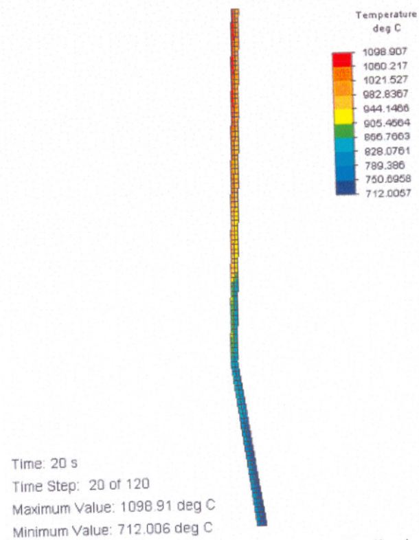
Figure D.81 Temperature distribution
