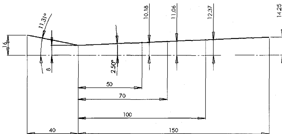
Figure A.2 Calculated optimum bore geometry of a thermo jet nozzle
