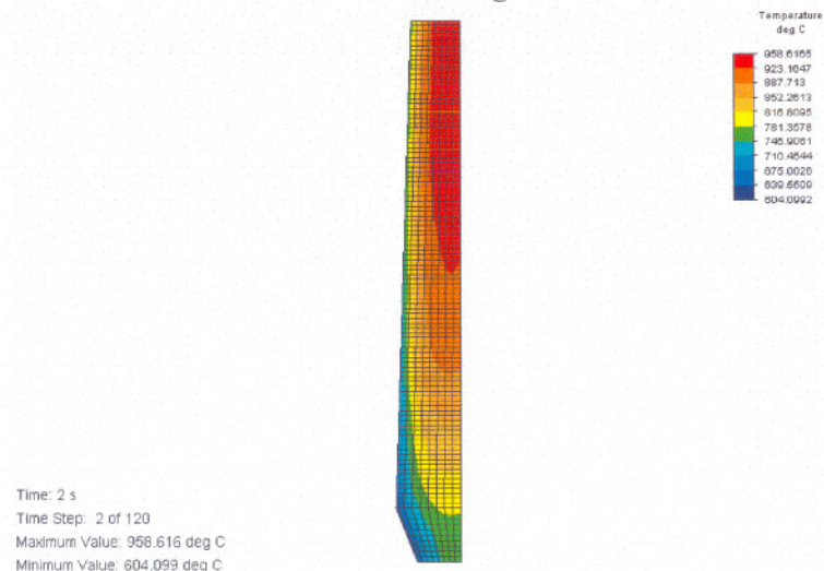
Figure D.40 Temperature distribution
