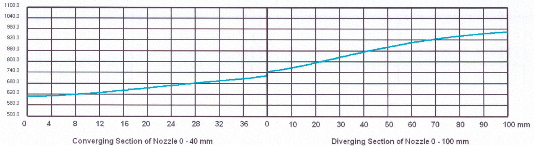
Figure C.20 Temperature distribution in the inner surface of the nozzle for the low fuel/air ratio (RNG turbulence model)
