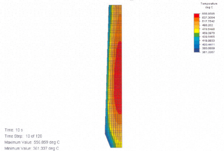
Figure D.48 Temperature distribution
