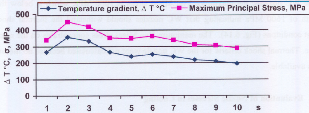
Figure 6.16. Temperature gradient and stress of the NSiC nozzle in cooling
