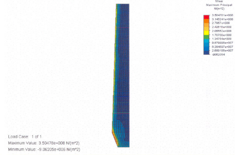
Figure D.47 Thermal stress distribution
