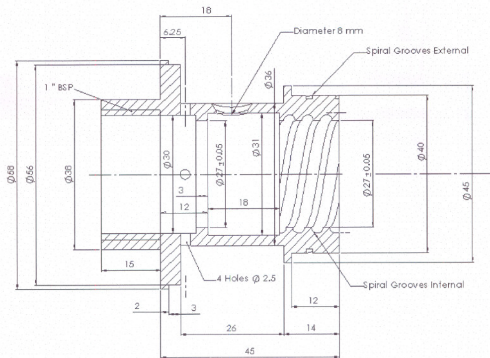
Figure E.4 Sectional view of the injector
