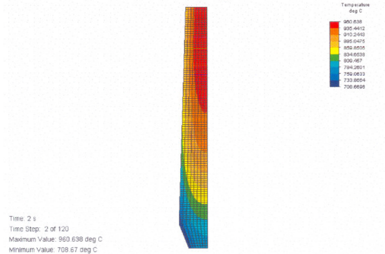
Figure D.17 Temperature distribution
