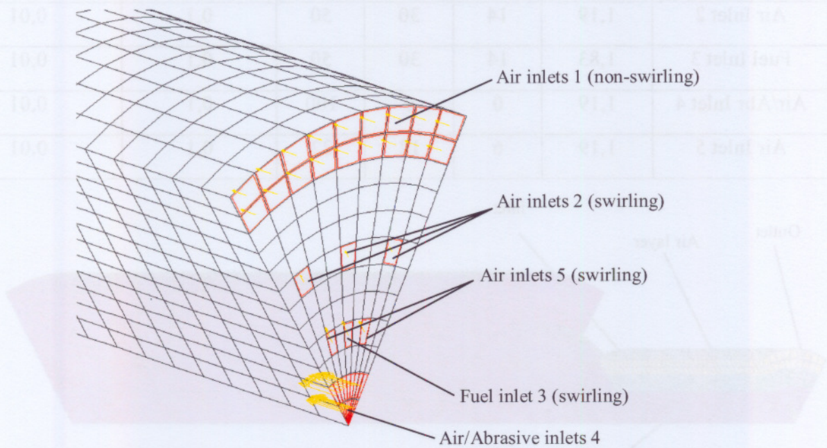
Figure 5.6. Inlet sets of the thermo-abrasive gun model
