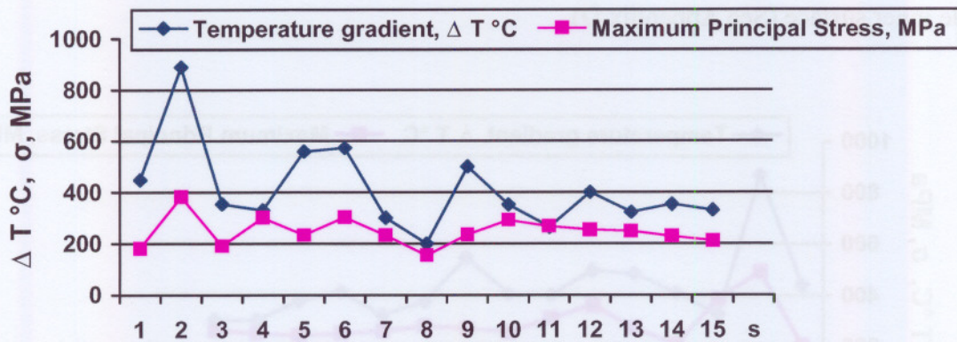
Figure 6.9. Temperature gradient and stress of the SiC nozzle with forced cooling
