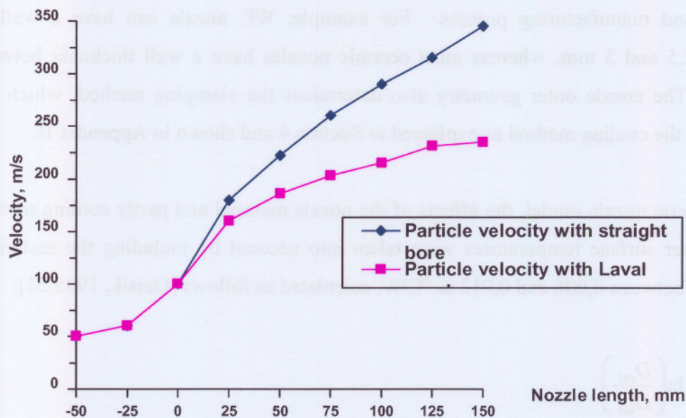
Figure 5.20. Particle velocities with and without combustion with a straight bore nozzle
