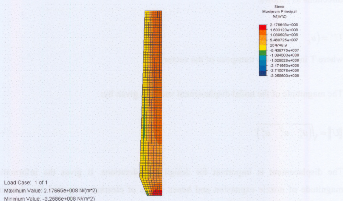
Figure 6.7. Stress distribution in the SiC nozzle in heating up
