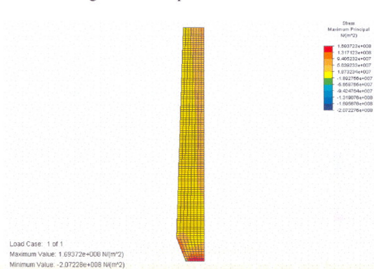
Figure D.8 Thermal stress distribution
