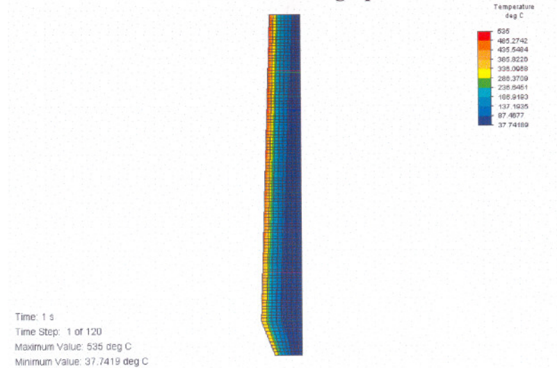
Figure D.26 Temperature distribution
