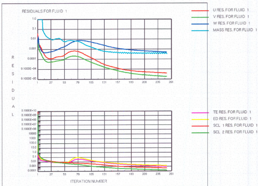
Figure C.22 Residual versus number of iterations for the initial cell grid
