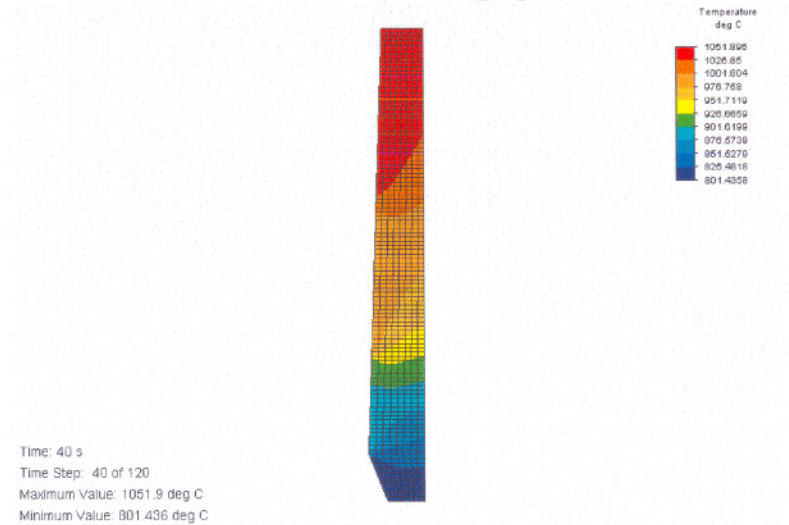
Figure D.9 Temperature distribution
