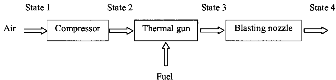
Figure 3.2. Elements and stages of a thermal gun system
