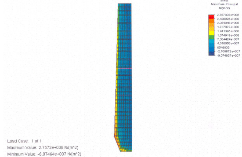
Figure D.20 Thermal stress distribution
