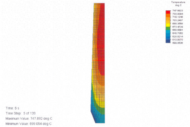
Figure D.22 Temperature distribution
