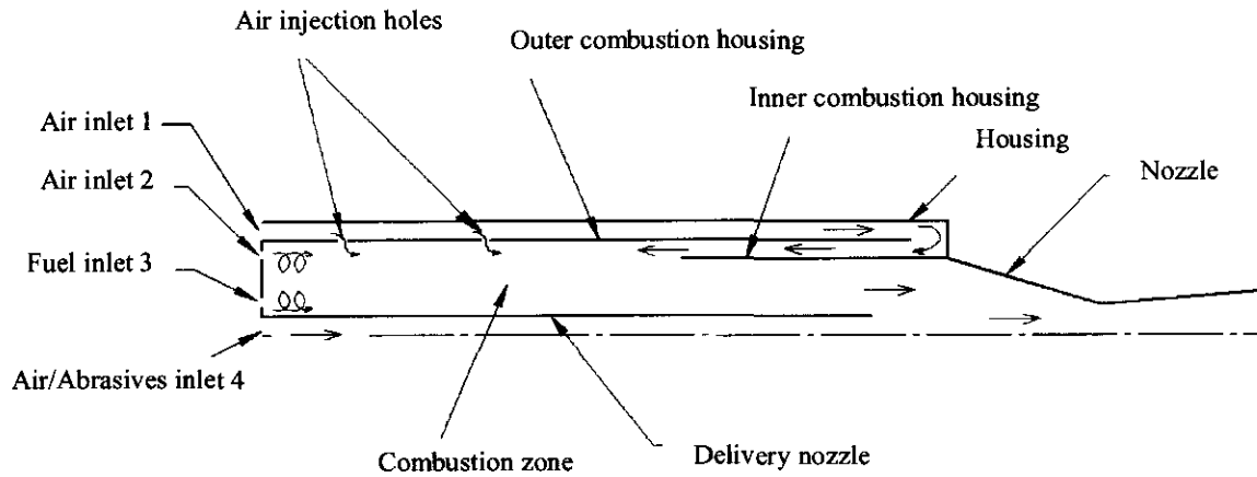
Figure 5.1. Schematic of a half cross section of the model
