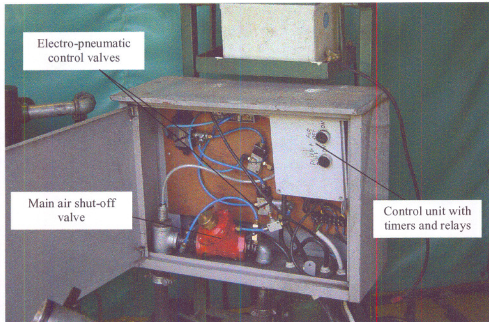
Figure E.8 Control unit of the thermo-abrasive system
