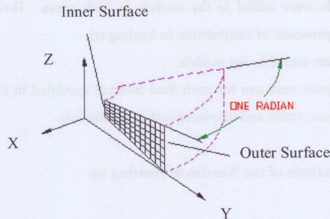
Figure 6.1. Axisymmetric element model
