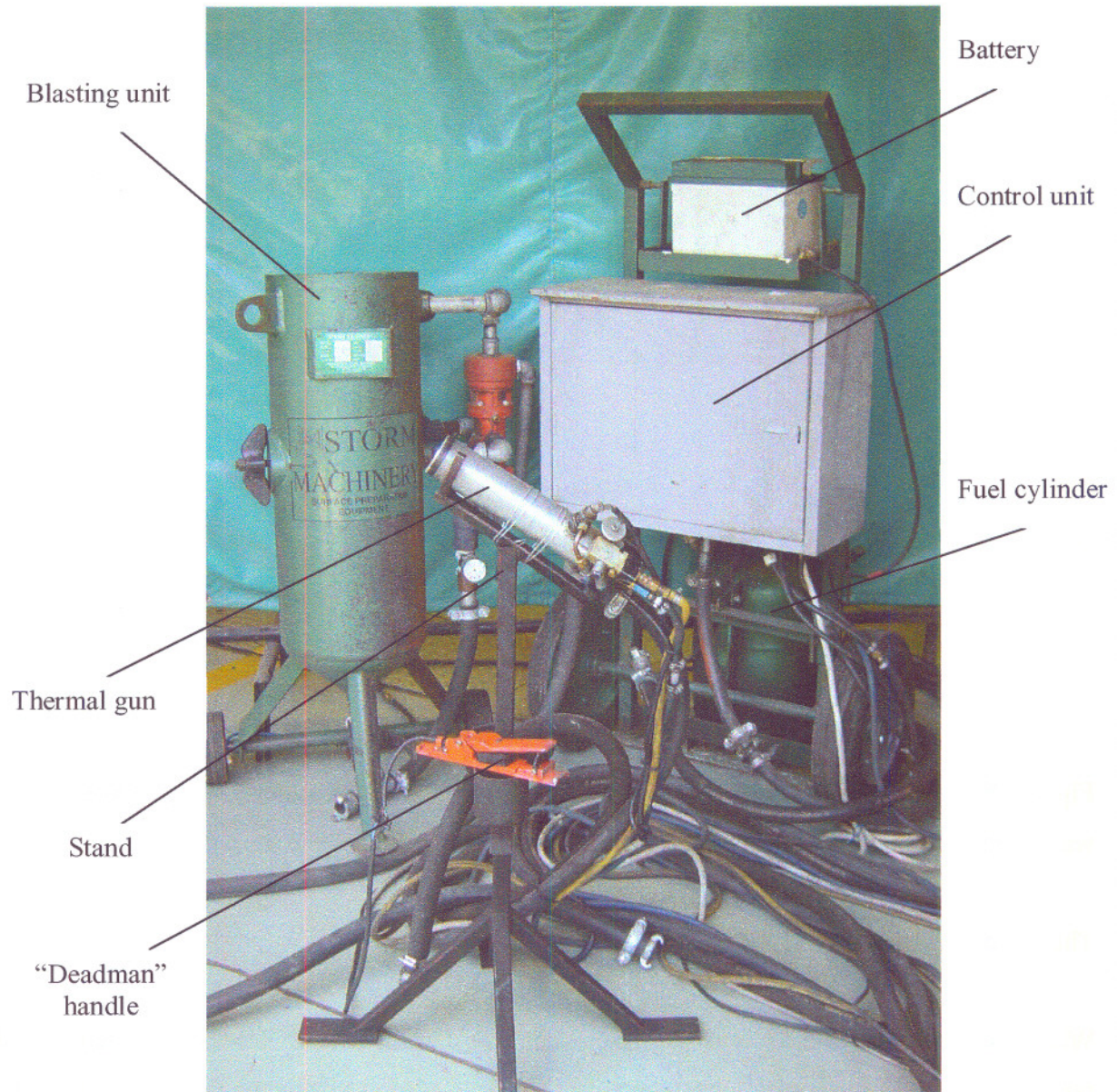
Figure E.7 New design of the thermo-abrasive system
