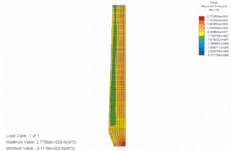
Figure D.31 Thermal stress distribution
