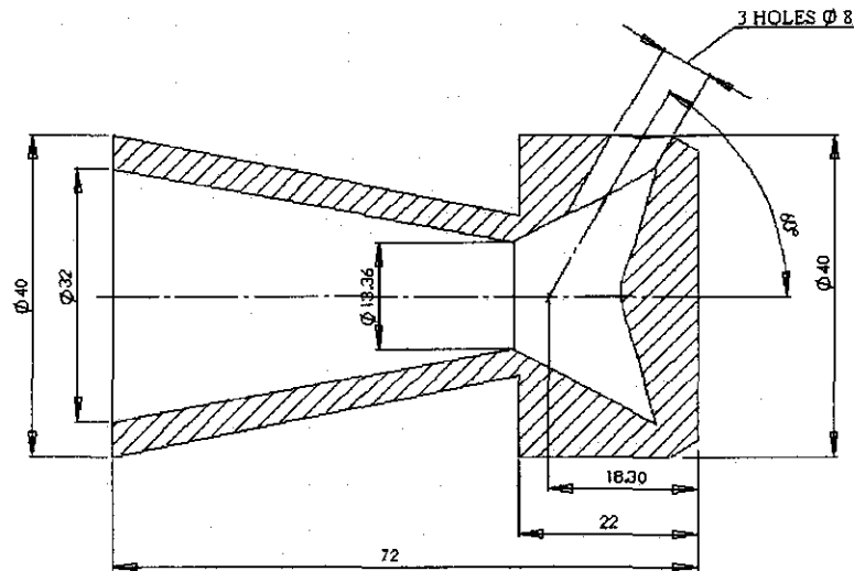
Figure 4.6. Section of the WC nozzle for blasting inside pipes
