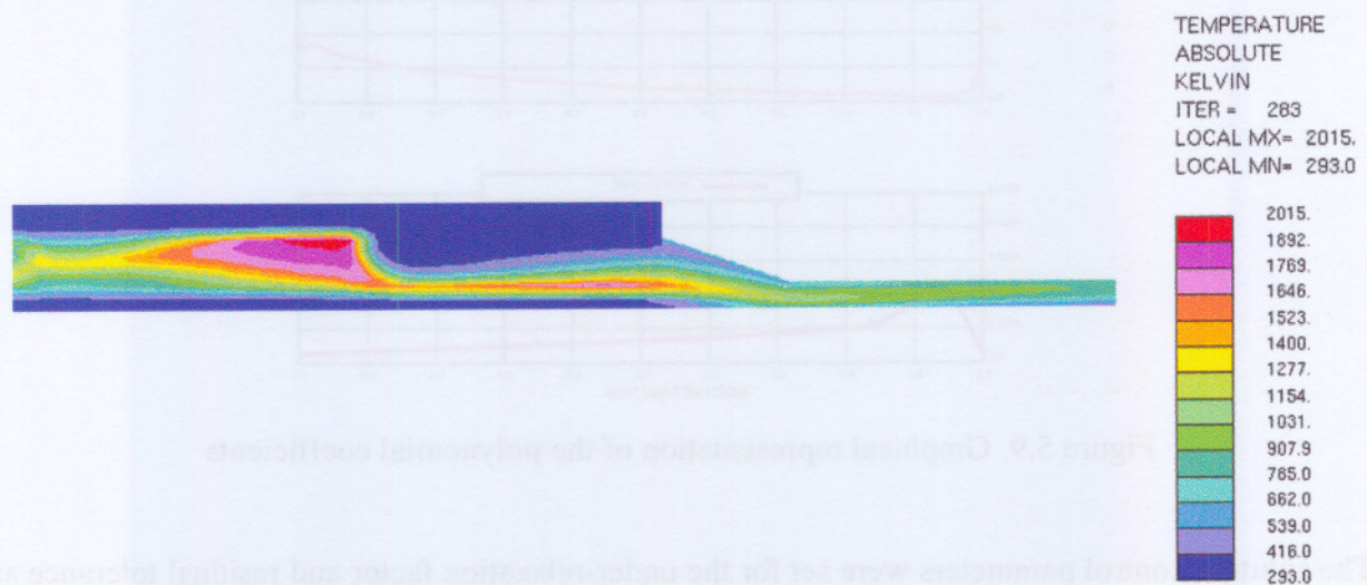
a) Temperature distribution with the k - \varepsilon turbulence model
