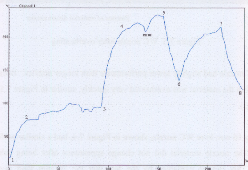
Figure 7.6. Recorded nozzle outer surface temperatures
