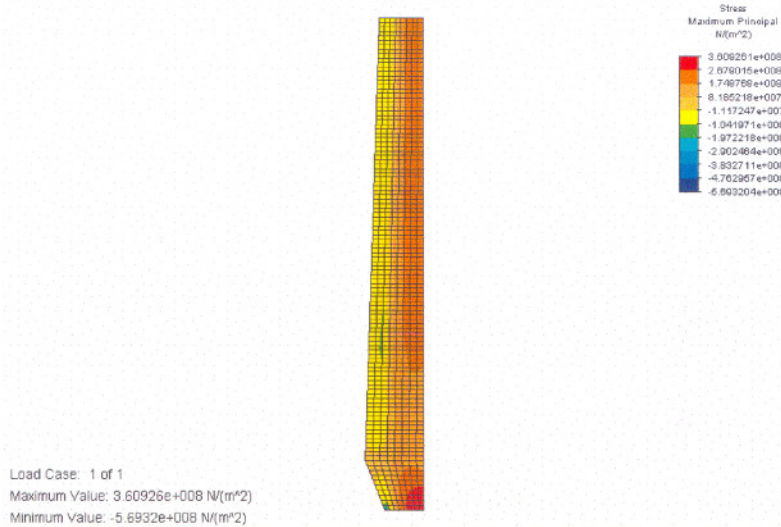
Figure D.29 Thermal stress distribution
