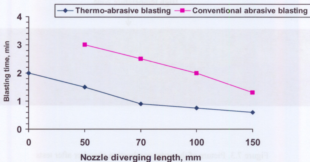
Figure 7.2. Blasting time to clean 1 \text{ m}^2 of steel surface with different nozzles
