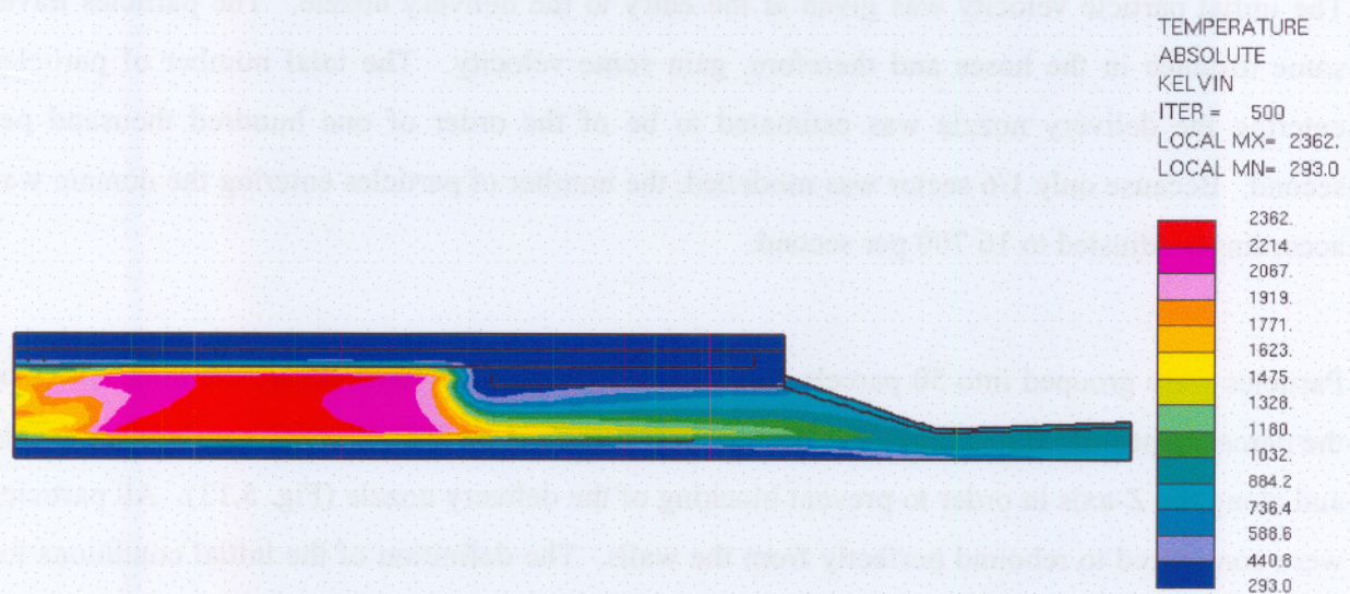
Figure 5.12. Temperature distributions of the three-stage combustion of C 3 H 8
