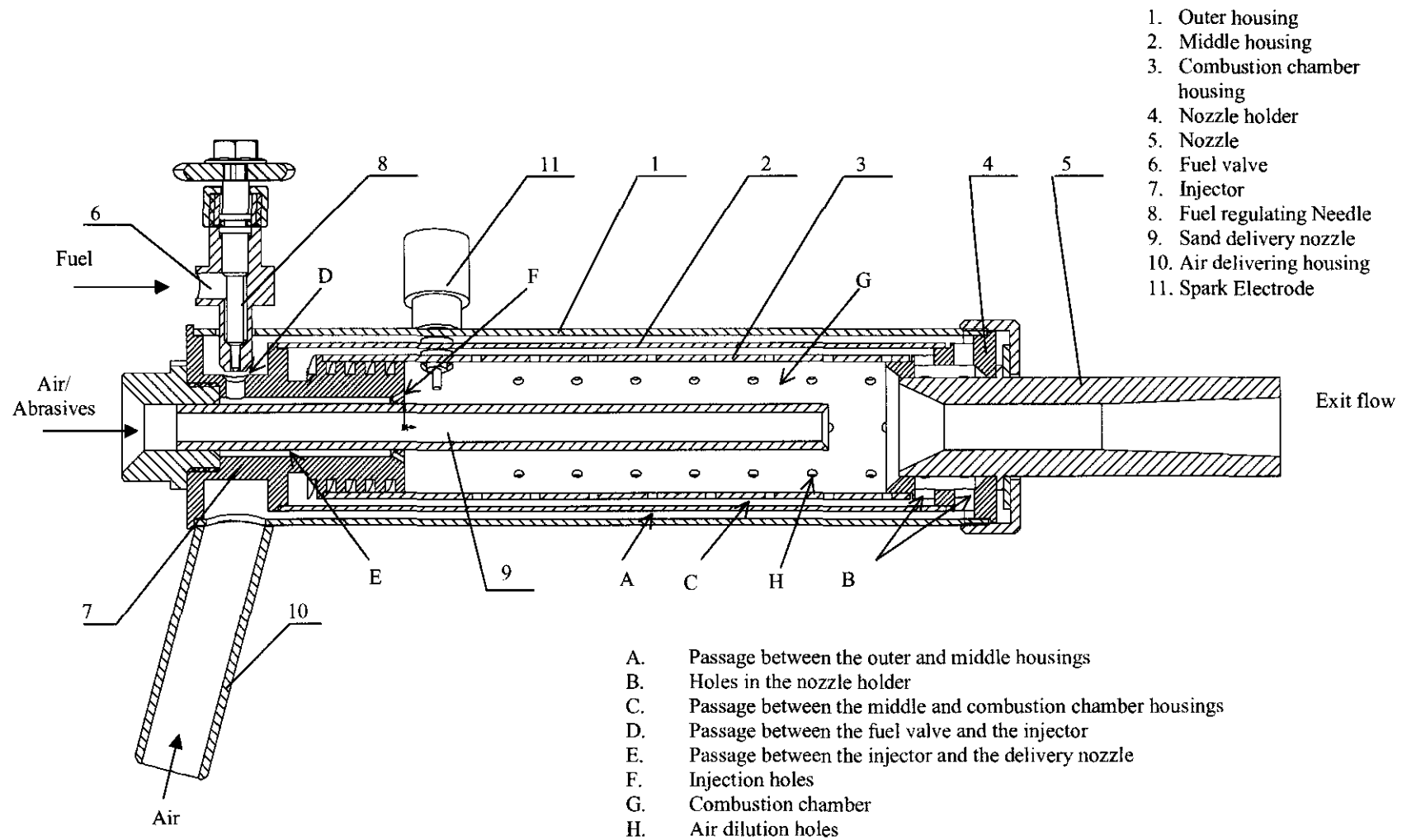
Figure 3. Schematic cross section of the prototype of the thermal-gun
