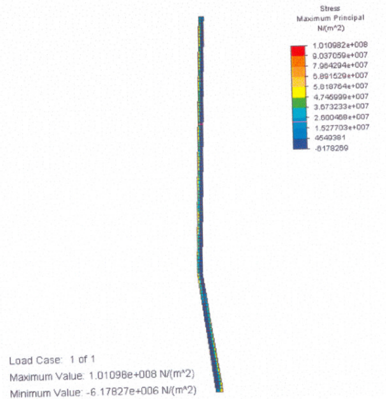
Figure D.54 Thermal stress distribution
