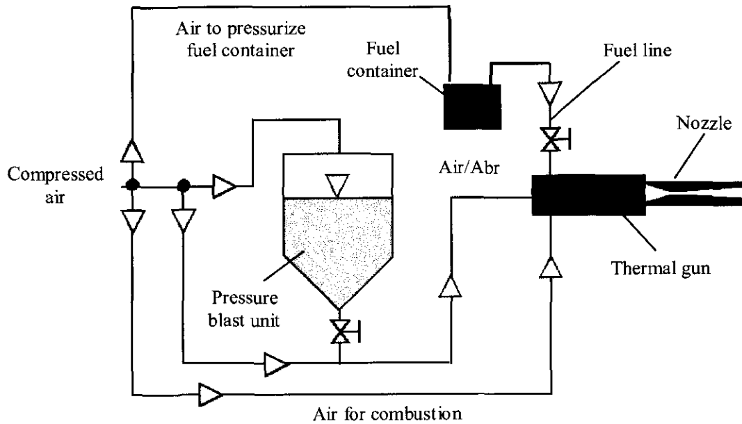
Figure 4. Schematic of the thermo-jet system for abrasive blasting
