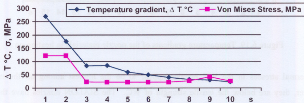
Figure 6.18. Temperature gradient and stress of the WC nozzle in cooling
