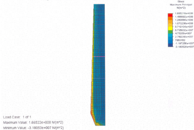
Figure D.25 Thermal stress distribution
