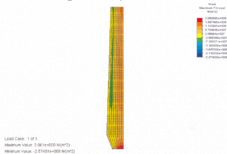
D.6 Thermal stress distribution
