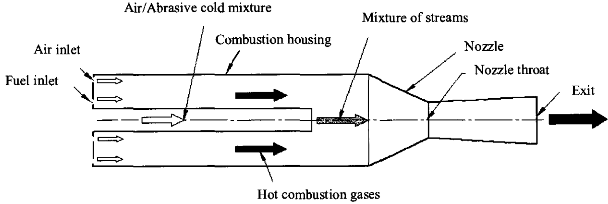
Figure 3.4. Diagram of the mixing of the streams
