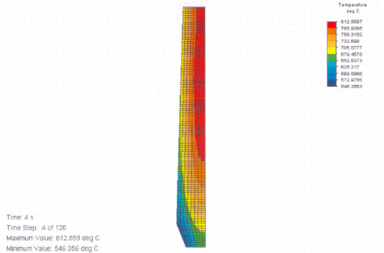
Figure D.44 Temperature distribution
