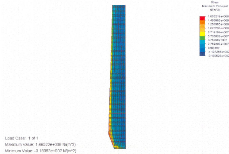
Figure D.23 Thermal stress distribution
