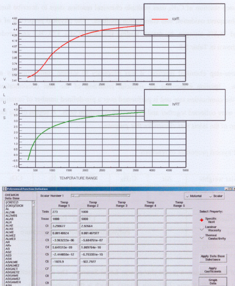
Figure 5.11. Graphical and tabular representations of polynomial coefficients for specific scalars for three-step chemical reaction
