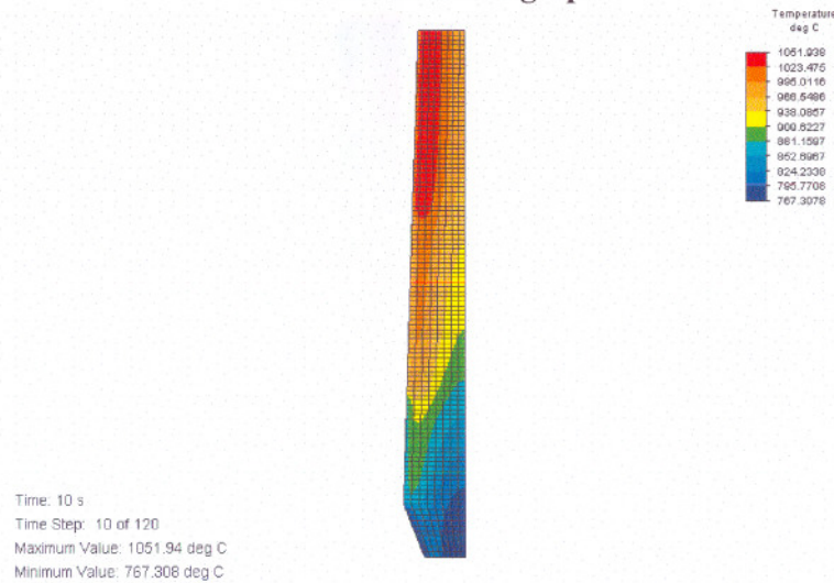
Figure D.5 Temperature distribution
