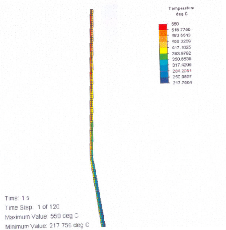
Figure D.50 Temperature distribution
