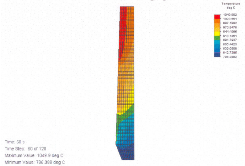
Figure D.36 Temperature distribution
