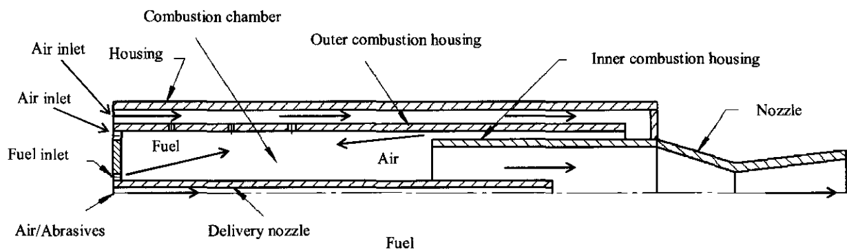
Figure 4.1. Sectional diagram of the improved design of the thermal gun
