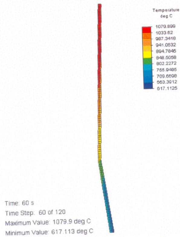
Figure D.59 Temperature distribution
