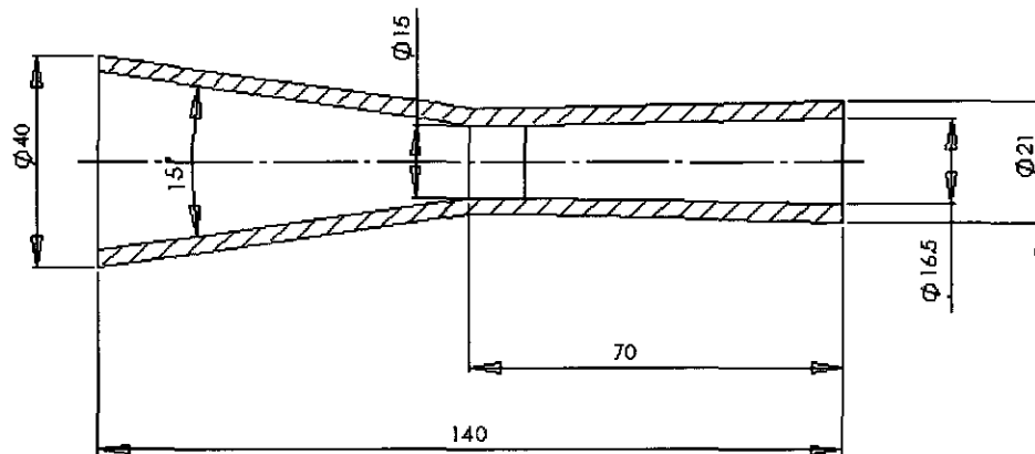
a) 70 mm WC nozzle
