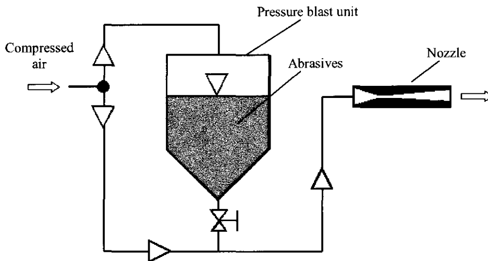
Figure 1. Schematic of a conventional abrasive blasting system
