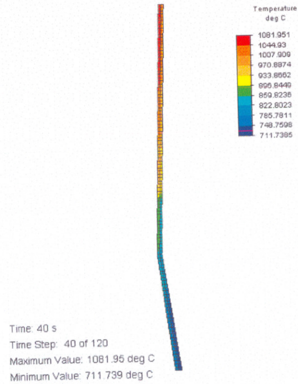
Figure D.83 Temperature distribution
