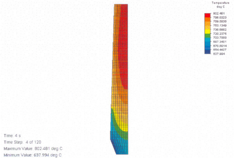
Figure D.21 Temperature distribution
