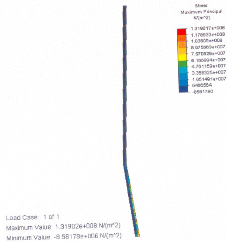
Figure D.56 Thermal stress distribution
