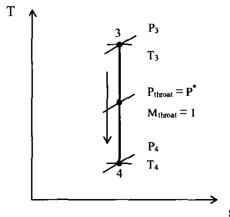
Figure 3.5. T - s diagram of expansion in the nozzle, Moran (1998)
