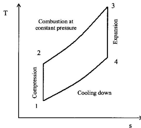
Figure 3.1. T-s diagram of an air-standard ideal Brayton cycle
