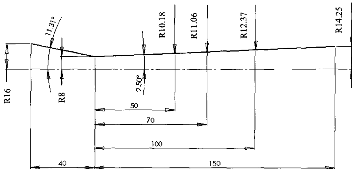
Figure 3.7. Calculated optimum bore geometry of a thermo jet nozzle
