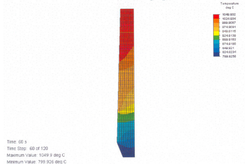
Figure D.11 Temperature distribution
