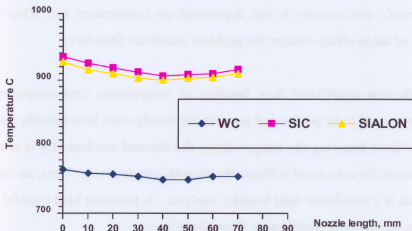
Figure 5.24. Temperature of the nozzle inner surface with forced cooling
