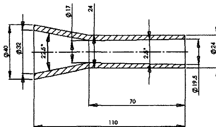
a) 17 mm bore size
