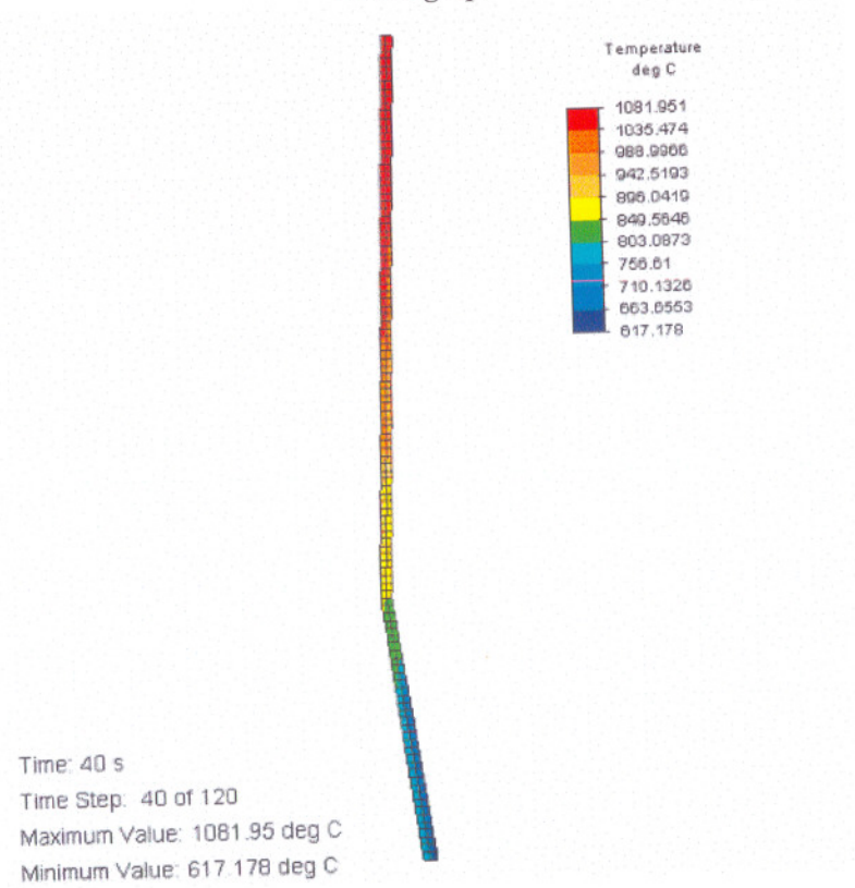
Figure D.57 Temperature distribution
