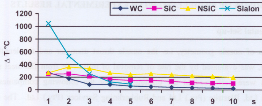
Figure 6.21. Temperature gradients of the nozzle materials in cooling
