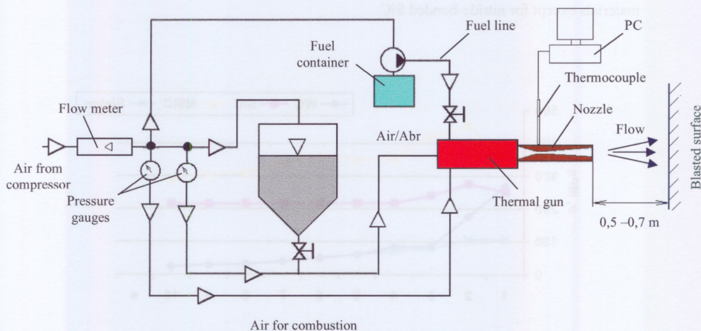
Figure 7.1. Experimental set-up
