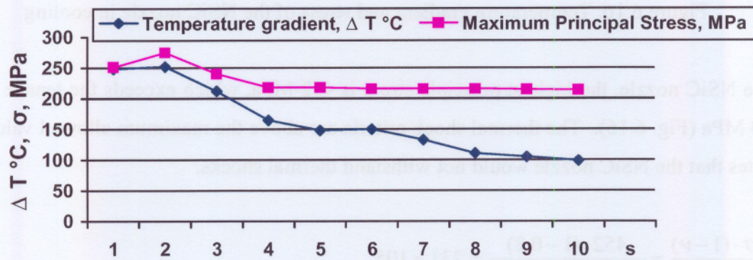
Figure 6.15. Temperature gradient and stress of the SiC nozzle in cooling
