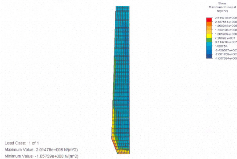
Figure D.14 Thermal stress distribution
