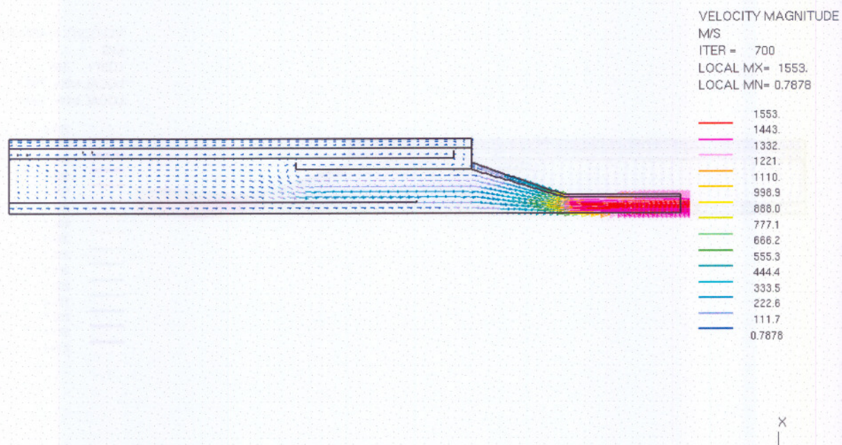
Figure C.3 Gas velocity with the 50 mm straight nozzle
