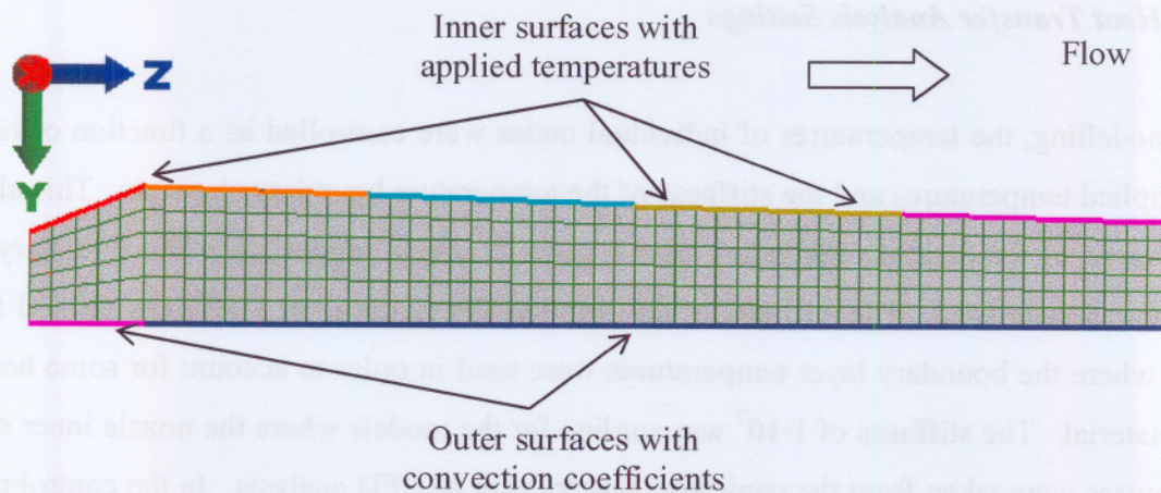
Figure 6.2. FEA Model of the SiC nozzle
