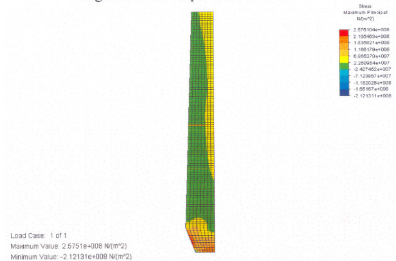
Figure D.35 Thermal stress distribution
