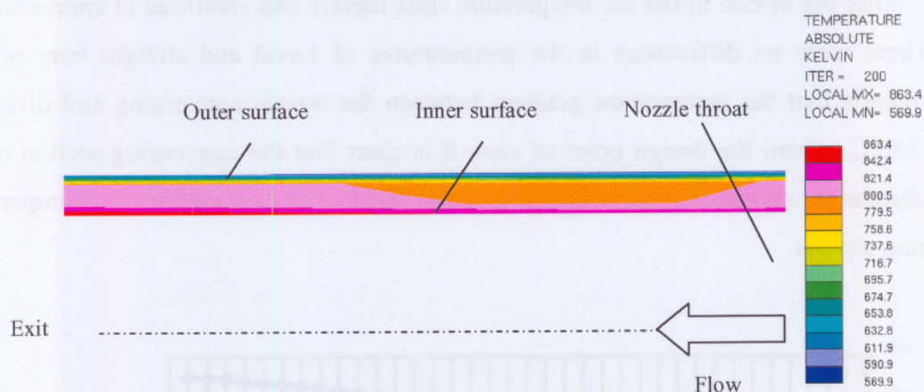
Figure 5.23. Temperature distribution in the WC nozzle with forced cooling
