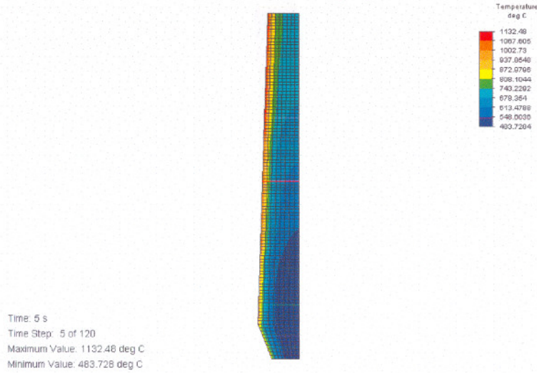
Figure D.28 Temperature distribution
