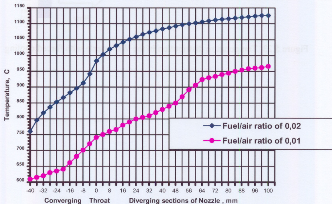
Figure 5.22. Temperature distribution in the boundary layer of a 100 mm nozzle
