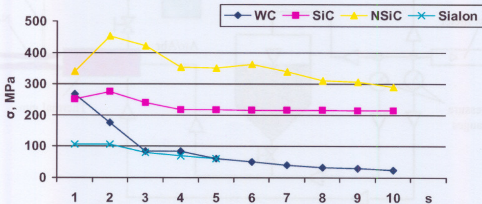
Figure 6.22. Thermal Stresses in the nozzle materials in cooling
