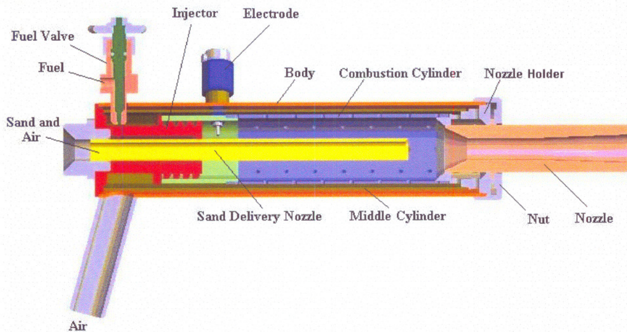
Figure E.2 Schematic section of the initial thermo-abrasive gun
