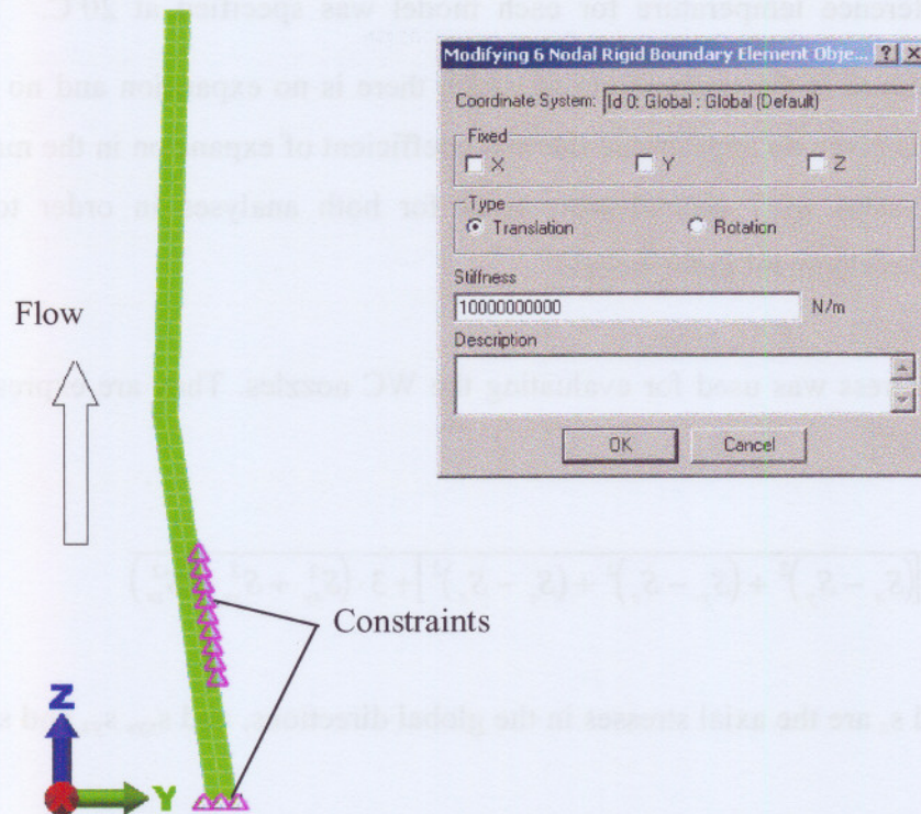
Figure 6.4. Constraints applied to the tungsten carbide nozzles
