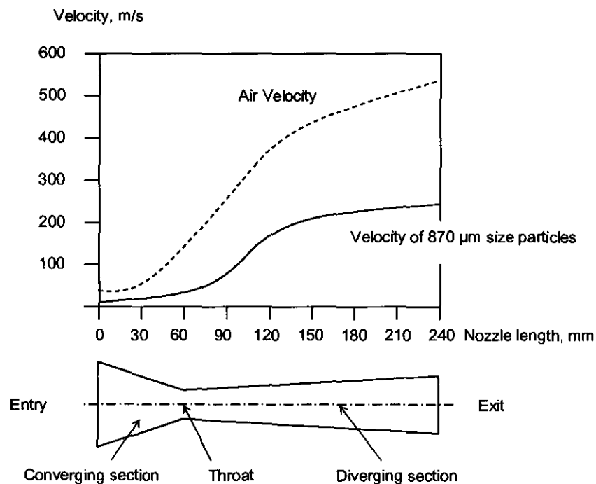
Figure 1.8. The relationship between nozzle length, air velocity and particle velocity, Seavey (1985)
