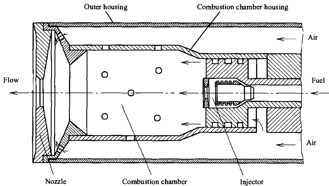
Figure 1.3. Schematic cross section of Varushin's N 2 HVAF gun for thermal spallation, (1973)
