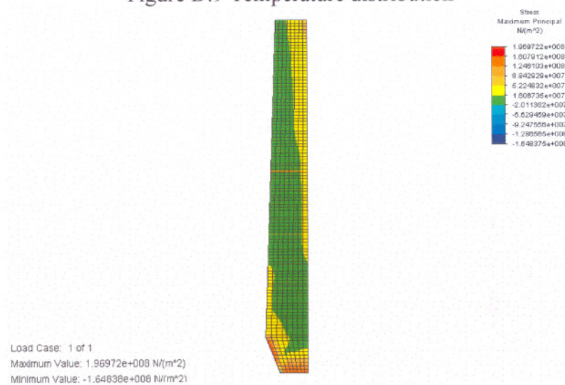
Figure D.10 Thermal stress distribution
