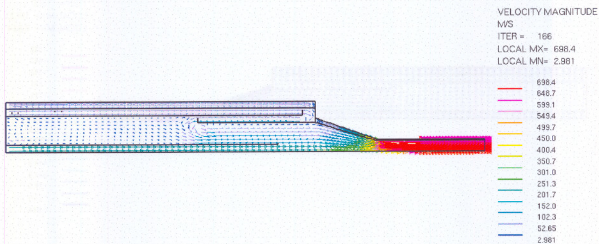
Figure C.2 Air velocity with the 50 mm straight nozzle
