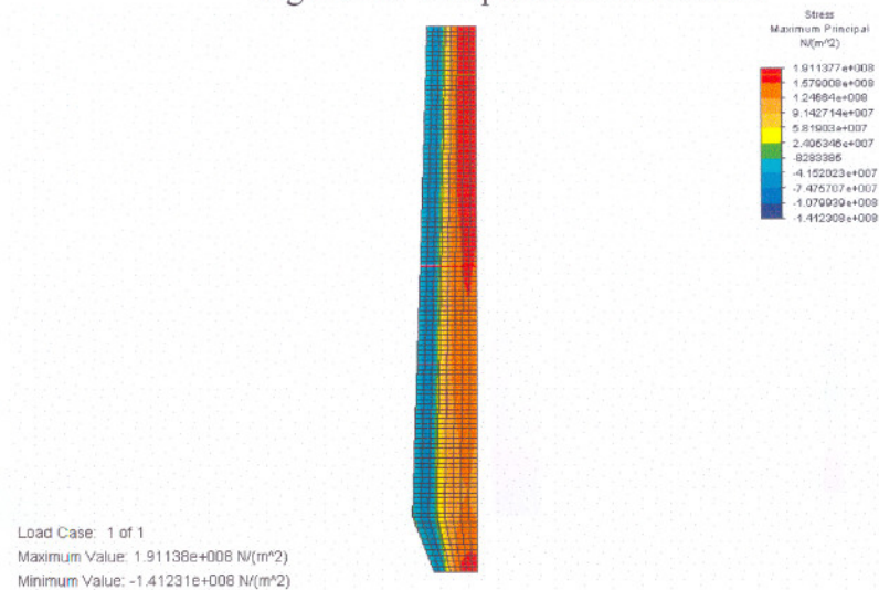
Figure D.2 Thermal stress distribution
