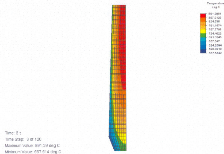
Figure D.42 Temperature distribution
