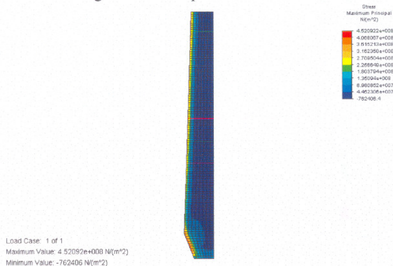
Figure D.42 Thermal stress distribution
