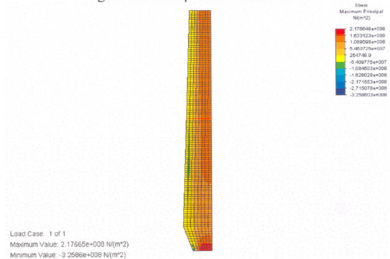
Figure D.4 Thermal stress distribution
