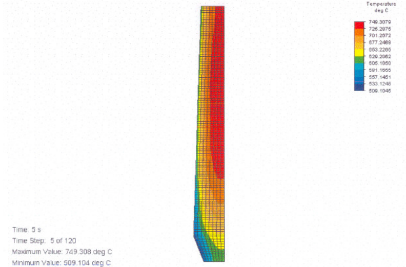
Figure D.46 Temperature distribution
