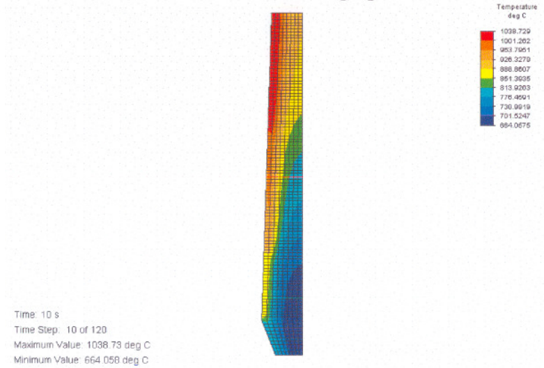
Figure D.30 Temperature distribution
