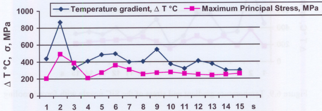
Figure 6.10. Temperature gradient and stress of the NSiC nozzle with free convection
