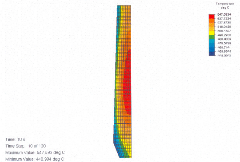
Figure D.24 Temperature distribution
