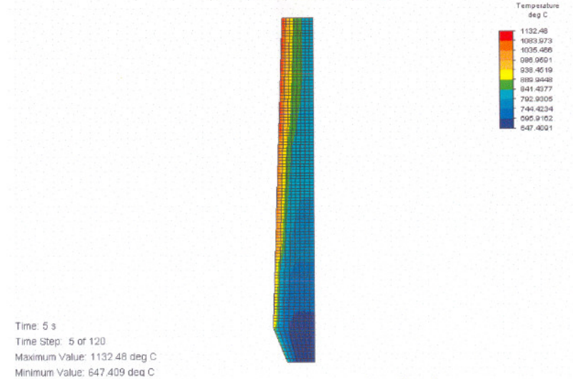
Figure D.3 Temperature distribution
