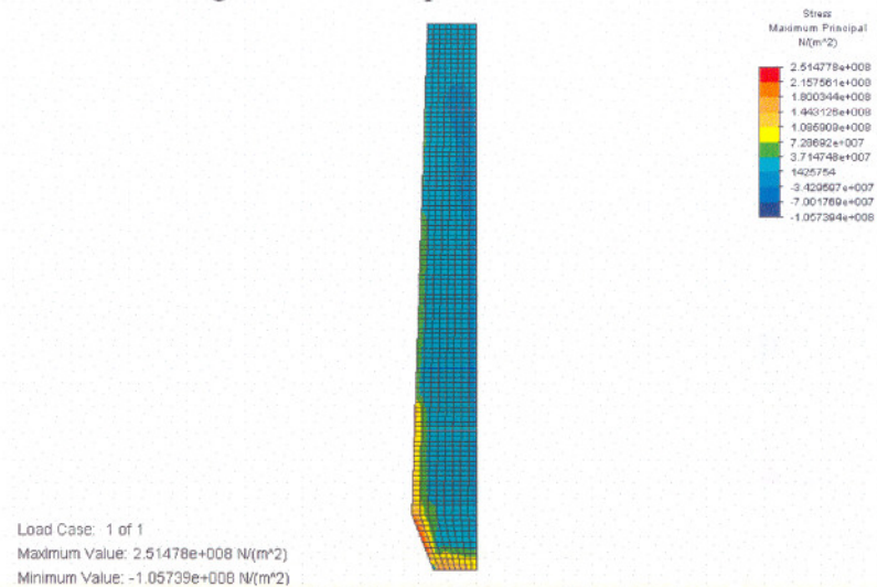
Figure D.16 Thermal stress distribution
