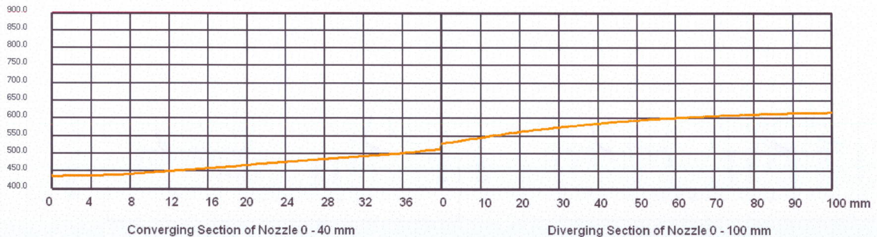
Figure C.21 Temperature distribution in the inner surface of the nozzle for the low fuel/air ratio ( k - \epsilon turbulence model)
