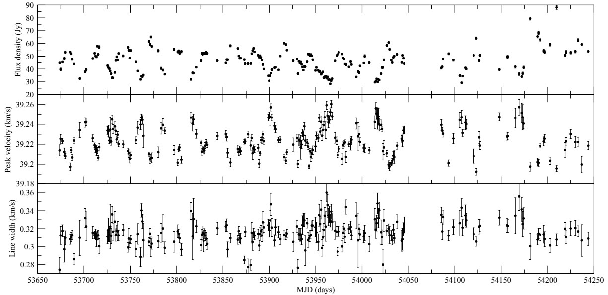
Figure 13. Results of Gaussian fits to the dominant spectral peak at 12.2 GHz. The top panel shows the flux density of the spectral channel at 39.23 \text{ km s}^{-1} , the middle and bottom panels show the change in the Gaussian peak position and width, respectively, of the spectral feature.
