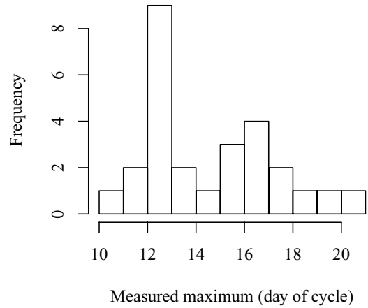
Figure 11. Histogram of measured peak flare times for 27 well-sampled cycles.
