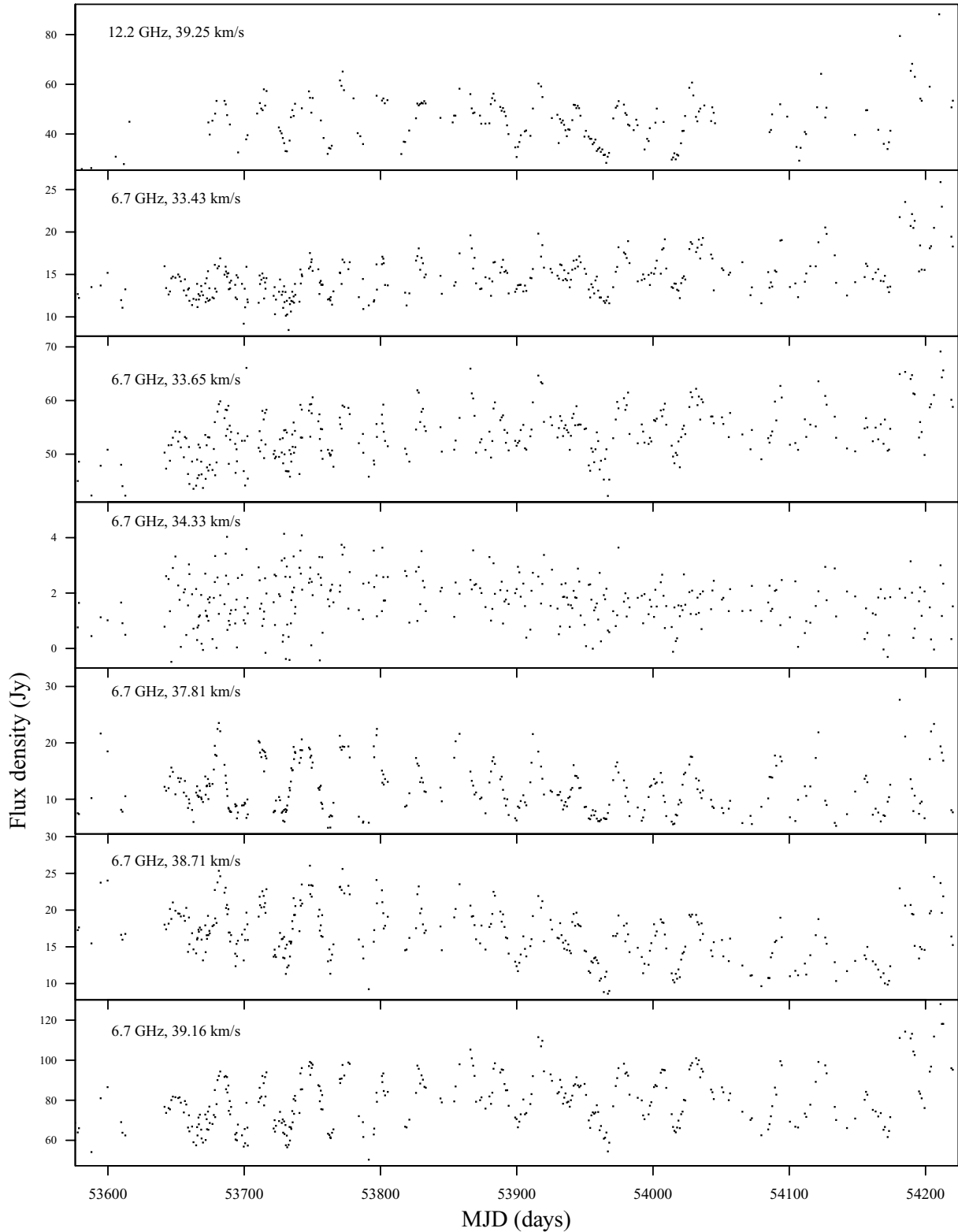
Figure 7. Time series for selected features in G12.89+0.49 covering the period over which daily monitoring was done. More features are shown in the online version of the article – see Supporting Information.
