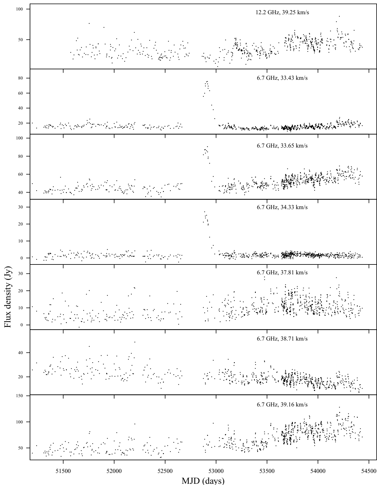
Figure 6. Time series for selected features in G12.89+0.49. Note that the top panel shows the 12.2 GHz feature while all the others are at 6.7 GHz. Plots of the time series of all of the identified features are available in the online version of the article – see Supporting Information.
