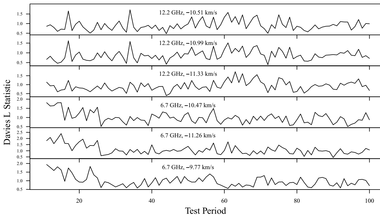
Figure 3. Result of epoch-fold period search on G351.42+0.64.
