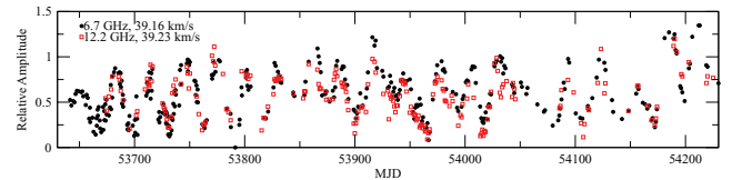
Figure 20. Comparison of flare behaviour at 12.2 and 6.7 GHz. Flare amplitudes have been normalized.
