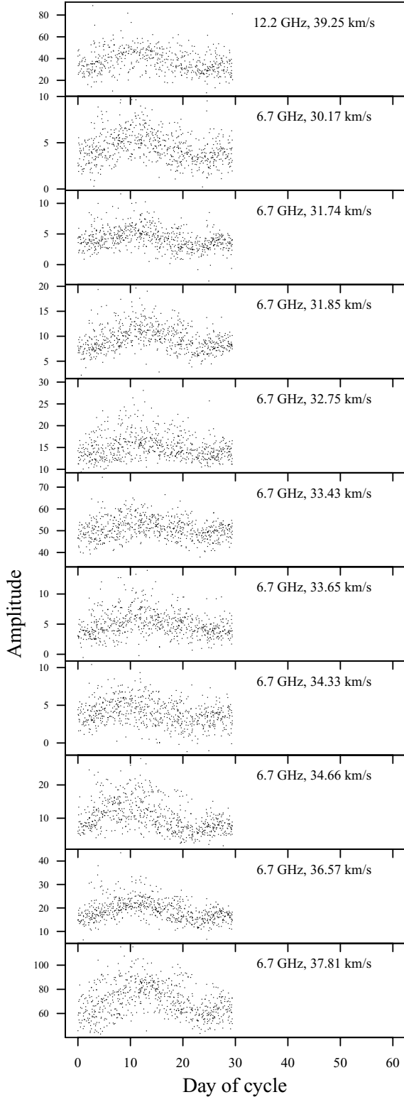
Figure 10. Time series folded modulo 29.5 d.
