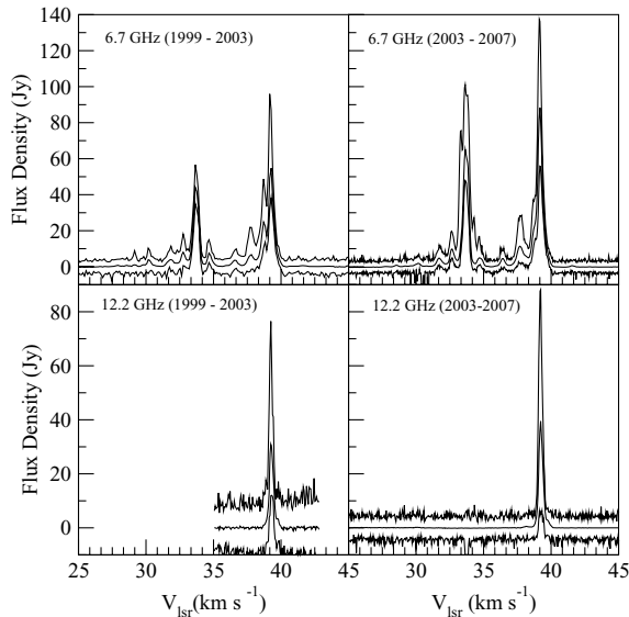
Figure 5. Range of variation of the masers in G12.89+0.49. In each panel, the upper curve shows the upper envelope, the middle curve is the averaged spectrum and the lower curve shows the lower envelope.
