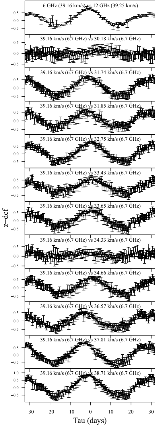
Figure 18. The z -transformed discrete correlation function for pairs of time series. The top panel is for the dominant peak ( 39 \text{ km s}^{-1} ) at 12.2 and 6.7 GHz. The subsequent plots are for cross-correlations at 6.7 GHz of the main peak against all other spectral features. The velocity channels are given in the legends.
