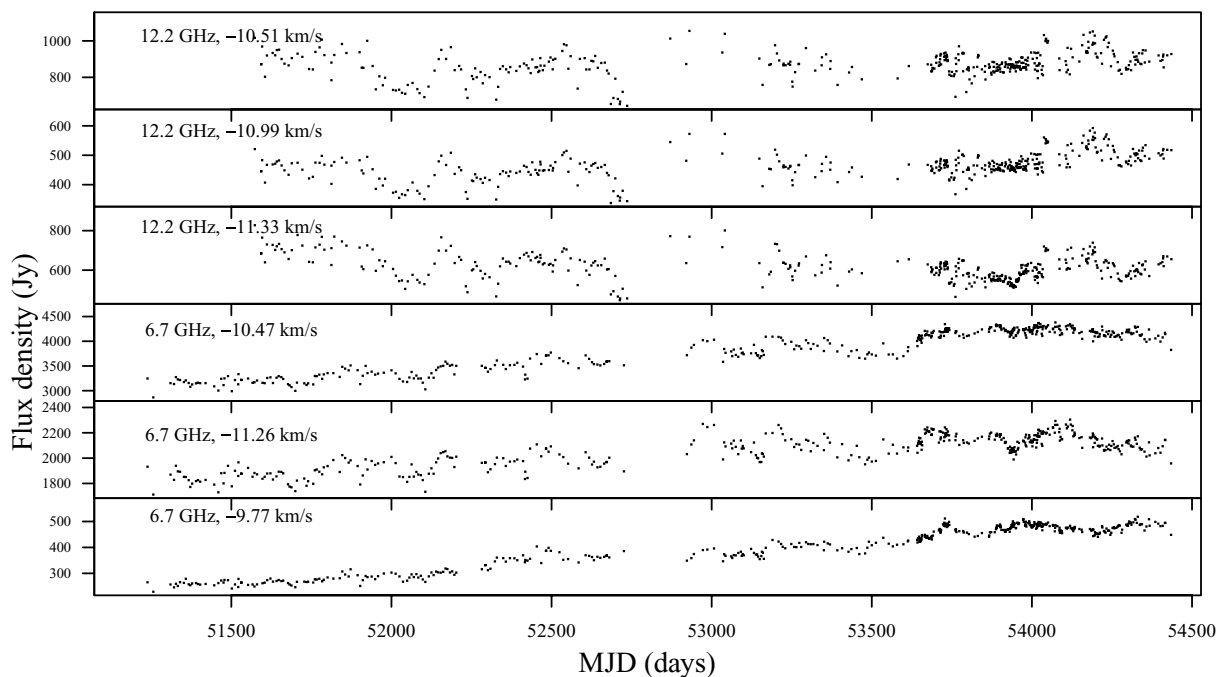
Figure 2. Time series for selected features in G351.42+0.64.
