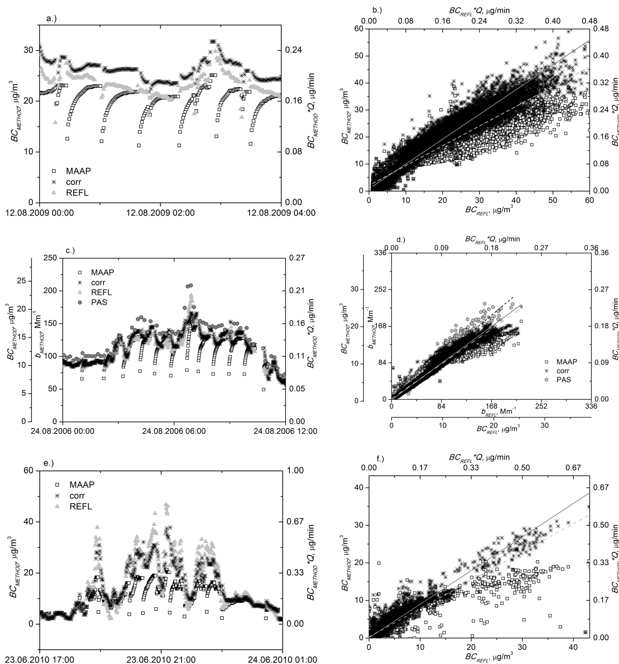
Fig. 5. Examples of the correction algorithm applied to the datasets from Gual Pahari (a, b), Beijing (c, d), and Welgegund (e, f). In panels (b), (d), and (f) the datasets from different methods are compared against the reflected BC signal, BC_{REFL} . Lines in these figures are linear fits to data. BC in Beijing was measured with 1 : 1 dilution. For Beijing, the absorption coefficients b_{METHOD} at 532 nm from the PAS and those derived from the MAAP (see text for details) are also shown.
