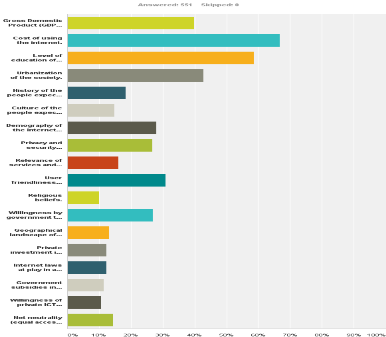
Fig 4.3: Factor ranking
