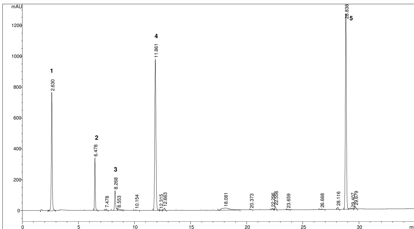
Figure 6. HPLC chromatogram of secondary compounds from various plants after 1 h of UV radiation. Solvent gradient was applied to obtain the results. The peaks were identified as: as: 1, nicotine; 2, salicin; 3, strophanthin-G; 4, rutin; 5, dienostrol.
