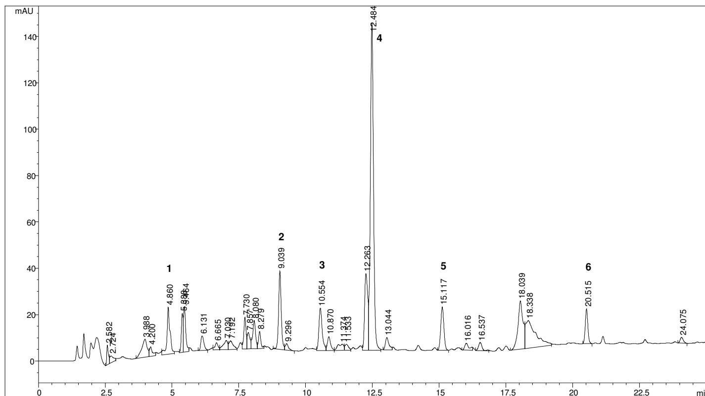
Figure 9. The chromatogram of P. auriculata compounds treated with UV-irradiation.
