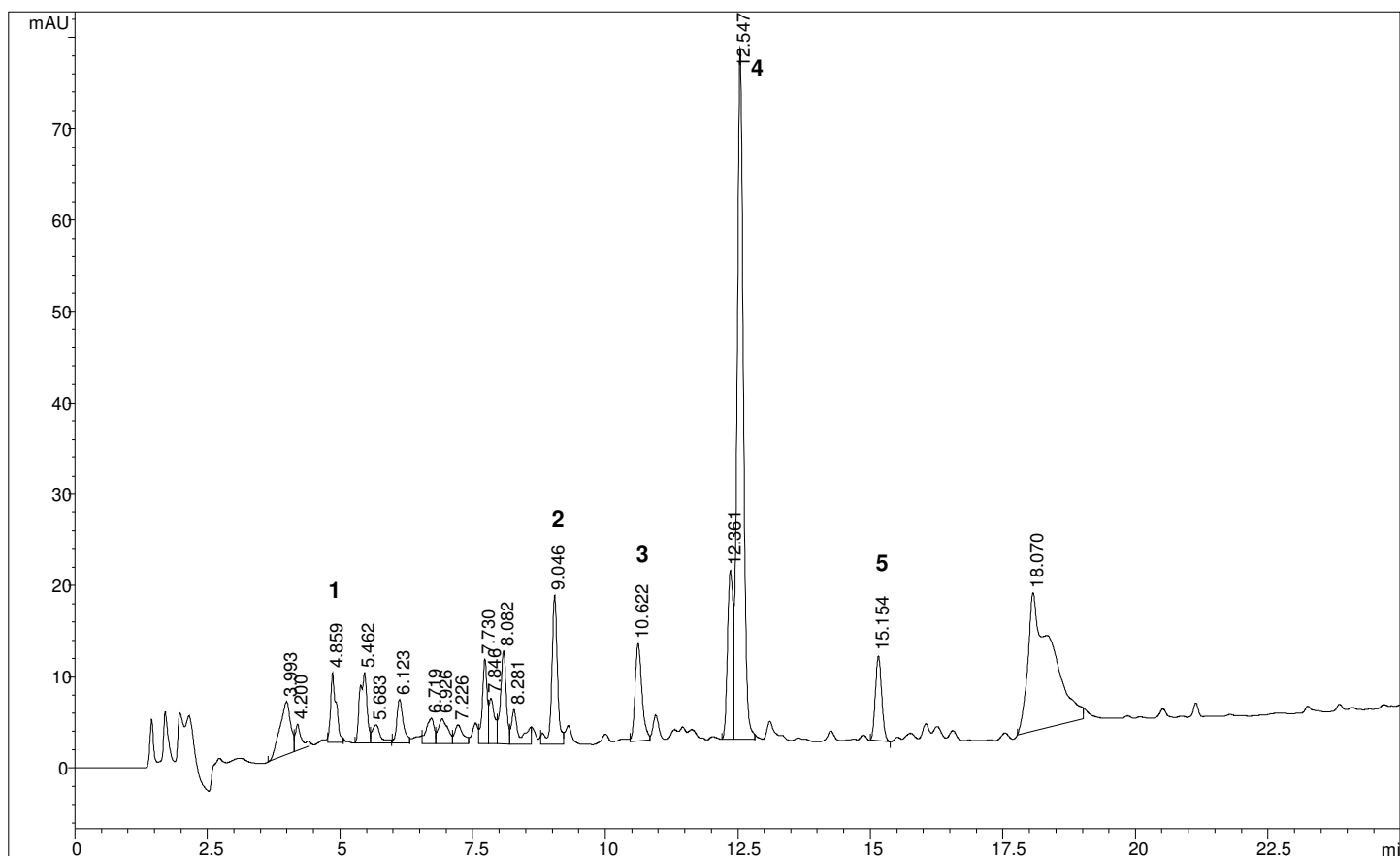
Figure 10. The HPLC chromatogram of P. auriculata compounds treated with activated charcoal.
