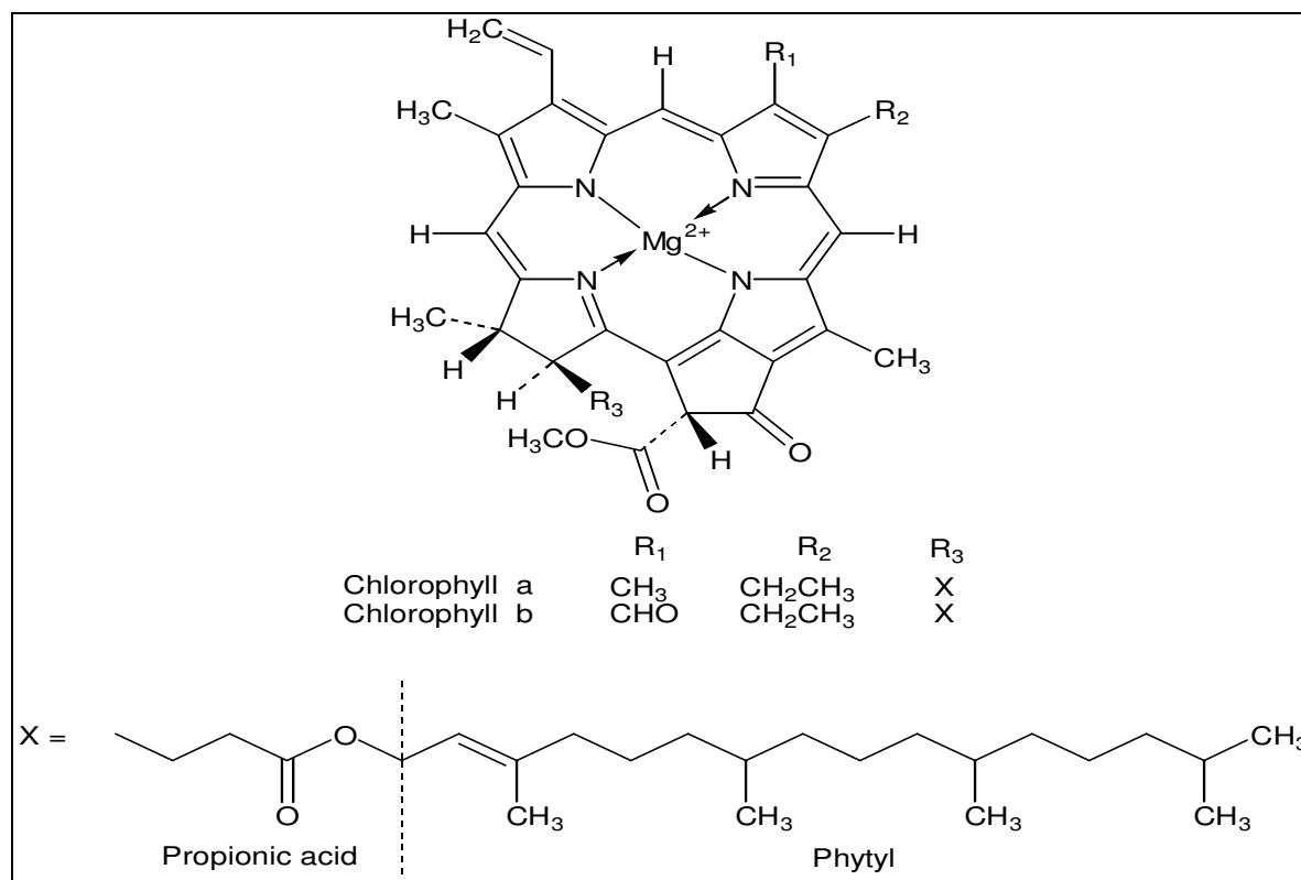
Figure 1. The chlorophyll molecule. (Merck index, 2000).
