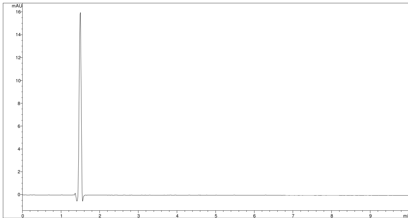
Figure 3. The chromatogram of the chlorophyll a sample that was treated with UV radiation showing that chlorophyll a was completely degraded after 1 h of treatment in the photochemical reactor.
