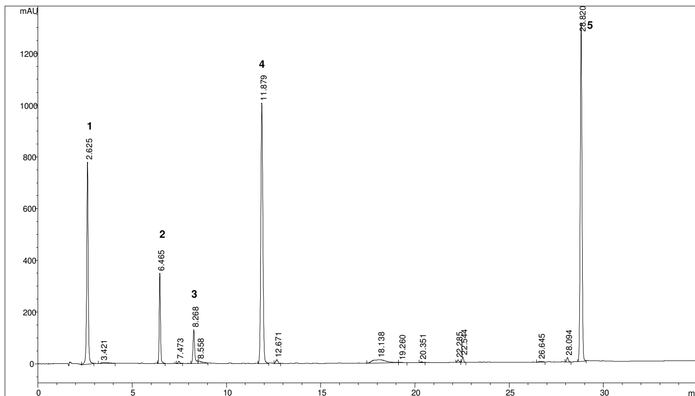
Figure 5. HPLC chromatogram of secondary compounds isolated from various plants recorded at 254 nm. Solvent gradient was applied to obtain the results. The peaks were identified as: 1, nicotine; 2, salicin; 3, strophanthin-g; 4, rutin; 5, dienostrol.
