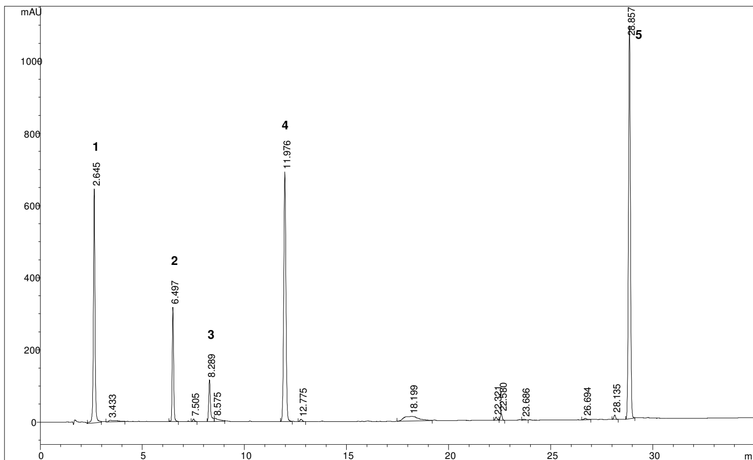
Figure 7. HPLC chromatogram of secondary compounds treated with activated charcoal. The peaks were identified as: 1, nicotine; 2, salicin; 3, strophanthin-G; 4, rutin; 5, dienolestrol.
