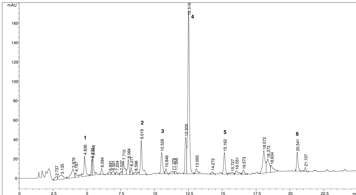
Figure 8. The chromatogram of P. auriculata compounds.
