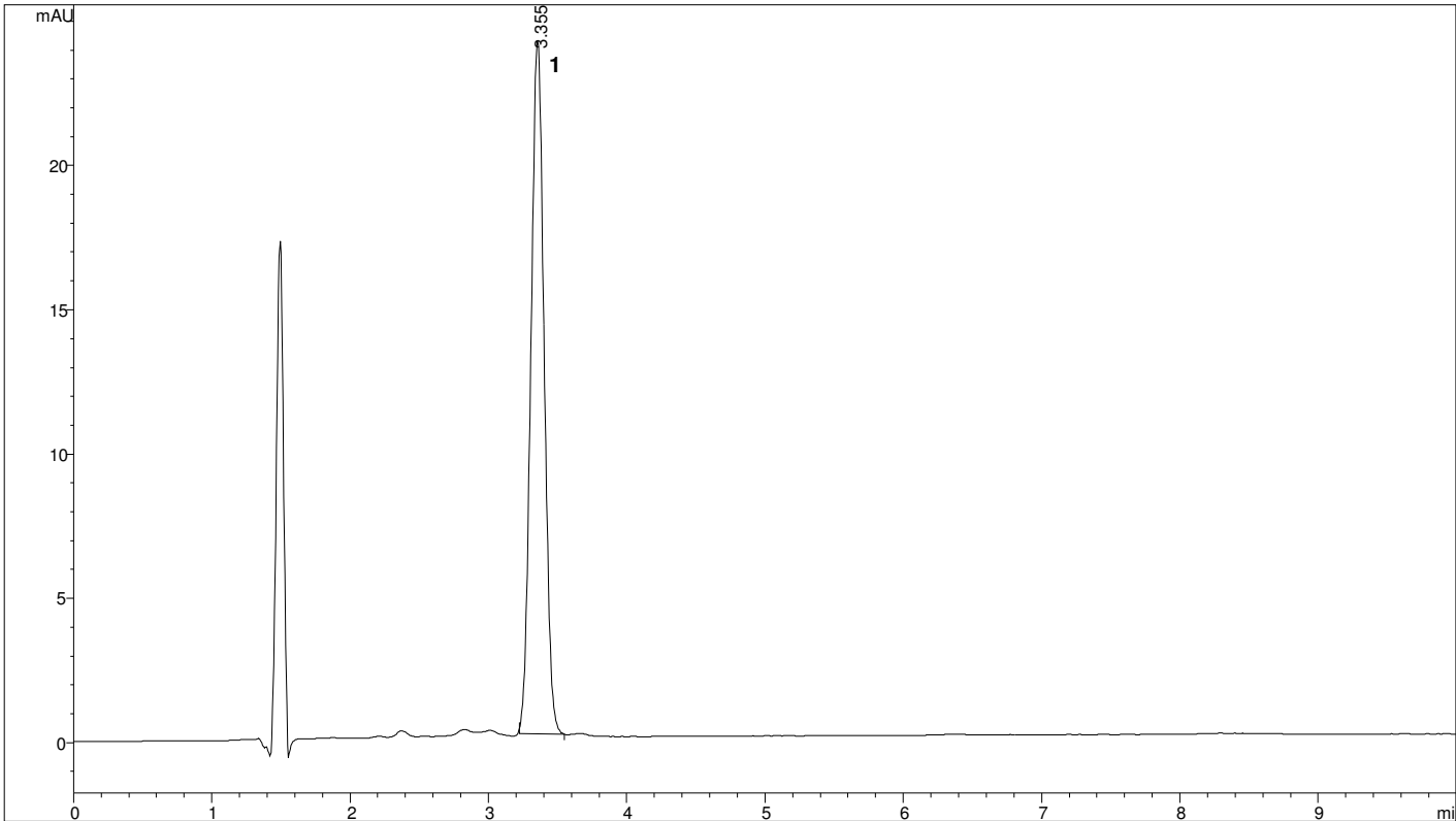
Figure 2. The peak of chlorophyll a eluted at time 3.355 min.
