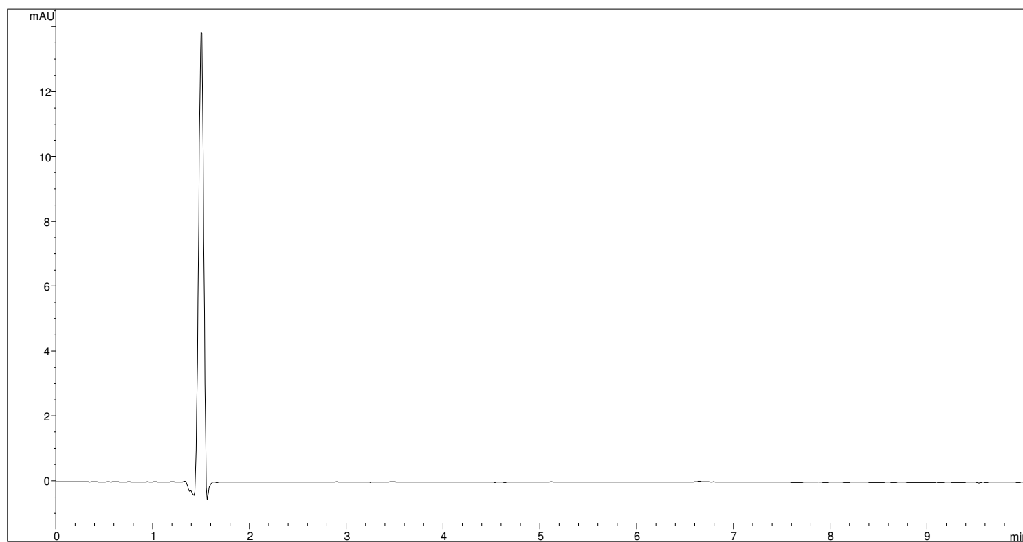
Figure 4. A typical chromatogram of chlorophyll a after treatment activated charcoal. The chromatogram shows that all the chlorophyll a was absorbed by the activated charcoal from the sample.
