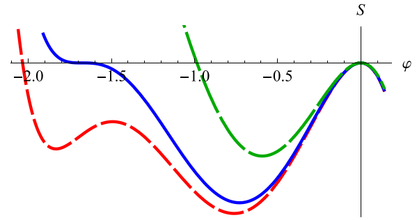
FIG. 14. Typical Sagdeev pseudopotentials having a negative triple root structure (solid blue curve, at M/M_s = 1.0390 ), a supersoliton (red dashes, at M/M_s = 1.0397 ), and an ordinary soliton (long green dashes, at M/M_s = 1.0352 ), all three for f=0.786 , \beta=0 , and \mu=1 .
