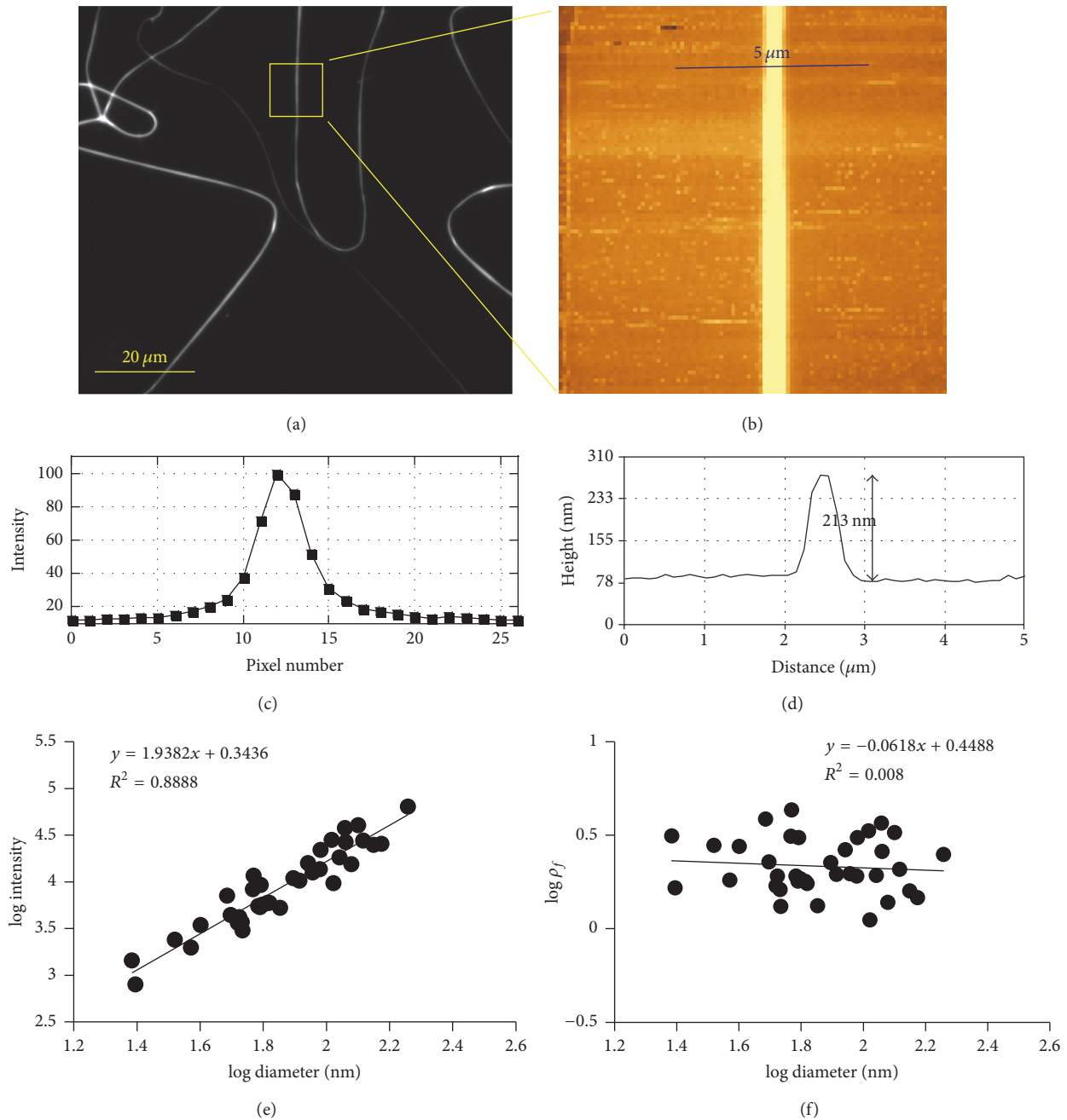
FIGURE 3: Fluorescence intensity of electrospun fibrinogen fiber cross-section as a function of diameter. (a) Fluorescence image (subsection of 180\ \mu\text{m} \times 180\ \mu\text{m} field of view) of electrospun fibrinogen fibers. (b) AFM image of the fiber in the yellow box. (c) Fluorescence intensity of the fiber in the yellow box along the blue line drawn in (b). One pixel is 200\ \text{nm} ( 40\times objective lens). (d) Height measurement along the indicated 5\ \mu\text{m} long blue line in (b). (e) The slope of the relationship between light intensity and fiber diameter is 1.9 on a log-log scale, close to the value of 2.0 expected for a homogenous fluorophore distribution within a cross-section. (f) Fluorophore density \rho_f = N_f/A is independent of fiber diameter, as would be expected for a homogeneous fiber. Each data point represents four measurements.
