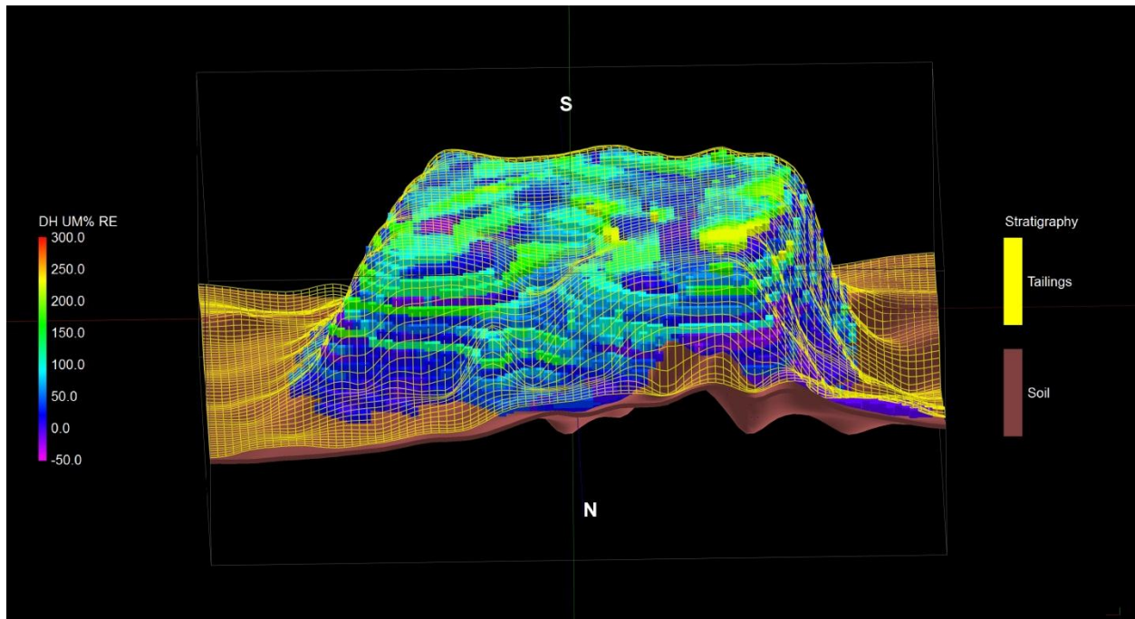
Figure D.1: U mobility results, north-south view
