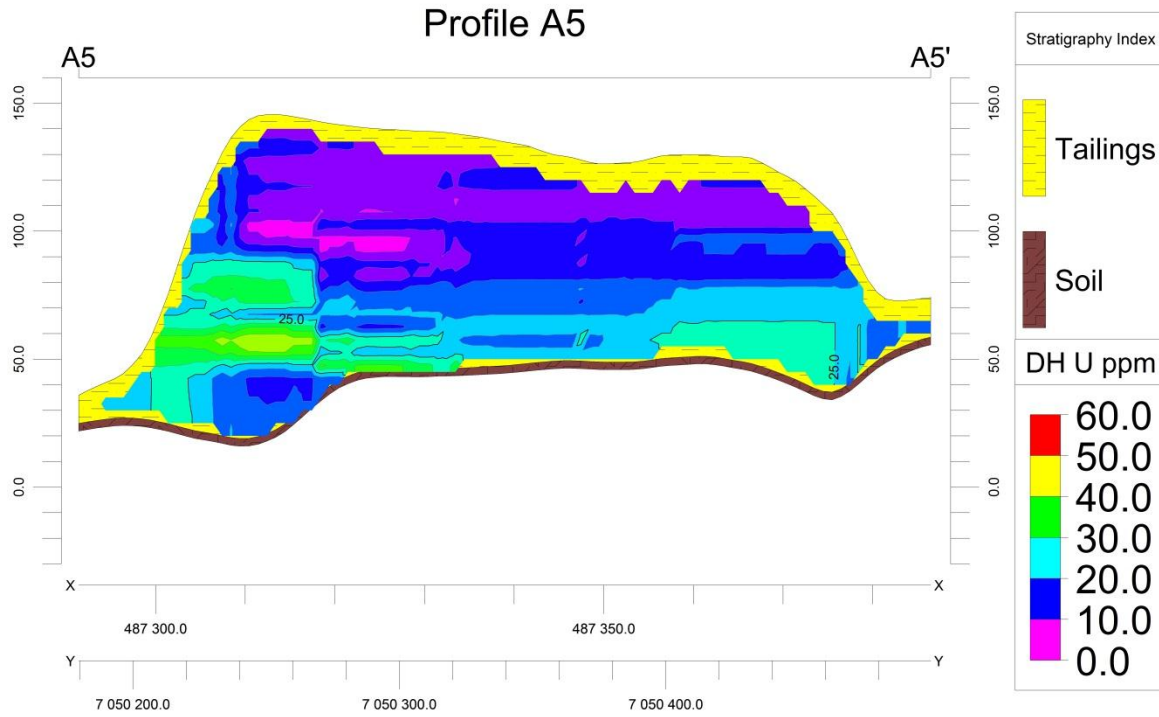
Figure A.10: Profile A5, New Machavie down-hole spectrometry
