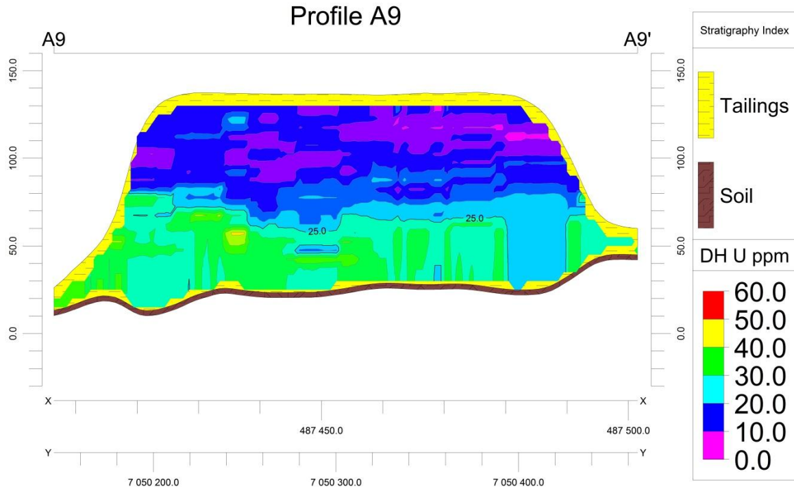
Figure A.14: Profile A9, New Machavie down-hole spectrometry
