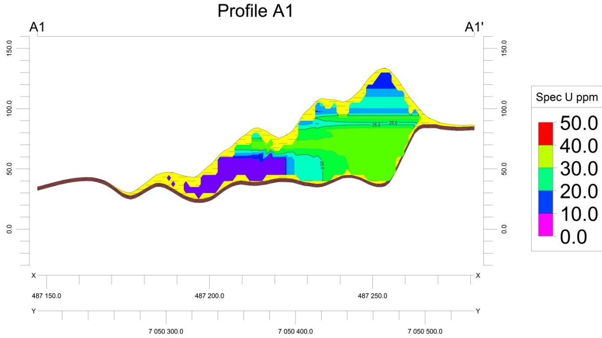
Figure B.6: Profile A1, Laboratory spectrometry model
