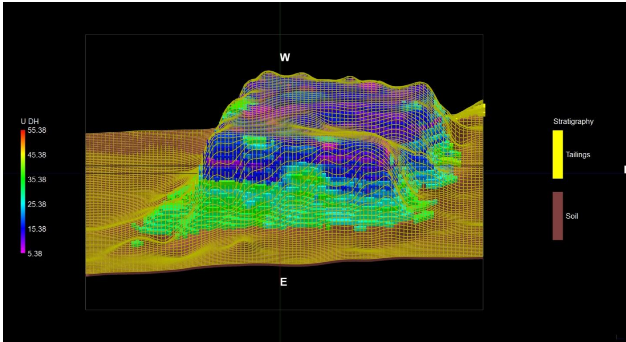
Figure A.3: New Machavie east-west view
