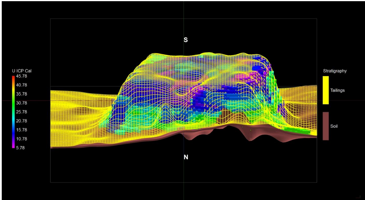
Figure B.1: Laboratory spectrometry model, north-south view
