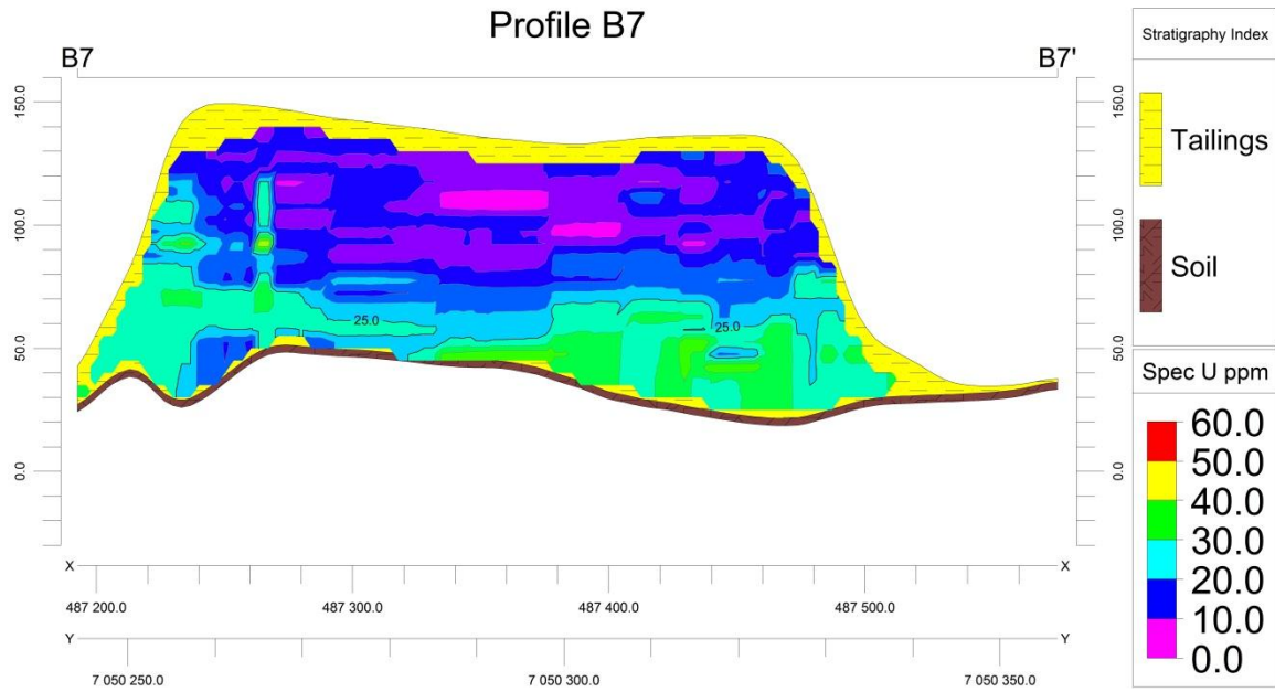
Figure A.23: Profile B7, New Machavie down-hole spectrometry
