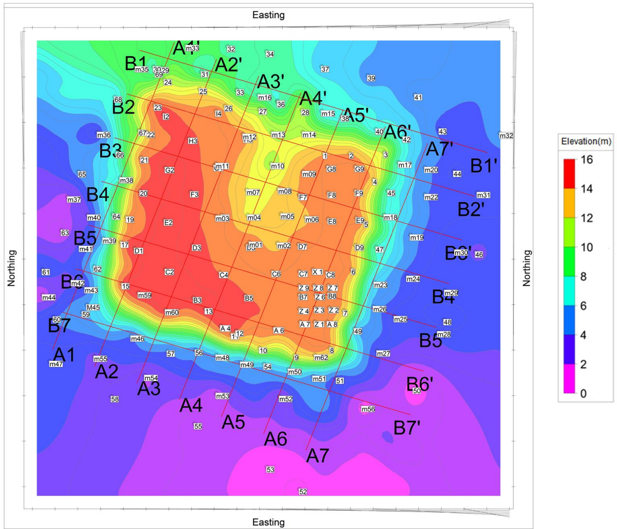
Figure B.5: Location map of laboratory spectrometry profiles
