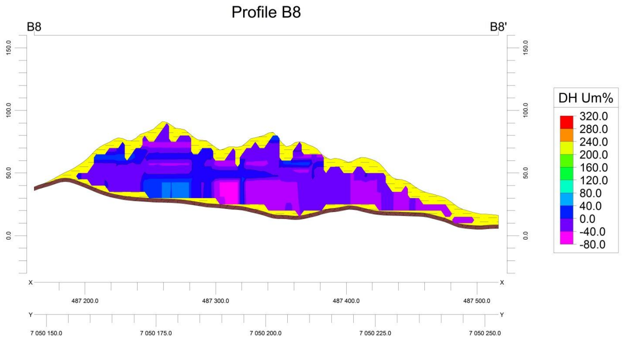
Figure D.21: Um% profile B8
