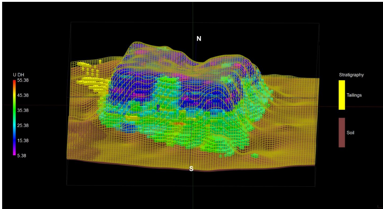
Figure A.1: New Machavie north-south view
