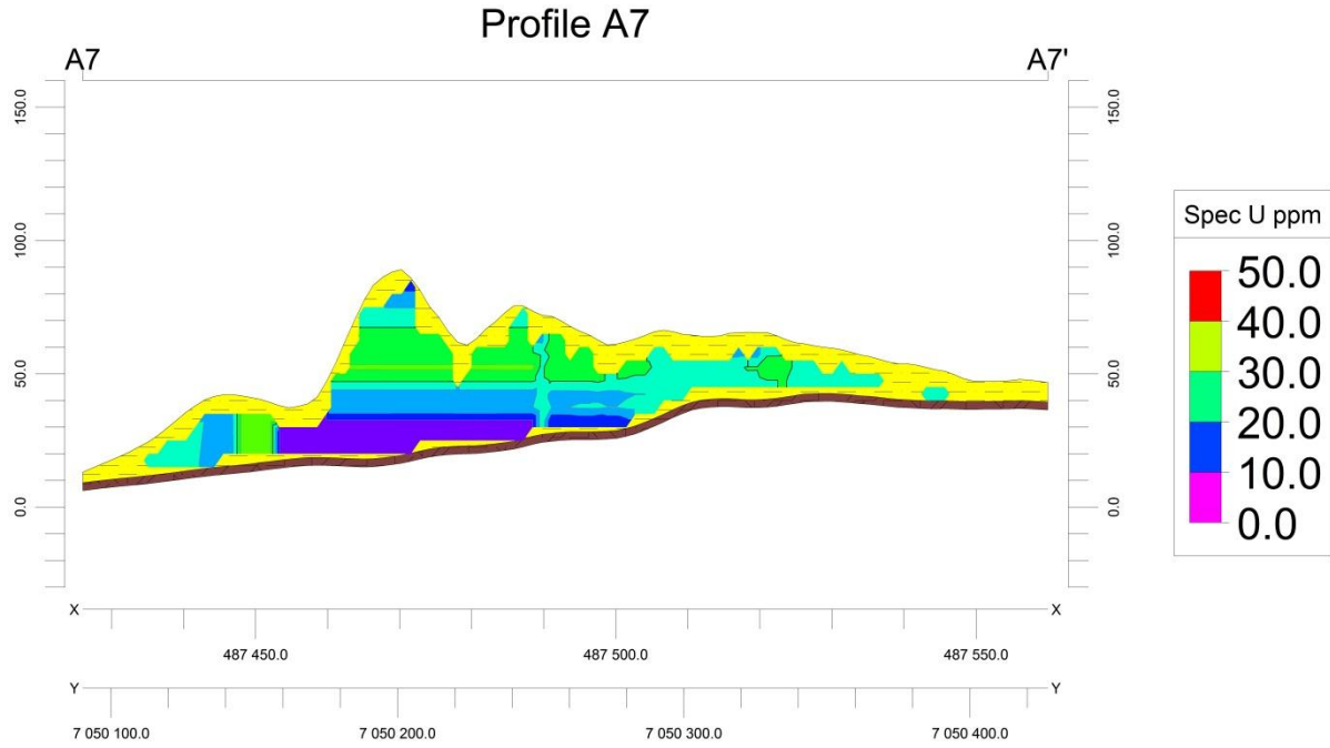
Figure B.12: Profile A7, Laboratory spectrometry model
