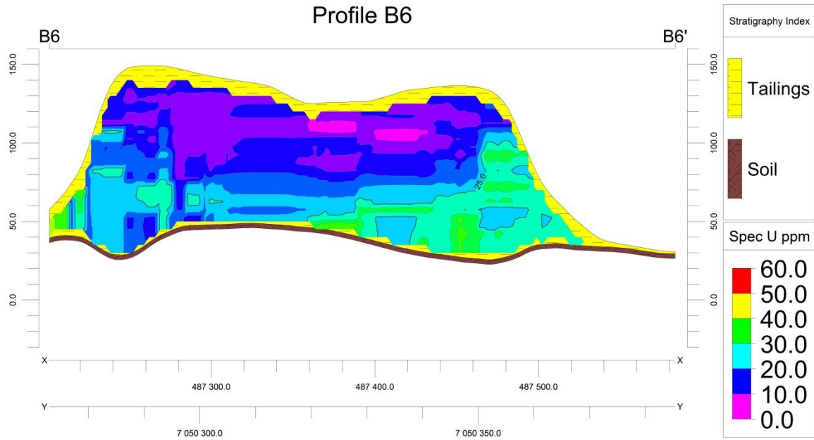
Figure A.22: Profile B6, New Machavie down-hole spectrometry
