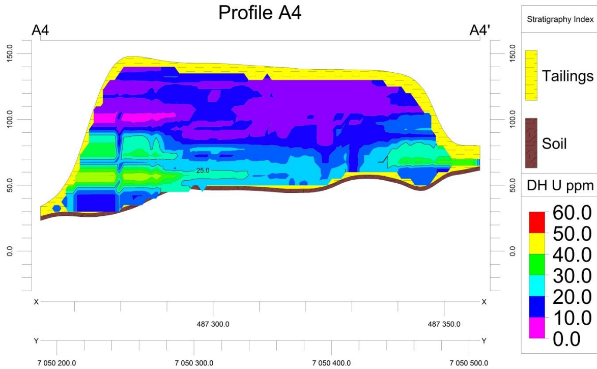
Figure A.9: Profile A4, New Machavie down-hole spectrometry
