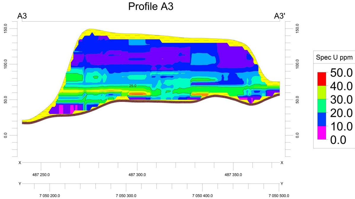
Figure B.8: Profile A3, Laboratory spectrometry model
