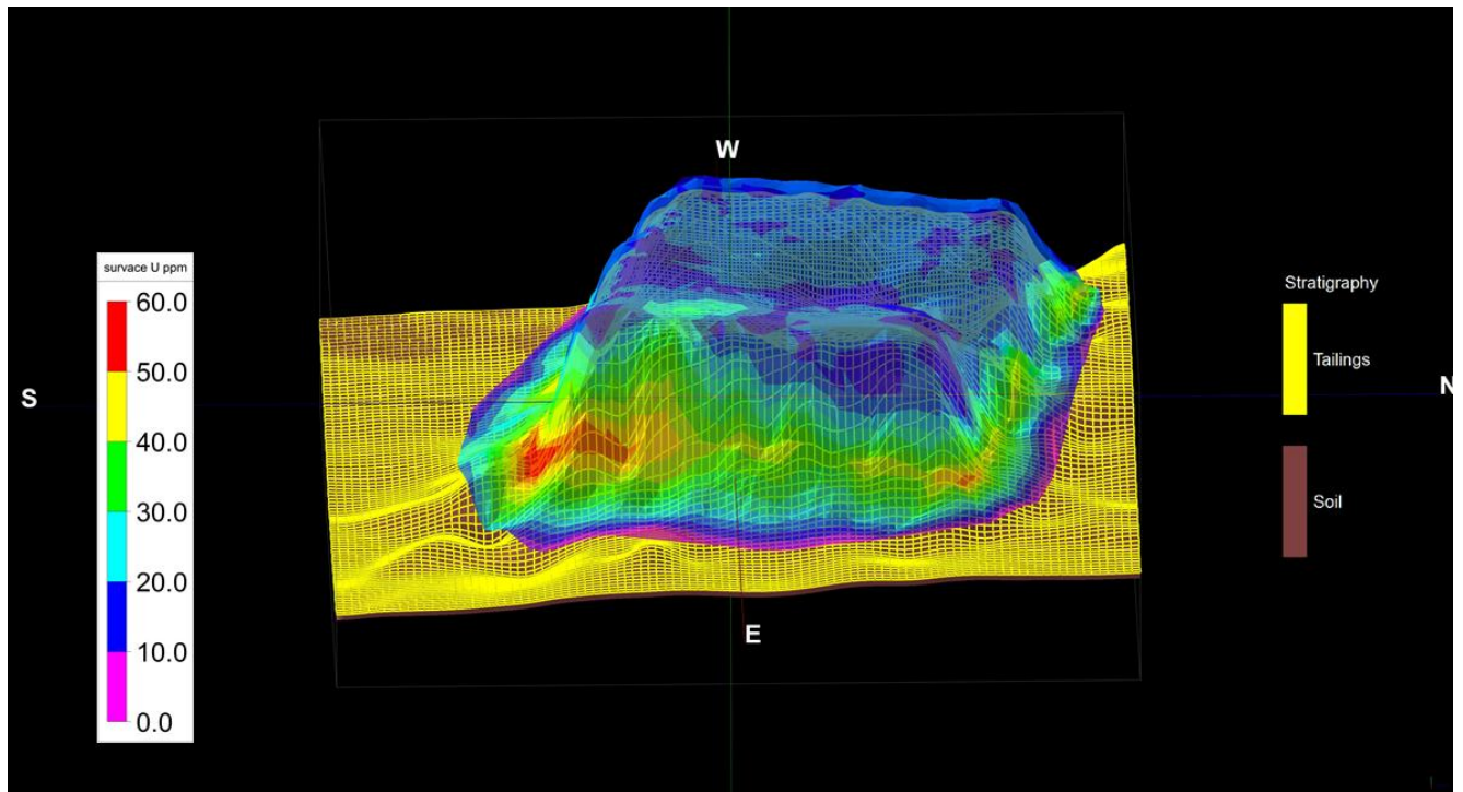
Figure C.3: Surface spectrometry results, east-west view
