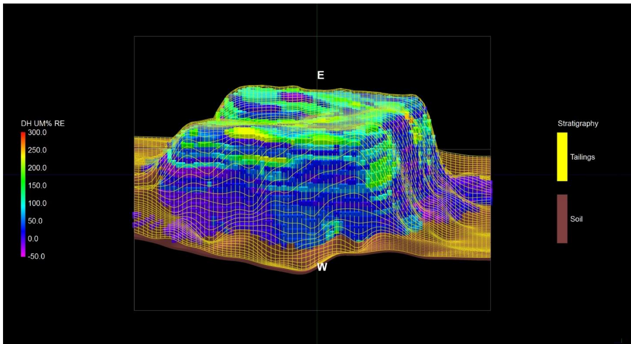
Figure D.4: U mobility results, west-east view
