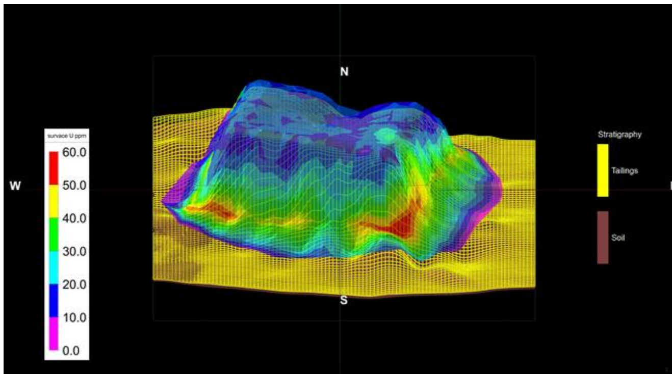
Figure C.1: Surface spectrometry results, south-north view
