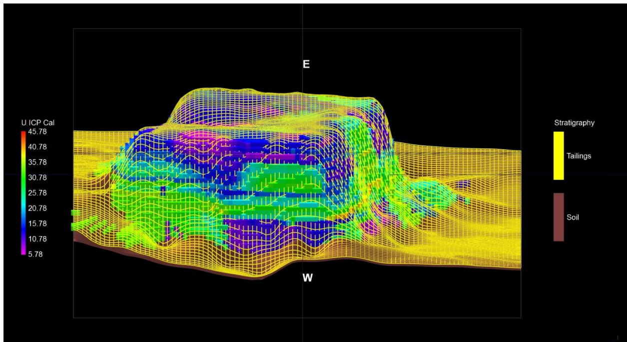
Figure B.4: Laboratory spectrometry model, west-east view
