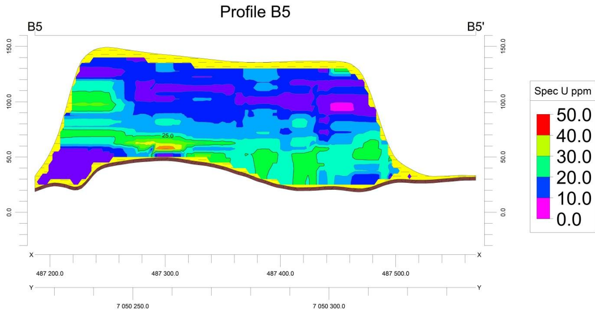
Figure B.17: Profile B5, Laboratory spectrometry model
