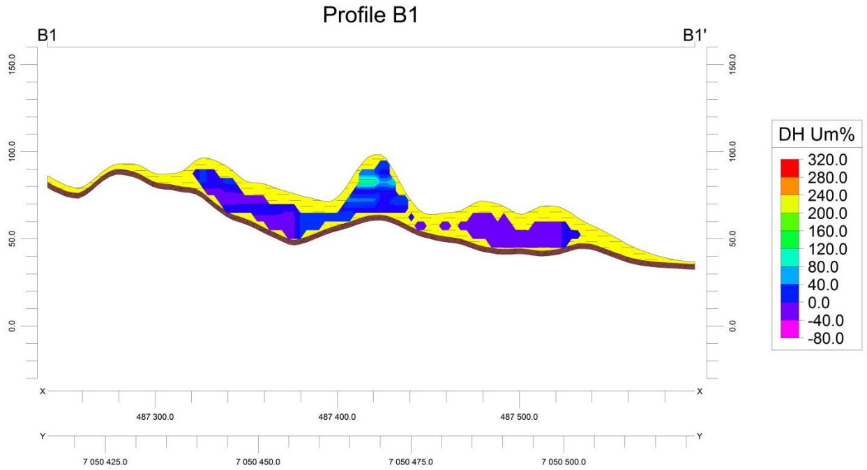
Figure D.14: Um% profile B1
