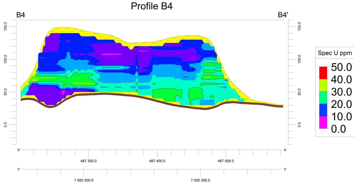
Figure B.16: Profile B4, Laboratory spectrometry model
