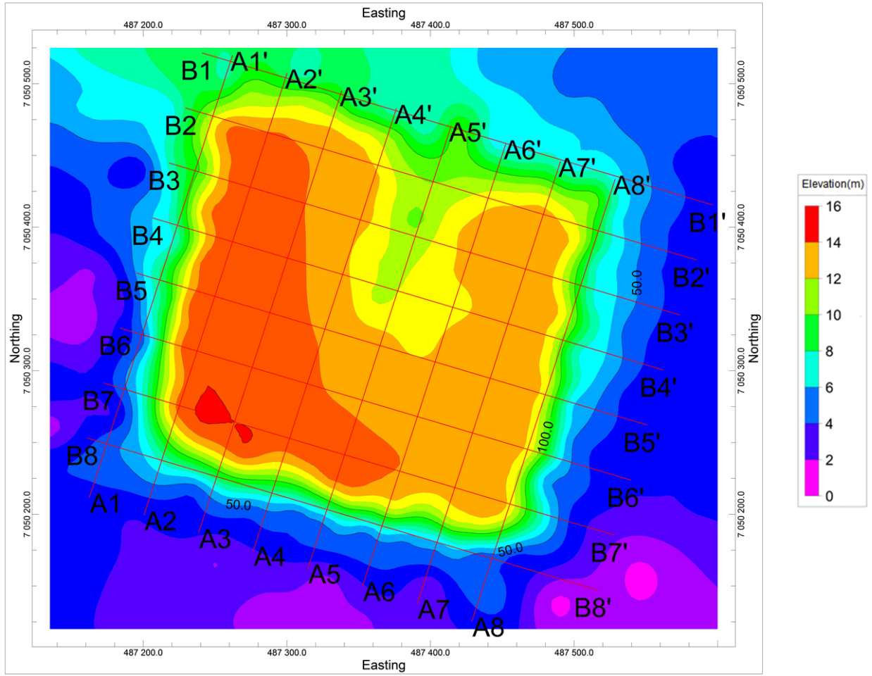
Figure D.5: Location map of U mobility profiles
