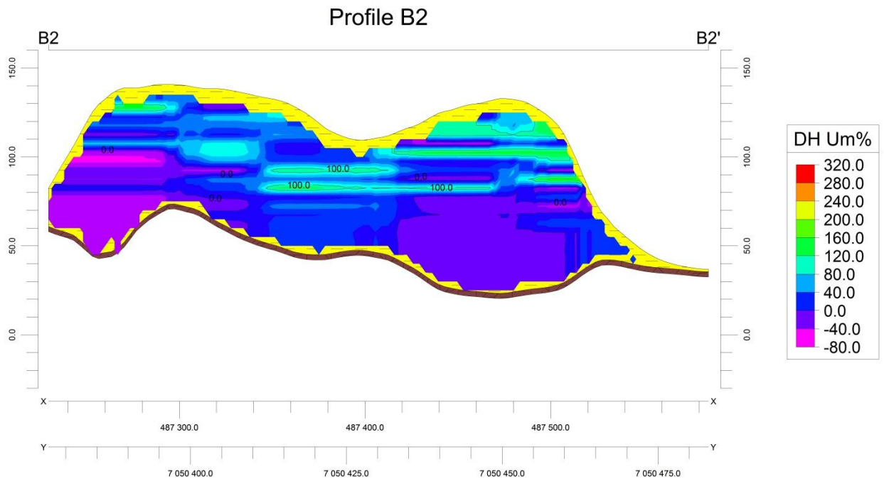
Figure D.15: Um% profile B2
