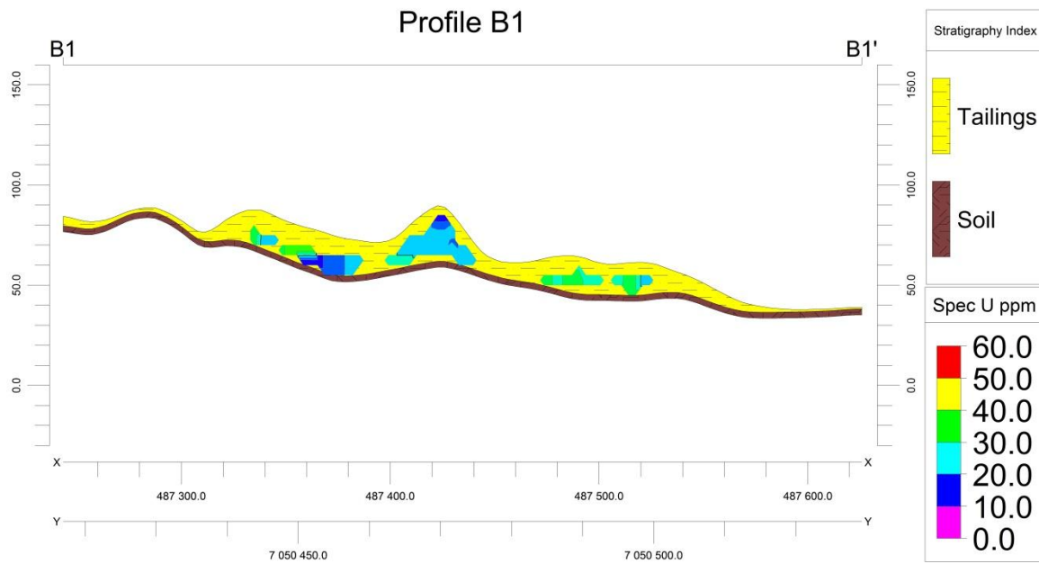
Figure A.17: Profile B1, New Machavie down-hole spectrometry
