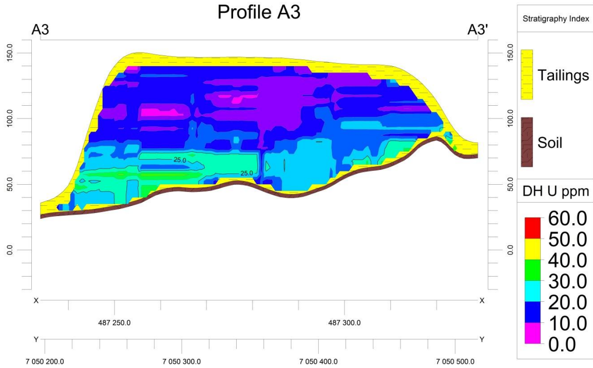
Figure A.8: Profile A3, New Machavie down-hole spectrometry
