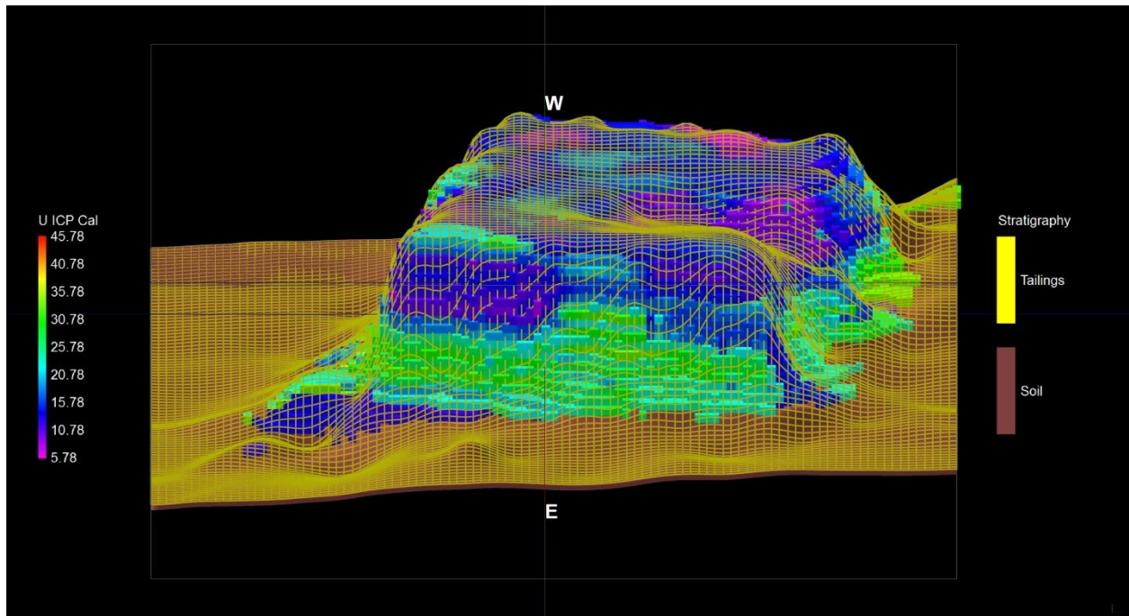
Figure B.3: Laboratory spectrometry model, east-west view
