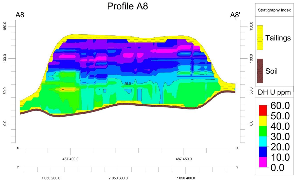
Figure A.13: Profile A8, New Machavie down-hole spectrometry
