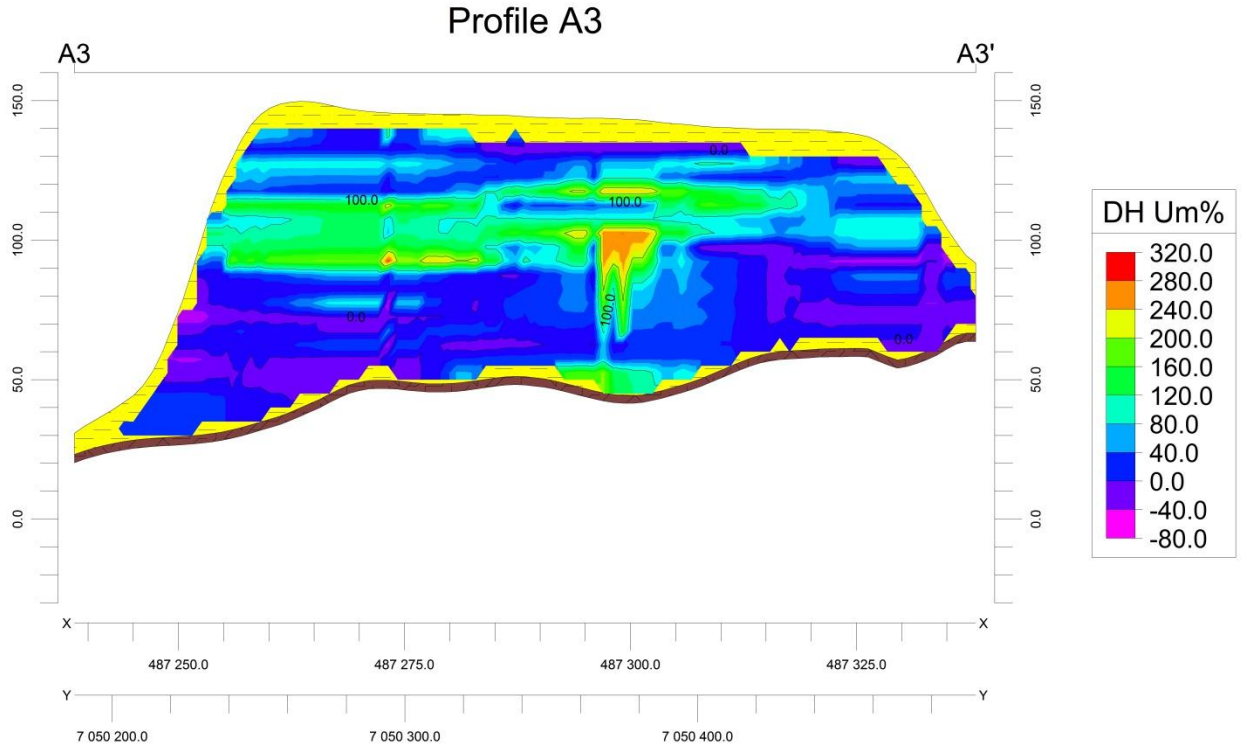
Figure D.8: Um% profile A3
