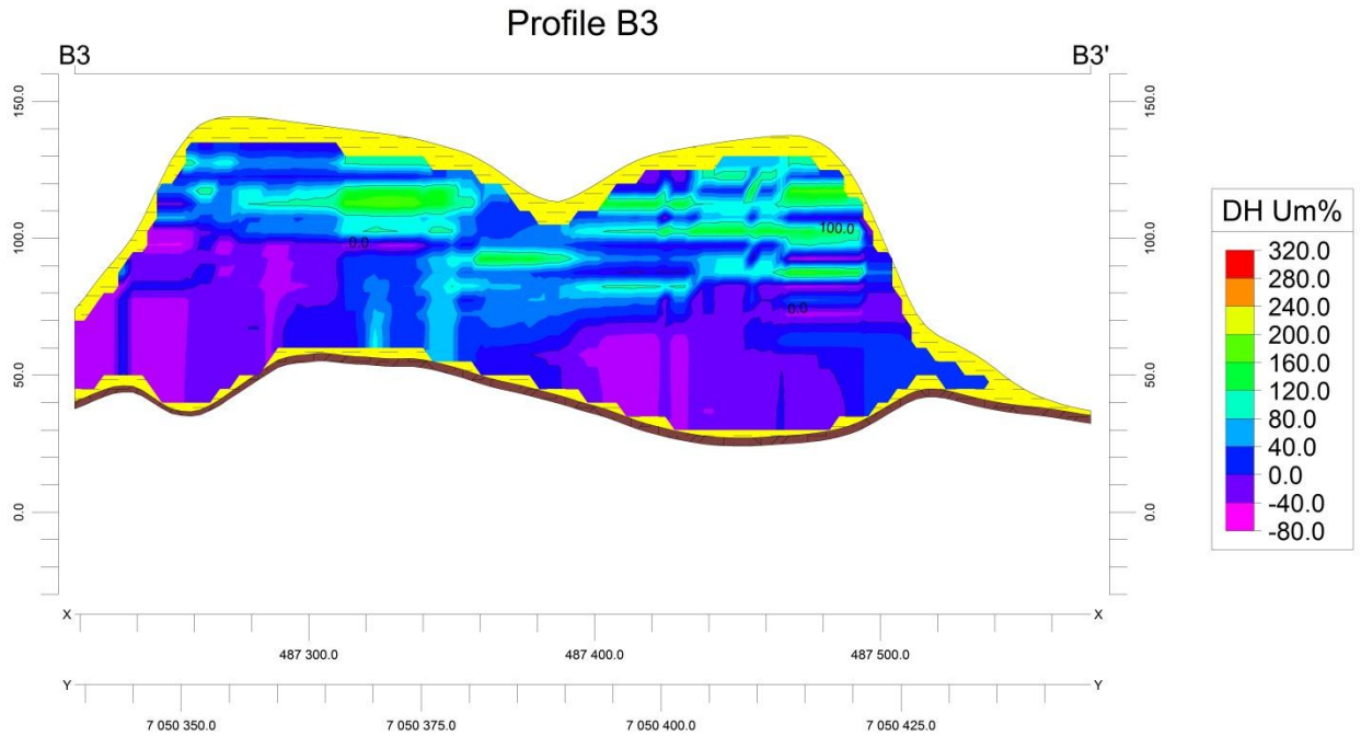
Figure D.16: Um% profile B3
