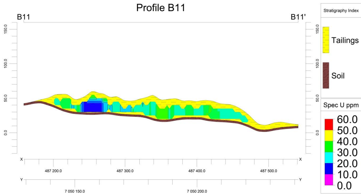
Figure A.27: Profile B11, New Machavie down-hole spectrometry
