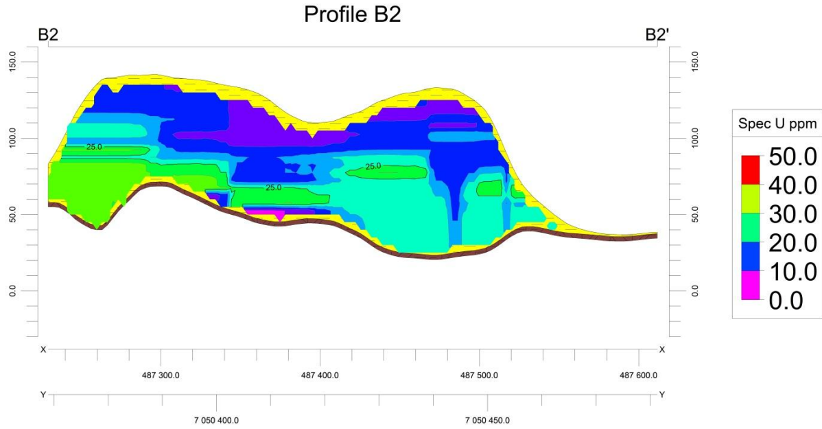
Figure B.14: Profile B2, Laboratory spectrometry model
