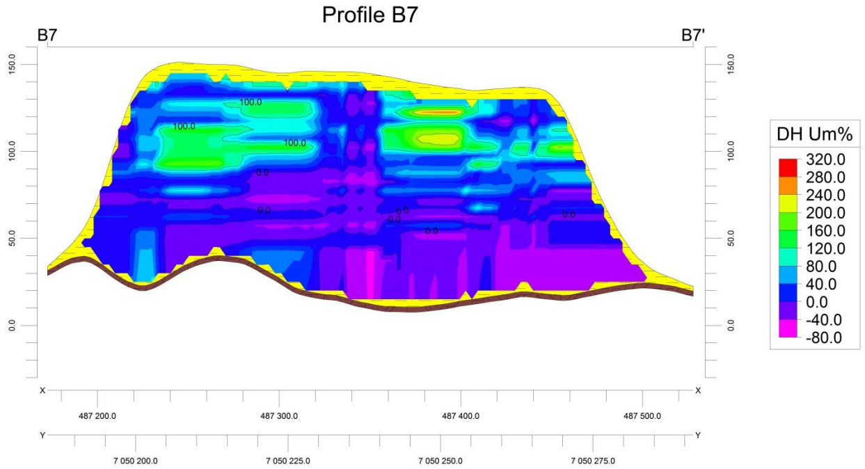
Figure D.20: Um% profile B7
