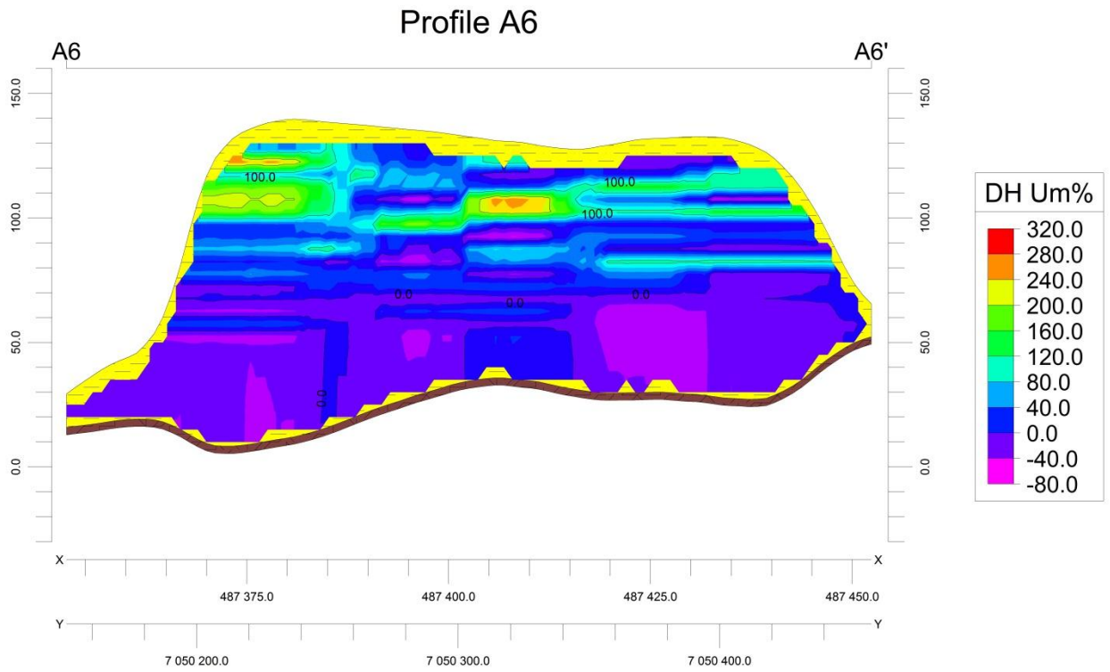
Figure D.11: Um% profile A6
