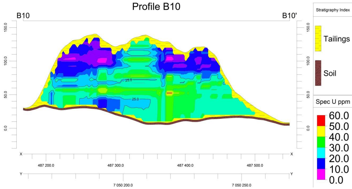
Figure A.26: Profile B10, New Machavie down-hole spectrometry
