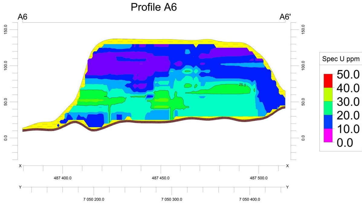
Figure B.11: Profile A6, Laboratory spectrometry model
