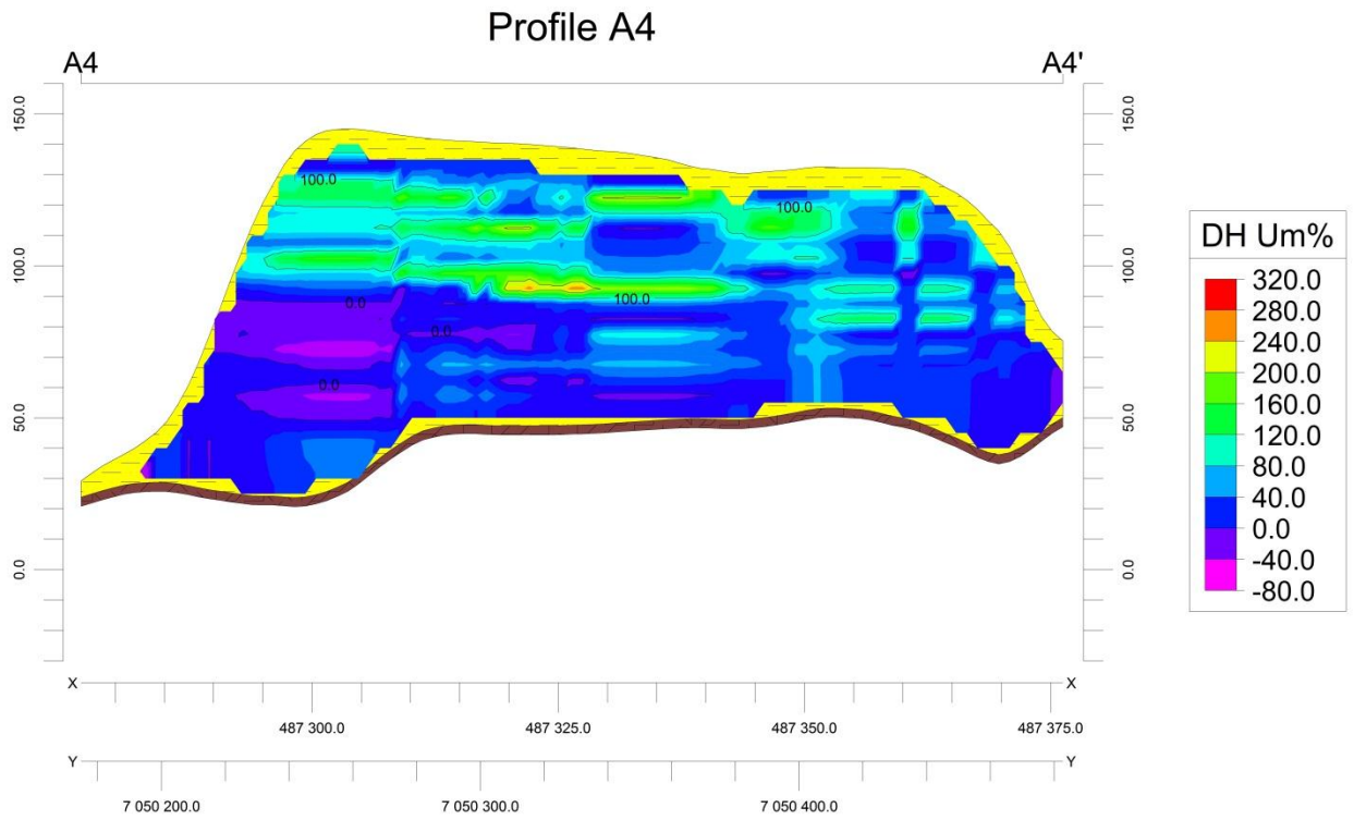
Figure D.9: Um% profile A4
