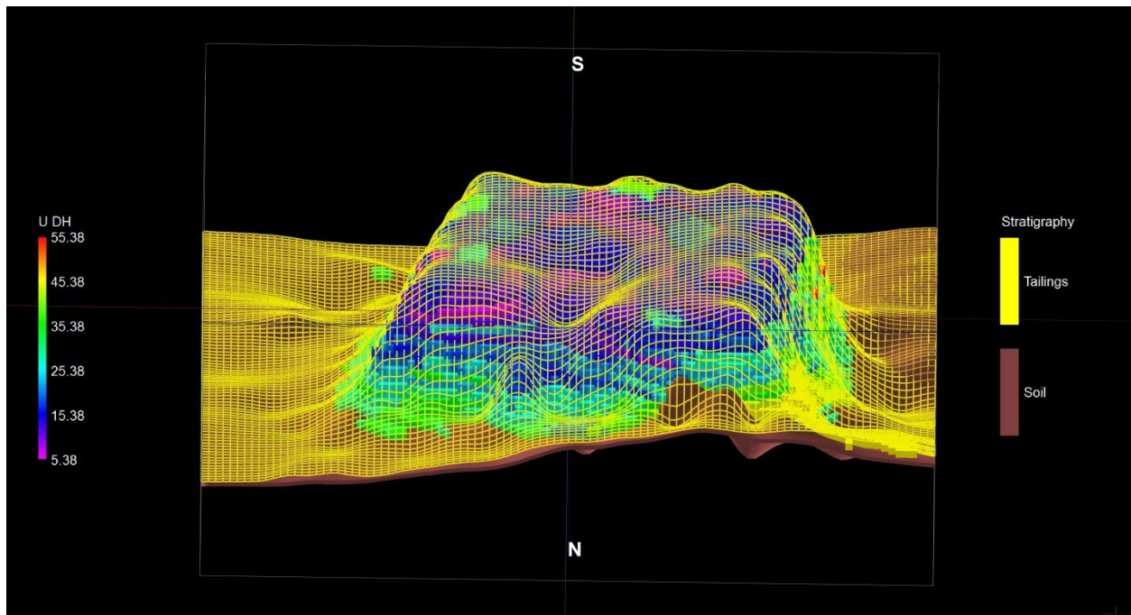
Figure A.2: New Machavie south-north view
