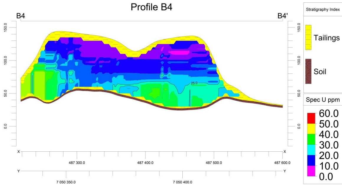
Figure A.20: Profile B4, New Machavie down-hole spectrometry
