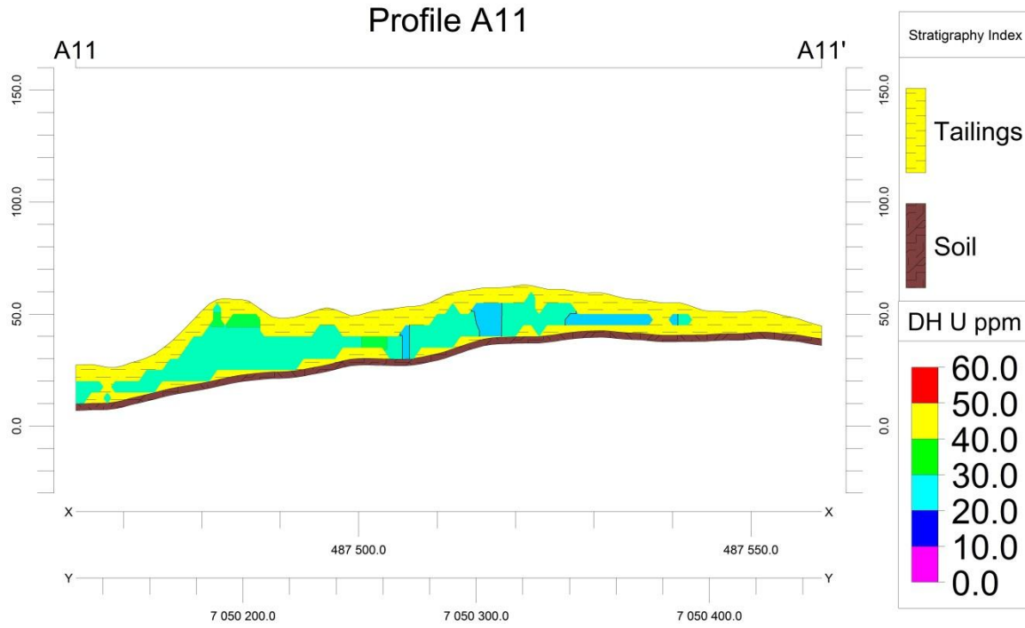
Figure A.16: Profile A11, New Machavie down-hole spectrometry
