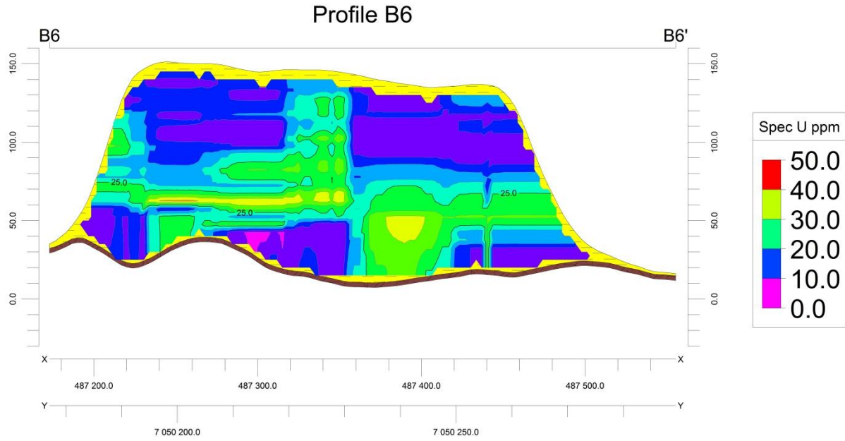
Figure B.18: Profile B6, Laboratory spectrometry model
