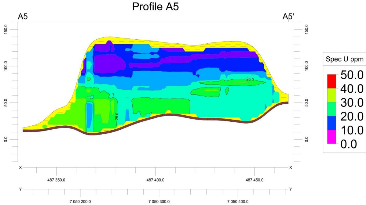
Figure B.10: Profile A5, Laboratory spectrometry model
