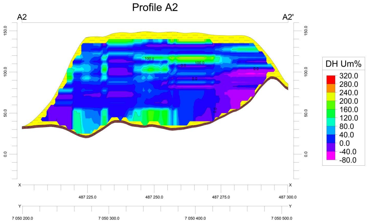
Figure D.7: Um% profile A2
