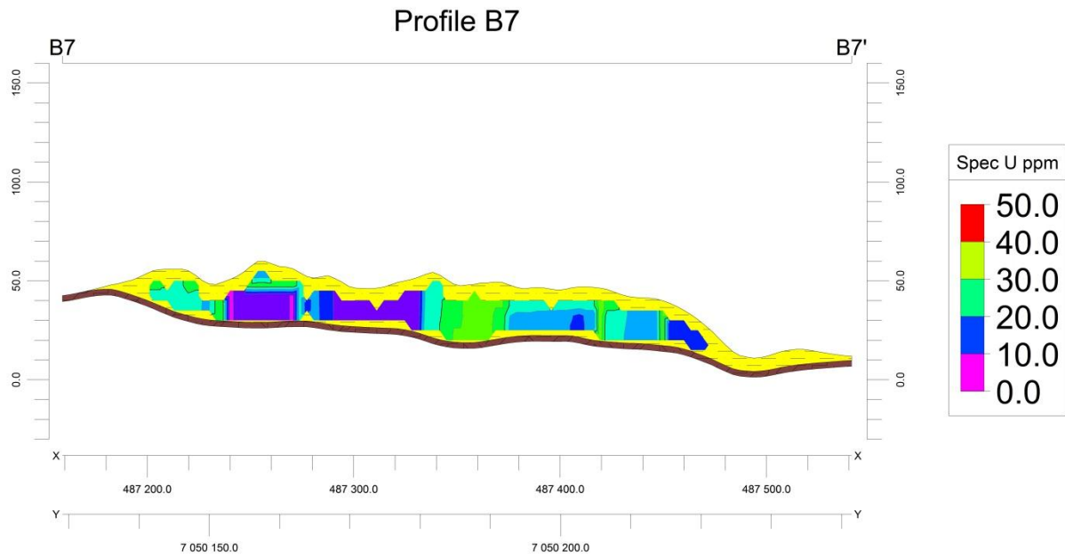
Figure B.19: Profile B7, Laboratory spectrometry model
