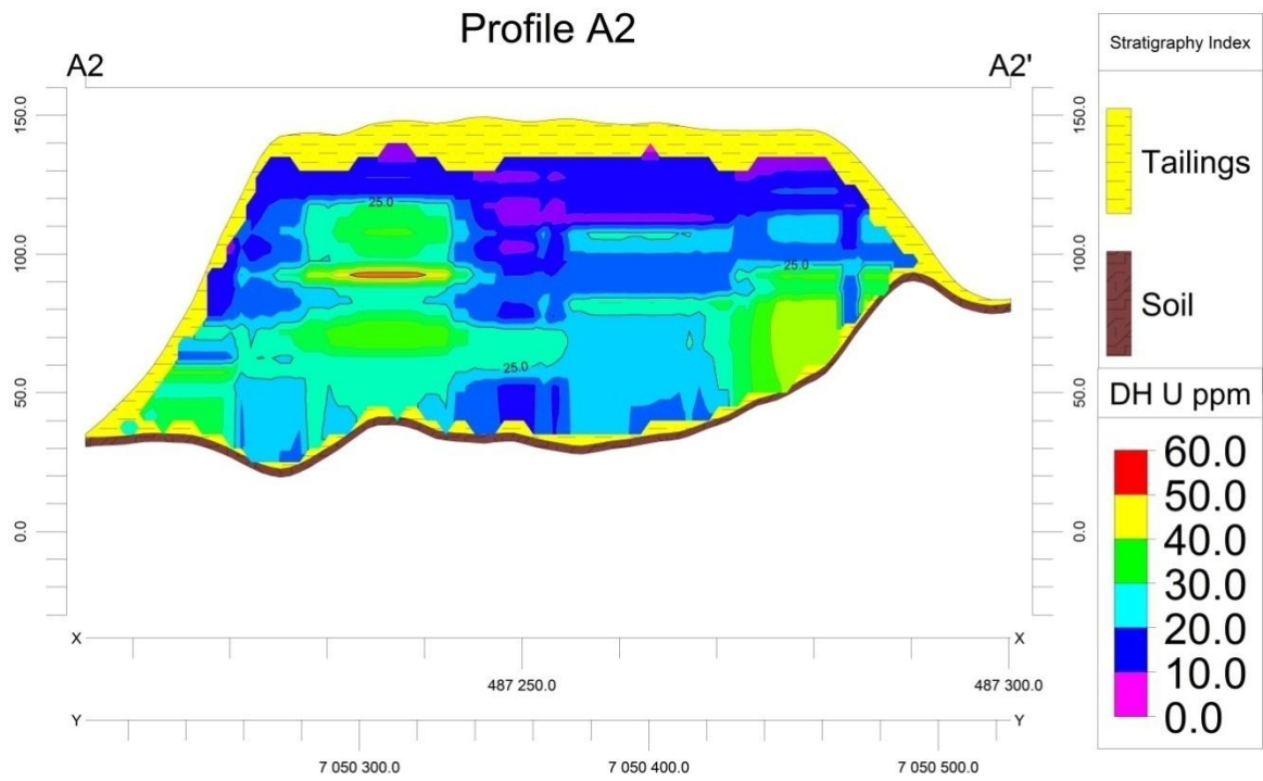
Figure A.7: Profile A2, New Machavie down-hole spectrometry
