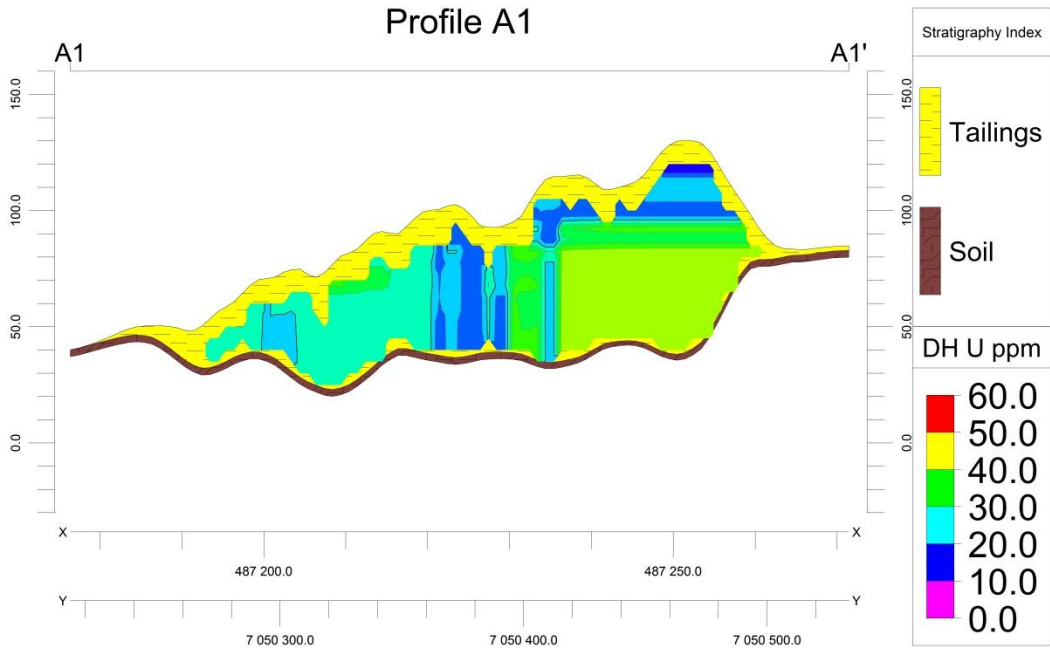
Figure A.6: Profile A1, New Machavie down-hole spectrometry
