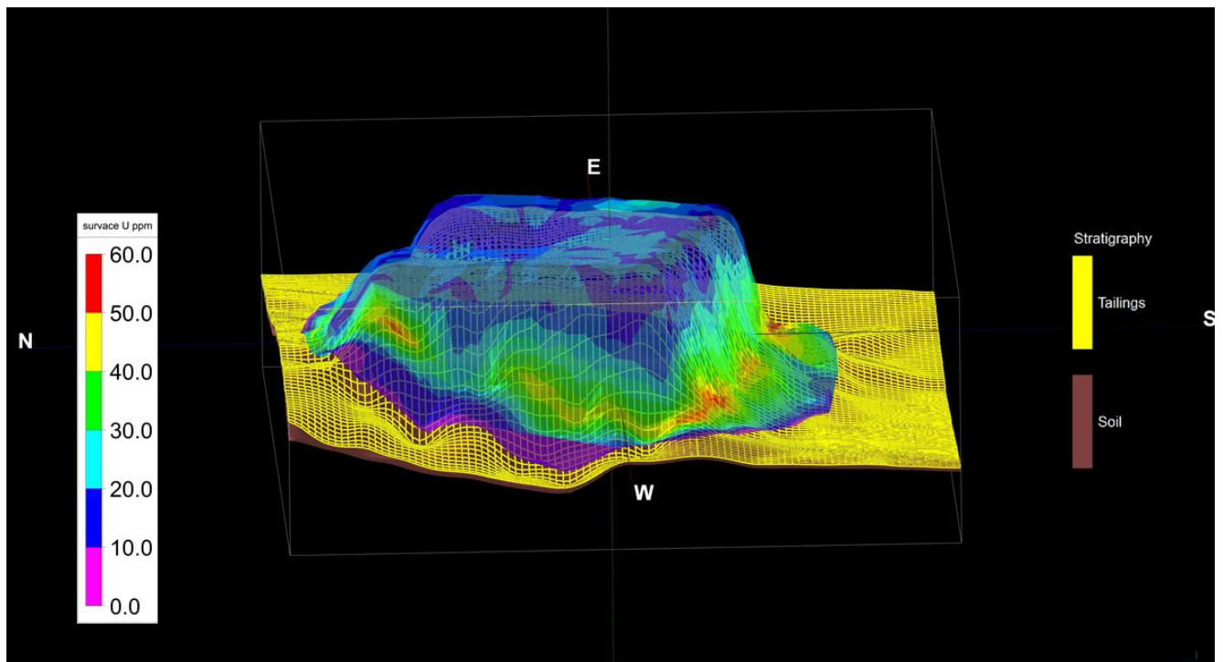
Figure C.4: Surface spectrometry results, west-east view
