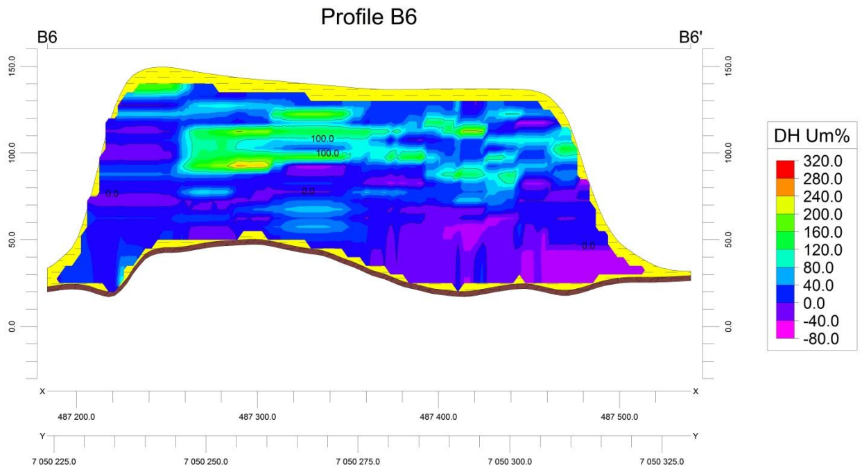
Figure D.19: Um% profile B6
