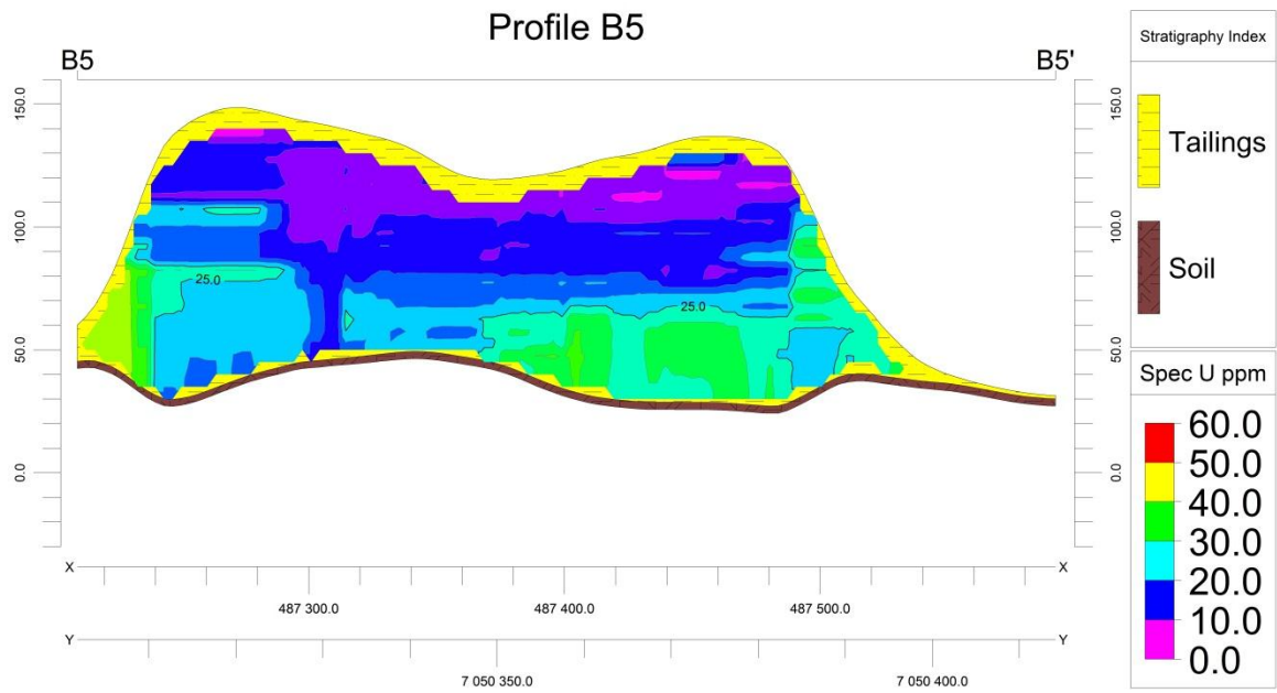
Figure A.21: Profile B5, New Machavie down-hole spectrometry
