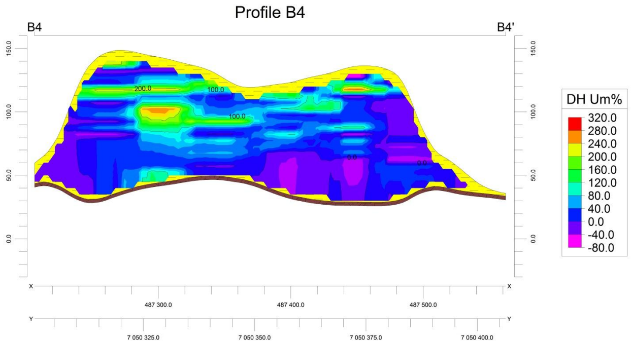
Figure D.17: Um% profile B4
