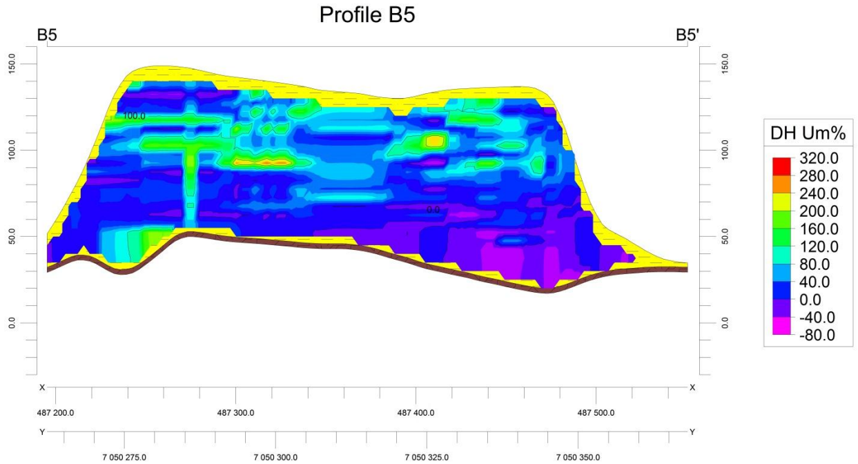
Figure D.18: Um% profile B5
