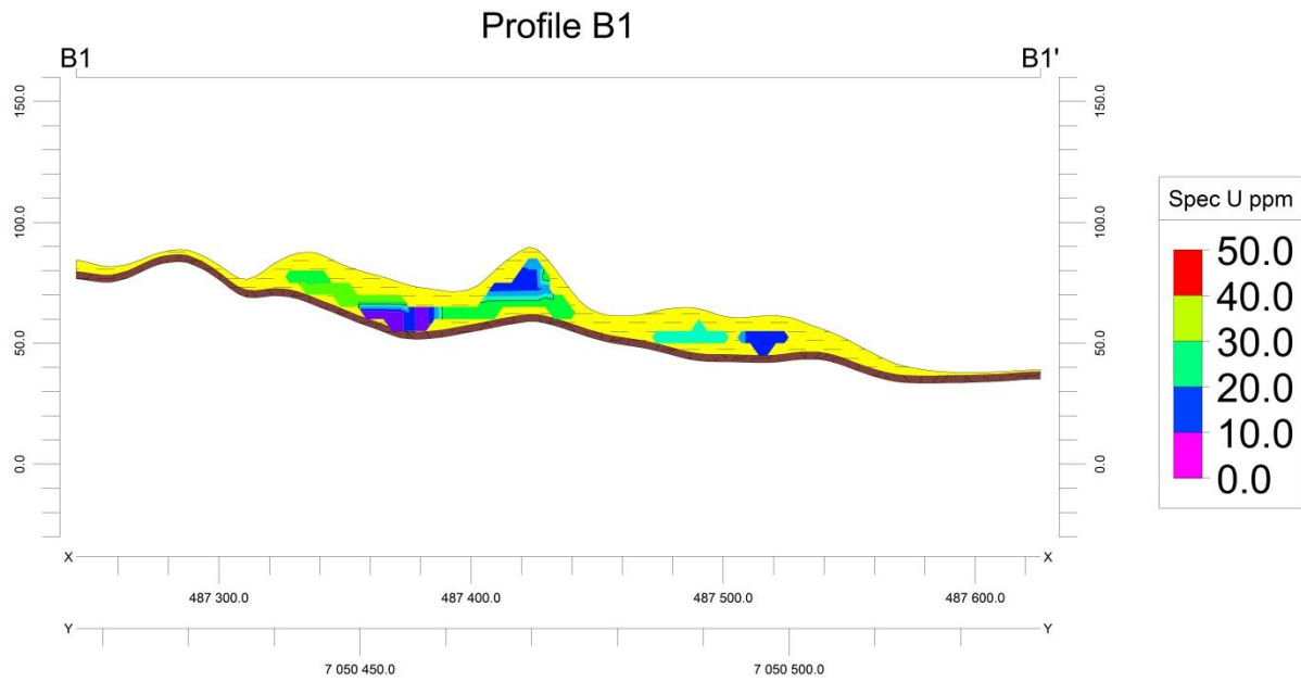
Figure B.13: Profile B1, Laboratory spectrometry model
