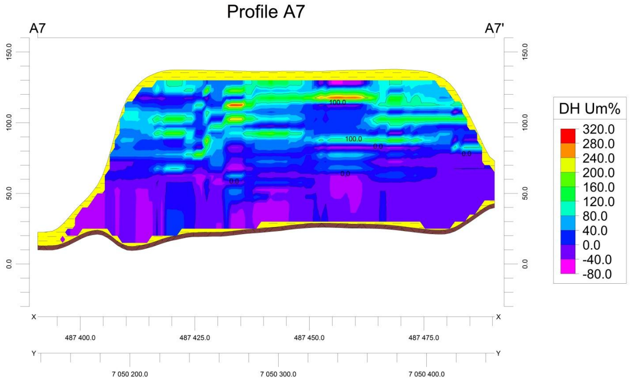
Figure D.12: Um% profile A7
