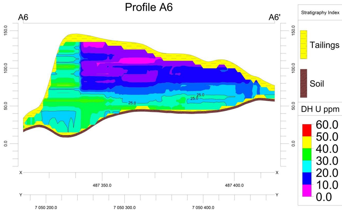
Figure A.11: Profile A6, New Machavie down-hole spectrometry
