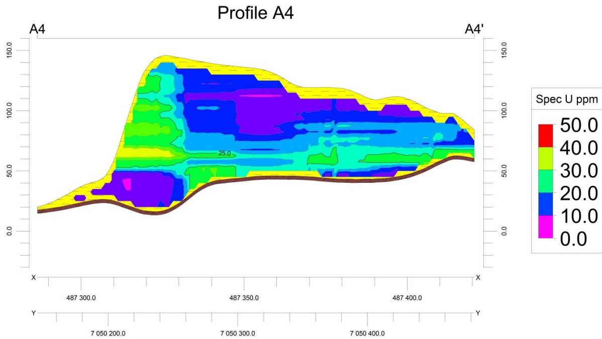
Figure B.9: Profile A4, Laboratory spectrometry model
