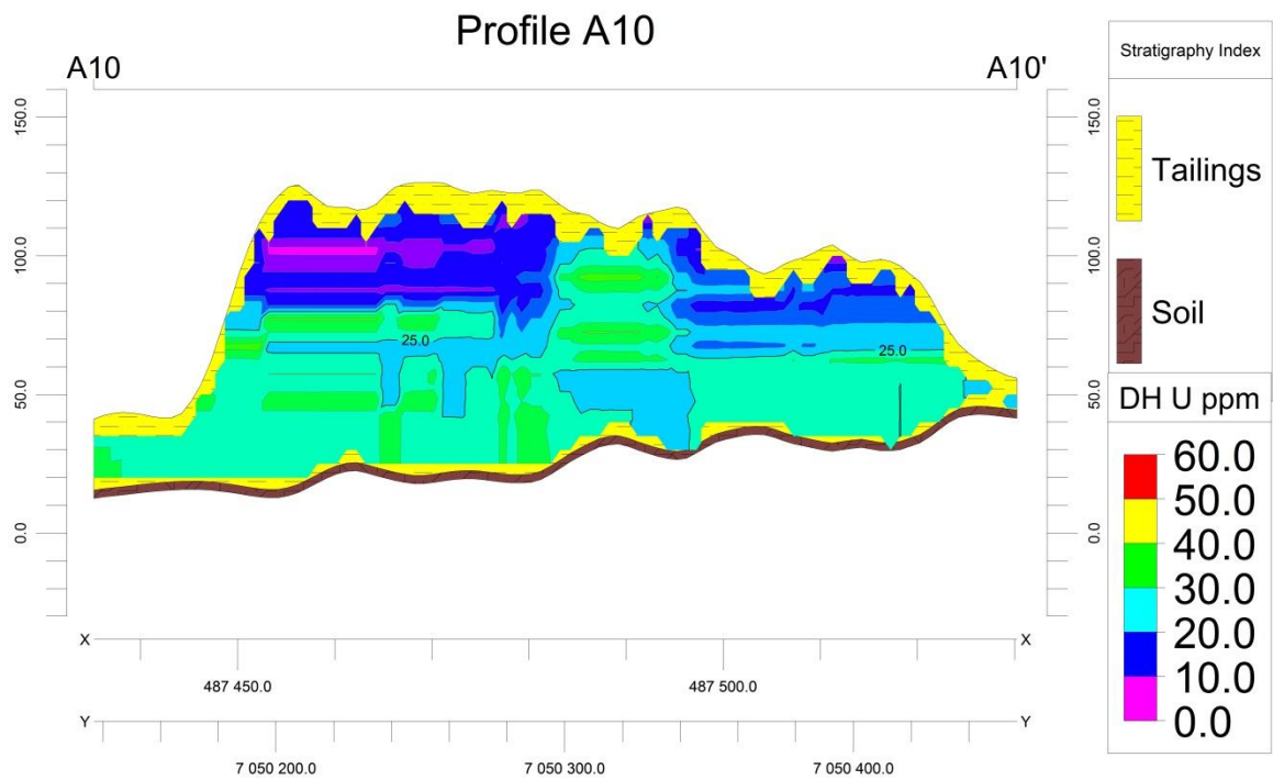
Figure A.15: Profile A10, New Machavie down-hole spectrometry
