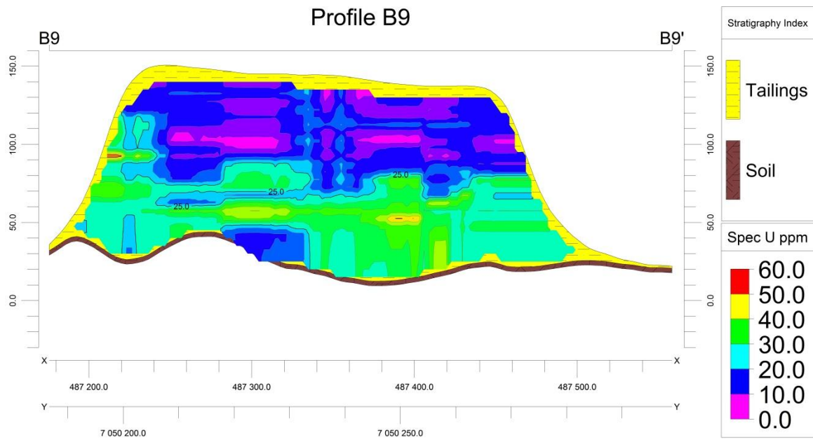
Figure A.25: Profile B9, New Machavie down-hole spectrometry
